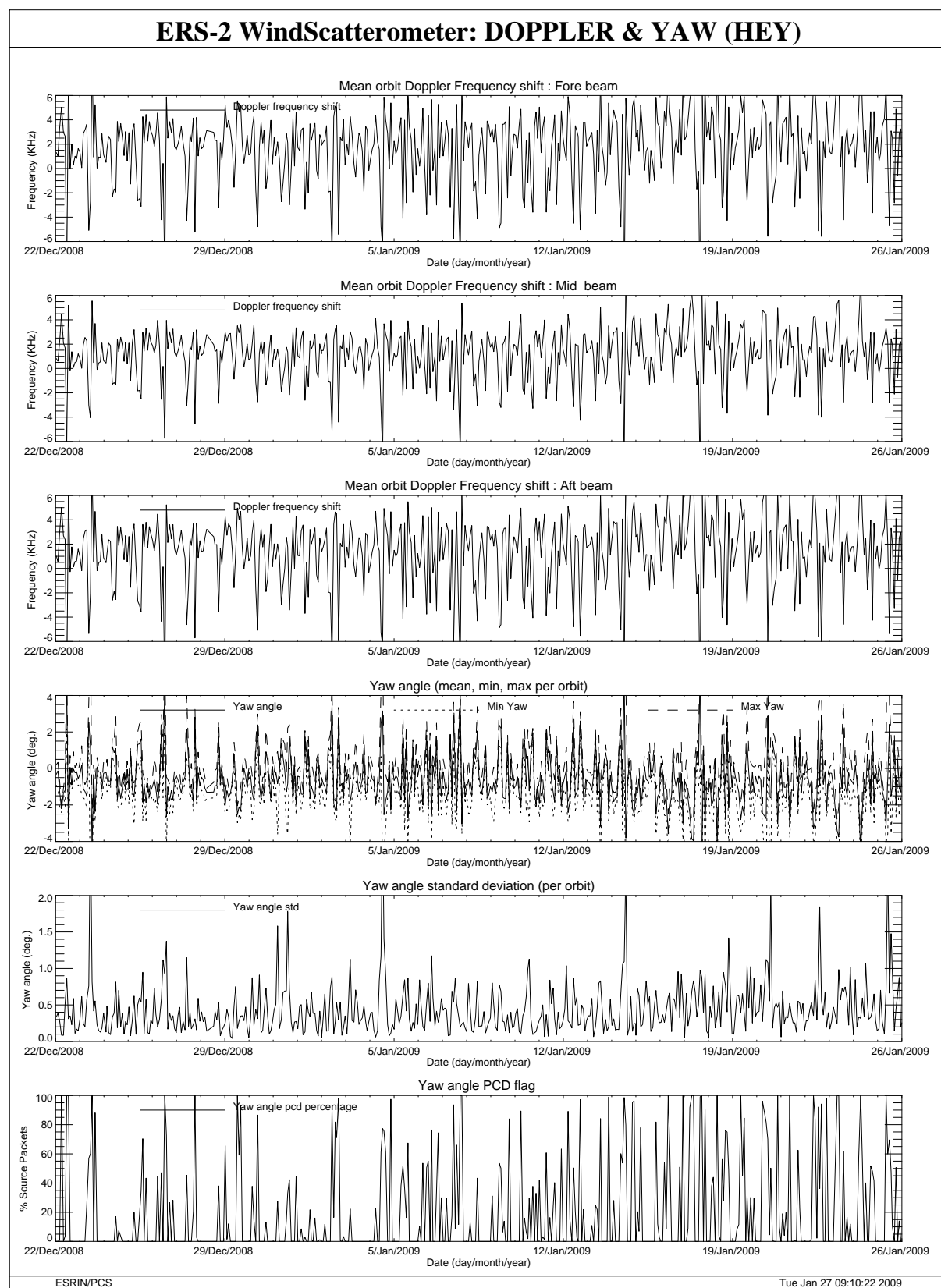
FIGURE 29 Doppler frequency shift and Yaw error angle evolution cycle 143.
