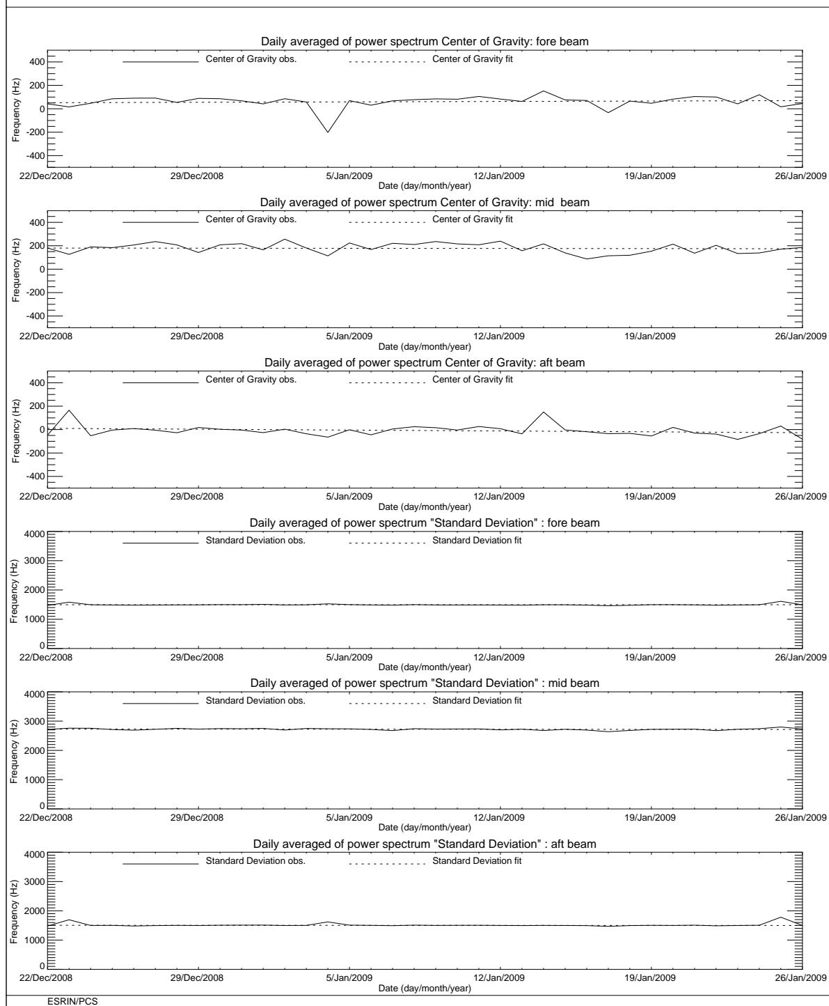
FIGURE 3 ERS-2 Scatterometer: Centre of Gravity and standard deviation of received power spectrum for cycle 143.
