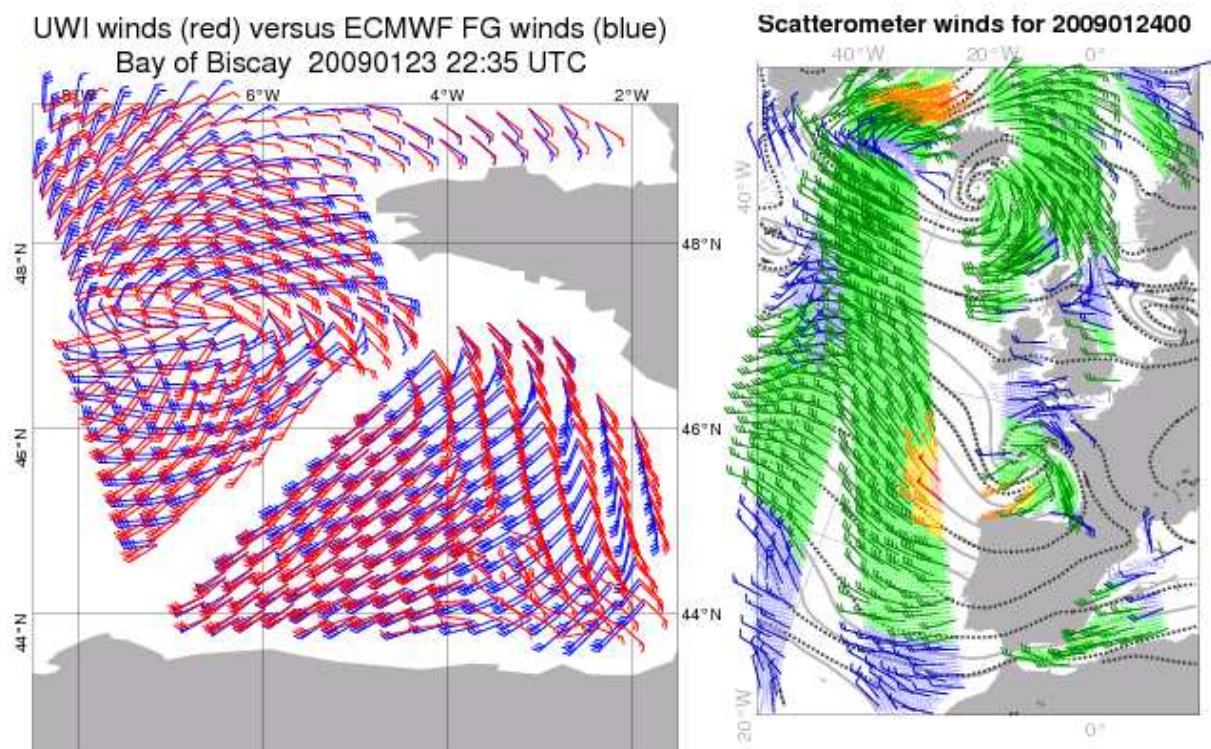
FIGURE 20 Comparison between UWI winds (in red) and ECMWF FG winds (in blue) for a case in the Bay of Biscay on 23 rd January 2009 (left panel), and the usage of all scatterometer data at ECMWF available in the 6-hourly batch centred around 00UTC 24January 2009. The track running through the low at Iceland and the Bay of Biscay, and the track west of Norway concerns ERS-2 data, the other tracks originate from ASCAT.
