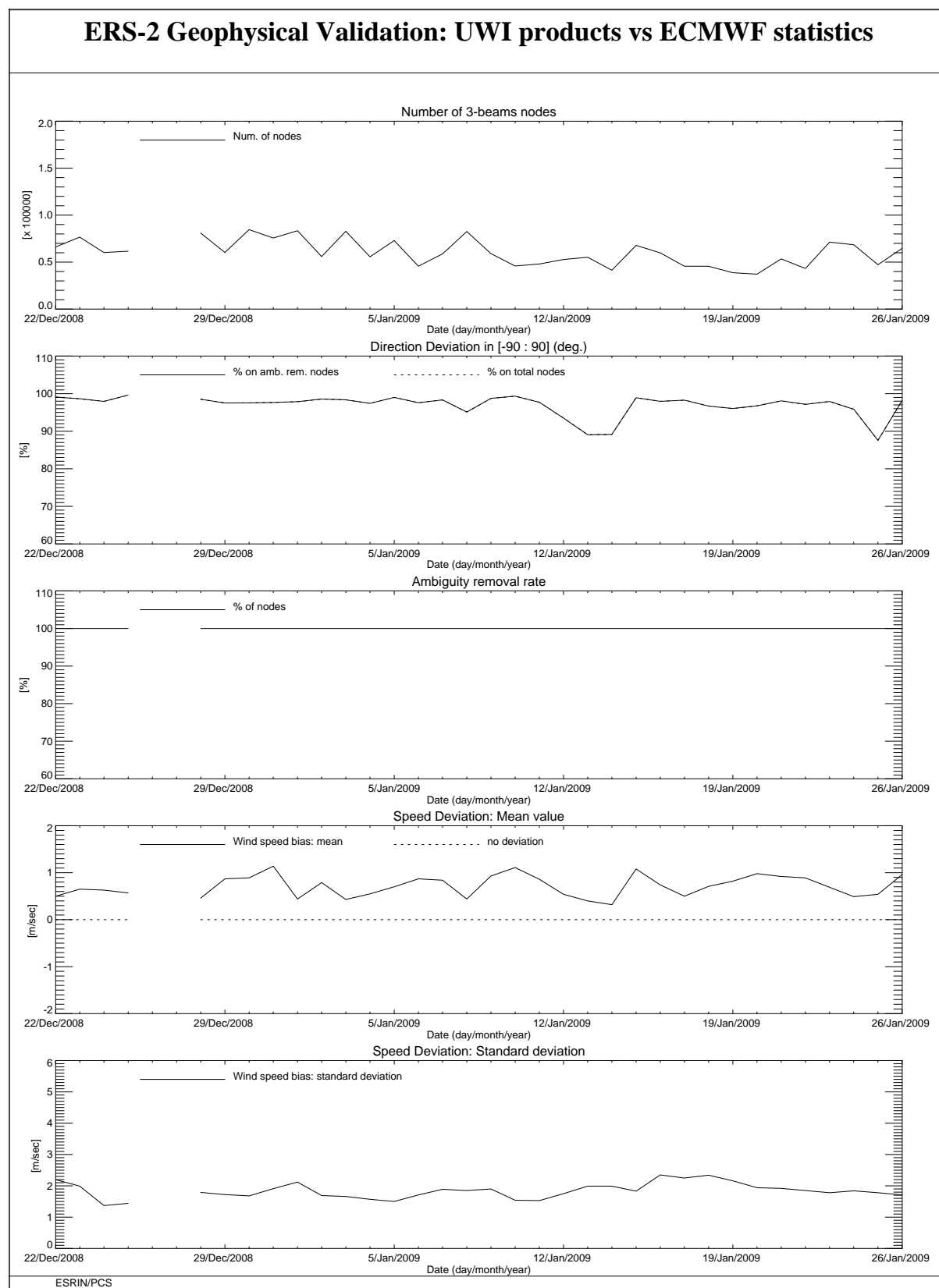
FIGURE 10 ERS-2 Scatterometer: wind products performance for cycle 143.
