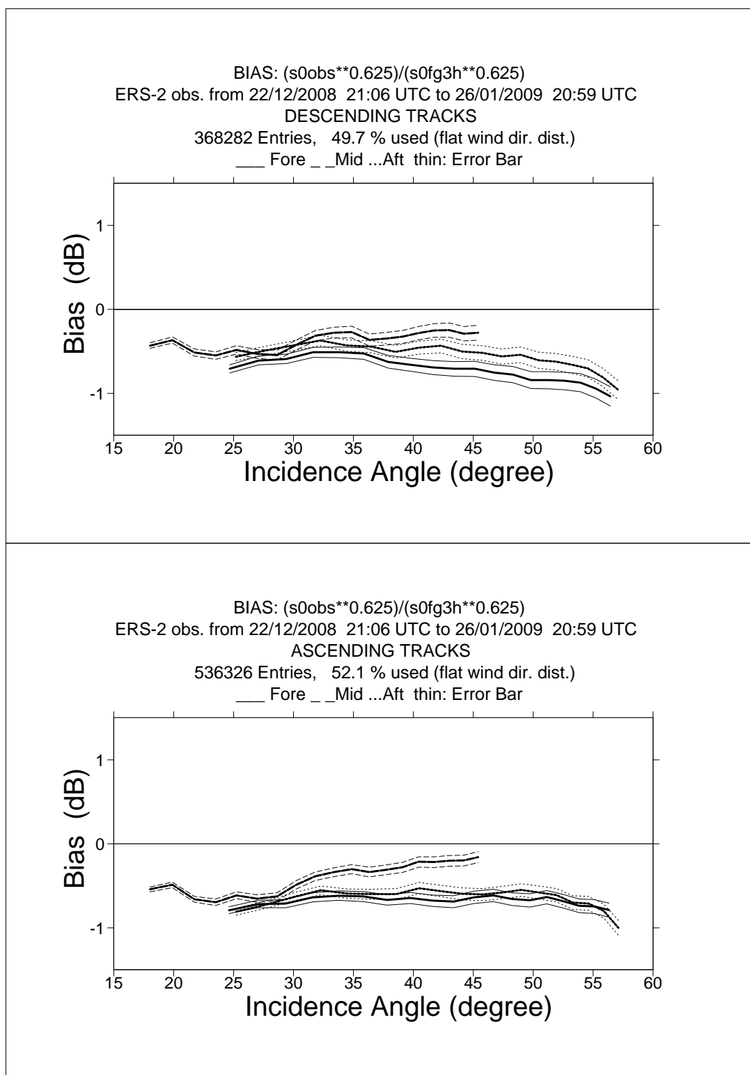
FIGURE 1 ERS-2 Scatterometer Ocean Calibration cycle 143. Ratio of \langle \sigma_0^{0.625} \rangle / \langle \text{CMOD4}(\text{First Guess})^{0.625} \rangle converted in dB for the fore beam (solid line), mid beam (dashed line) an aft beam (dotted line), as a function of incidence angle for descending and ascending tracks. The thin lines indicate the error bars on the estimated mean. First-guess winds are based on the in time closest (+3h, +6h, +9h, or +12h) T511 forecast field, and are bilinearly interpolated in space.
