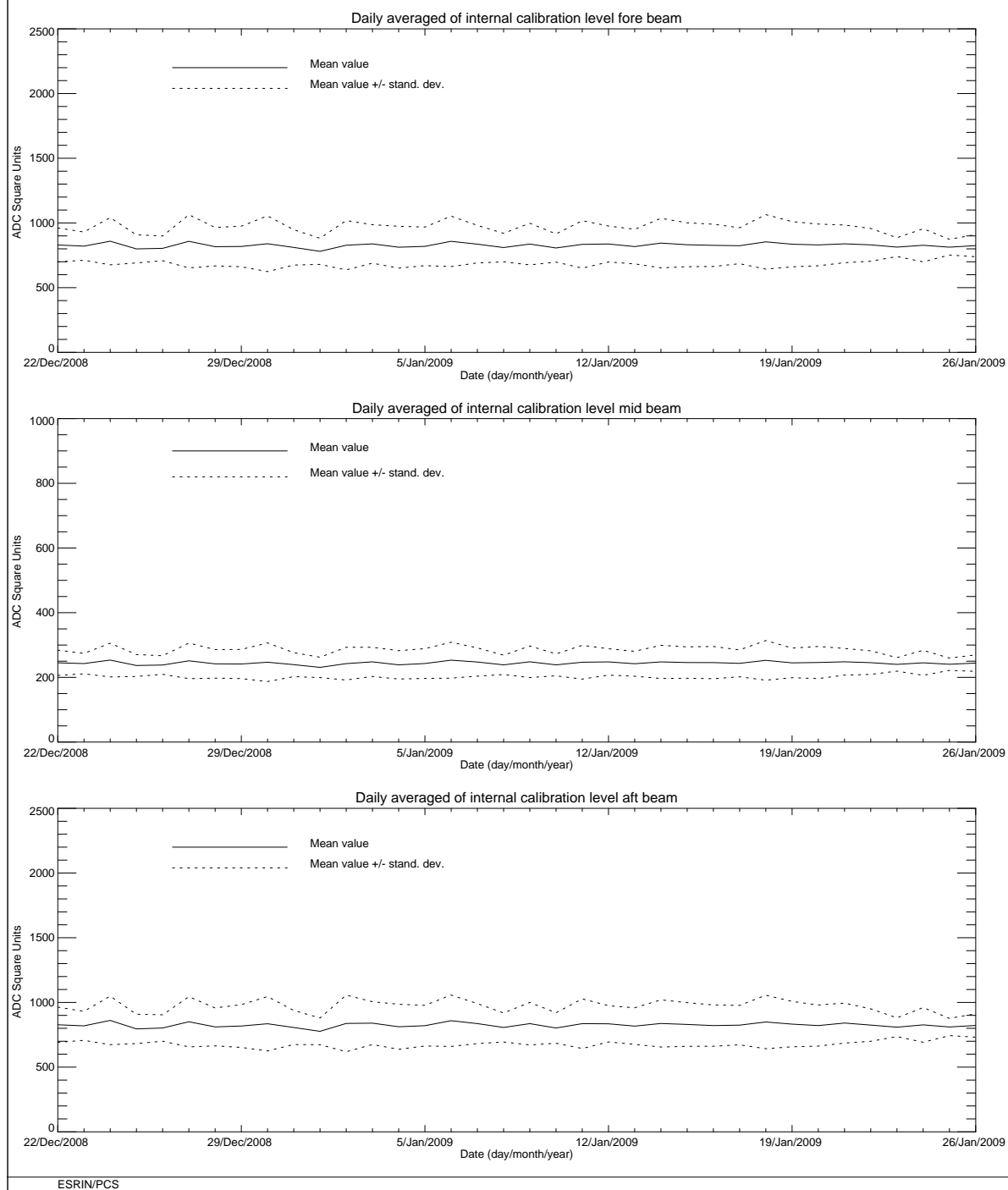
FIGURE 7 ERS-2 Scatterometer: power of internal calibration level cycle 143.
