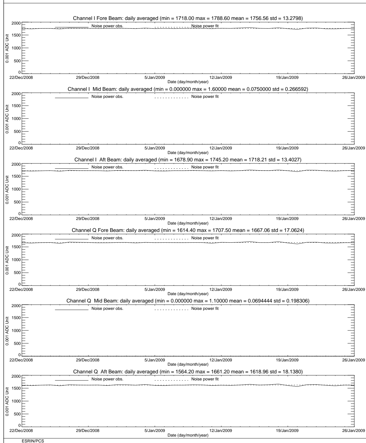
FIGURE 5 ERS-2 Scatterometer: noise power I and Q channel for cycle 143.
