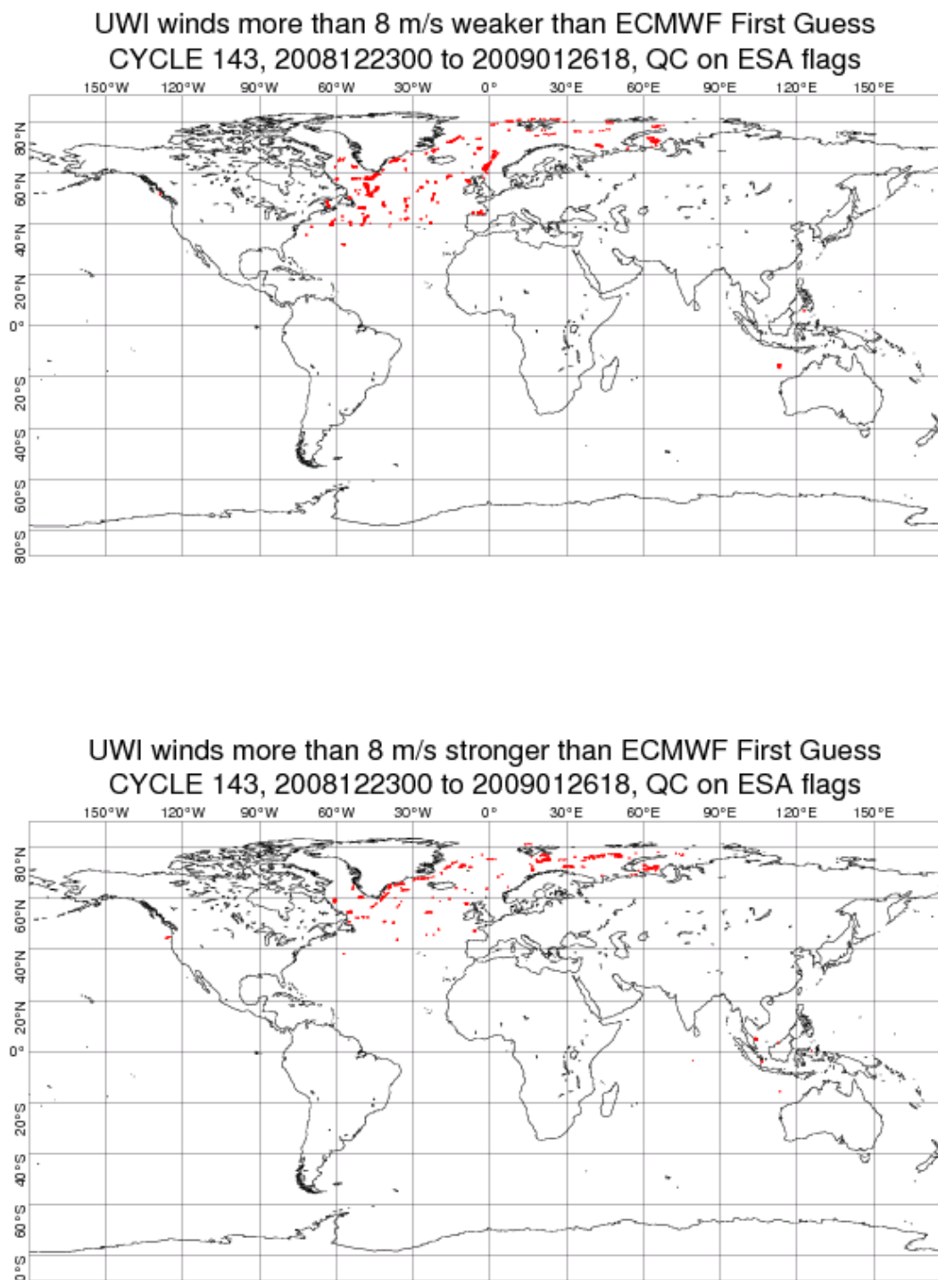
FIGURE 19 Locations of data during cycle 143 for which UWI winds are more than 8 m/s weaker (top panel) respectively stronger (lower panel) than FGAT, and on which QC on UWI flags and the ECMWF land/sea-ice mask was applied.
