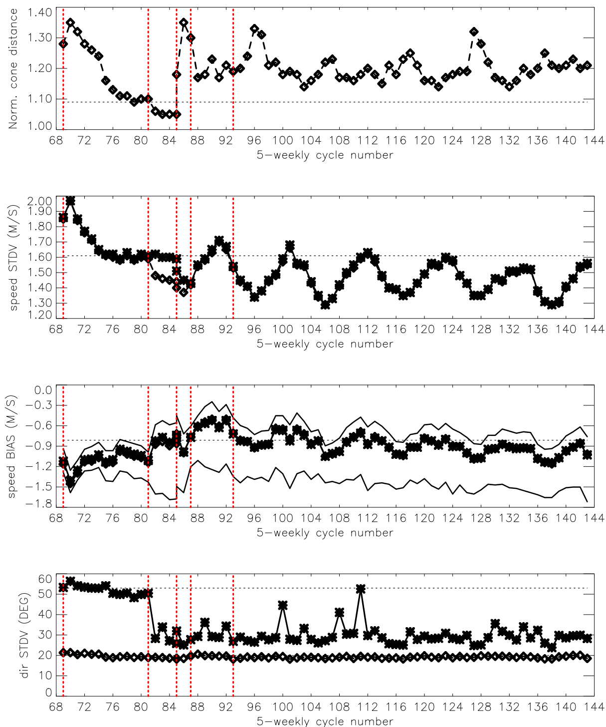
FIGURE 11 Evolution of the performance of the ERS-2 Scatterometer averaged over 5-weekly cycles from 12 December 2001 (cycle 69) to 26 January 2009 (end cycle 143) for the UWI product (solid, star) and de-aliased winds based on CMOD4 (dashed, diamond). Results are based on data that passed the UWI QC flags. For cycle 85 two values are plotted; the first value for the global set, the second one for the regional set. Dotted lines represent values for cycle 59 (5 December 2000 to 17 January 2001), i.e. the last stable cycle of the nominal period. From top to bottom panel are shown the normalized distance to the one (CMOD4 only) the standard deviation of the wind speed compared to FG winds, the corresponding bias (for UWI winds the extreme inter-node averages are shown as well), and the standard deviation of wind direction compared to FG.
