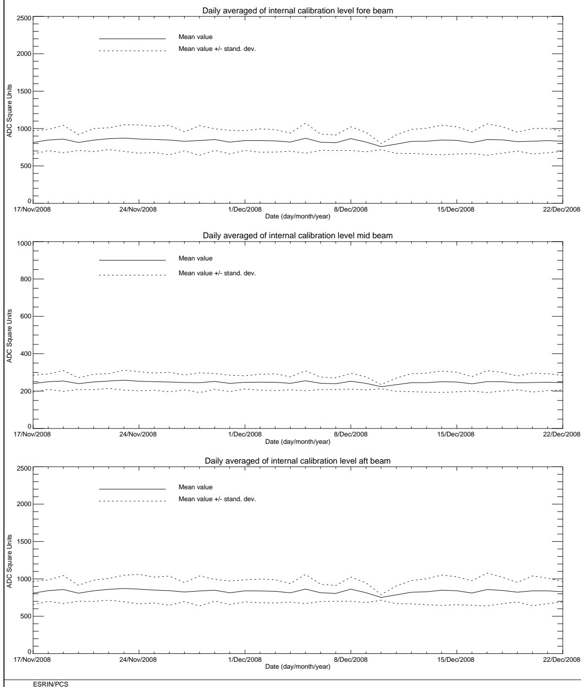
FIGURE 7 ERS-2 Scatterometer: power of internal calibration level cycle 142.
