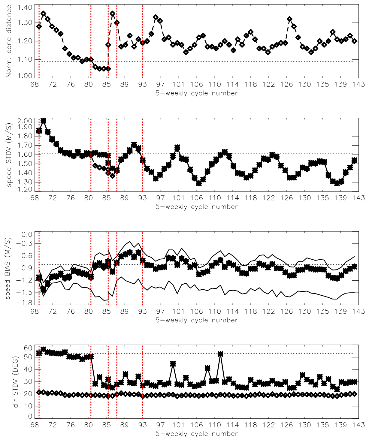
FIGURE 11 Evolution of the performance of the ERS-2 Scatterometer averaged over 5-weekly cycles from 12 December 2001 (cycle 69) to 22 December 2008 (end cycle 142) for the UWI product (solid, star) and de-aliased winds based on CMOD4 (dashed, diamond). Results are based on data that passed the UWI QC flags. For cycle 85 two values are plotted; the first value for the global set, the second one for the regional set. Dotted lines represent values for cycle 59 (5 December 2000 to 17 January 2001), i.e. the last stable cycle of the nominal period. From top to bottom panel are shown the normalized distance to the one (CMOD4 only) the standard deviation of the wind speed compared to FG winds, the corresponding bias (for UWI winds the extreme inter-node averages are shown as well), and the standard deviation of wind direction compared to FG.
