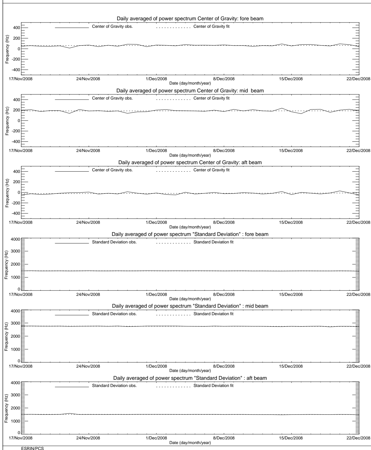
FIGURE 3 ERS-2 Scatterometer: Centre of Gravity and standard deviation of received power spectrum for cycle 142.
