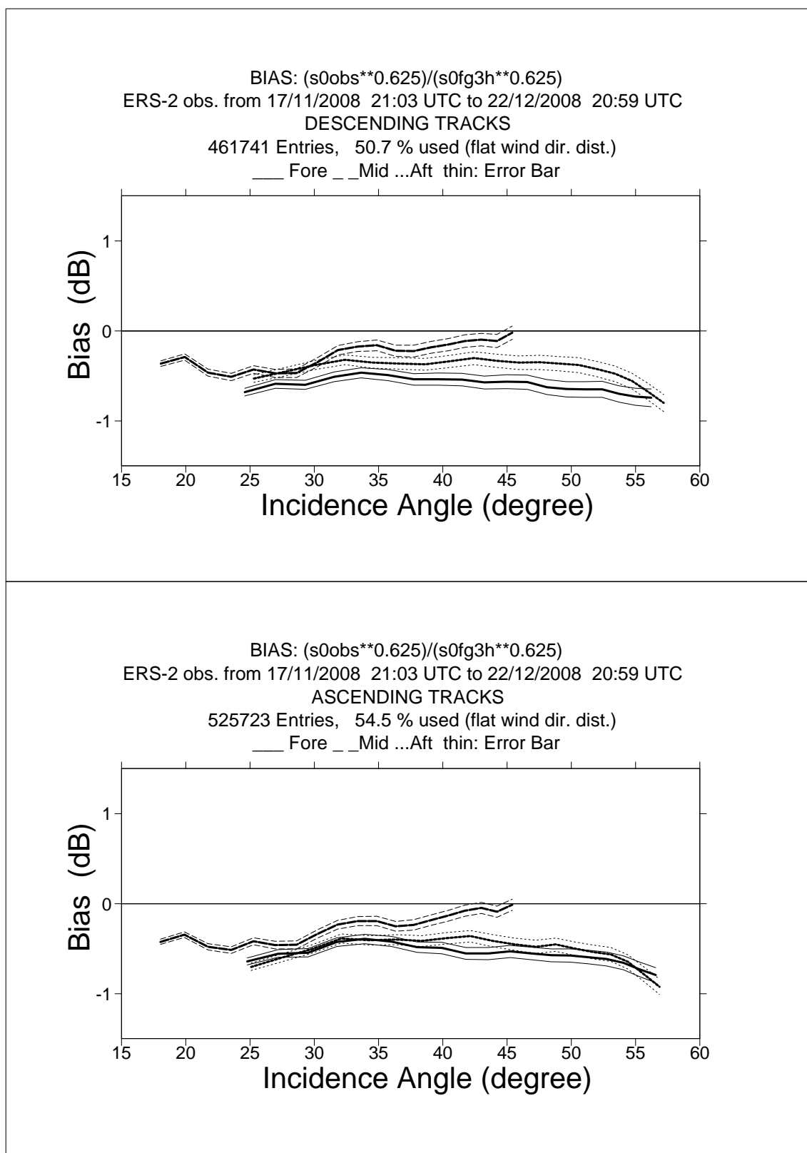
FIGURE 1 ERS-2 Scatterometer Ocean Calibration cycle 142. Ratio of \langle \sigma_0^{0.625} \rangle / \langle \text{CMOD4}(\text{First Guess})^{0.625} \rangle converted in dB for the fore beam (solid line), mid beam (dashed line) and aft beam (dotted line), as a function of incidence angle for descending and ascending tracks. The thin lines indicate the error bars on the estimated mean. First-guess winds are based on the in time closest (+3h, +6h, +9h, or +12h) T511 forecast field, and are bilinearly interpolated in space.
