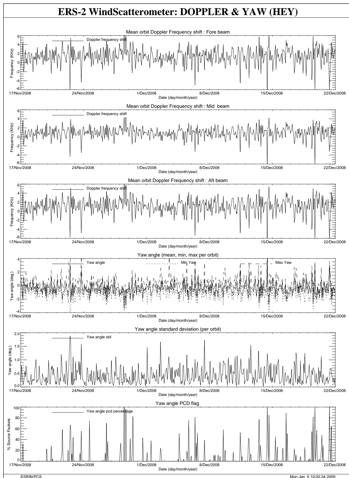
FIGURE 29 Doppler frequency shift and Yaw error angle evolution cycle 142.
