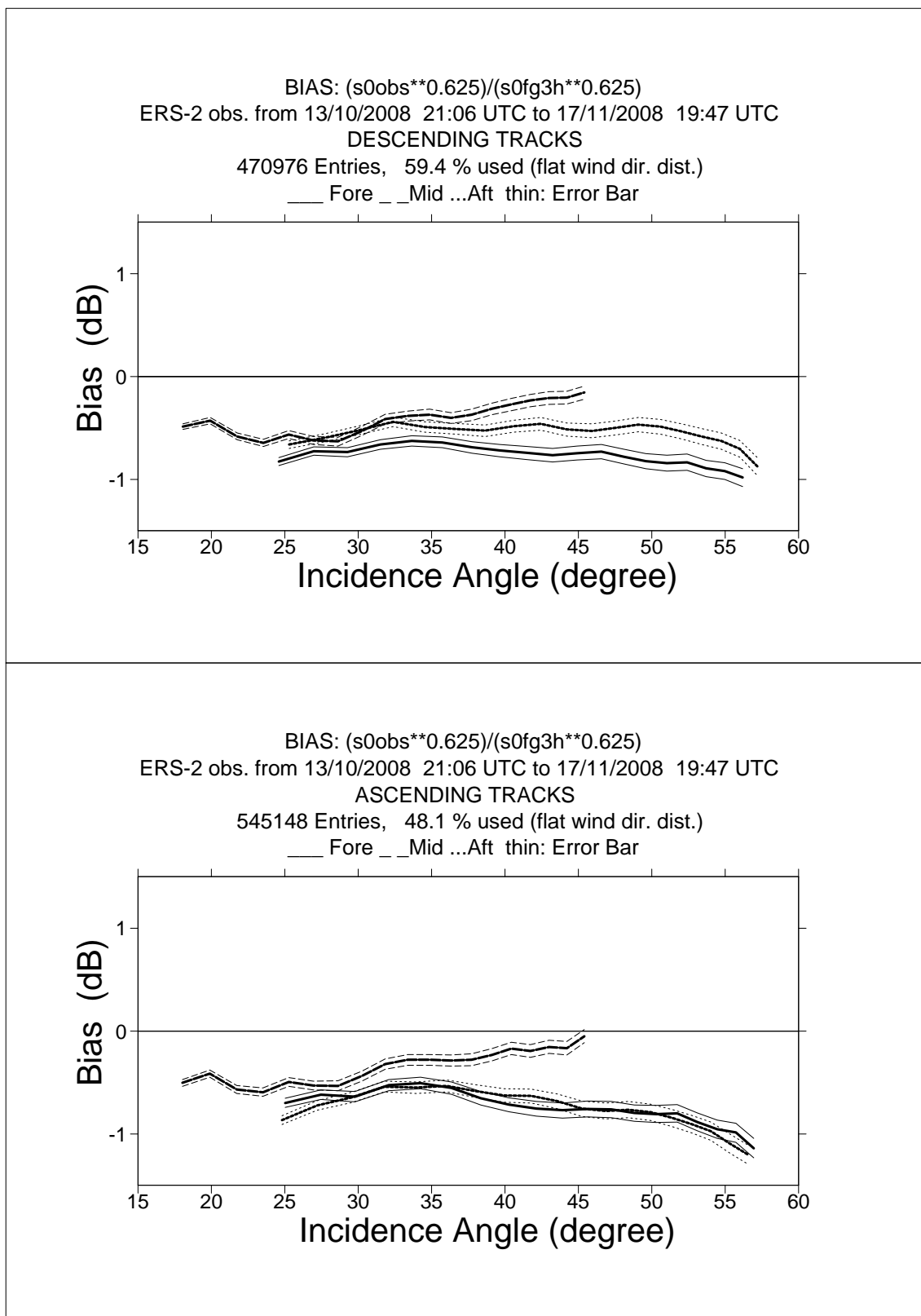
FIGURE 1 ERS-2 Scatterometer Ocean Calibration cycle 141. Ratio of \langle \sigma_0^{0.625} \rangle / \langle CMOD4(\text{First Guess})^{0.625} \rangle converted in dB for the fore beam (solid line), mid beam (dashed line) an aft beam (dotted line), as a function of incidence angle for descending and ascending tracks. The thin lines indicate the error bars on the estimated mean. First-guess winds are based on the in time closest (+3h, +6h, +9h, or +12h) T511 forecast field, and are bilinearly interpolated in space.
