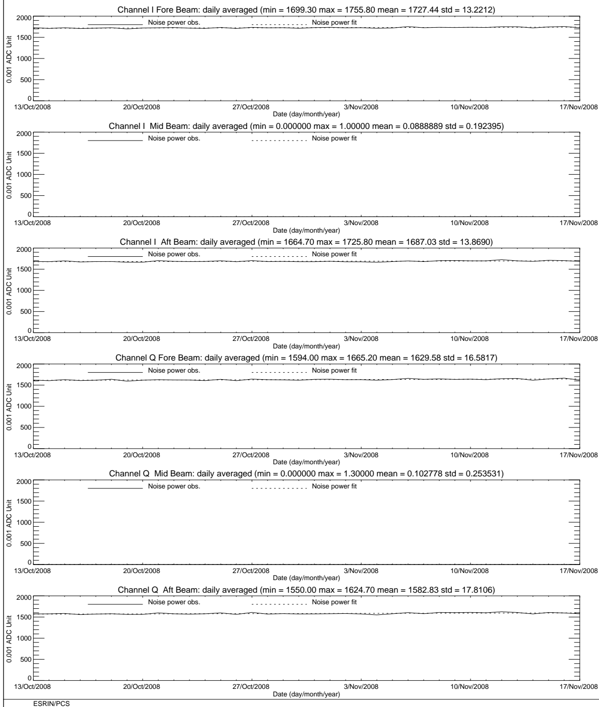
FIGURE 5 ERS-2 Scatterometer: noise power I and Q channel for cycle 141.
