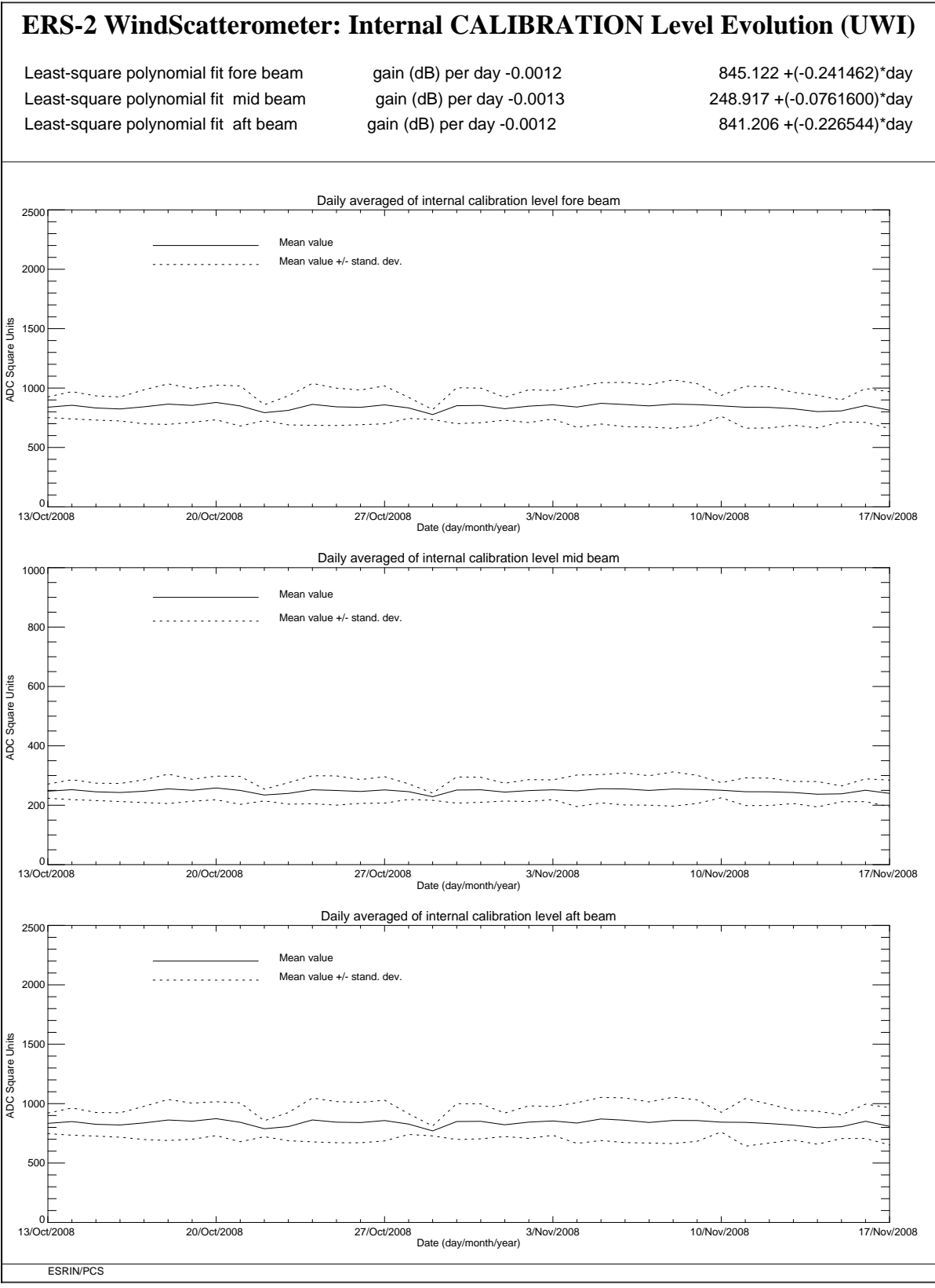
FIGURE 7 ERS-2 Scatterometer: power of internal calibration level cycle 141.
