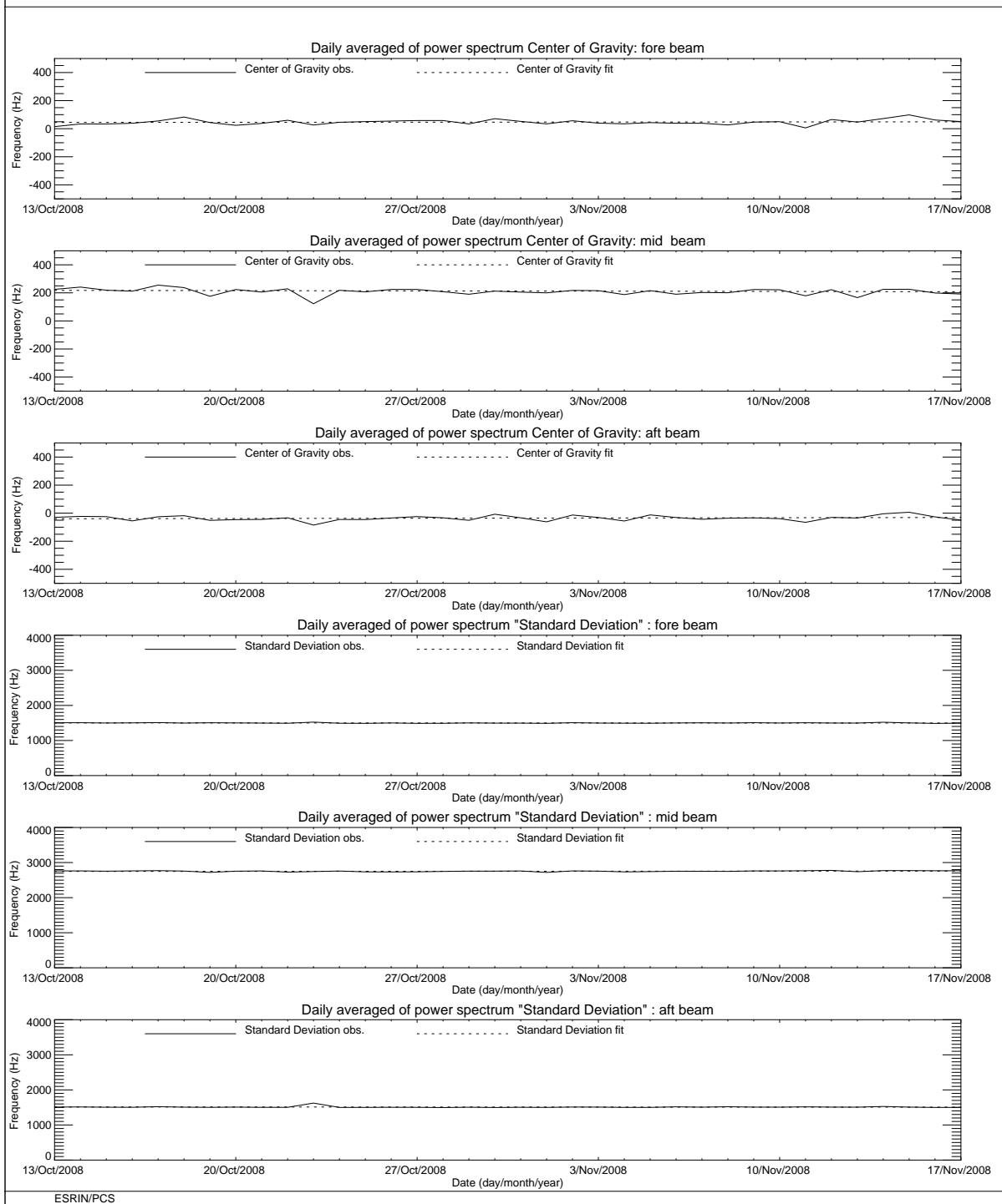
FIGURE 3 ERS-2 Scatterometer: Centre of Gravity and standard deviation of received power spectrum for cycle 141.
