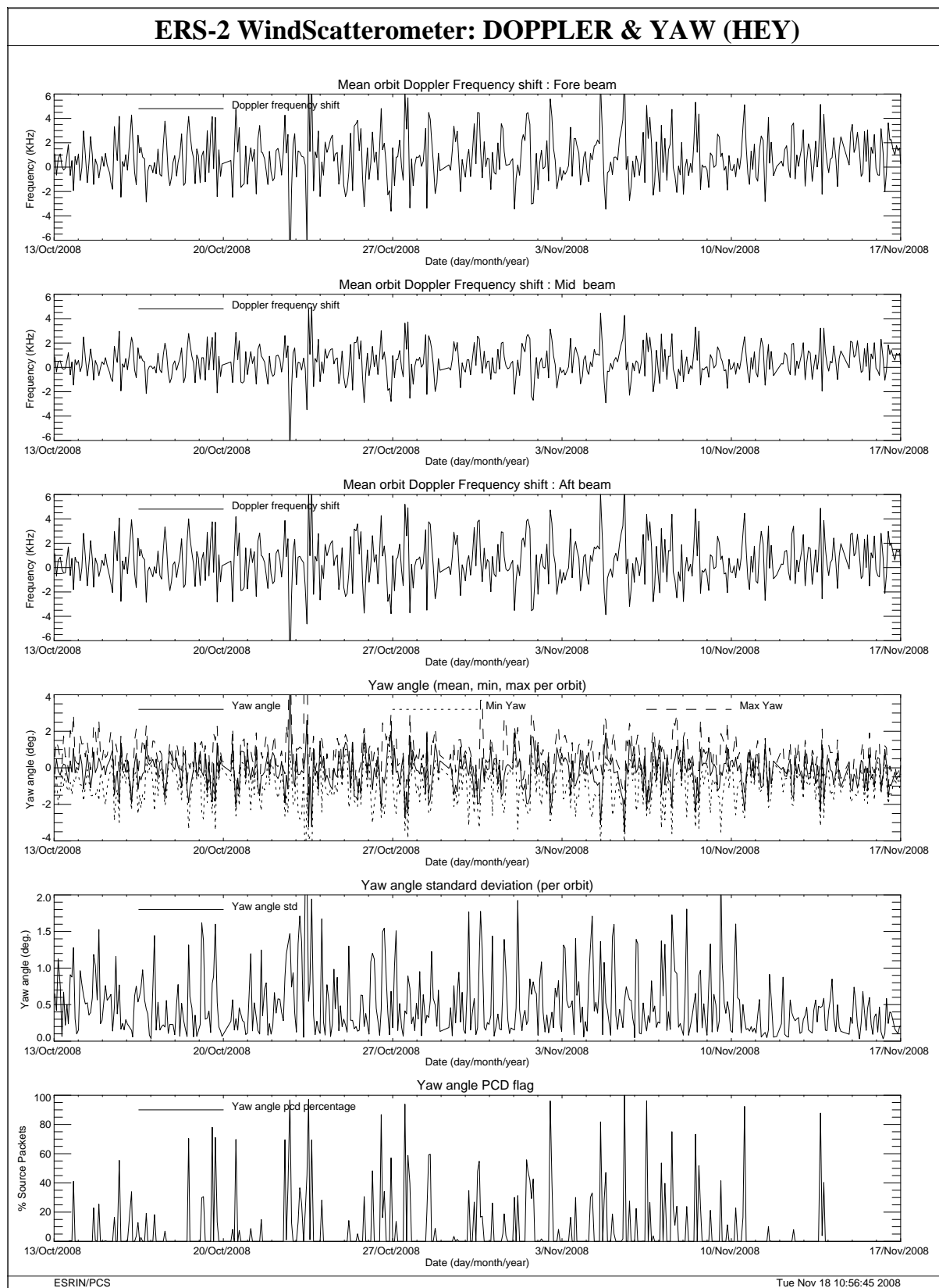
FIGURE 29 Doppler frequency shift and Yaw error angle evolution cycle 141.
