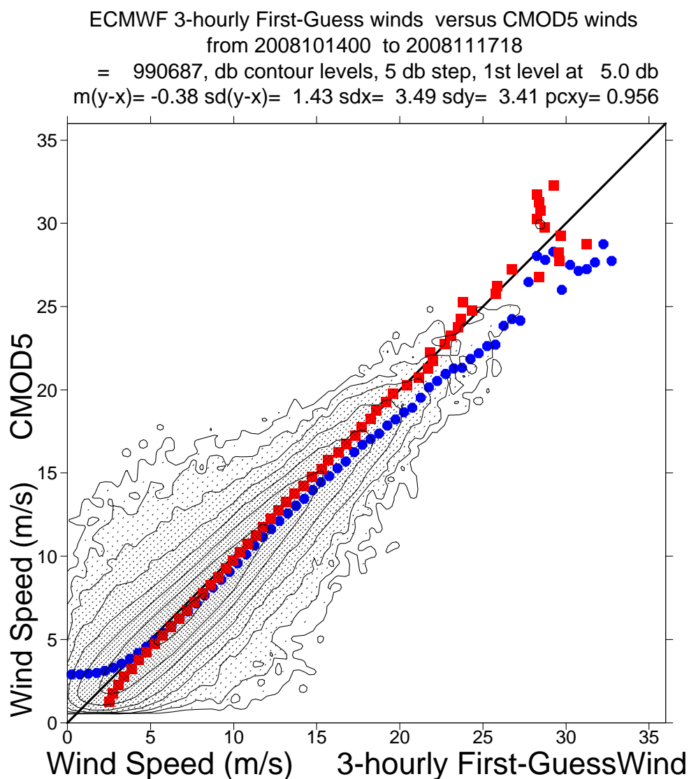
FIGURE 24 Same as Fig. 21, but for de-aliased CMOD5 winds.
