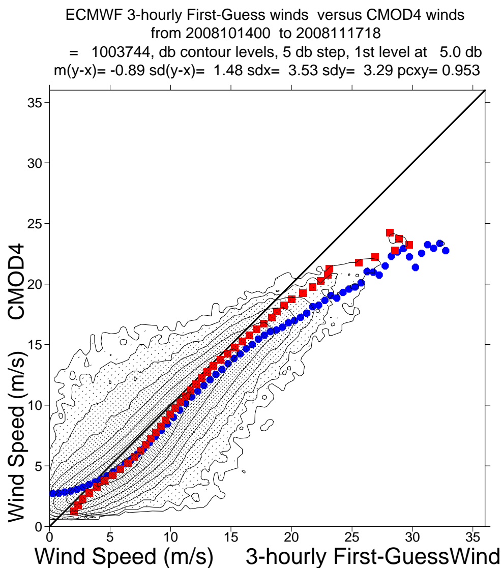
FIGURE 23 Same as Fig. 21, but for de-aliased CMOD4 winds.
