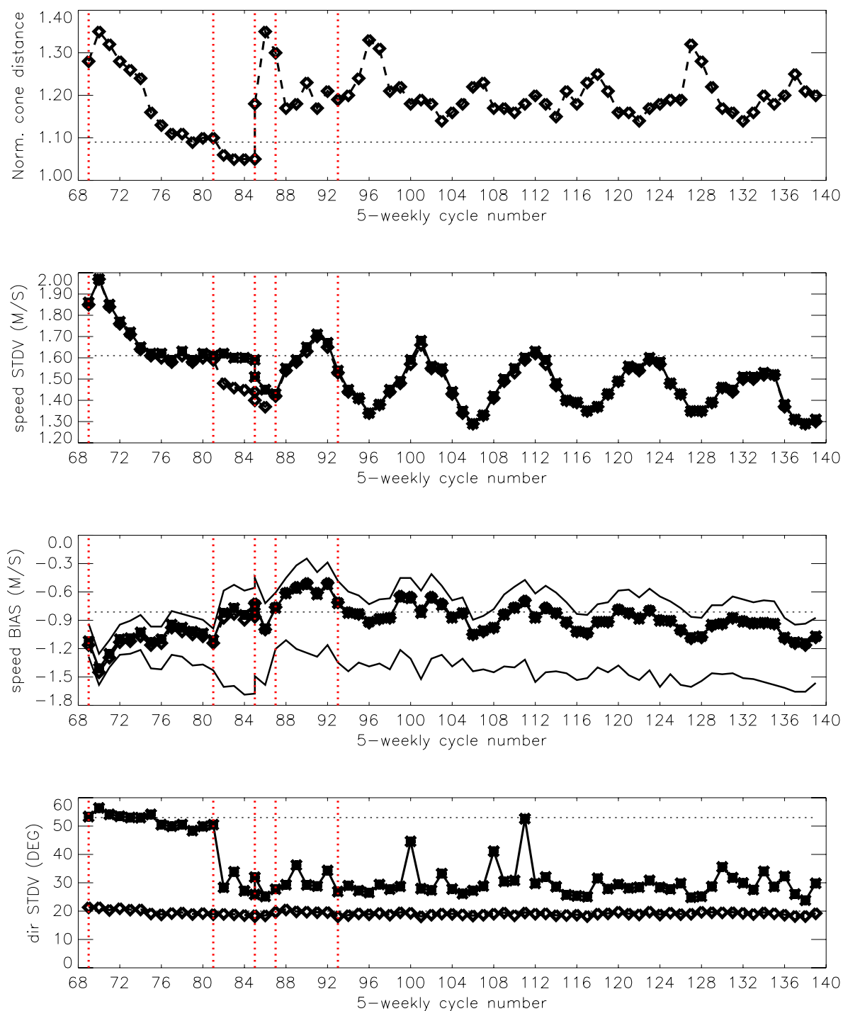
FIGURE 11 Evolution of the performance of the ERS-2 Scatterometer averaged over 5-weekly cycles from 12 December 2001 (cycle 69) to 8 September 2008 (end cycle 139) for the UWI product (solid, star) and de-aliased winds based on CMOD4 (dashed, diamond). Results are based on data that passed the UWI QC flags. For cycle 85 two values are plotted; the first value for the global set, the second one for the regional set. Dotted lines represent values for cycle 59 (5 December 2000 to 17 January 2001), i.e. the last stable cycle of the nominal period. From top to bottom panel are shown the normalized distance to the one (CMOD4 only) the standard deviation of the wind speed compared to FG winds, the corresponding bias (for UWI winds the extreme inter-node averages are shown as well), and the standard deviation of wind direction compared to FG.
