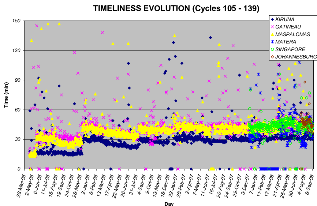
FIGURE 26 Timeliness evolution from 19 th April 2005 to 8 th September 2008 for Gatineau, Kiruna, Maspalomas, Matera, Singapore and Johannesburg ground stations.
