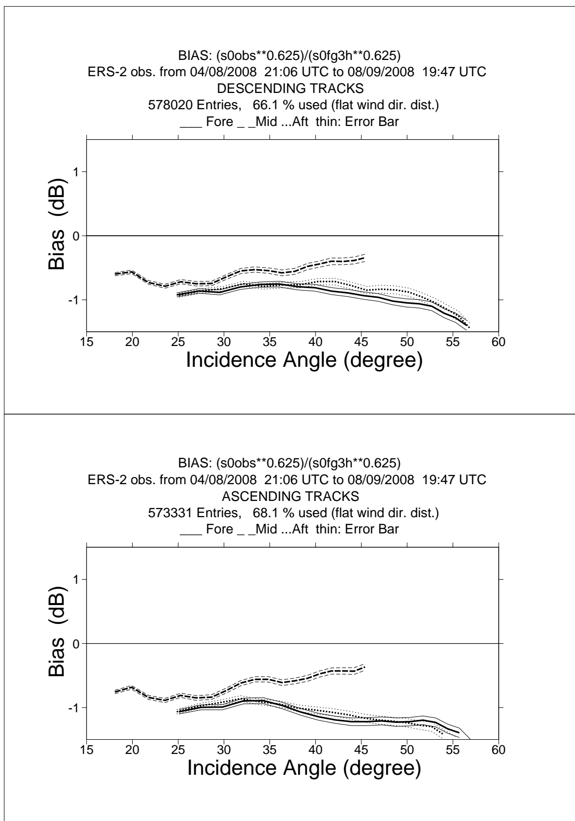
FIGURE 1 ERS-2 Scatterometer Ocean Calibration cycle 139. Ratio of \langle \sigma_0^{0.625} \rangle / \langle \text{CMOD4}(\text{First Guess})^{0.625} \rangle converted in dB for the fore beam (solid line), mid beam (dashed line) and aft beam (dotted line), as a function of incidence angle for descending and ascending tracks. The thin lines indicate the error bars on the estimated mean. First-guess winds are based on the in time closest (+3h, +6h, +9h, or +12h) T511 forecast field, and are bilinearly interpolated in space.
