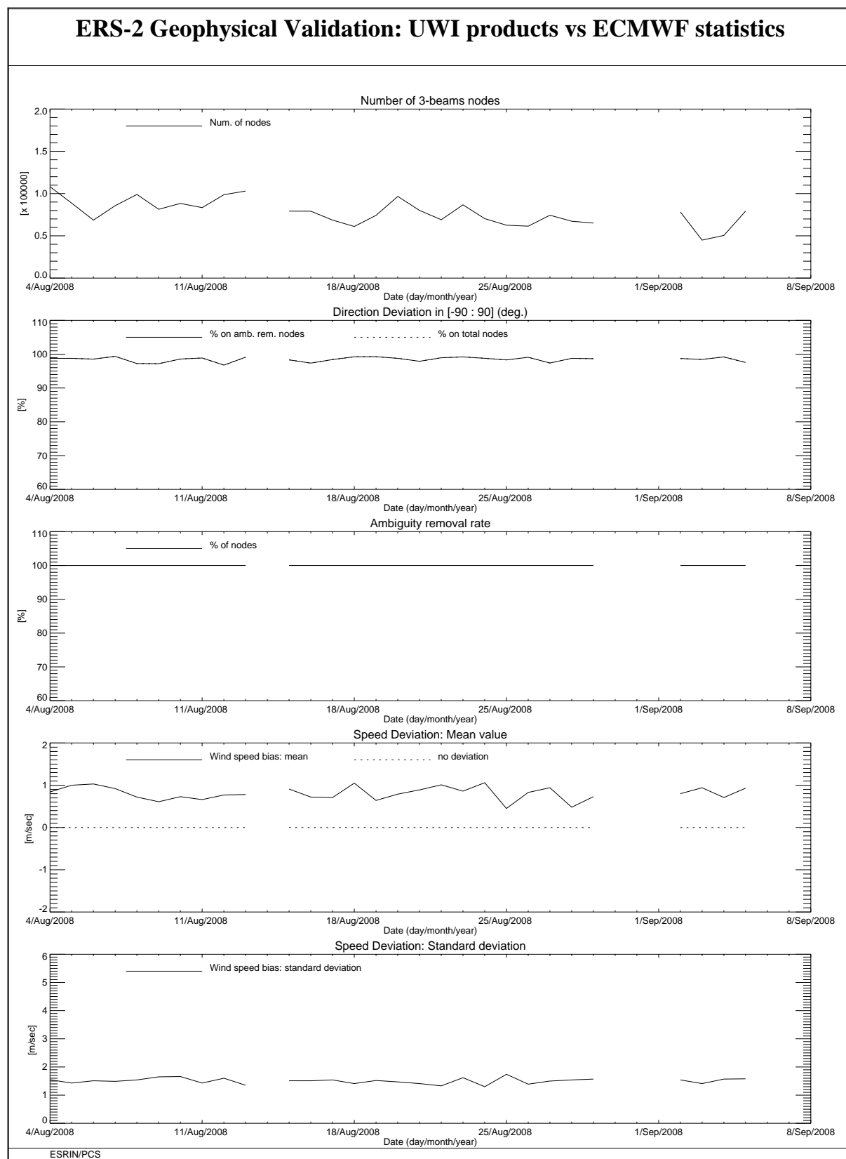
FIGURE 10 ERS-2 Scatterometer: wind products performance for cycle 139.
