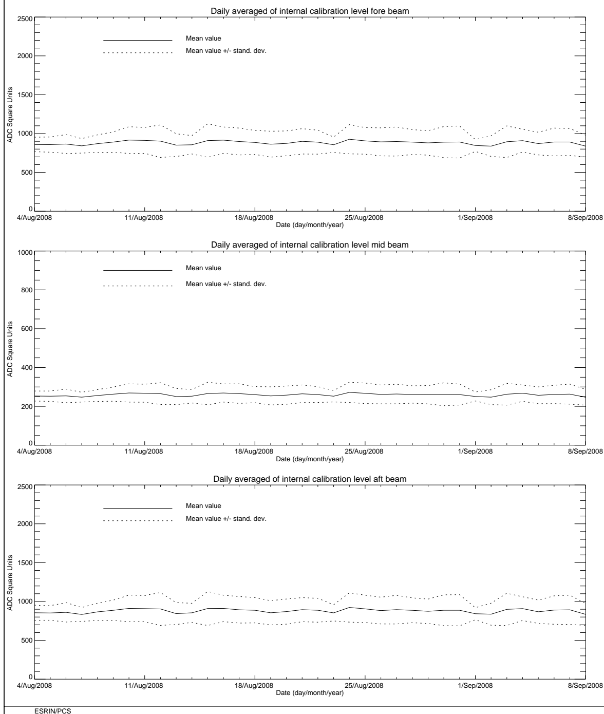
FIGURE 7 ERS-2 Scatterometer: power of internal calibration level cycle 139.
