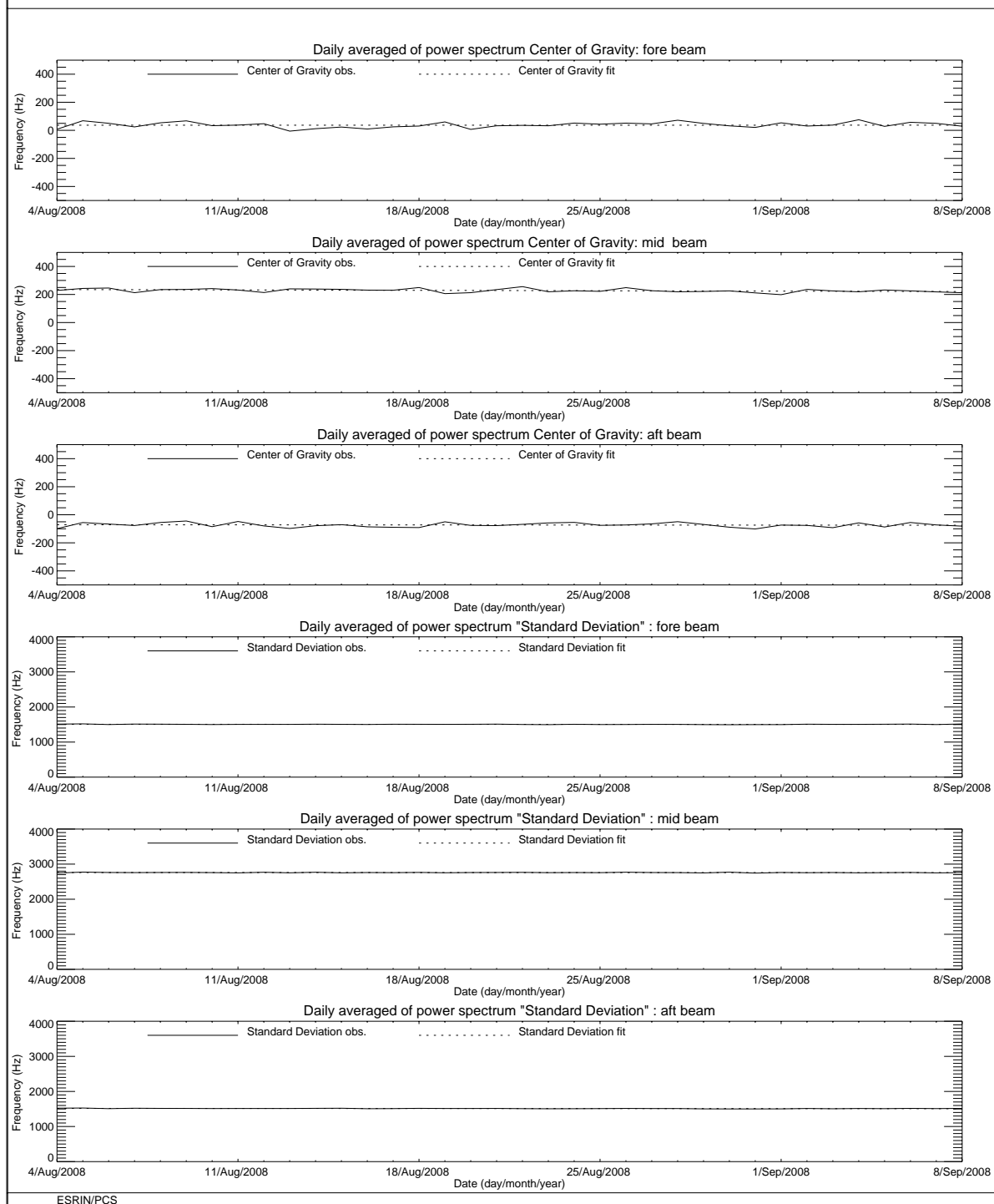
FIGURE 3 ERS-2 Scatterometer: Centre of Gravity and standard deviation of received power spectrum for cycle 139.
