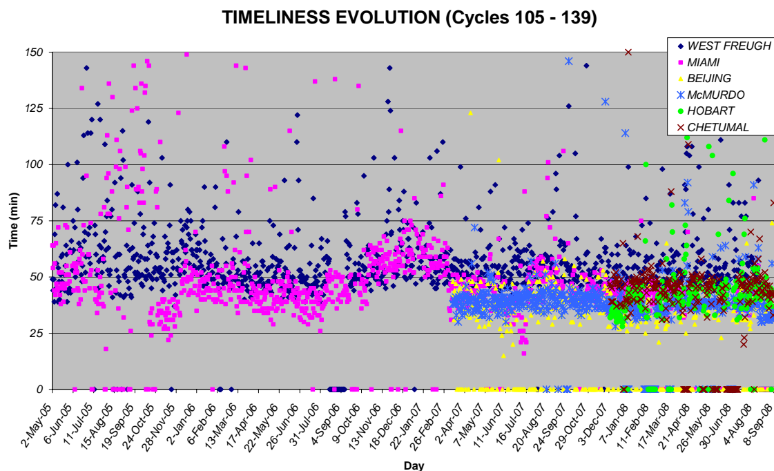
FIGURE 27 : Timeliness evolution from 19 April 2005 to 8 th September 2008 for West Freugh, Miami, Beijing, McMurdo, Hobart and Chetumal ground stations.
