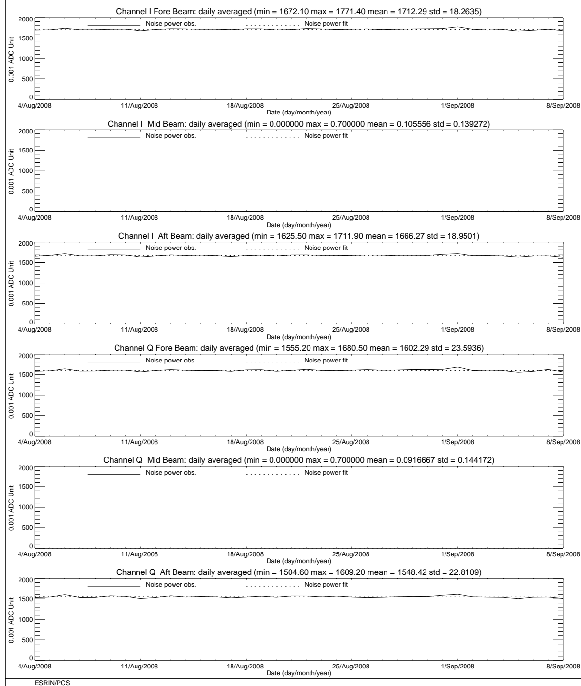
FIGURE 5 ERS-2 Scatterometer: noise power I and Q channel for cycle 139.
