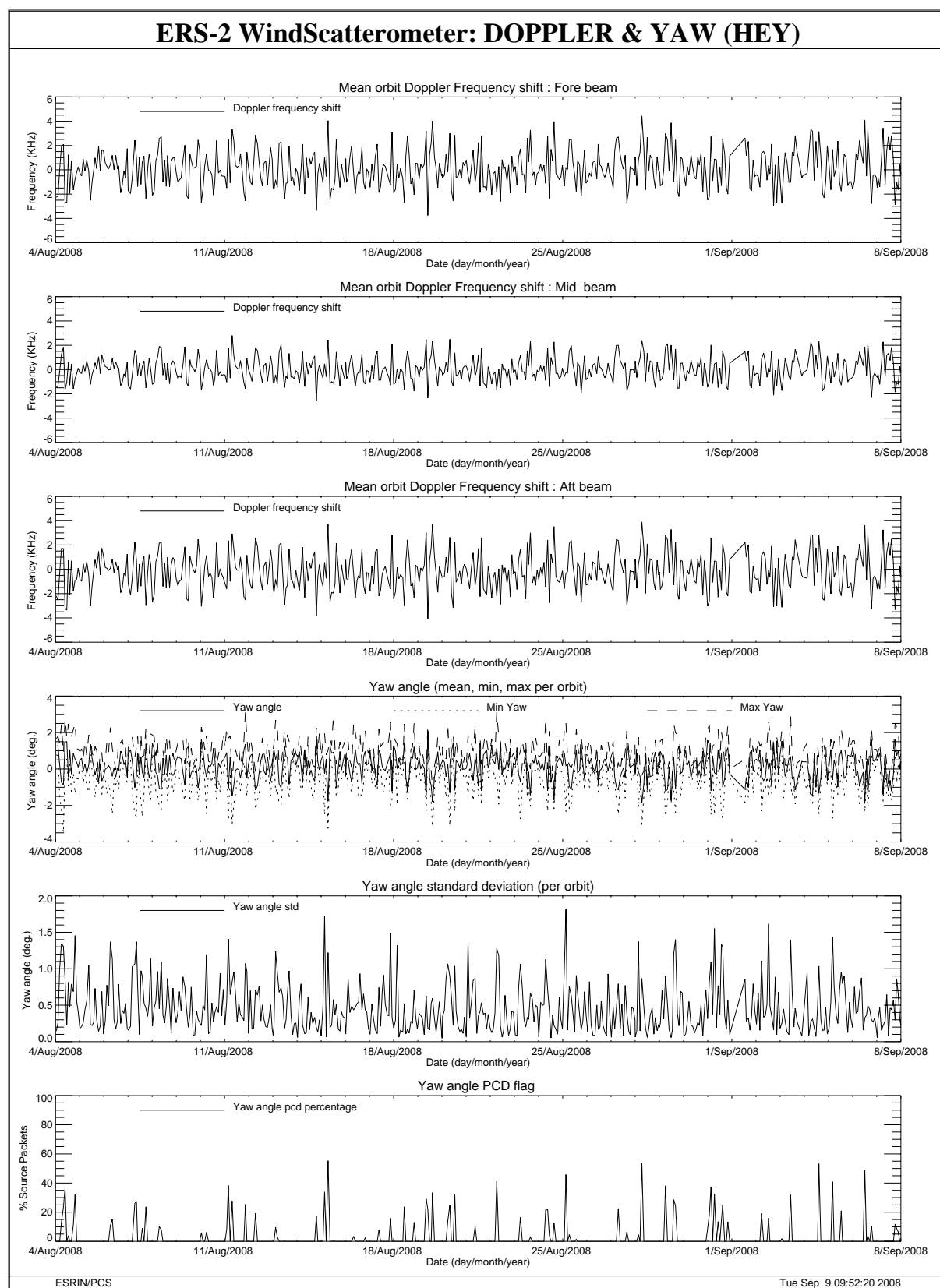
FIGURE 29 Doppler frequency shift and Yaw error angle evolution cycle 139.
