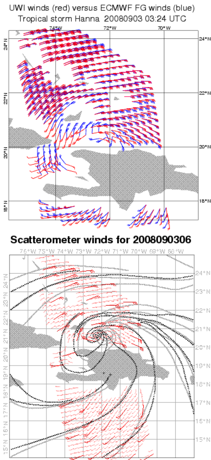
FIGURE 20 Comparison between UWI winds (in red) and ECMWF FG winds (in blue) for hurricane Hanna on 3 September 2008 (top panel). The lower panel shows the usage of this data in the ECMWF analysis system. Fat, large barbs indicate (CMOD5.4-based) winds that were actively used, while thin, small barbs were not used (mostly because of data thinning). Solid and gray contours are surface-wind streamlines for the ECMWF analysis respectively ECMWF first guess.
