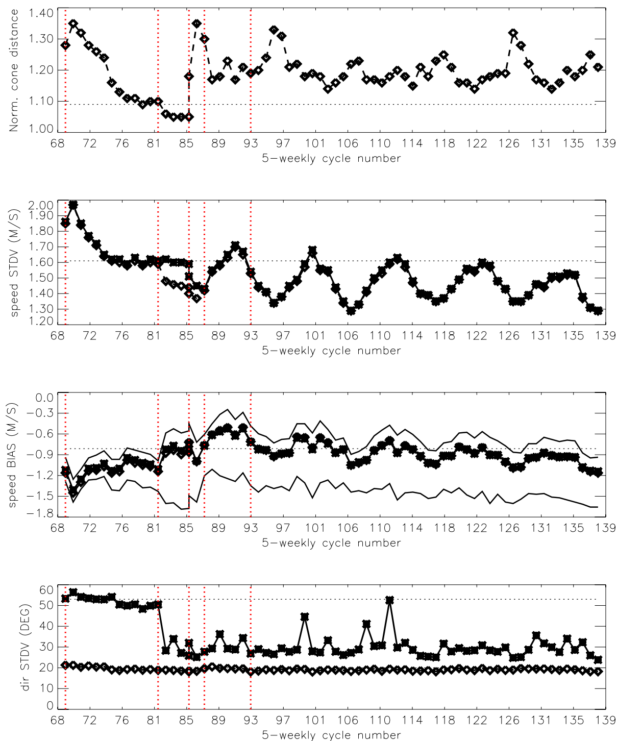
FIGURE 11 Evolution of the performance of the ERS-2 Scatterometer averaged over 5-weekly cycles from 12 December 2001 (cycle 69) to 4 August 2008 (end cycle 138) for the UWI product (solid, star) and de-aliased winds based on CMOD4 (dashed, diamond). Results are based on data that passed the UWI QC flags. For cycle 85 two values are plotted; the first value for the global set, the second one for the regional set. Dotted lines represent values for cycle 59 (5 December 2000 to 17 January 2001), i.e. the last stable cycle of the nominal period. From top to bottom panel are shown the normalized distance to the one (CMOD4 only) the standard deviation of the wind speed compared to FG winds, the corresponding bias (for UWI winds the extreme inter-node averages are shown as well), and the standard deviation of wind direction compared to FG.
