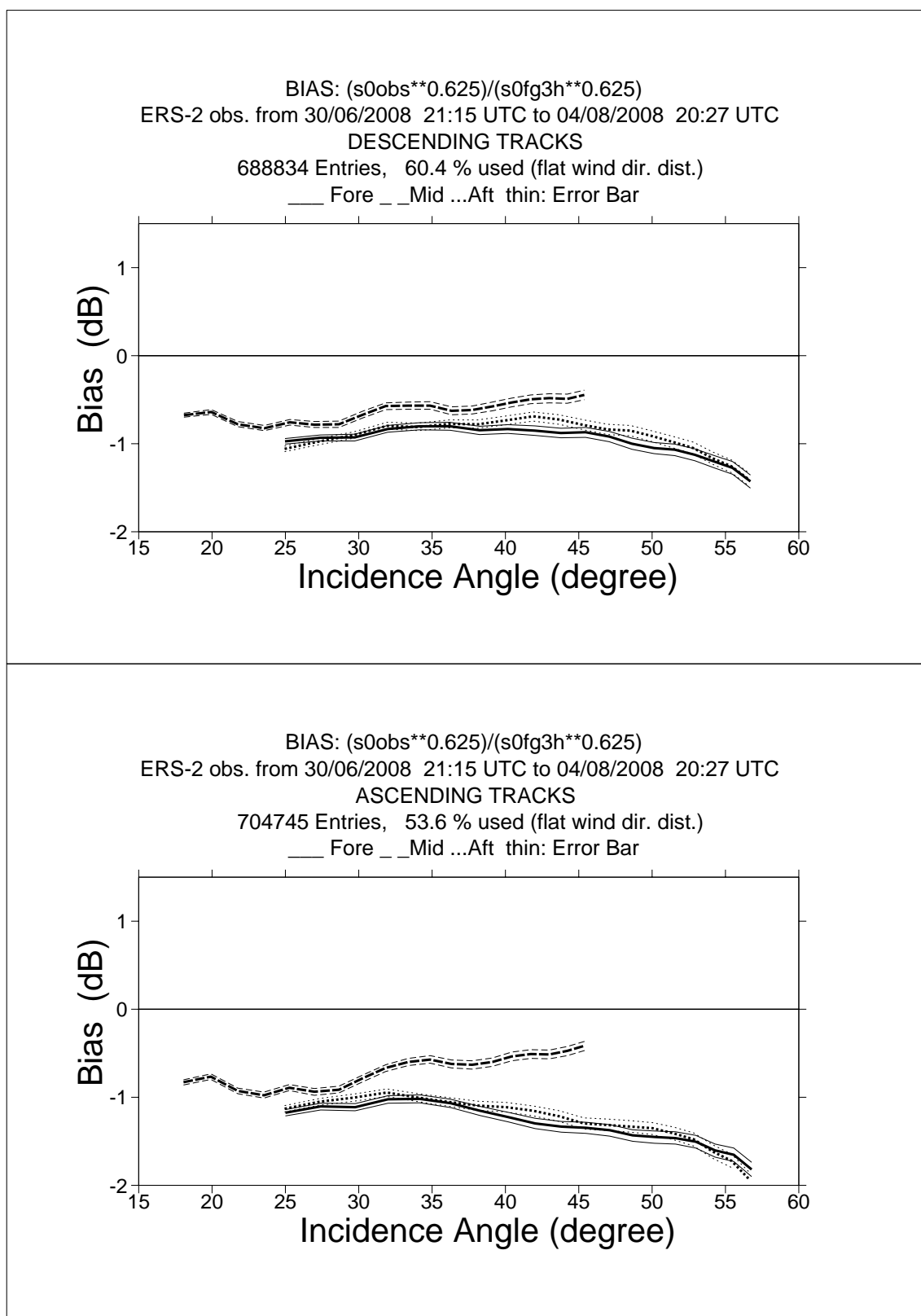
FIGURE 1 ERS-2 Scatterometer Ocean Calibration cycle 138. Ratio of \langle \sigma_0^{0.625} \rangle / \langle \text{CMOD4}(\text{First Guess})^{0.625} \rangle converted in dB for the fore beam (solid line), mid beam (dashed line) and aft beam (dotted line), as a function of incidence angle for descending and ascending tracks. The thin lines indicate the error bars on the estimated mean. First-guess winds are based on the in time closest (+3h, +6h, +9h, or +12h) T511 forecast field, and are bilinearly interpolated in space.
