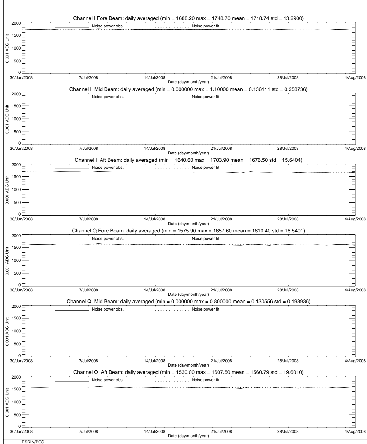
FIGURE 5 ERS-2 Scatterometer: noise power I and Q channel for cycle 138.
