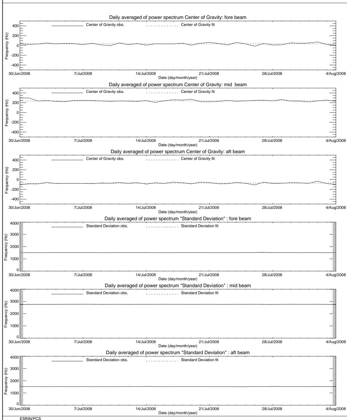
FIGURE 3 ERS-2 Scatterometer: Centre of Gravity and standard deviation of received power spectrum for cycle 138.
