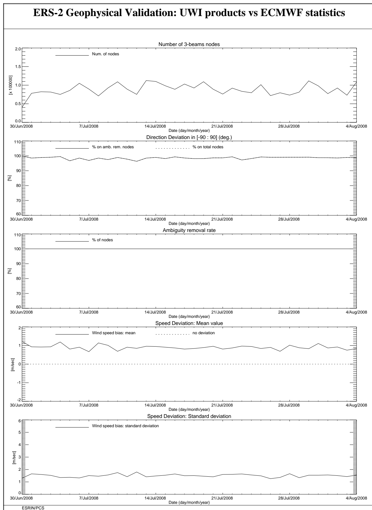
FIGURE 10 ERS-2 Scatterometer: wind products performance for cycle 138.
