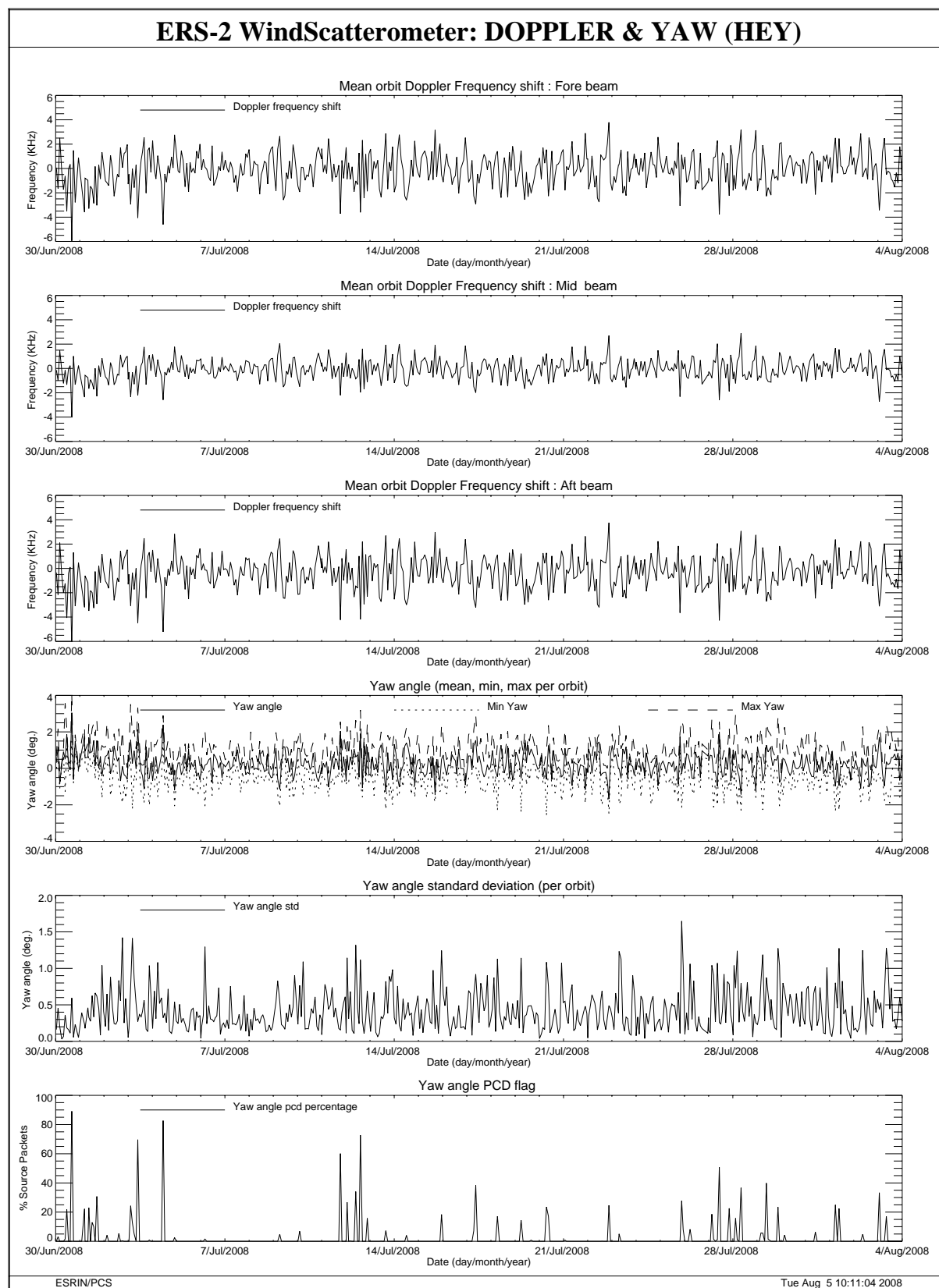
FIGURE 29 Doppler frequency shift and Yaw error angle evolution cycle 138.
