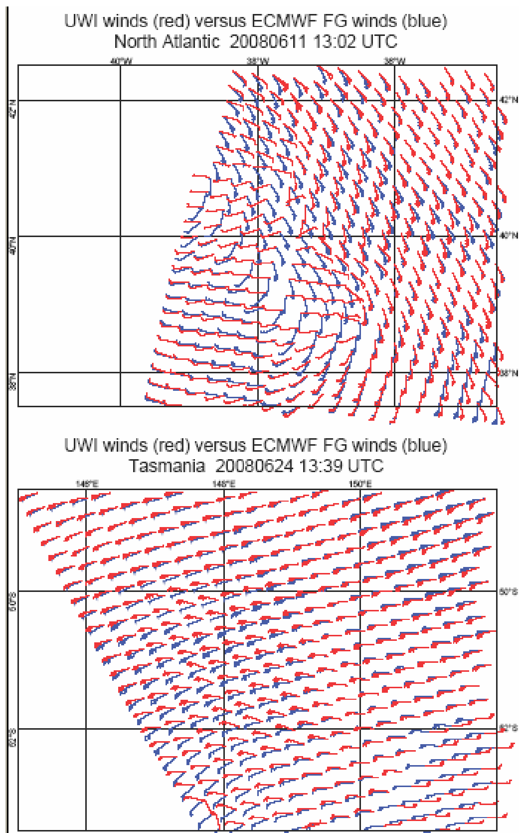
FIGURE 20 Comparison between UWI winds (in red) and ECMWF FG winds (in blue) for a case in the North Atlantic on 11 June 2008 (top panel) and for a case south of Tasmania on 24 June 2008 (lower panel).
