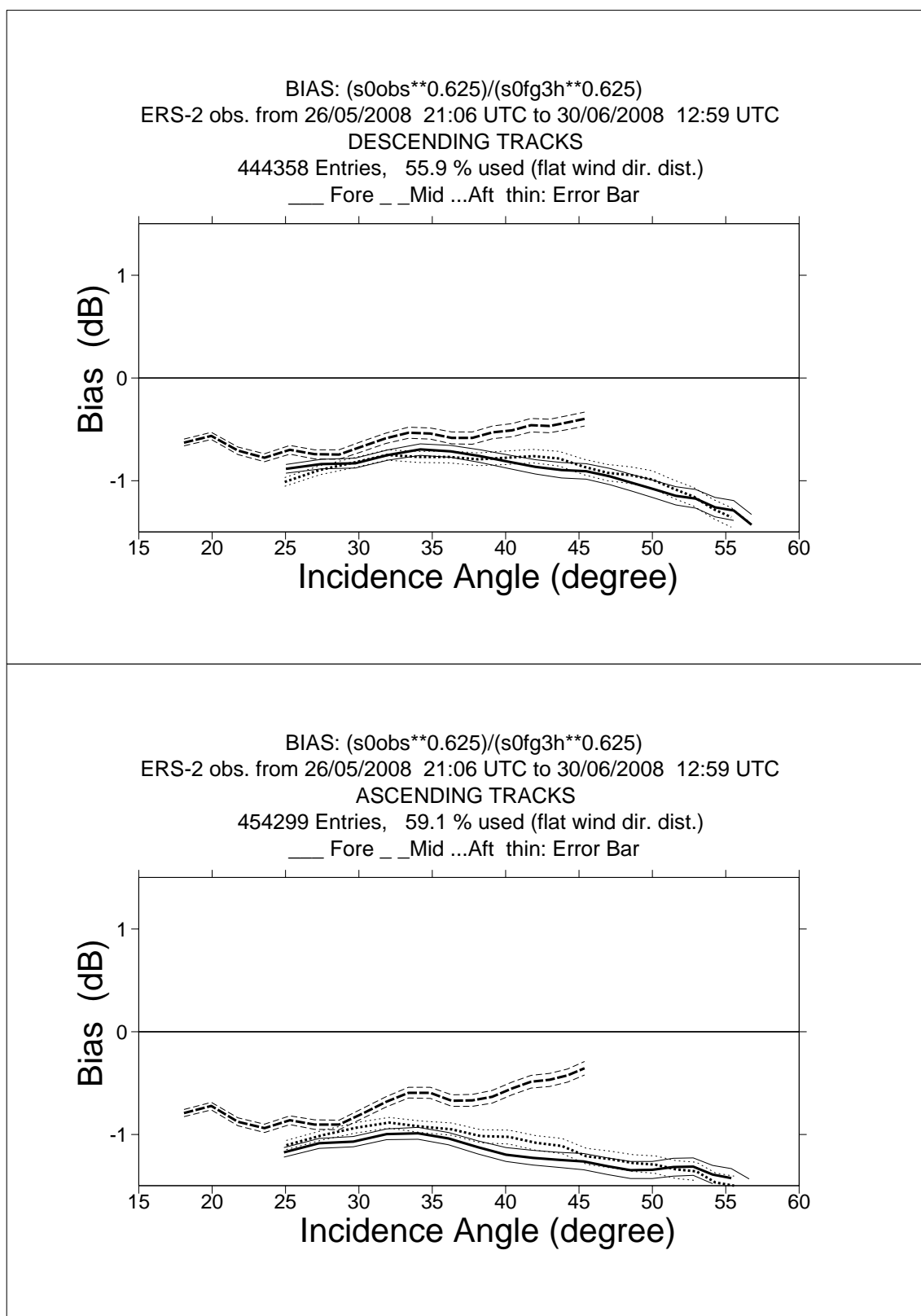
FIGURE 1 ERS-2 Scatterometer Ocean Calibration cycle 137. Ratio of \langle \sigma_0^{0.625} \rangle / \langle \text{CMOD4}(\text{First Guess})^{0.625} \rangle converted in dB for the fore beam (solid line), mid beam (dashed line) and aft beam (dotted line), as a function of incidence angle for descending and ascending tracks. The thin lines indicate the error bars on the estimated mean. First-guess winds are based on the in time closest (+3h, +6h, +9h, or +12h) T511 forecast field, and are bilinearly interpolated in space.
