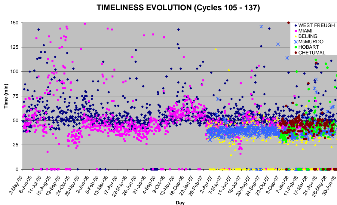
FIGURE 27 : Timeliness evolution from 19 April 2005 to 30 th June 2008 for West Freugh, Miami, Beijing, McMurdo, Hobart and Chetumal ground stations.
