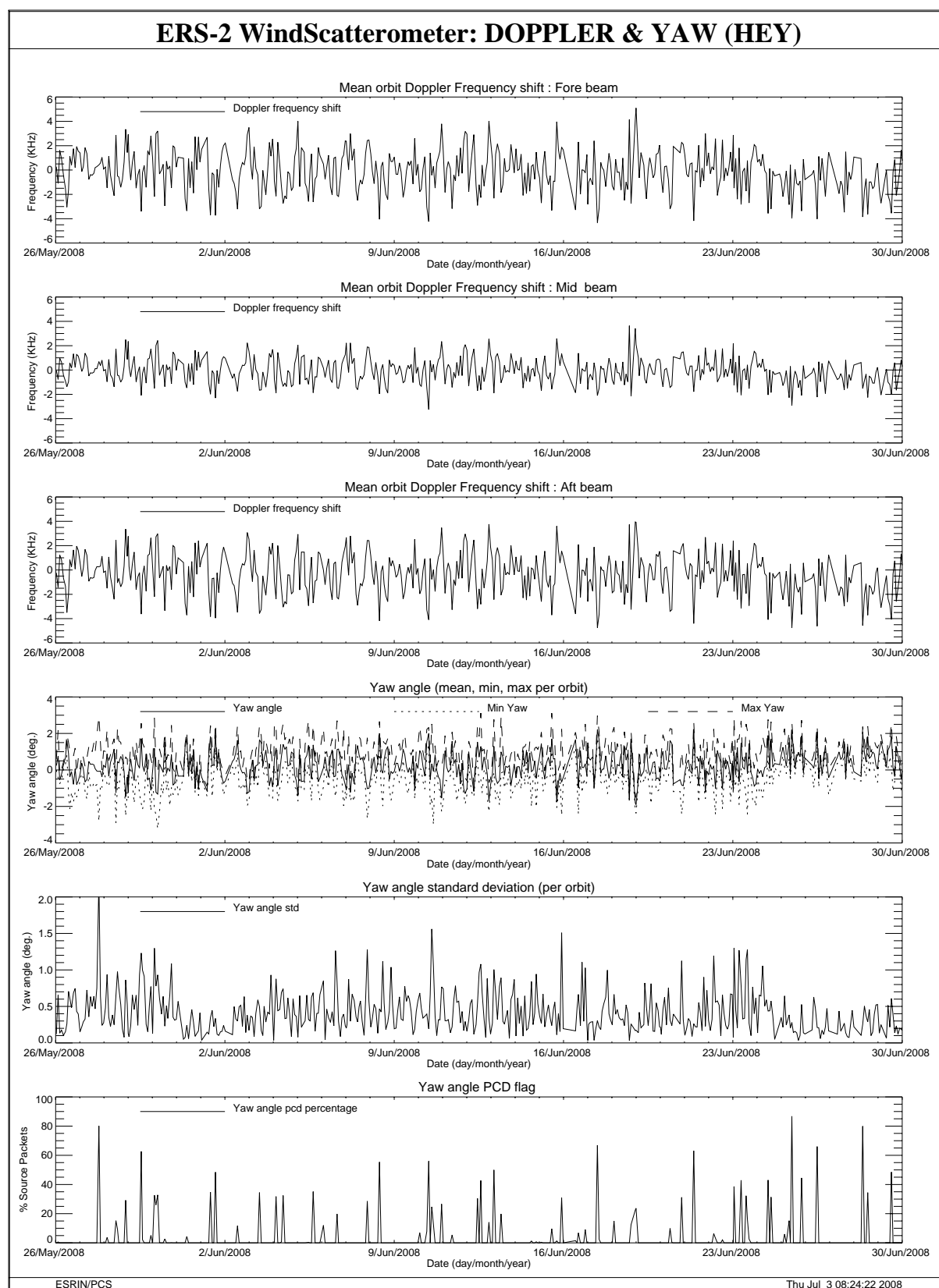
FIGURE 29 Doppler frequency shift and Yaw error angle evolution cycle 137.
