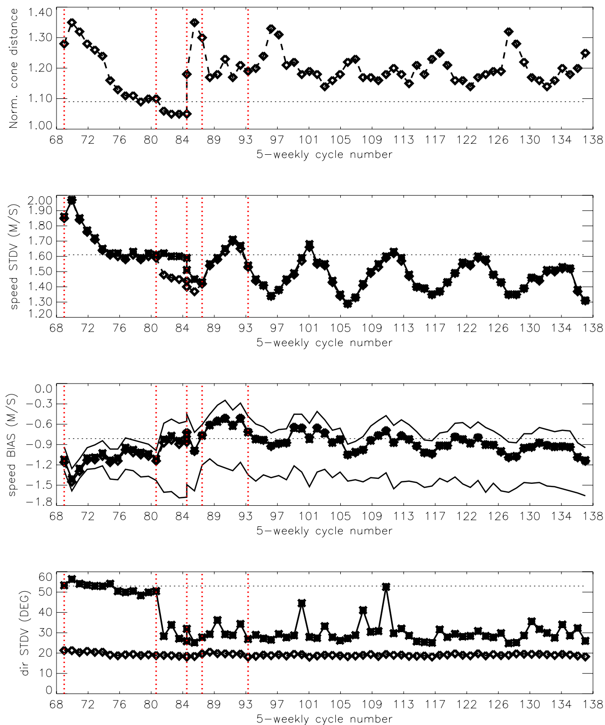
FIGURE 11 Evolution of the performance of the ERS-2 Scatterometer averaged over 5-weekly cycles from 12 December 2001 (cycle 69) to 30 June 2008 (end cycle 137) for the UWI product (solid, star) and de-aliased winds based on CMOD4 (dashed, diamond). Results are based on data that passed the UWI QC flags. For cycle 85 two values are plotted; the first value for the global set, the second one for the regional set. Dotted lines represent values for cycle 59 (5 December 2000 to 17 January 2001), i.e. the last stable cycle of the nominal period. From top to bottom panel are shown the normalized distance to the one (CMOD4 only) the standard deviation of the wind speed compared to FG winds, the corresponding bias (for UWI winds the extreme inter-node averages are shown as well), and the standard deviation of wind direction compared to FG.
