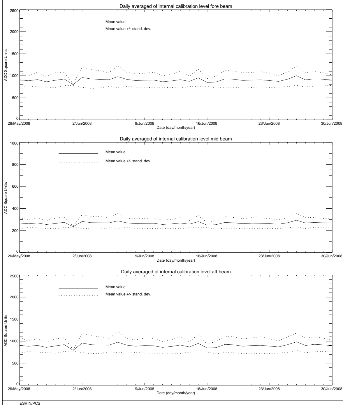
FIGURE 7 ERS-2 Scatterometer: power of internal calibration level cycle 137.
