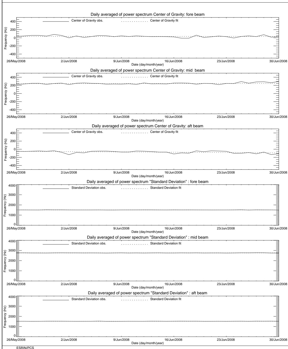
FIGURE 3 ERS-2 Scatterometer: Centre of Gravity and standard deviation of received power spectrum for cycle 137.
