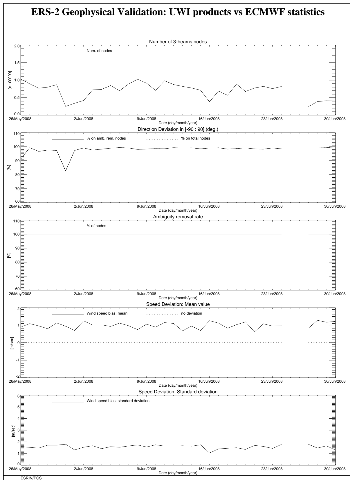
FIGURE 10 ERS-2 Scatterometer: wind products performance for cycle 137.
