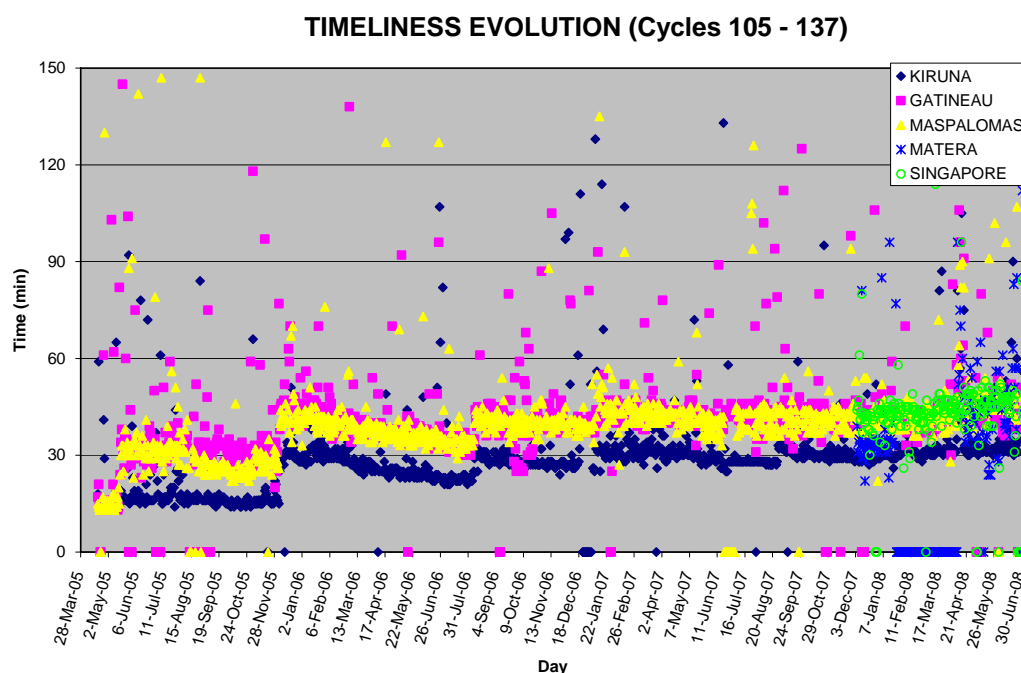
FIGURE 26 : Timeliness evolution from 19 th April 2005 to 30 th June 2008 for Gatineau, Kiruna, Maspalomas, Matera and Singapore ground stations.
