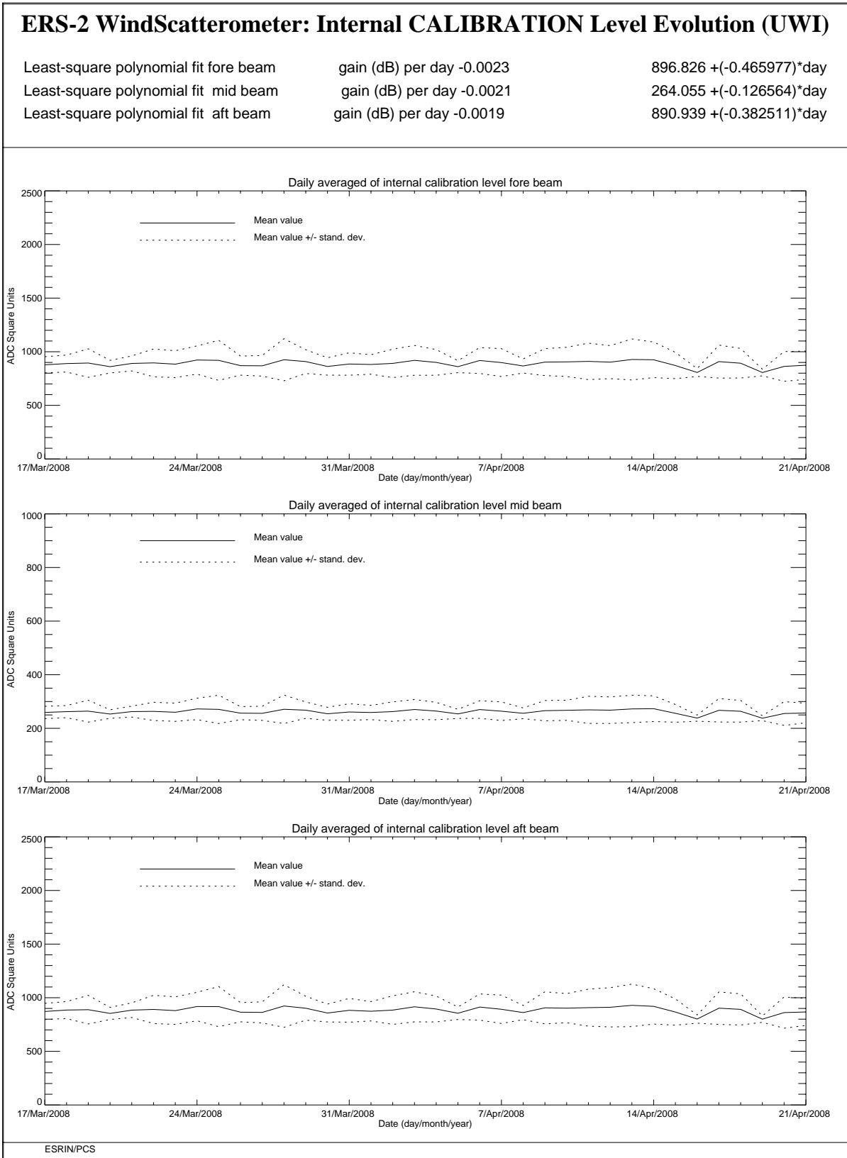
FIGURE 7 ERS-2 Scatterometer: power of internal calibration level cycle 135.
