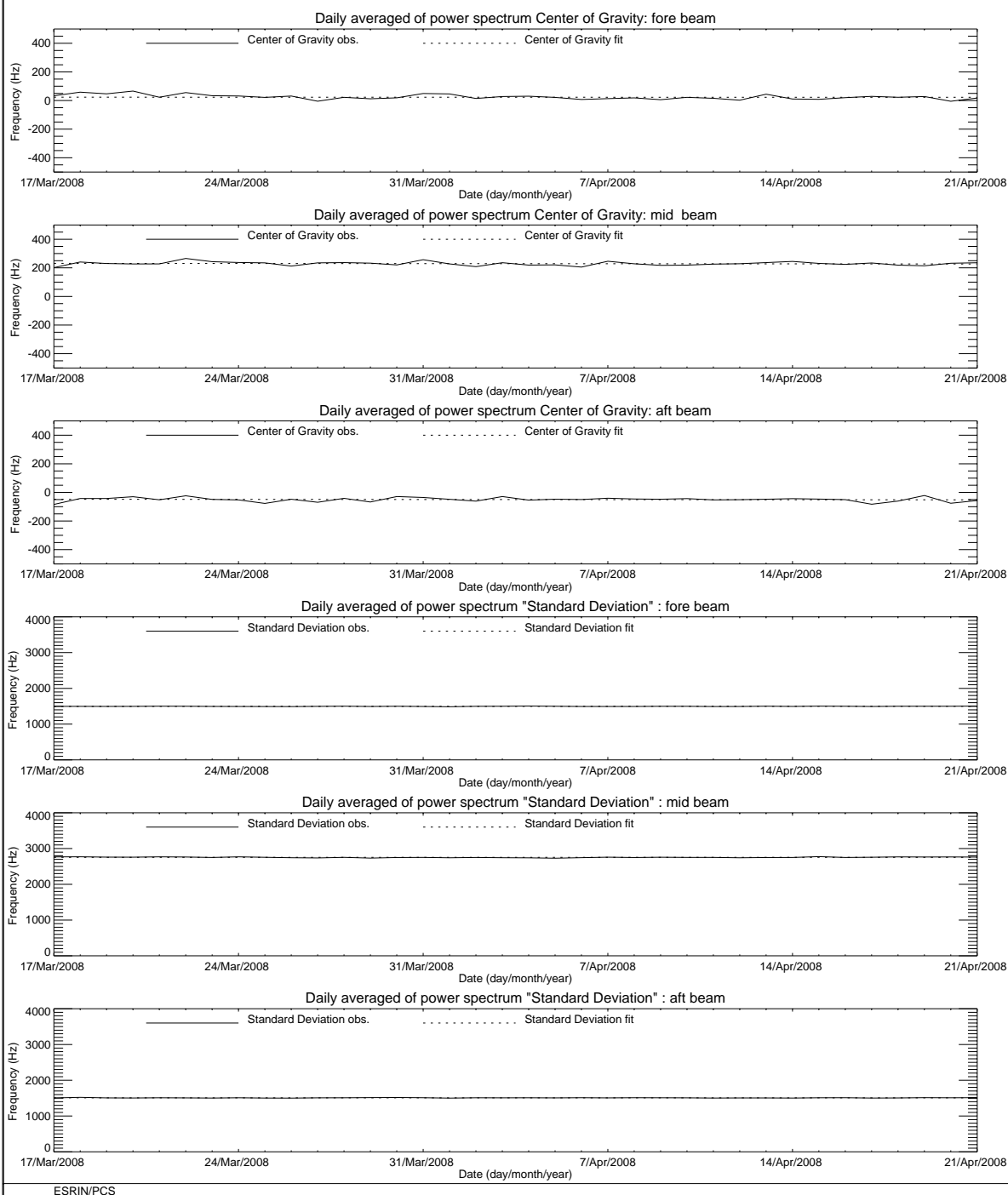
FIGURE 3 ERS-2 Scatterometer: Centre of Gravity and standard deviation of received power spectrum for cycle 135.
