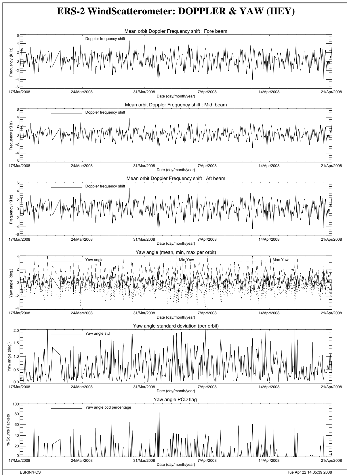
FIGURE 29 Doppler frequency shift and Yaw error angle evolution cycle 135.
