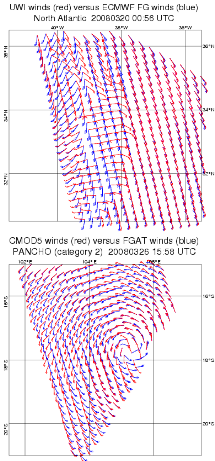
FIGURE 20 Comparison between UWI winds (in red) and ECMWF FG winds (in blue) for a case on 20 March 2008 in the North Atlantic (top panel) and de-aliased CMOD5 winds (in red) versus ECMWF FG winds (in blue) for tropical cyclone Pancho on 26 March 2008 in the South Indian Ocean (lower panel).
