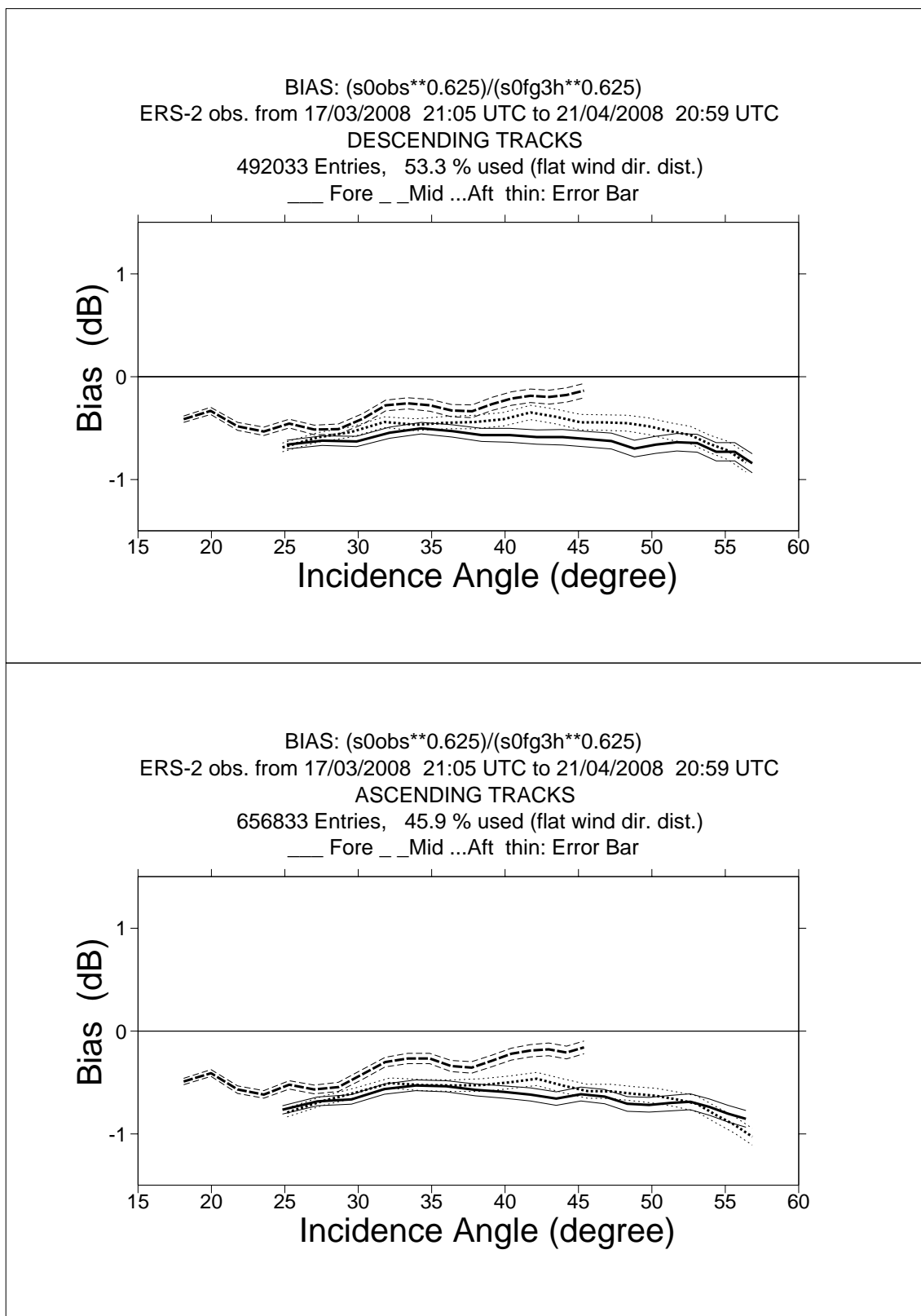
FIGURE 1 ERS-2 Scatterometer Ocean Calibration cycle 135. Ratio of \langle \sigma_0^{0.625} \rangle / \langle CMOD4(\text{First Guess})^{0.625} \rangle converted in dB for the fore beam (solid line), mid beam (dashed line) an aft beam (dotted line), as a function of incidence angle for descending and ascending tracks. The thin lines indicate the error bars on the estimated mean. First-guess winds are based on the in time closest (+3h, +6h, +9h, or +12h) T511 forecast field, and are bilinearly interpolated in space.
