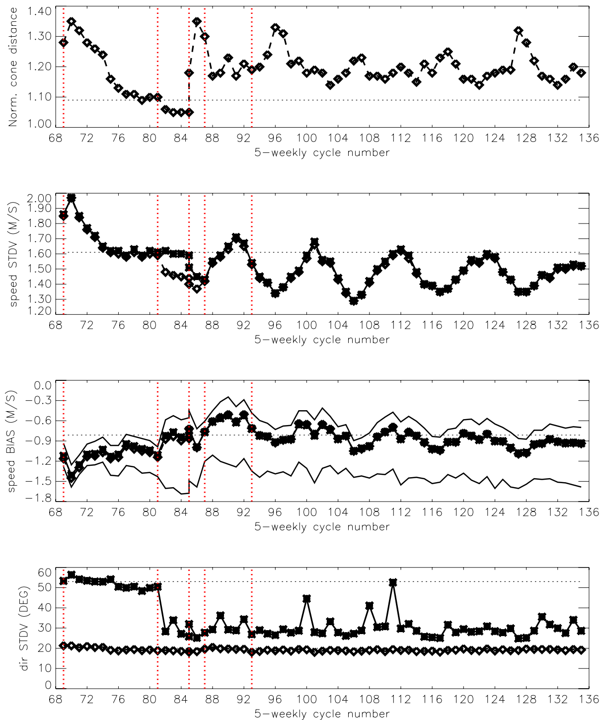
FIGURE 11 Evolution of the performance of the ERS-2 Scatterometer averaged over 5-weekly cycles from 12 December 2001 (cycle 69) to 21 April 2008 (end cycle 135) for the UWI product (solid, star) and de-aliased winds based on CMOD4 (dashed, diamond). Results are based on data that passed the UWI QC flags. For cycle 85 two values are plotted; the first value for the global set, the second one for the regional set. Dotted lines represent values for cycle 59 (5 December 2000 to 17 January 2001), i.e. the last stable cycle of the nominal period. From top to bottom panel are shown the normalized distance to the one (CMOD4 only) the standard deviation of the wind speed compared to FG winds, the corresponding bias (for UWI winds the extreme inter-node averages are shown as well), and the standard deviation of wind direction compared to FG.
