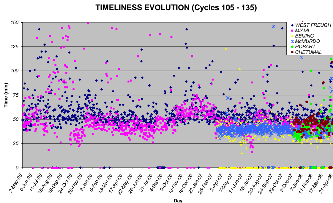
FIGURE 27 : Timeliness evolution from 19 April 2005 to 21 st April 2008 for West Freugh, Miami, Beijing, McMurdo, Hobart and Chetumal ground stations.
