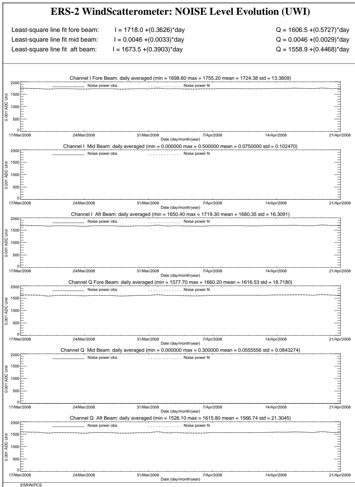
FIGURE 5 ERS-2 Scatterometer: noise power I and Q channel for cycle 135.
