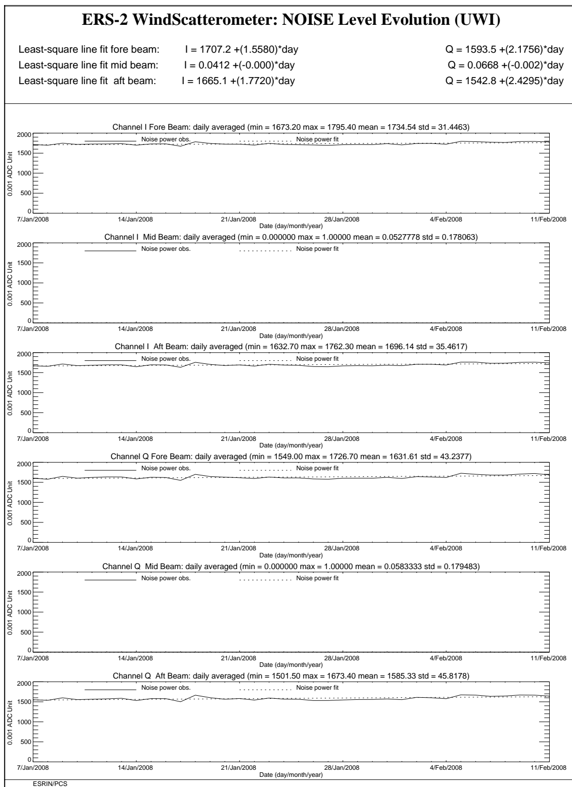
FIGURE 5 ERS-2 Scatterometer: noise power I and Q channel for cycle 133.
