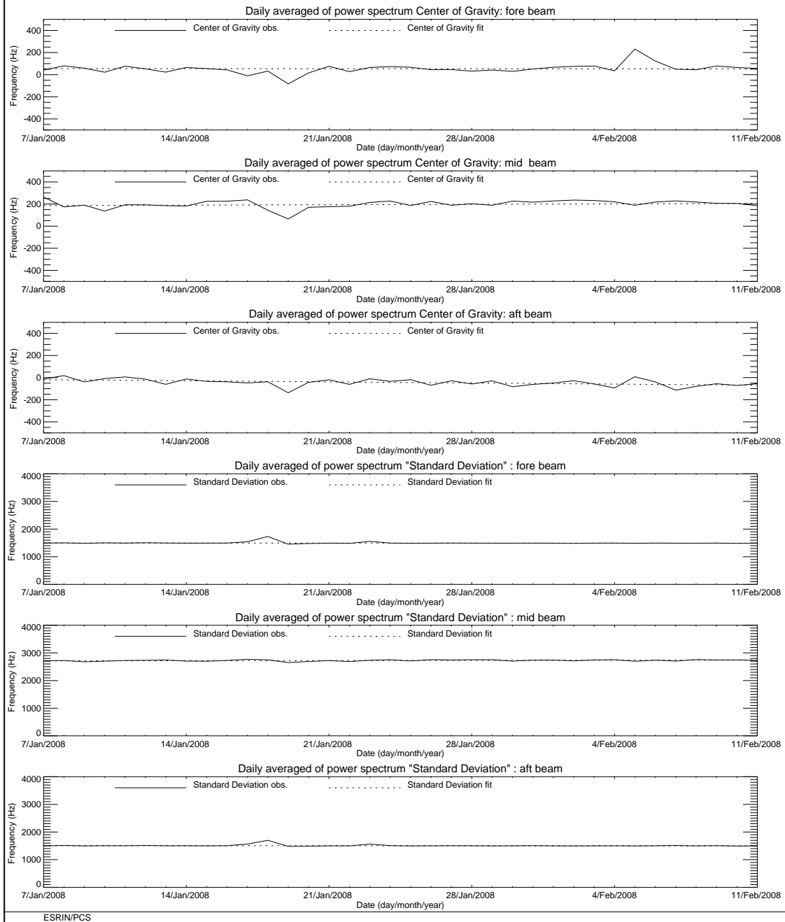
FIGURE 3 ERS-2 Scatterometer: Centre of Gravity and standard deviation of received power spectrum for cycle 133.
