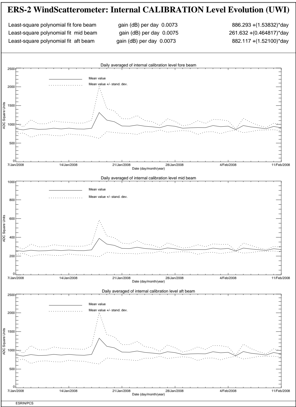
FIGURE 7 ERS-2 Scatterometer: power of internal calibration level cycle 133.
