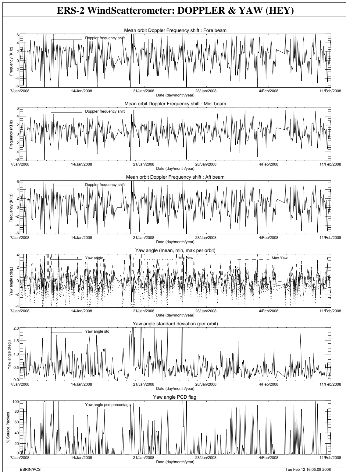
FIGURE 29 Doppler frequency shift and Yaw error angle evolution cycle 133.
