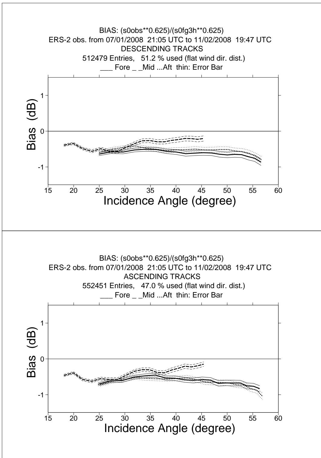
FIGURE 1 ERS-2 Scatterometer Ocean Calibration cycle 133. Ratio of \langle \sigma_0^{0.625} \rangle / \langle CMOD4(\text{First Guess})^{0.625} \rangle converted in dB for the fore beam (solid line), mid beam (dashed line) an aft beam (dotted line), as a function of incidence angle for descending and ascending tracks. The thin lines indicate the error bars on the estimated mean. First-guess winds are based on the in time closest (+3h, +6h, +9h, or +12h) T511 forecast field, and are bilinearly interpolated in space.
