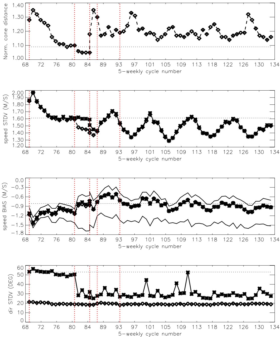
FIGURE 11 Evolution of the performance of the ERS-2 Scatterometer averaged over 5-weekly cycles from 12 December 2001 (cycle 69) to 11 February 2008 (end cycle 133) for the UWI product (solid, star) and de-aliased winds based on CMOD4 (dashed, diamond). Results are based on data that passed the UWI QC flags. For cycle 85 two values are plotted; the first value for the global set, the second one for the regional set. Dotted lines represent values for cycle 59 (5 December 2000 to 17 January 2001), i.e. the last stable cycle of the nominal period. From top to bottom panel are shown the normalized distance to the one (CMOD4 only) the standard deviation of the wind speed compared to FG winds, the corresponding bias (for UWI winds the extreme inter-node averages are shown as well), and the standard deviation of wind direction compared to FG.
