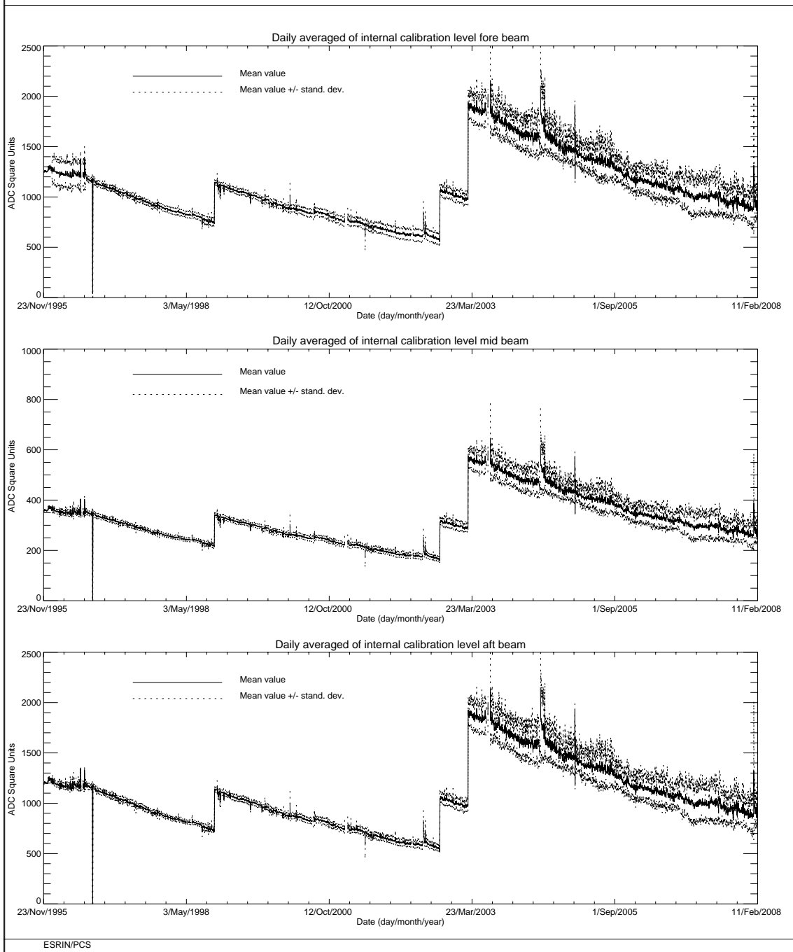
FIGURE 6 ERS-2 Scatterometer: power of internal calibration pulse since the beginning of the mission.
