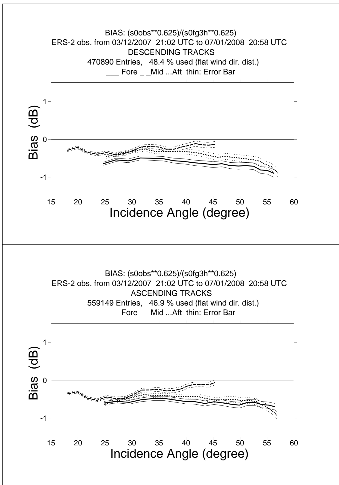
FIGURE 1 ERS-2 Scatterometer Ocean Calibration cycle 132. Ratio of \langle \sigma_0^{0.625} \rangle / \langle \text{CMOD4}(\text{First Guess})^{0.625} \rangle converted in dB for the fore beam (solid line), mid beam (dashed line) and aft beam (dotted line), as a function of incidence angle for descending and ascending tracks. The thin lines indicate the error bars on the estimated mean. First-guess winds are based on the in time closest (+3h, +6h, +9h, or +12h) T511 forecast field, and are bilinearly interpolated in space.
