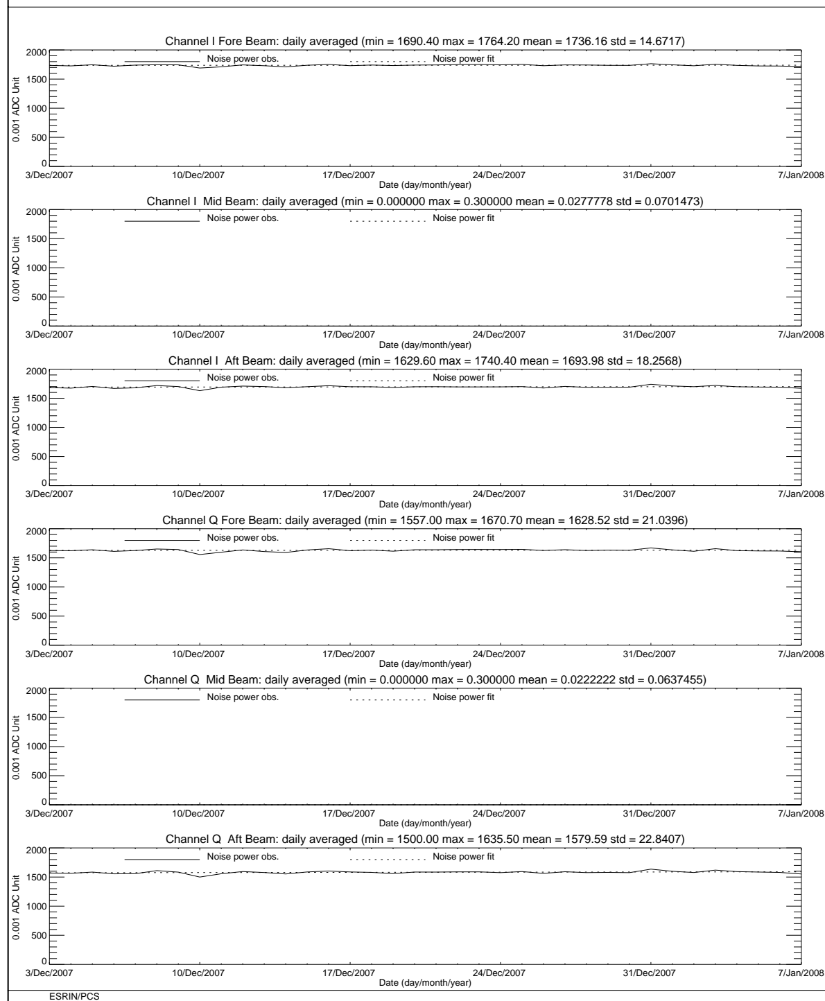
FIGURE 5 ERS-2 Scatterometer: noise power I and Q channel for cycle 132.
