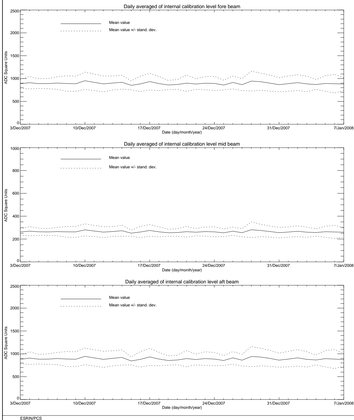
FIGURE 7 ERS-2 Scatterometer: power of internal calibration level cycle 132.
