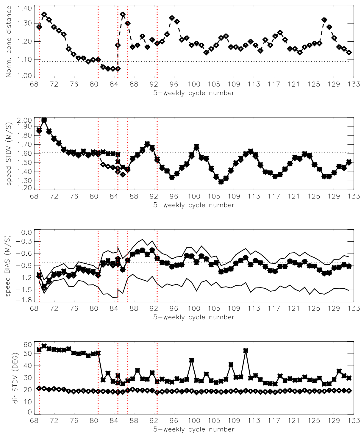
FIGURE 11 Evolution of the performance of the ERS-2 Scatterometer averaged over 5-weekly cycles from 12 December 2001 (cycle 69) to 7 January 2008 (end cycle 132) for the UWI product (solid, star) and de-aliased winds based on CMOD4 (dashed, diamond). Results are based on data that passed the UWI QC flags. For cycle 85 two values are plotted; the first value for the global set, the second one for the regional set. Dotted lines represent values for cycle 59 (5 December 2000 to 17 January 2001), i.e. the last stable cycle of the nominal period. From top to bottom panel are shown the normalized distance to the one (CMOD4 only) the standard deviation of the wind speed compared to FG winds, the corresponding bias (for UWI winds the extreme inter-node averages are shown as well), and the standard deviation of wind direction compared to FG.
