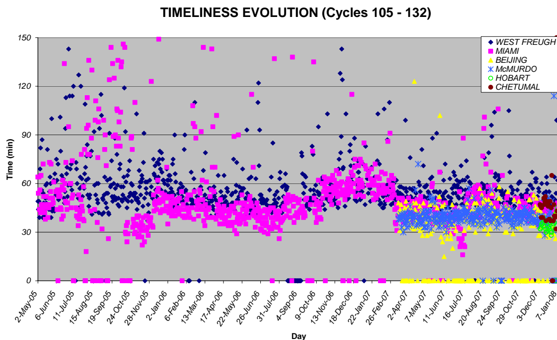
FIGURE 27 : Timeliness evolution from 19 April 2005 to 7 January 2008 for West Freugh, Miami, Beijing, McMurdo, Hobart and Chetumal ground stations.
