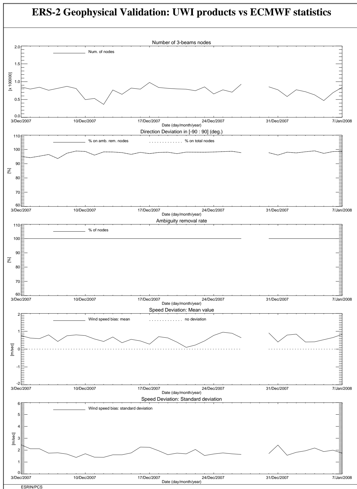
FIGURE 10 ERS-2 Scatterometer: wind products performance for cycle 132.
