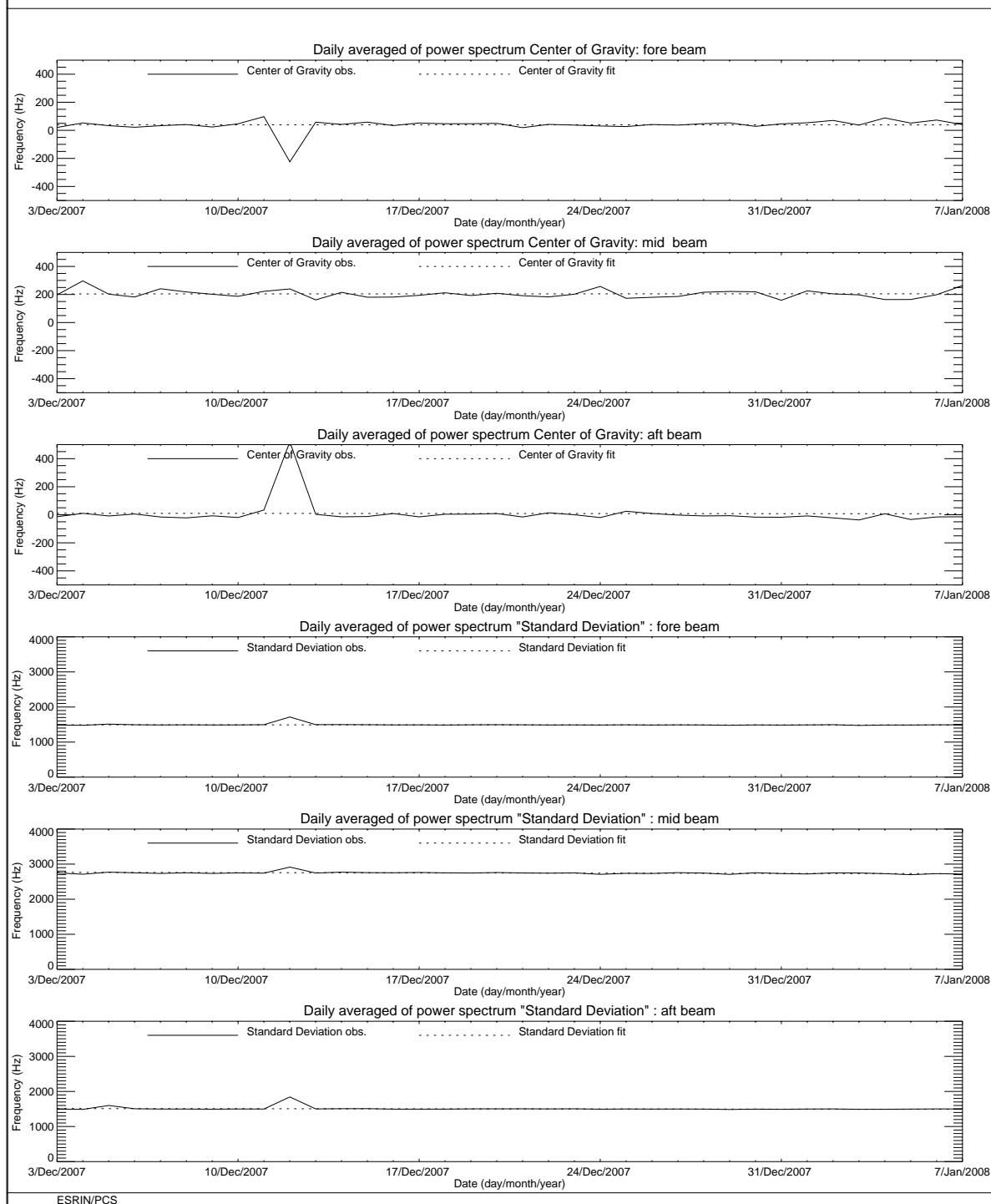
FIGURE 3 ERS-2 Scatterometer: Centre of Gravity and standard deviation of received power spectrum for cycle 132.
