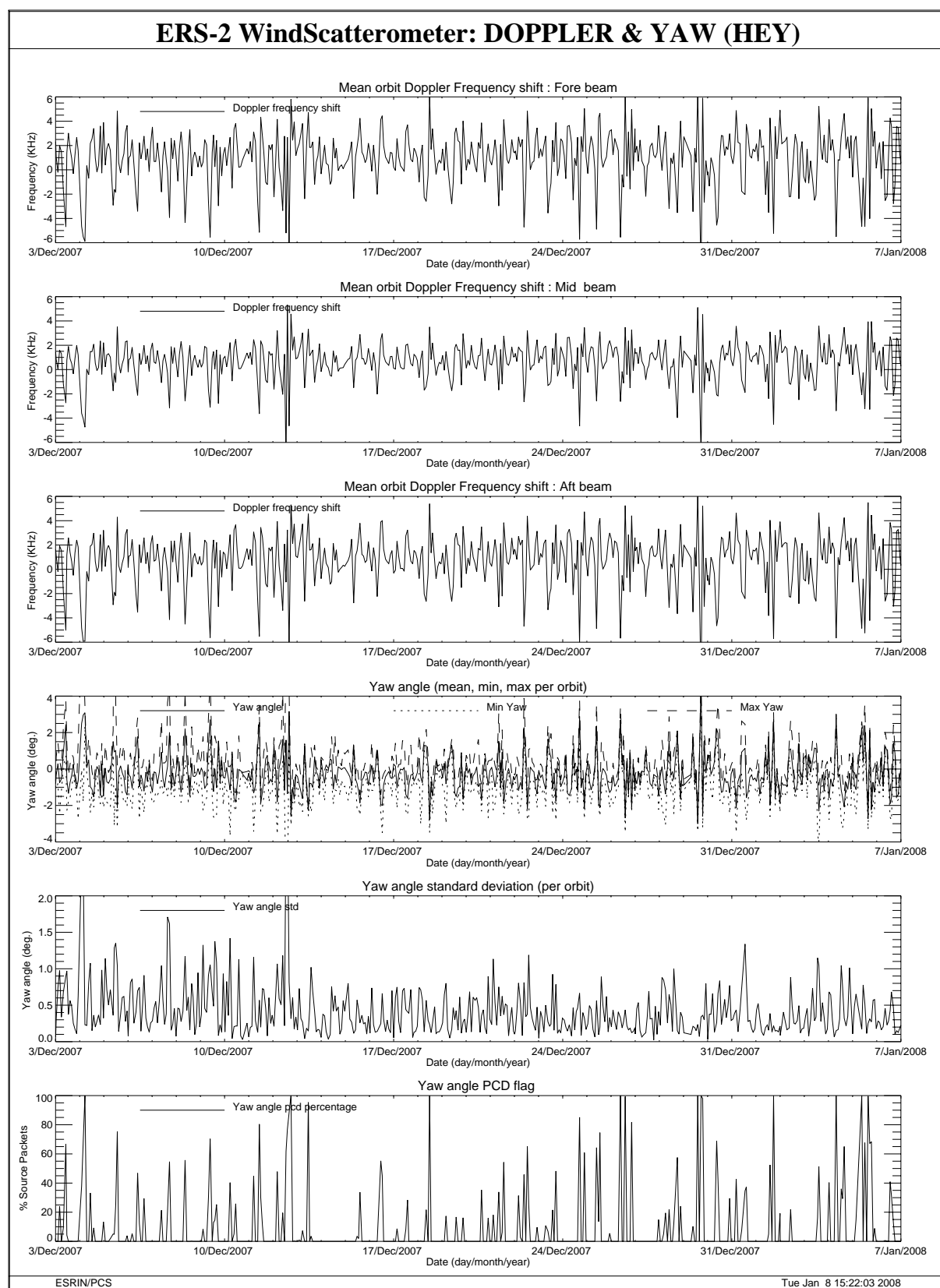
FIGURE 29 Doppler frequency shift and Yaw error angle evolution cycle 132.
