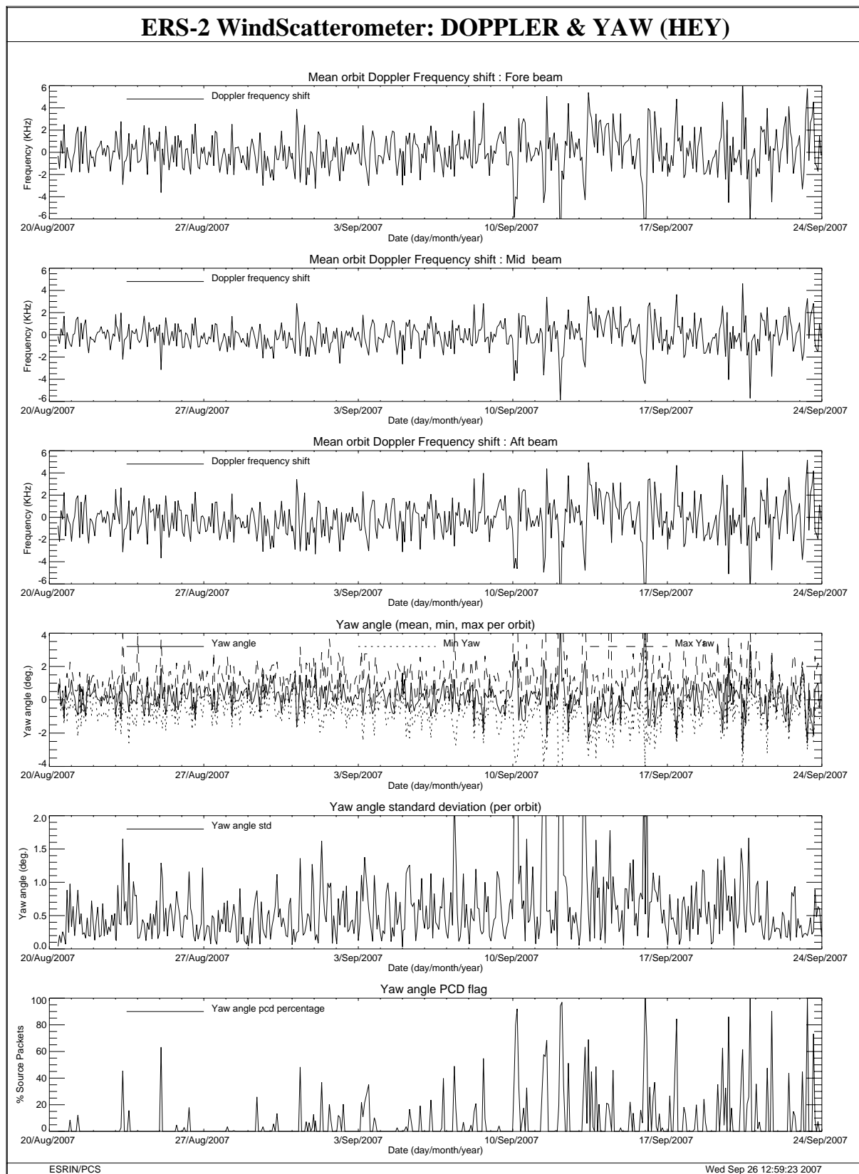
FIGURE 29 Doppler frequency shift and Yaw error angle evolution cycle 129.
