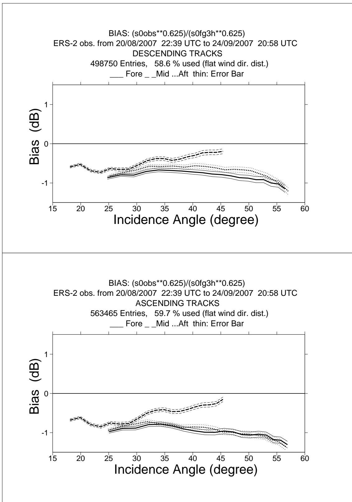
FIGURE 1 ERS-2 Scatterometer Ocean Calibration cycle 129. Ratio of \langle \sigma_0^{0.625} \rangle / \langle CMOD4(First\ Guess)^{0.625} \rangle converted in dB for the fore beam (solid line), mid beam (dashed line) an aft beam (dotted line), as a function of incidence angle for descending and ascending tracks. The thin lines indicate the error bars on the estimated mean. First-guess winds are based on the in time closest (+3h, +6h, +9h, or +12h) T511 forecast field, and are bilinearly interpolated in space.
