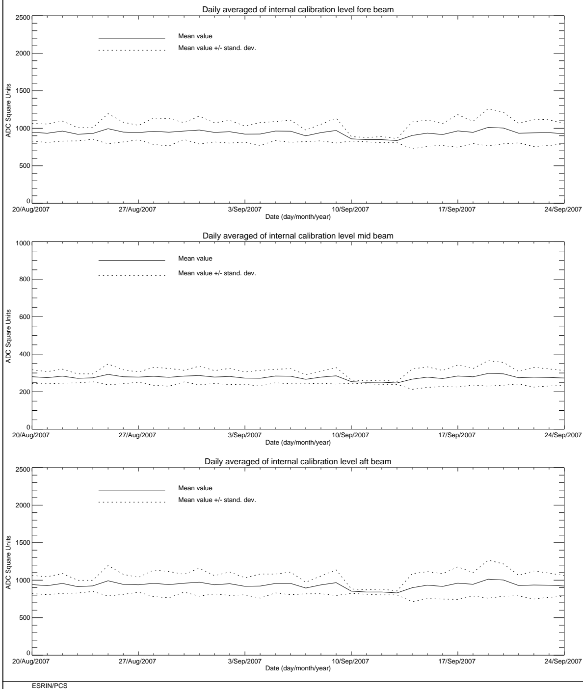
FIGURE 7 ERS-2 Scatterometer: power of internal calibration level cycle 129.
