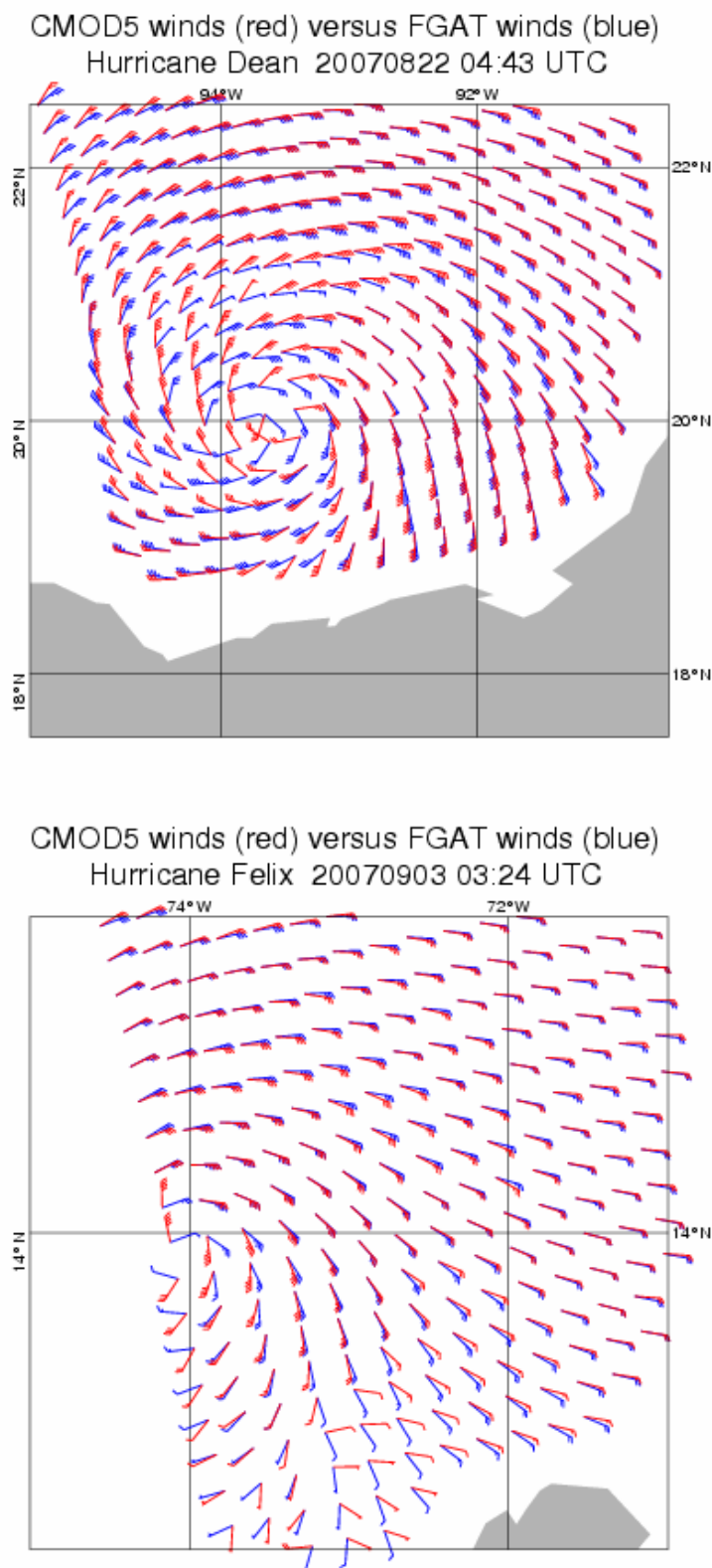
FIGURE 20 Comparison between de-aliased CMOD5 winds (in red) and ECMWF FG winds (in blue) for Hurricane Dean on 22 August 2007 (top panel) and Hurricane Felix on 3 September 2007 (lower panel).
