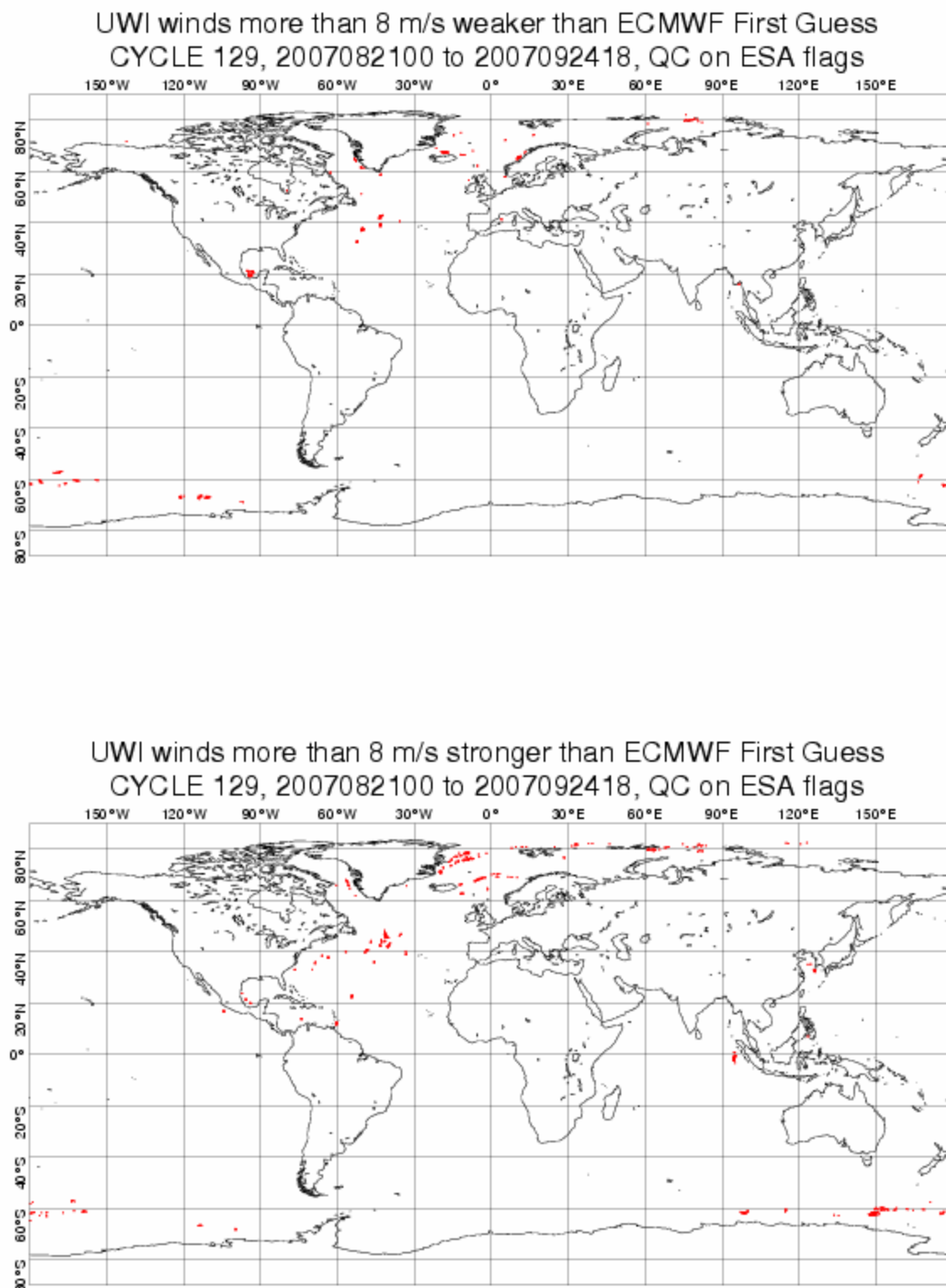
FIGURE 19 Locations of data during cycle 129 for which UWI winds are more than 8 m/s weaker (top panel) respectively stronger (lower panel) than FGAT, and on which QC on UWI flags and the ECMWF land/sea-ice mask was applied.
