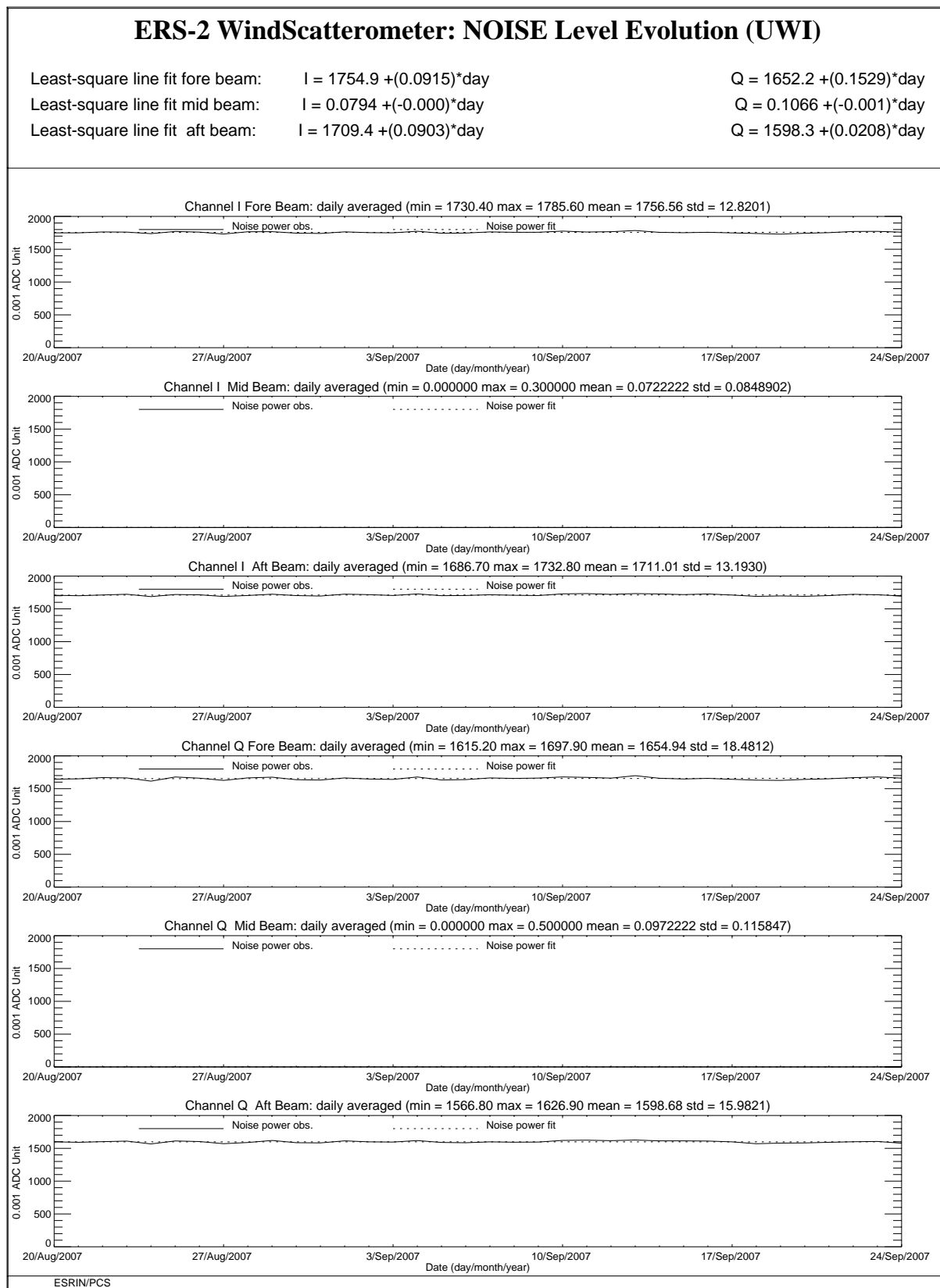
FIGURE 5 ERS-2 Scatterometer: noise power I and Q channel for cycle 129.
