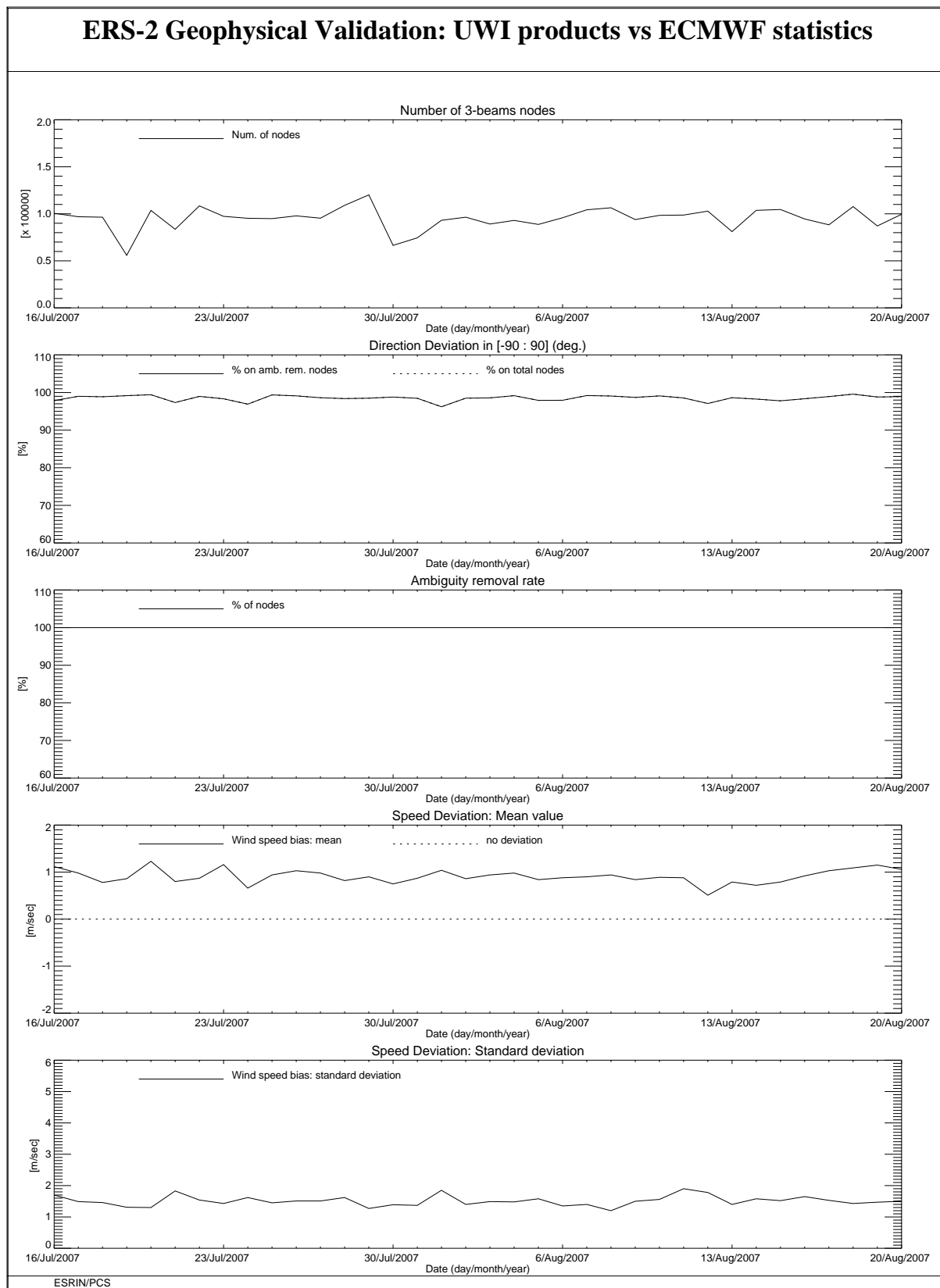
FIGURE 10 ERS-2 Scatterometer: wind products performance for cycle 128.
