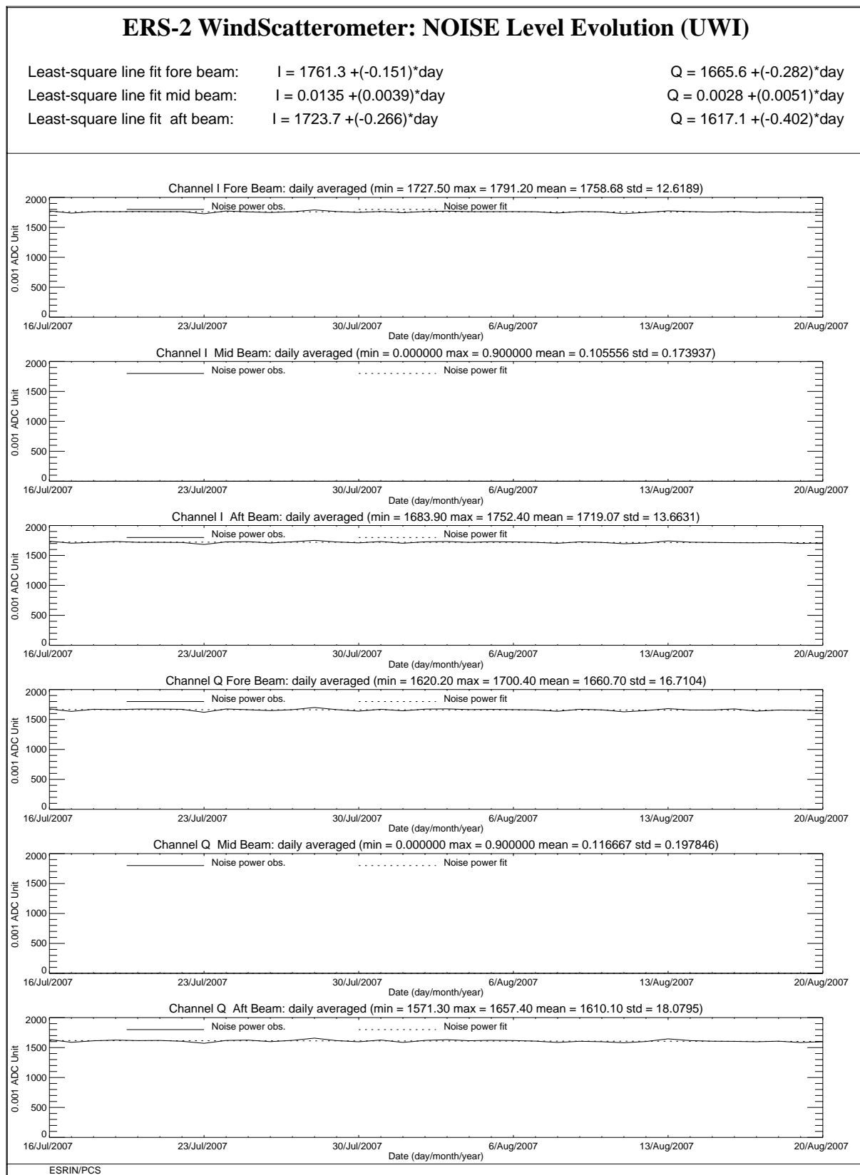
FIGURE 5 ERS-2 Scatterometer: noise power I and Q channel for cycle 128.
