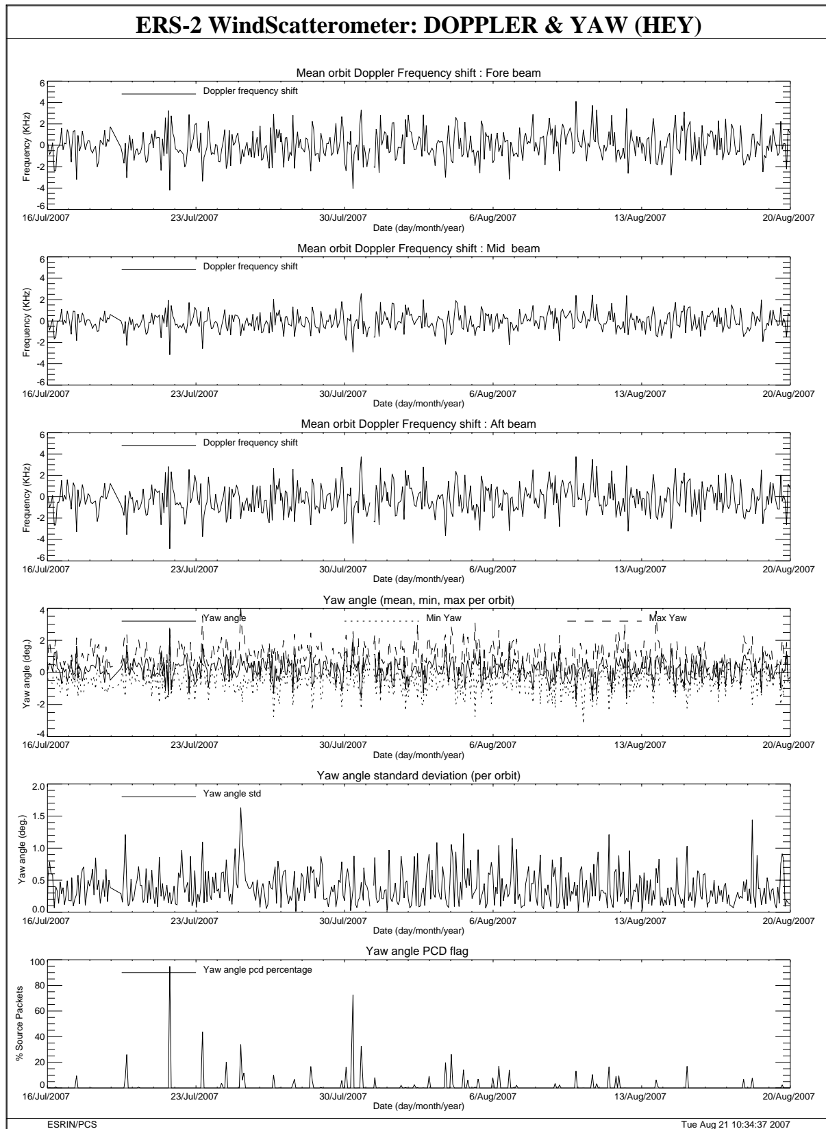
FIGURE 29 Doppler frequency shift and Yaw error angle evolution cycle 128.
