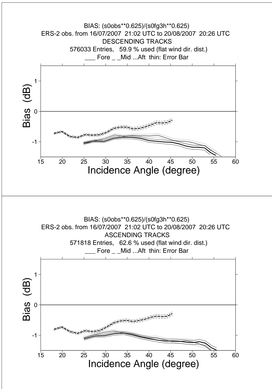
FIGURE 1 ERS-2 Scatterometer Ocean Calibration cycle 128. Ratio of \langle \sigma_0^{0.625} \rangle / \langle CMOD4(First\ Guess)^{0.625} \rangle converted in dB for the fore beam (solid line), mid beam (dashed line) an aft beam (dotted line), as a function of incidence angle for descending and ascending tracks. The thin lines indicate the error bars on the estimated mean. First-guess winds are based on the in time closest (+3h, +6h, +9h, or +12h) T511 forecast field, and are bilinearly interpolated in space.
