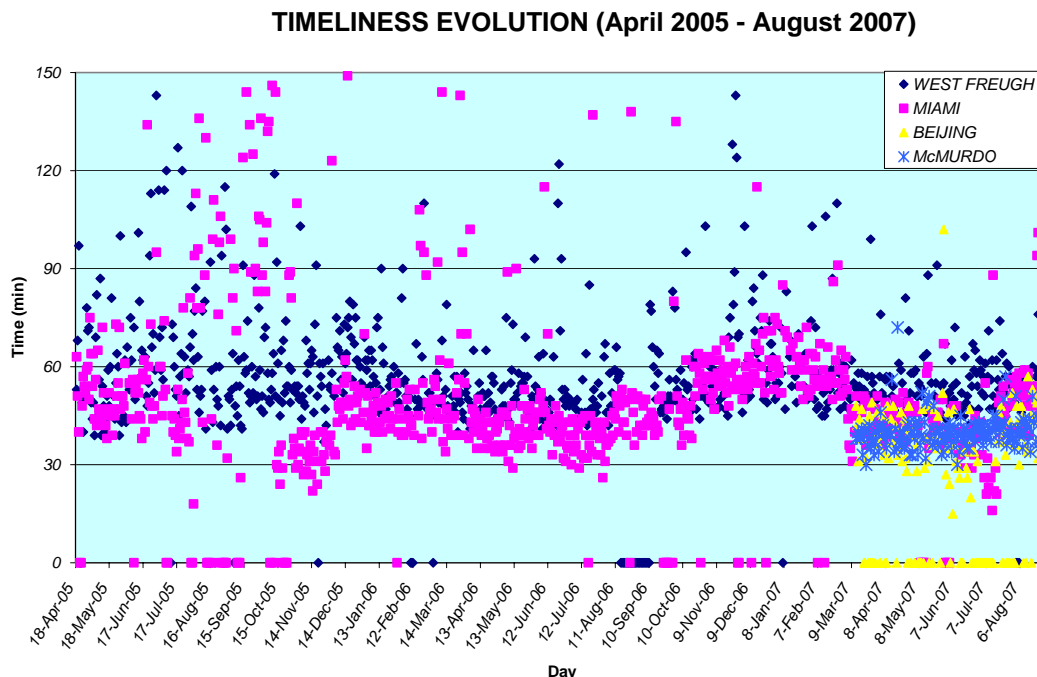
FIGURE 27 : Timeliness evolution from 19 April 2005 to 20 August 2007 for West Freugh, Miami, Beijing and McMurdo ground stations (Timeliness is zero when no products are received).
