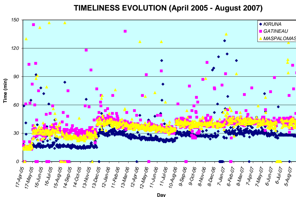
FIGURE 26 : Timeliness evolution from 19 April 2005 to 20 August 2007 for Gatineau, Kiruna and Maspalomas ground stations (Timeliness is zero when no products are received).
