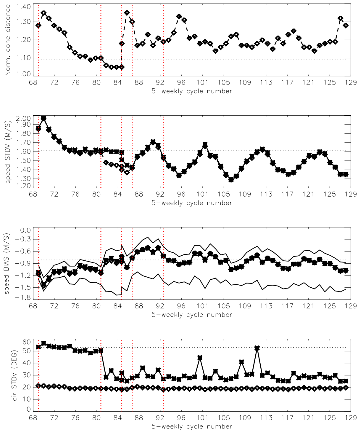
FIGURE 11 Evolution of the performance of the ERS-2 Scatterometer averaged over 5-weekly cycles from 12 December 2001 (cycle 69) to 20 August 2007 (end cycle 128) for the UWI product (solid, star) and de-aliased winds based on CMOD4 (dashed, diamond). Results are based on data that passed the UWI QC flags. For cycle 85 two values are plotted; the first value for the global set, the second one for the regional set. Dotted lines represent values for cycle 59 (5 December 2000 to 17 January 2001), i.e. the last stable cycle of the nominal period. From top to bottom panel are shown the normalized distance to the one (CMOD4 only) the standard deviation of the wind speed compared to FG winds, the corresponding bias (for UWI winds the extreme inter-node averages are shown as well), and the standard deviation of wind direction compared to FG.
