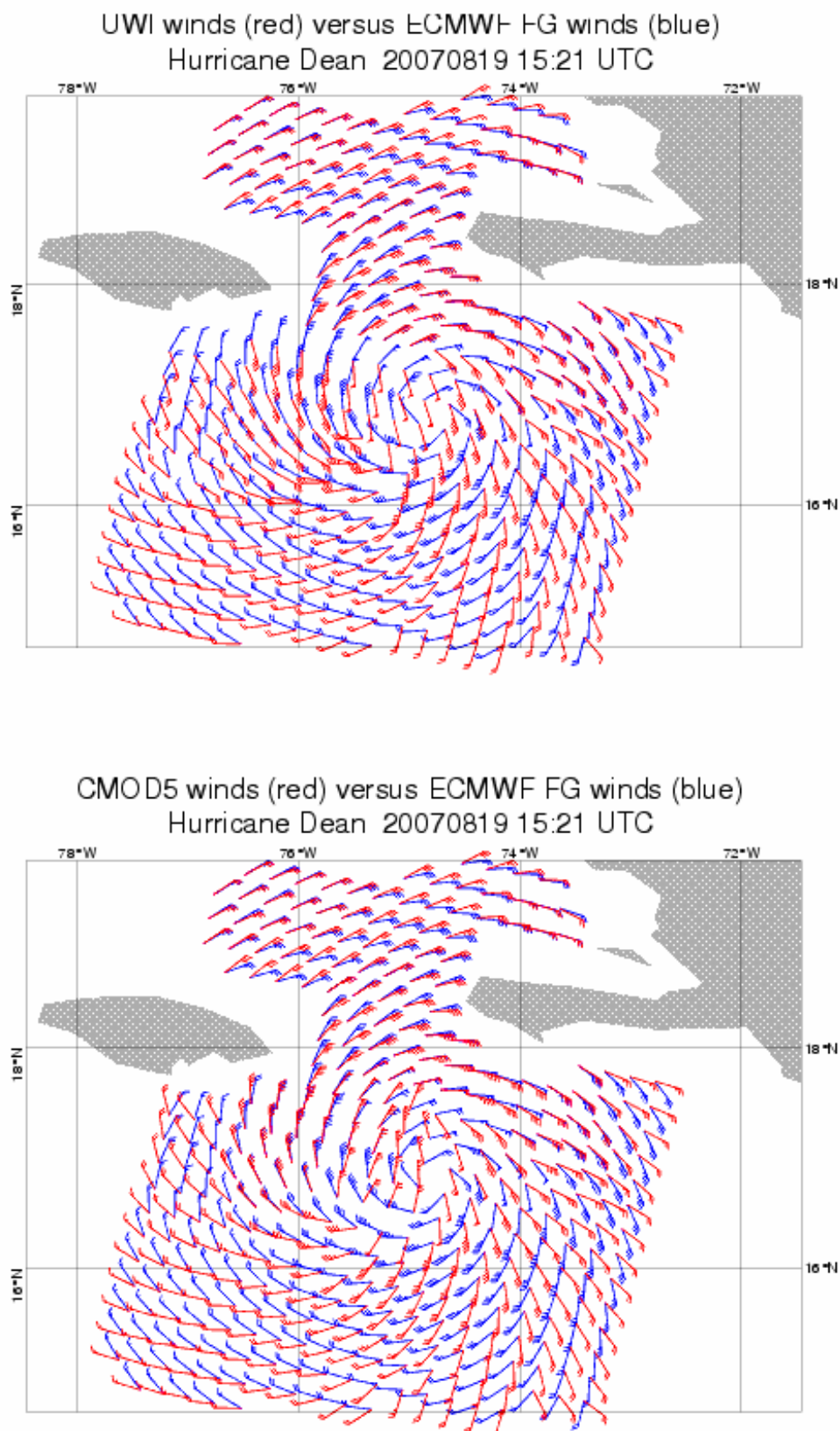
FIGURE 20 Comparison between UWI (top panel) respectively de-aliased CMOD5 (lower panel) winds (red) and ECMWF FG (blue) winds for Hurricane Dean on 19 August 2007 (Category 4), just before it hit Jamaica.
