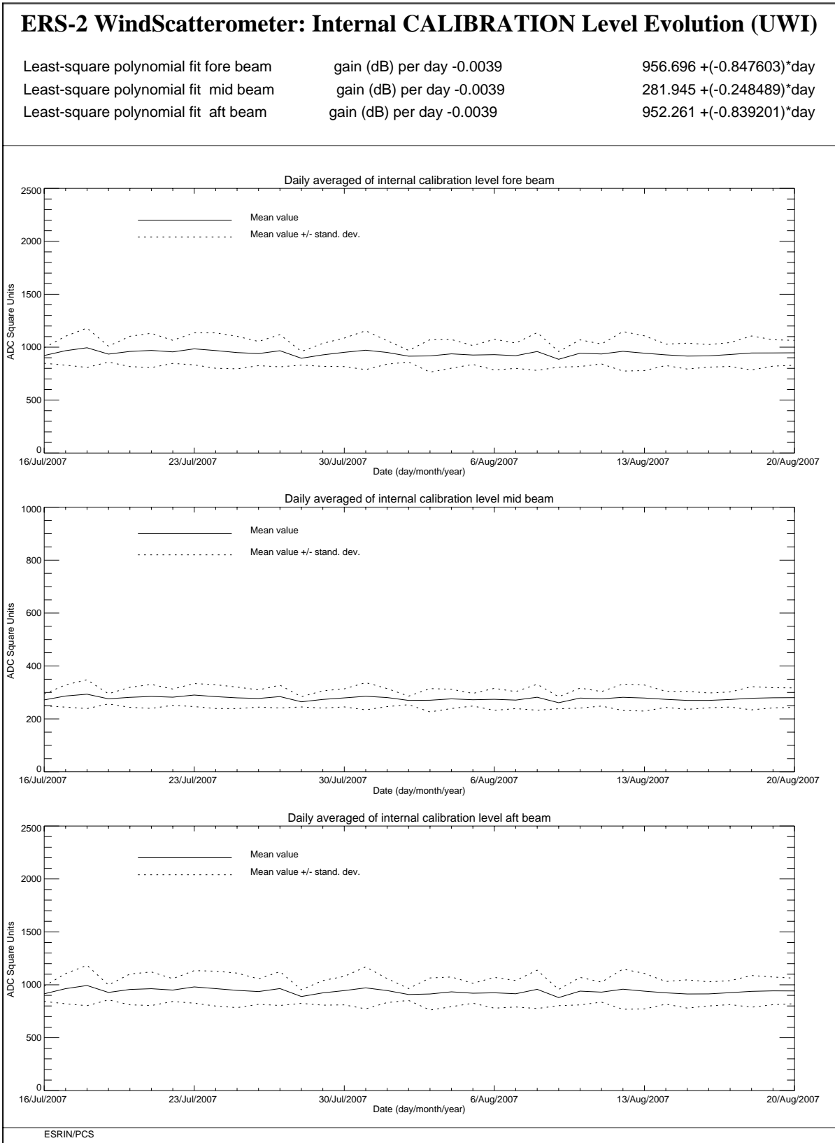
FIGURE 7 ERS-2 Scatterometer: power of internal calibration level cycle 128.
