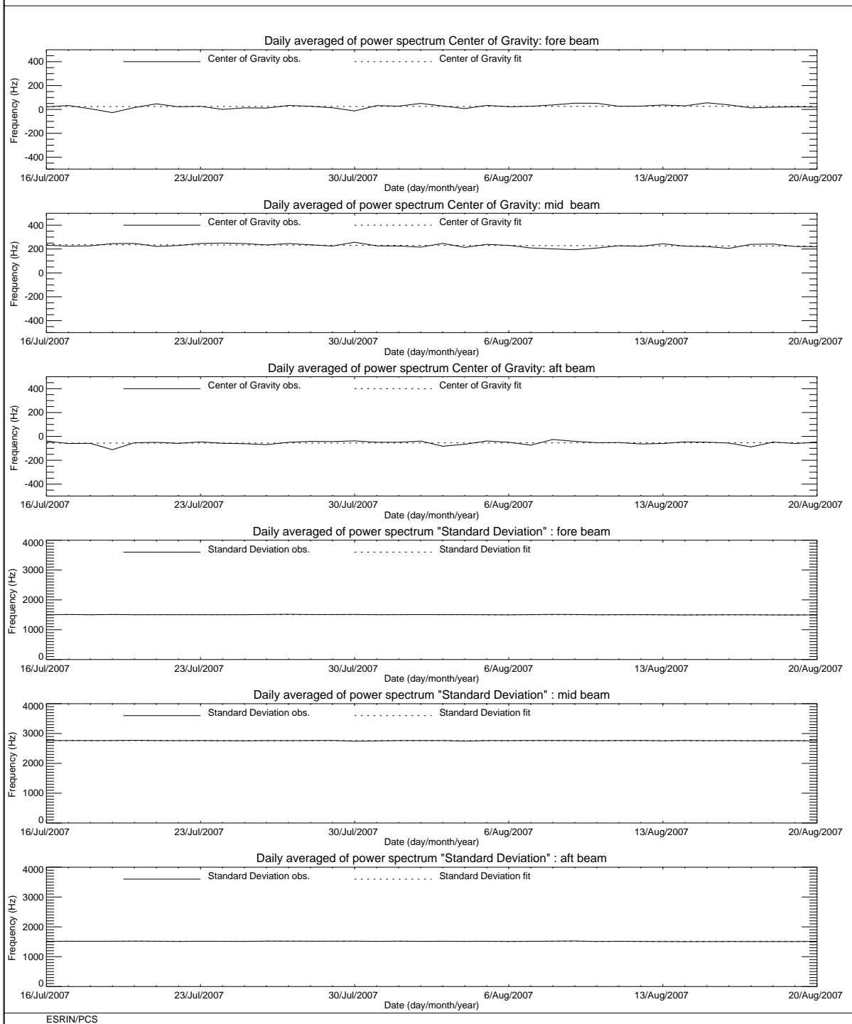
FIGURE 3 ERS-2 Scatterometer: Centre of Gravity and standard deviation of received power spectrum for cycle 128.
