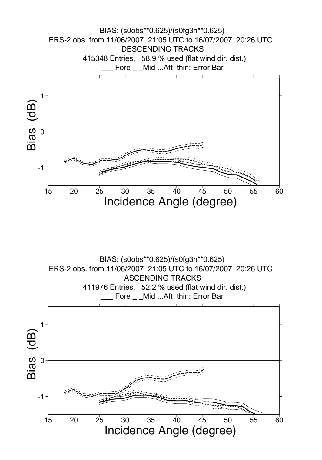
FIGURE 1 ERS-2 Scatterometer Ocean Calibration cycle 127. Ratio of \langle \sigma_0^{0.625} \rangle / \langle CMOD4(\text{First Guess})^{0.625} \rangle converted in dB for the fore beam (solid line), mid beam (dashed line) an aft beam (dotted line), as a function of incidence angle for descending and ascending tracks. The thin lines indicate the error bars on the estimated mean. First-guess winds are based on the in time closest (+3h, +6h, +9h, or +12h) T511 forecast field, and are bilinearly interpolated in space.
