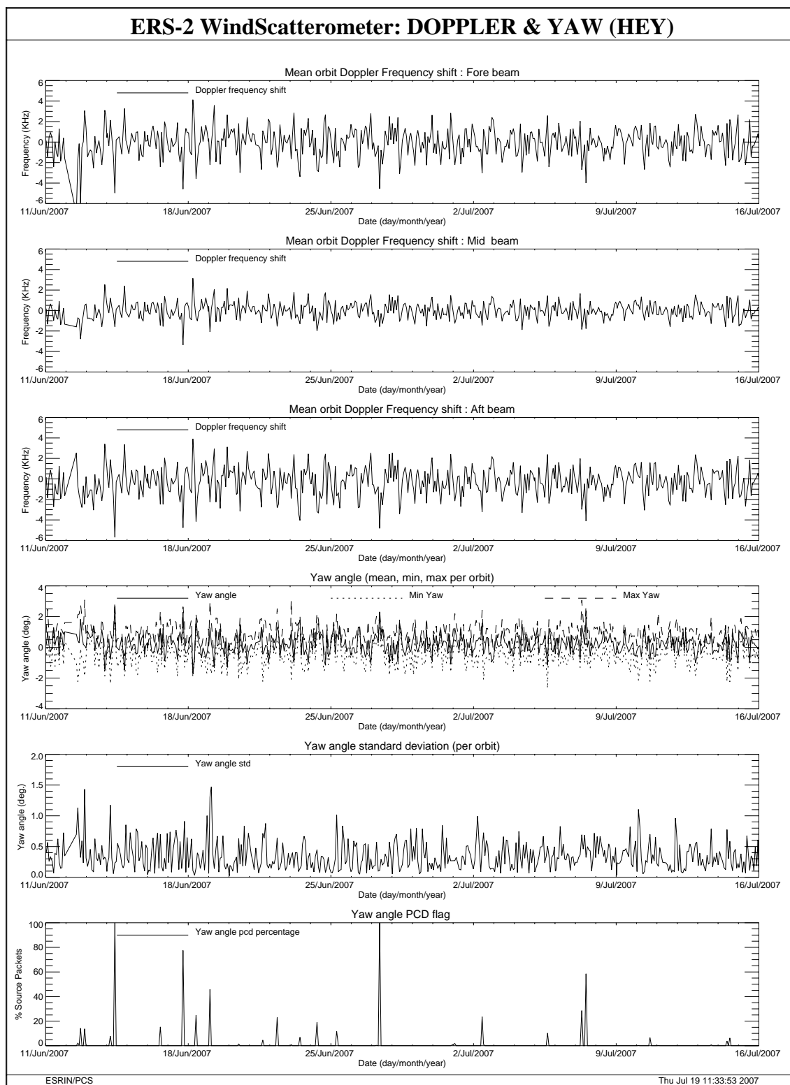
FIGURE 29 Doppler frequency shift and Yaw error angle evolution cycle 127.
