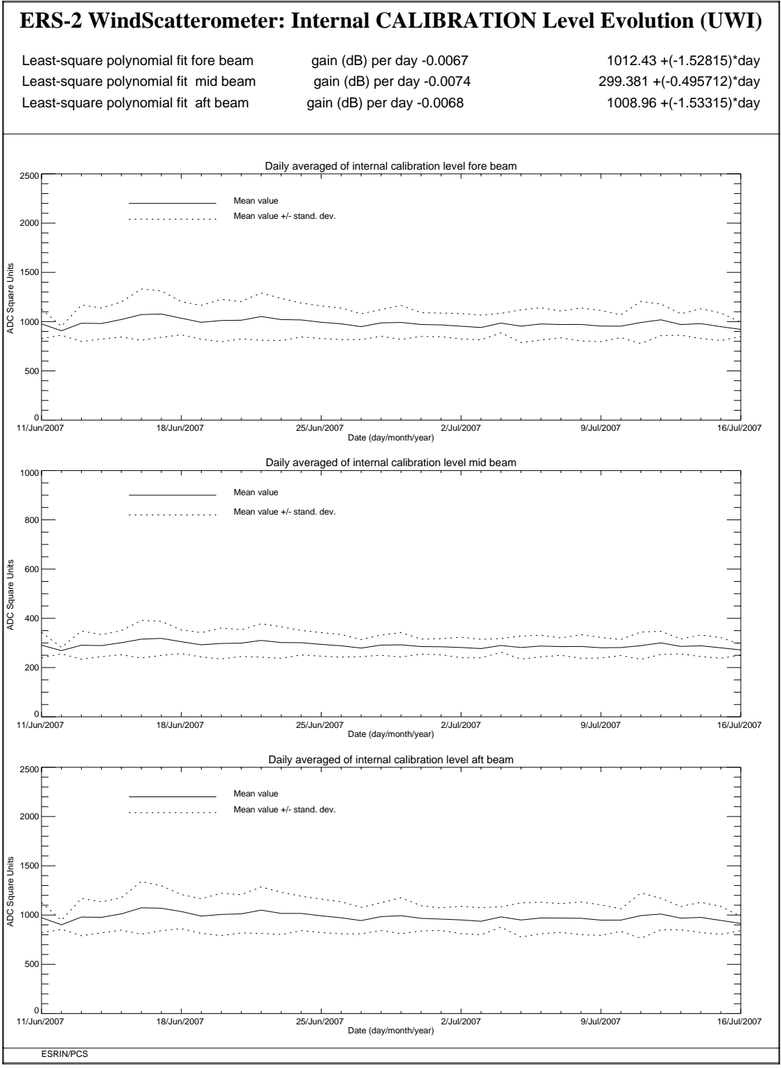
FIGURE 7 ERS-2 Scatterometer: power of internal calibration level cycle 127.
