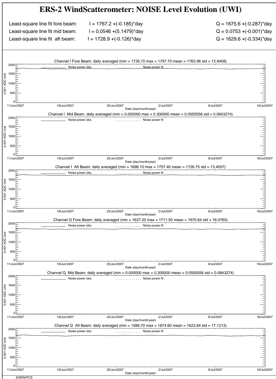
FIGURE 5 ERS-2 Scatterometer: noise power I and Q channel for cycle 127.
