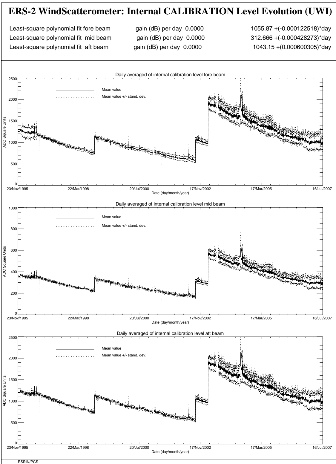
FIGURE 6 ERS-2 Scatterometer: power of internal calibration pulse since the beginning of the mission.
