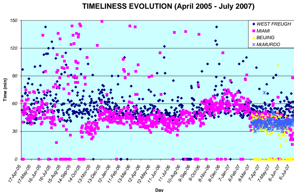
FIGURE 27 : Timeliness evolution from 19 April 2005 to 16 July 2007 for West Freugh, Miami, Beijing and McMurdo ground stations (Timeliness is zero when no products are received).
