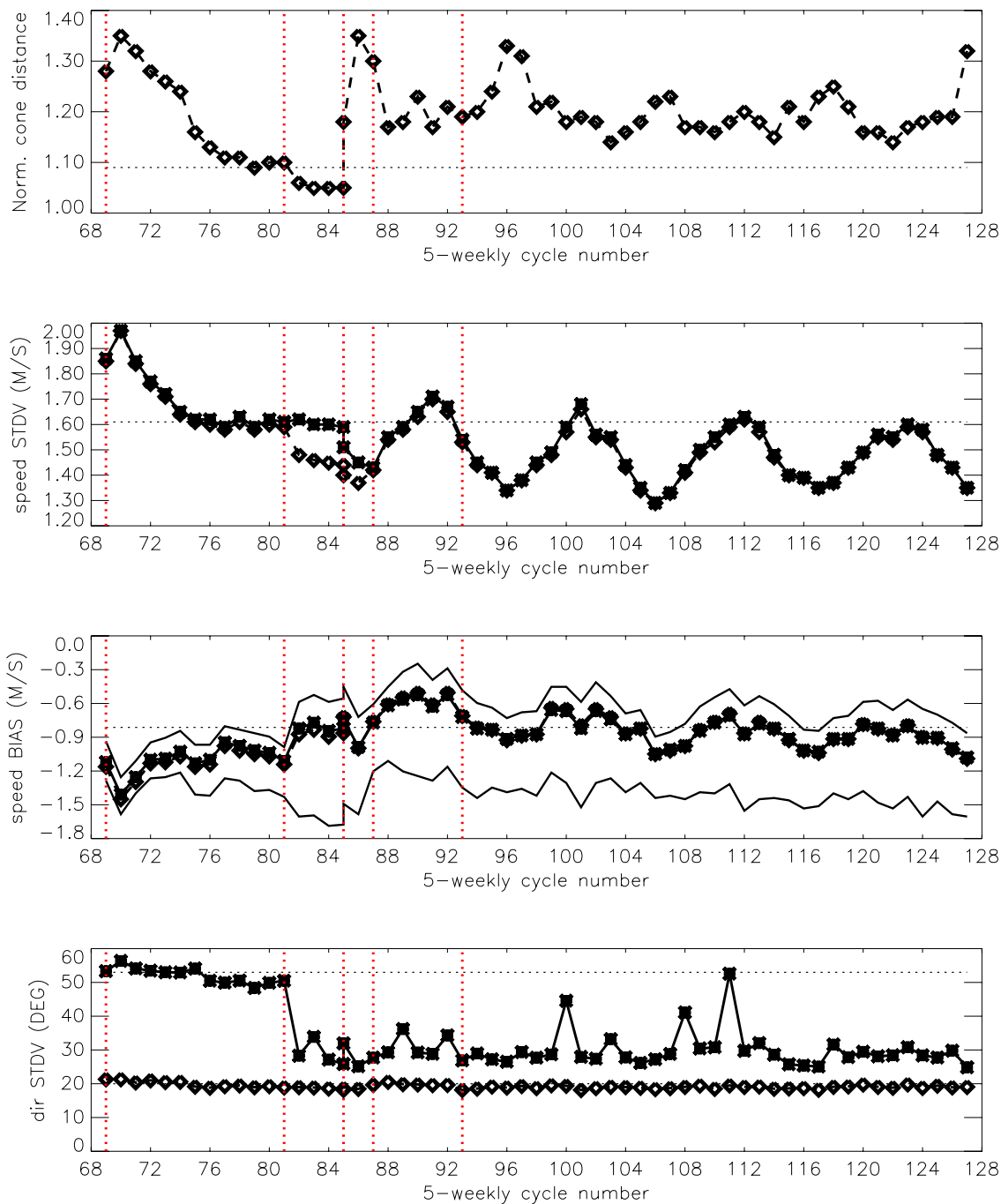
FIGURE 11 Evolution of the performance of the ERS-2 Scatterometer averaged over 5-weekly cycles from 12 December 2001 (cycle 69) to 16 July 2007 (end cycle 127) for the UWI product (solid, star) and de-aliased winds based on CMOD4 (dashed, diamond). Results are based on data that passed the UWI QC flags. For cycle 85 two values are plotted; the first value for the global set, the second one for the regional set. Dotted lines represent values for cycle 59 (5 December 2000 to 17 January 2001), i.e. the last stable cycle of the nominal period. From top to bottom panel are shown the normalized distance to the one (CMOD4 only) the standard deviation of the wind speed compared to FG winds, the corresponding bias (for UWI winds the extreme inter-node averages are shown as well), and the standard deviation of wind direction compared to FG.
