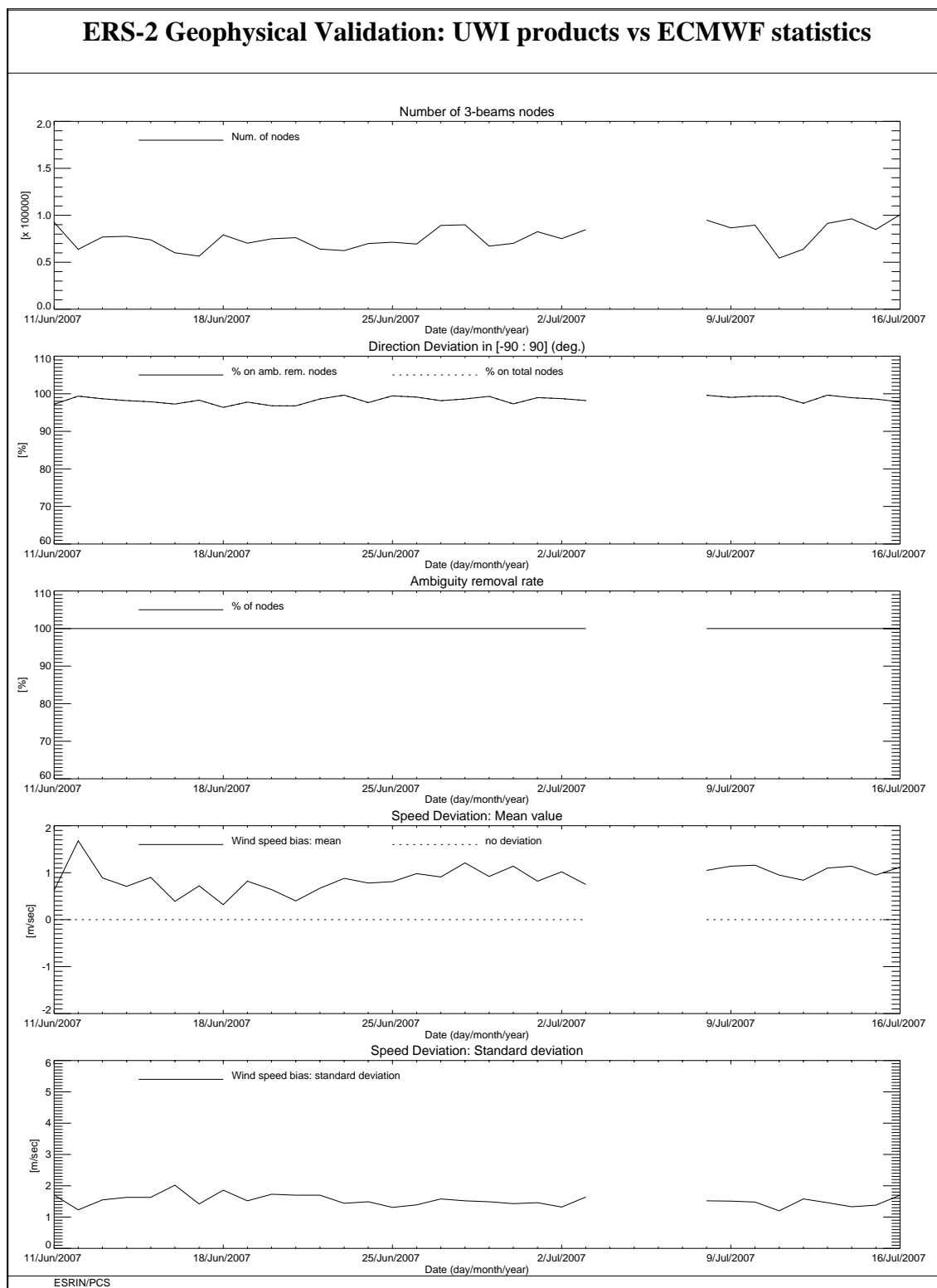
FIGURE 10 ERS-2 Scatterometer: wind products performance for cycle 127.
