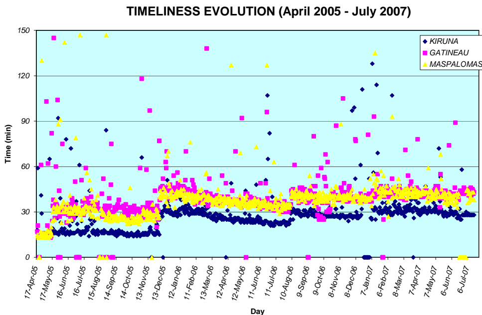
FIGURE 26 : Timeliness evolution from 19 April 2005 to 16 July 2007 for Gatineau, Kiruna and Maspalomas ground stations (Timeliness is zero when no products are received).
