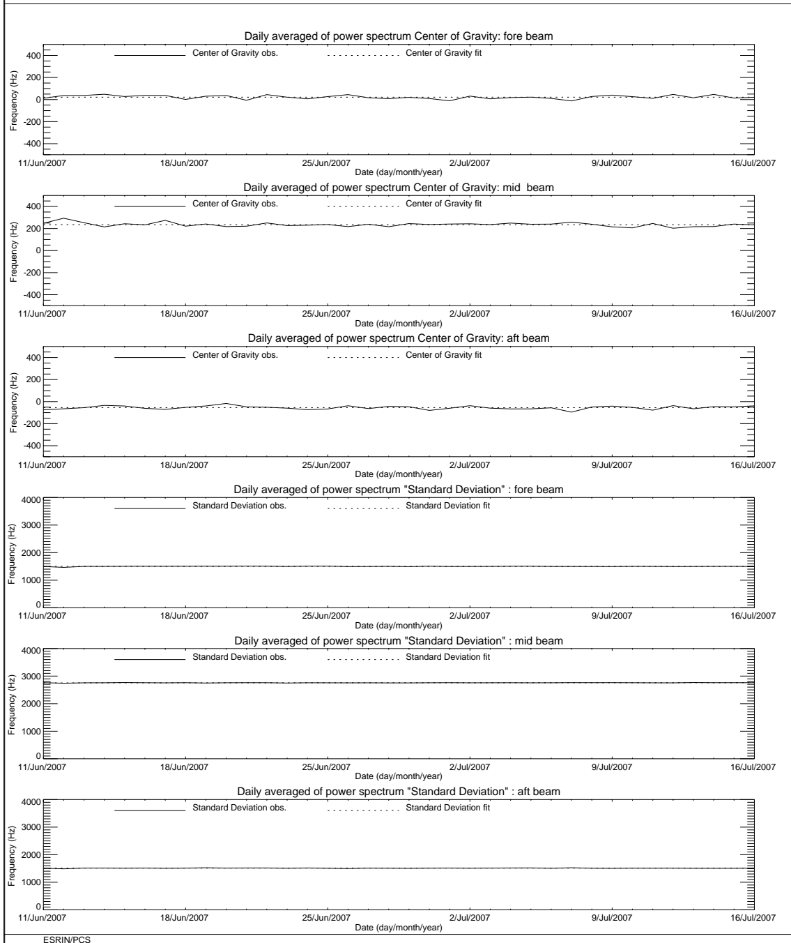
FIGURE 3 ERS-2 Scatterometer: Centre of Gravity and standard deviation of received power spectrum for cycle 127.
