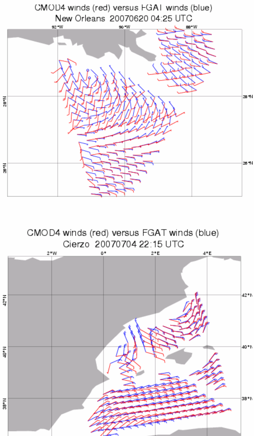
FIGURE 20 Comparison between UWI (red) and ECMWF FG (blue) winds for a case South New Orleans on 20 June 2007 (top panel) and for a case South of Tortosa (Spain) for 4 July 2007 (lower panel).
