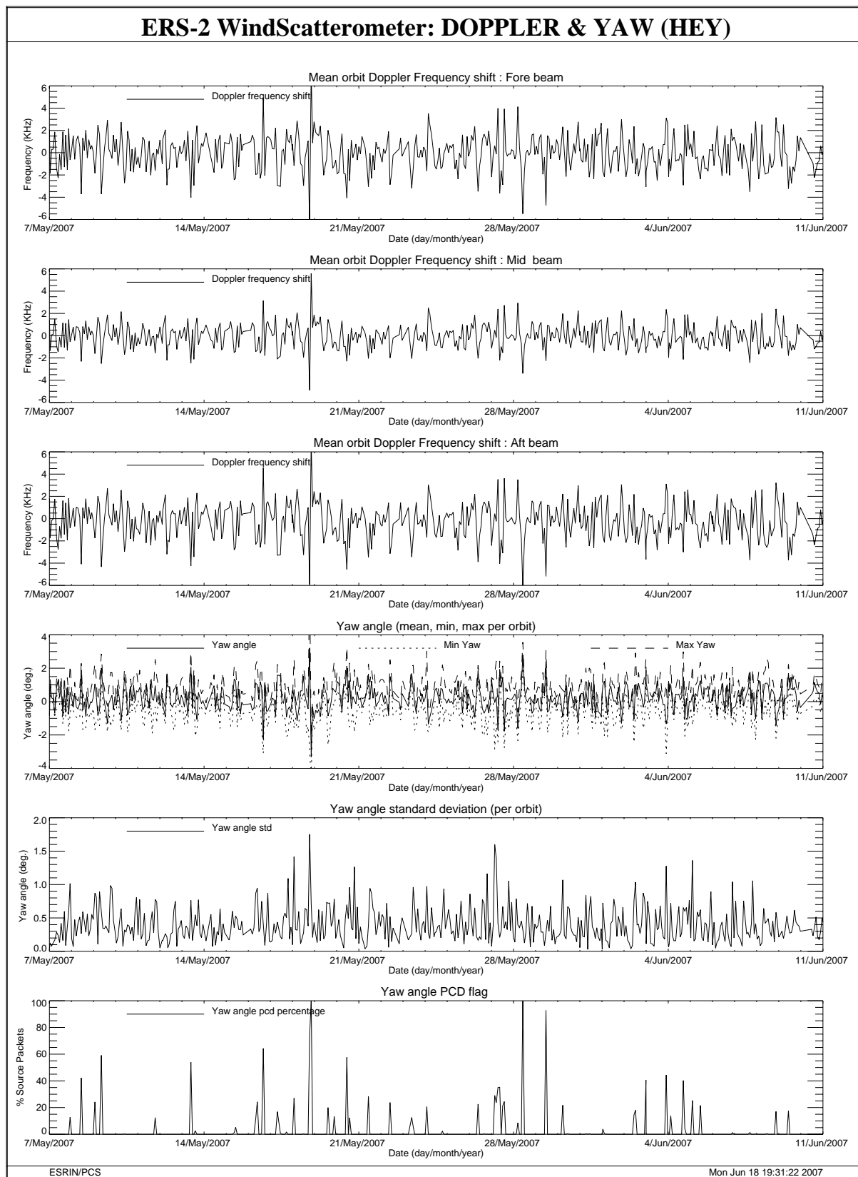
FIGURE 29 Doppler frequency shift and Yaw error angle evolution cycle 126.
