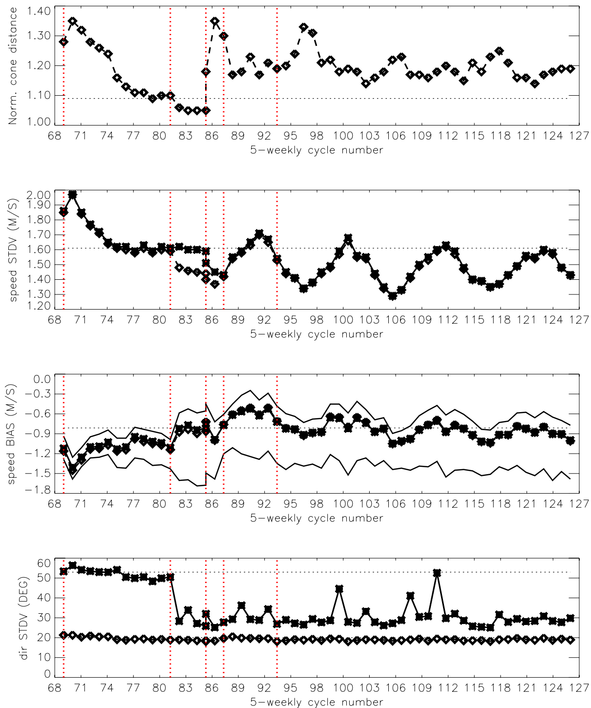
FIGURE 11 Evolution of the performance of the ERS-2 Scatterometer averaged over 5-weekly cycles from 12 December 2001 (cycle 69) to 11 June 2007 (end cycle 126) for the UWI product (solid, star) and de-aliased winds based on CMOD4 (dashed, diamond). Results are based on data that passed the UWI QC flags. For cycle 85 two values are plotted; the first value for the global set, the second one for the regional set. Dotted lines represent values for cycle 59 (5 December 2000 to 17 January 2001), i.e. the last stable cycle of the nominal period. From top to bottom panel are shown the normalized distance to the one (CMOD4 only) the standard deviation of the wind speed compared to FG winds, the corresponding bias (for UWI winds the extreme inter-node averages are shown as well), and the standard deviation of wind direction compared to FG.
