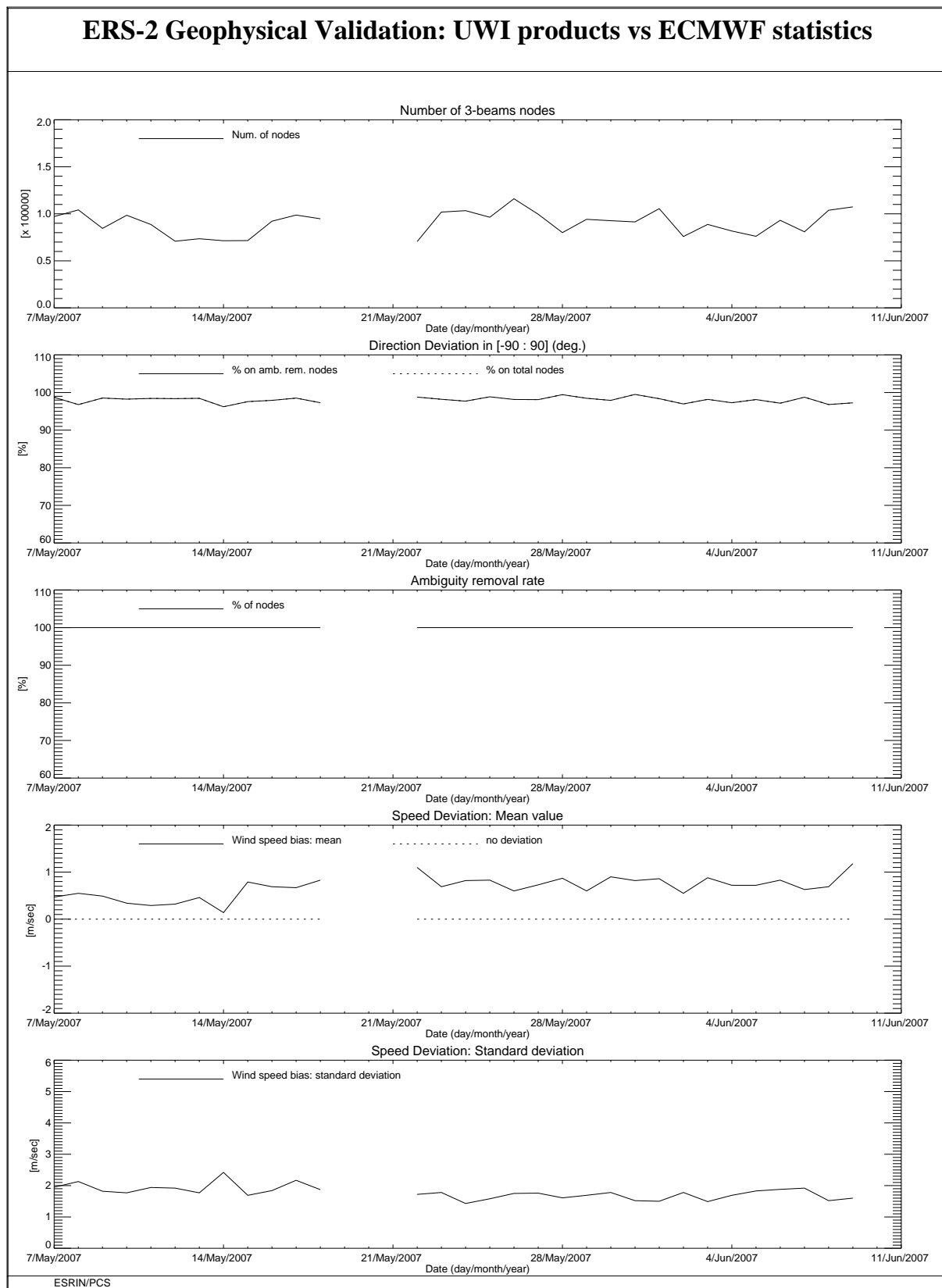
FIGURE 10 ERS-2 Scatterometer: wind products performance for cycle 126.
