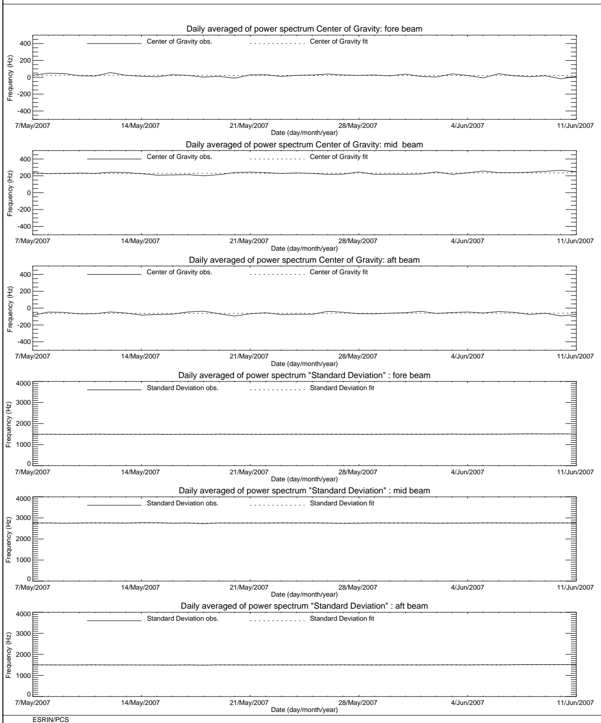
FIGURE 3 ERS-2 Scatterometer: Centre of Gravity and standard deviation of received power spectrum for cycle 126.
