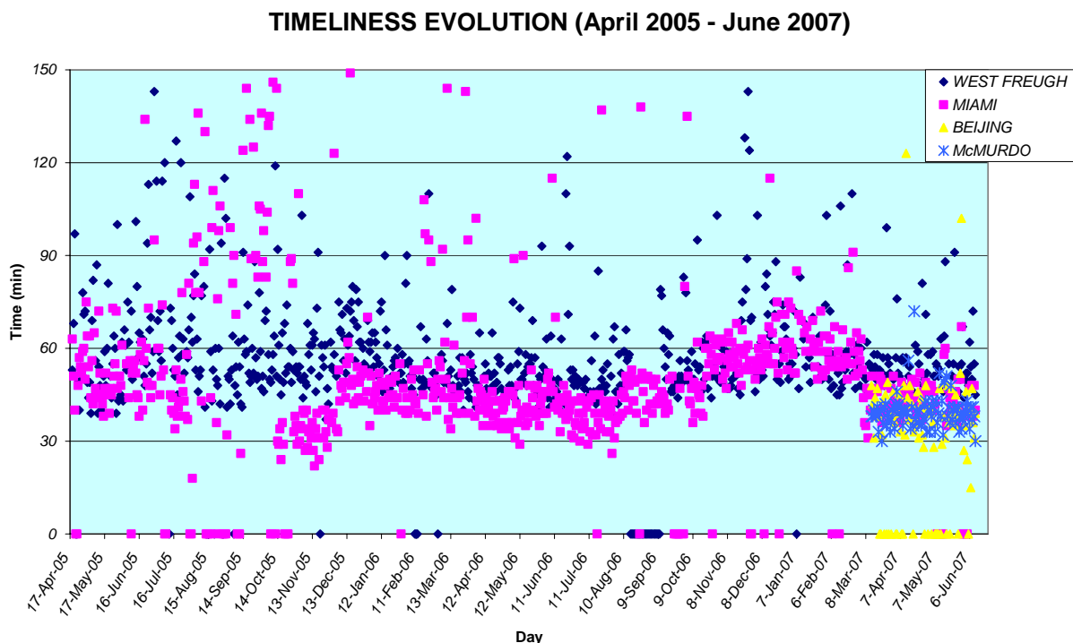
FIGURE 27 : Timeliness evolution from 19 April 2005 to 11 June 2007 for West Freugh, Miami, Beijing and McMurdo ground stations.
