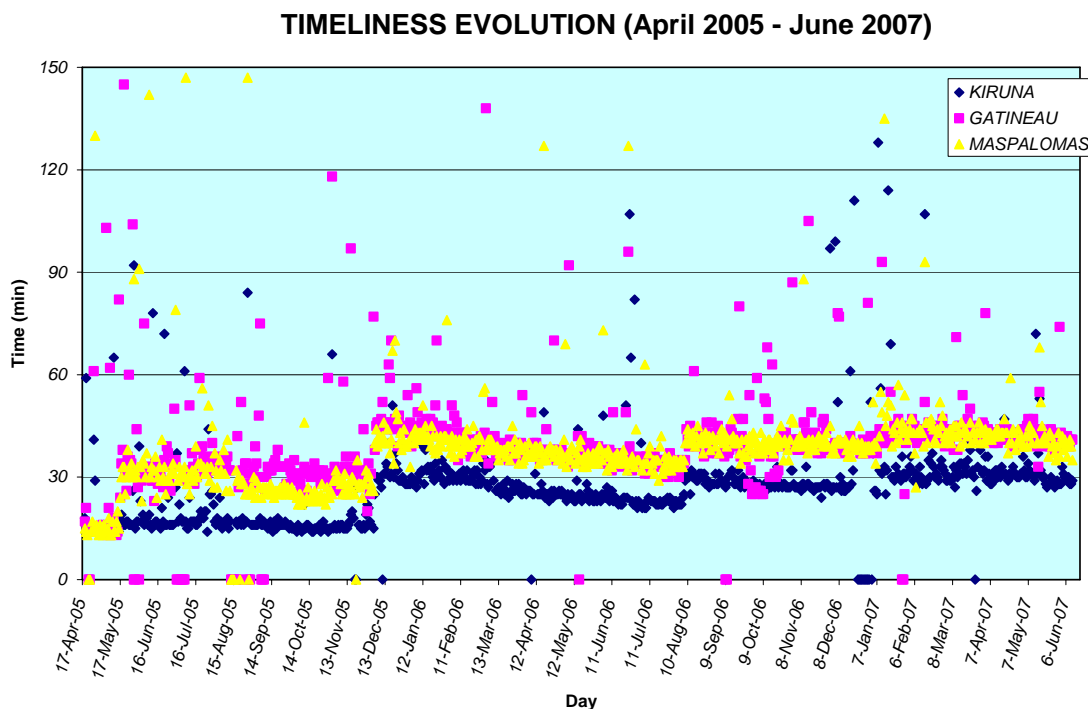
FIGURE 26 : Timeliness evolution from 19 April 2005 to 11 June 2007 for Gatineau, Kiruna and Maspalomas ground stations.
