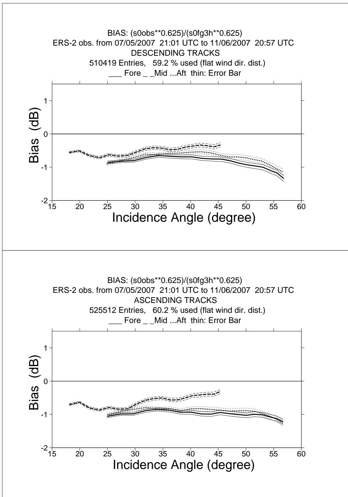
FIGURE 1 ERS-2 Scatterometer Ocean Calibration cycle 126. Ratio of \langle \sigma_0^{0.625} \rangle / \langle CMOD4(\text{First Guess})^{0.625} \rangle converted in dB for the fore beam (solid line), mid beam (dashed line) an aft beam (dotted line), as a function of incidence angle for descending and ascending tracks. The thin lines indicate the error bars on the estimated mean. First-guess winds are based on the in time closest (+3h, +6h, +9h, or +12h) T511 forecast field, and are bilinearly interpolated in space.
