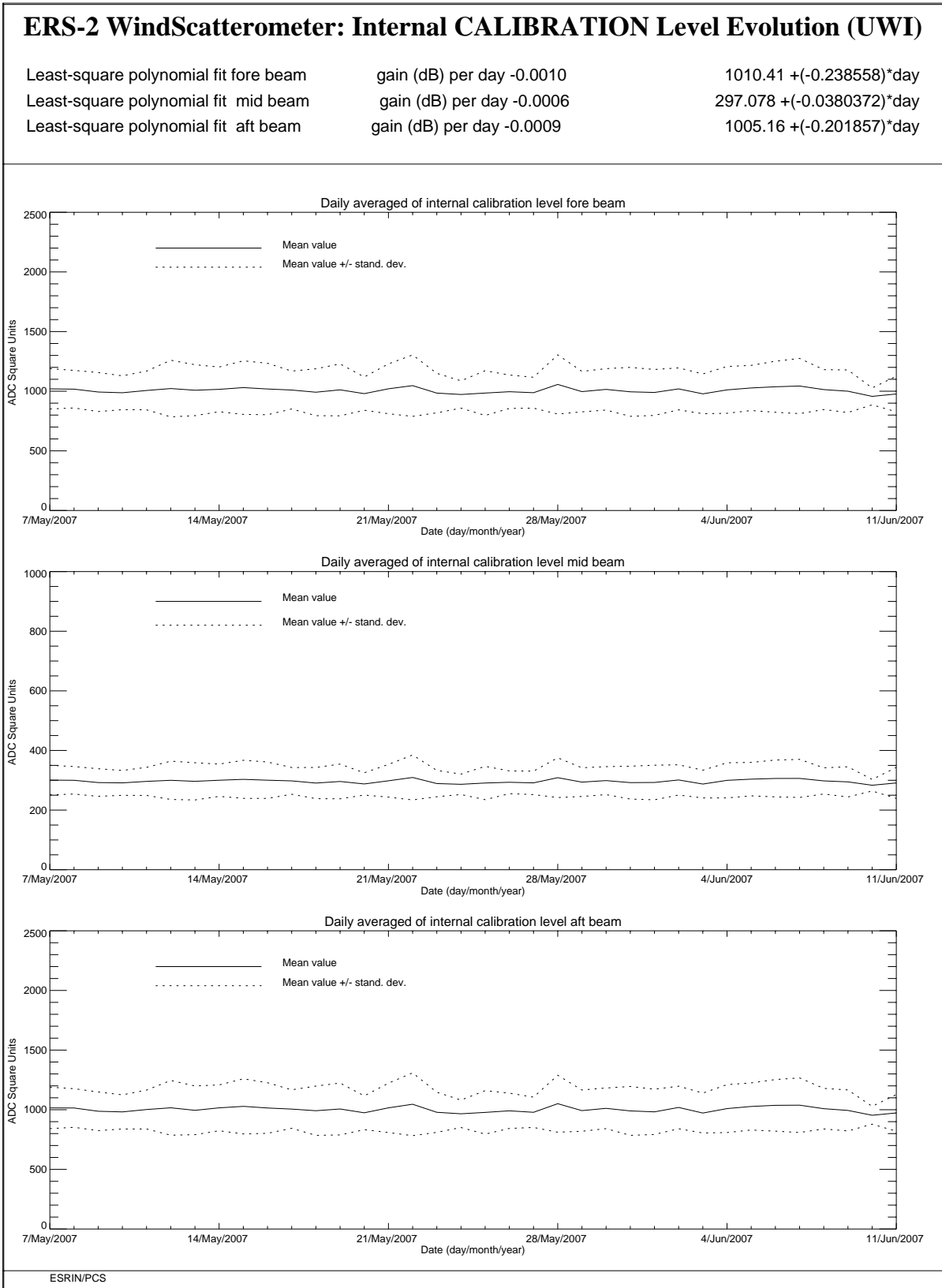
FIGURE 7 ERS-2 Scatterometer: power of internal calibration level cycle 126.
