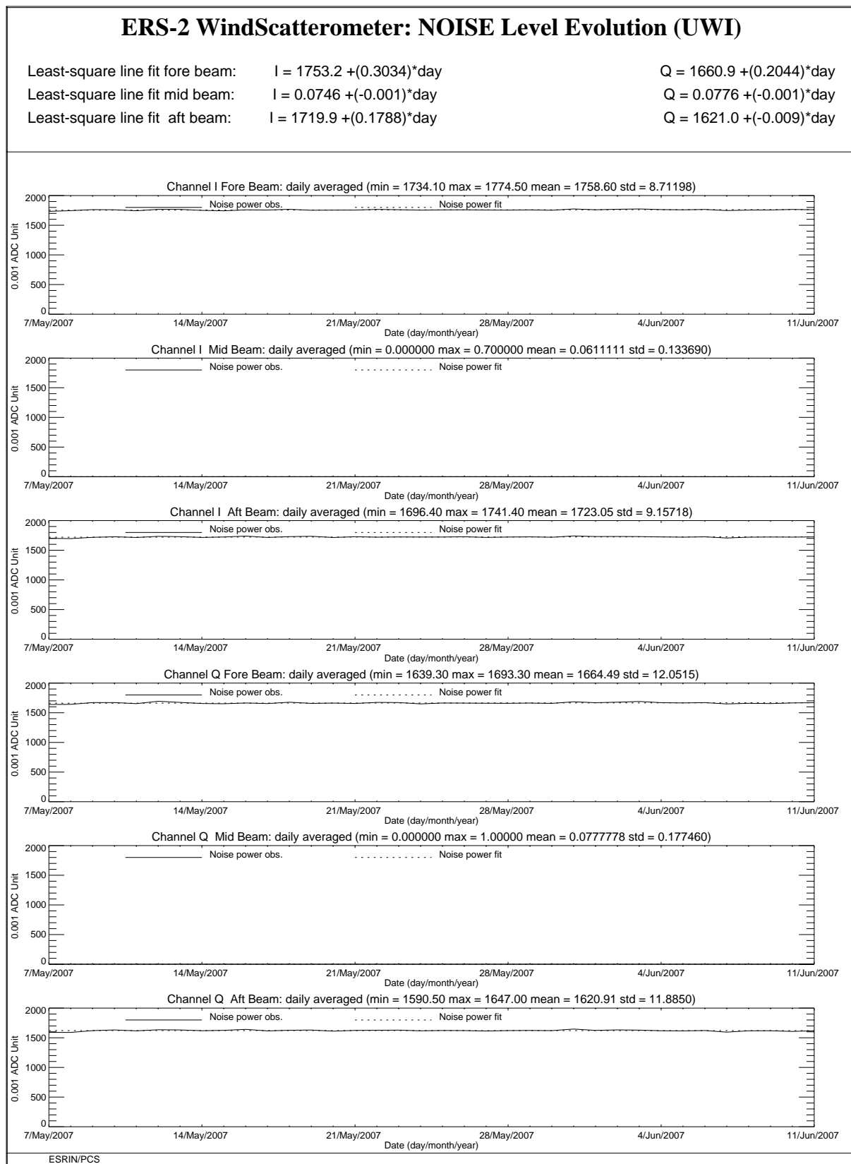
FIGURE 5 ERS-2 Scatterometer: noise power I and Q channel for cycle 126.
