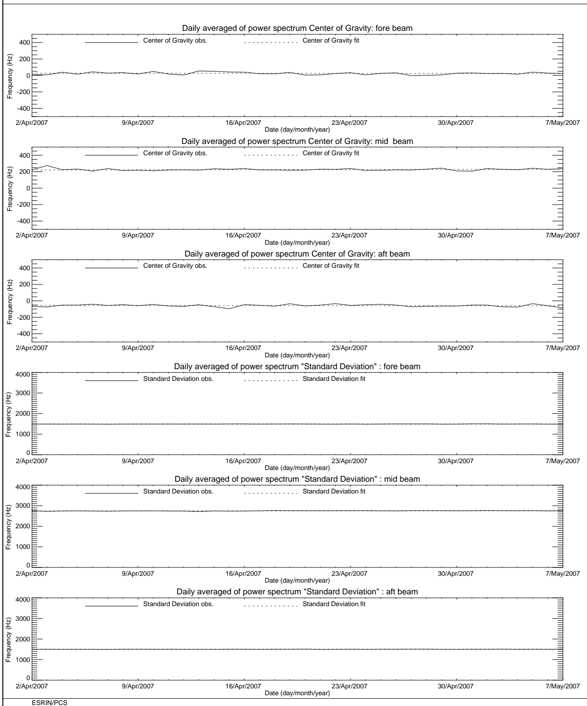
FIGURE 3 ERS-2 Scatterometer: Centre of Gravity and standard deviation of received power spectrum for cycle 125.
