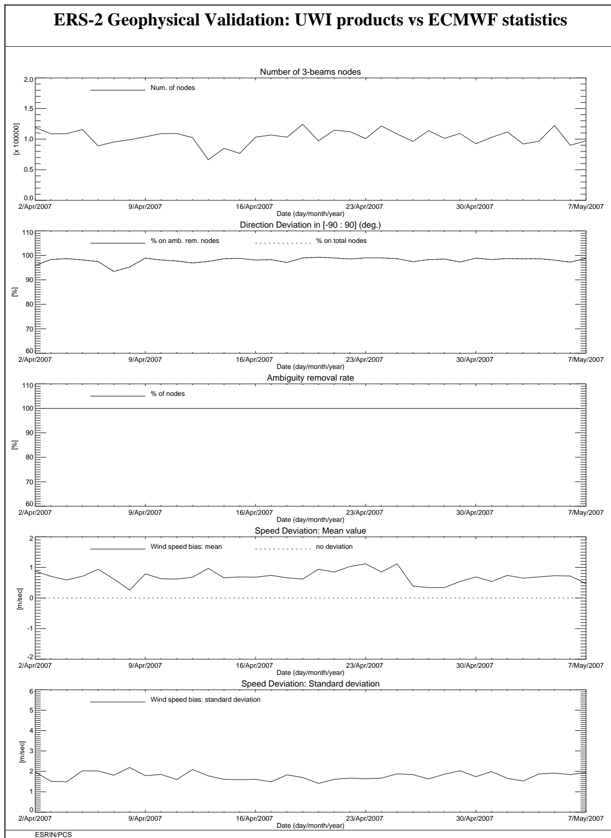
FIGURE 10 ERS-2 Scatterometer: wind products performance for cycle 125.
