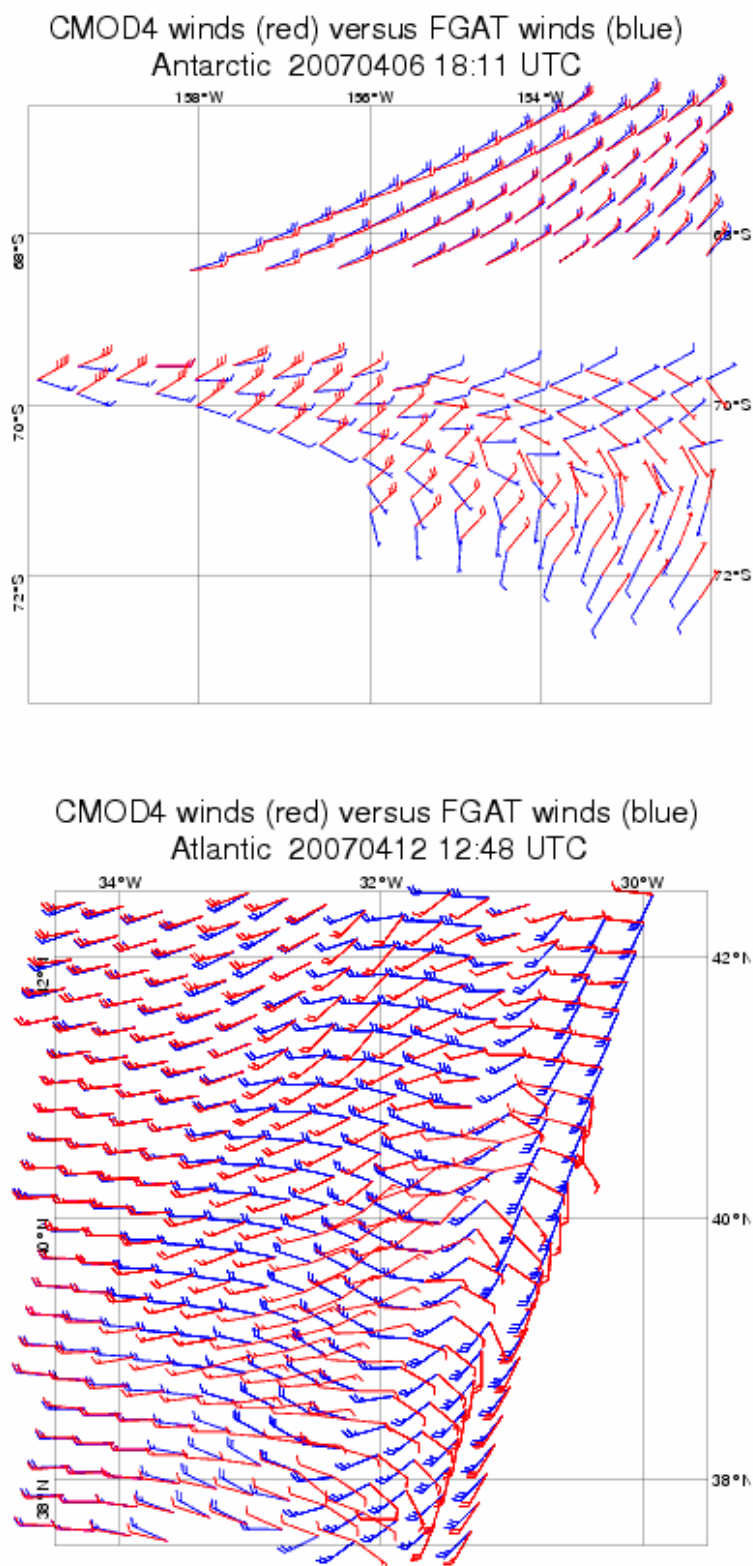
FIGURE 20 Comparison between UWI (red) and ECMWF FG (blue) winds for a case in the Antarctic region on 6 April 2007 (top panel) and for a case in the North Atlantic for 12 April 2007 (lower panel).
