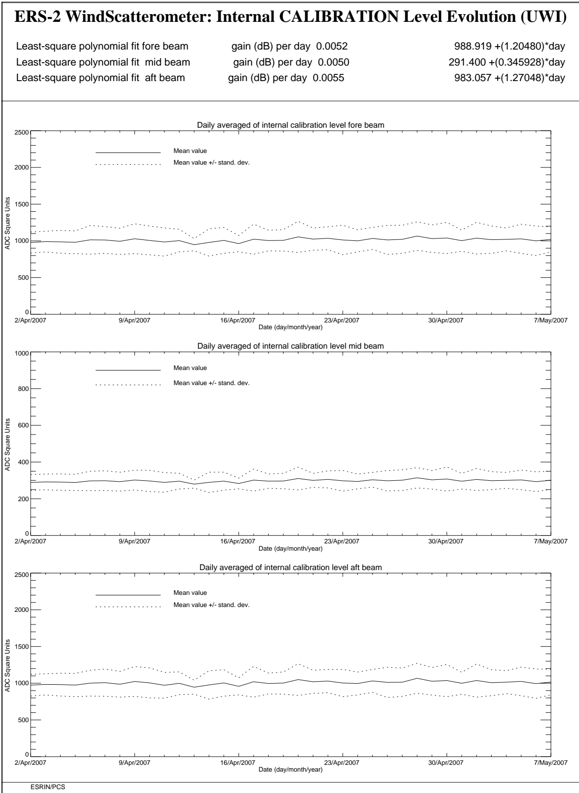
FIGURE 7 ERS-2 Scatterometer: power of internal calibration level cycle 125.
