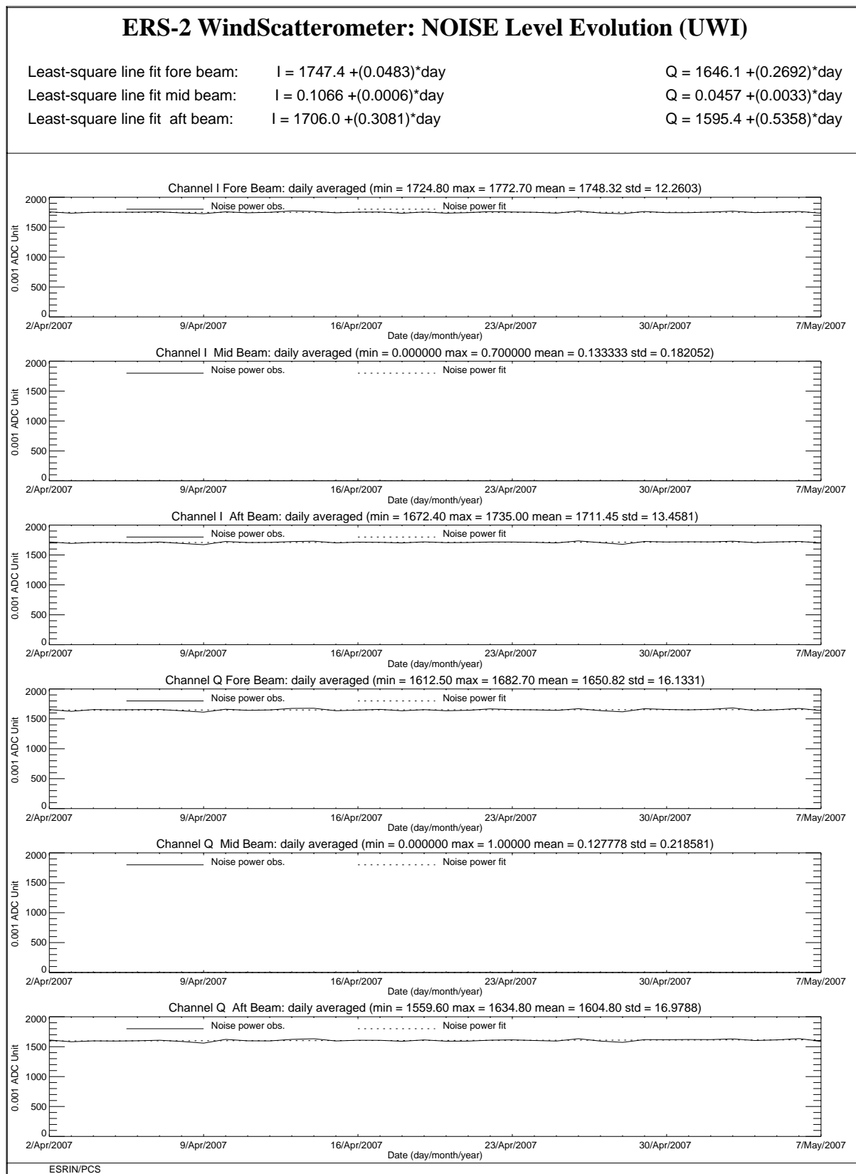
FIGURE 5 ERS-2 Scatterometer: noise power I and Q channel for cycle 125.
