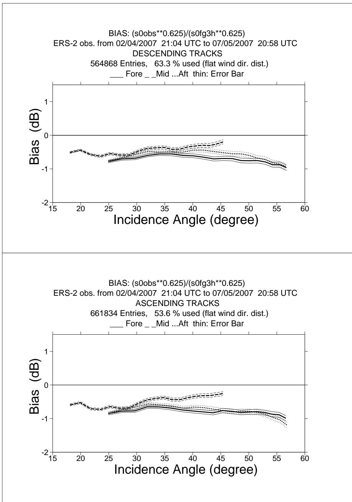
FIGURE 1 ERS-2 Scatterometer Ocean Calibration cycle 125. Ratio of \langle \sigma_0^{0.625} \rangle / \langle CMOD4(\text{First Guess})^{0.625} \rangle converted in dB for the fore beam (solid line), mid beam (dashed line) an aft beam (dotted line), as a function of incidence angle for descending and ascending tracks. The thin lines indicate the error bars on the estimated mean. First-guess winds are based on the in time closest (+3h, +6h, +9h, or +12h) T511 forecast field, and are bilinearly interpolated in space.
