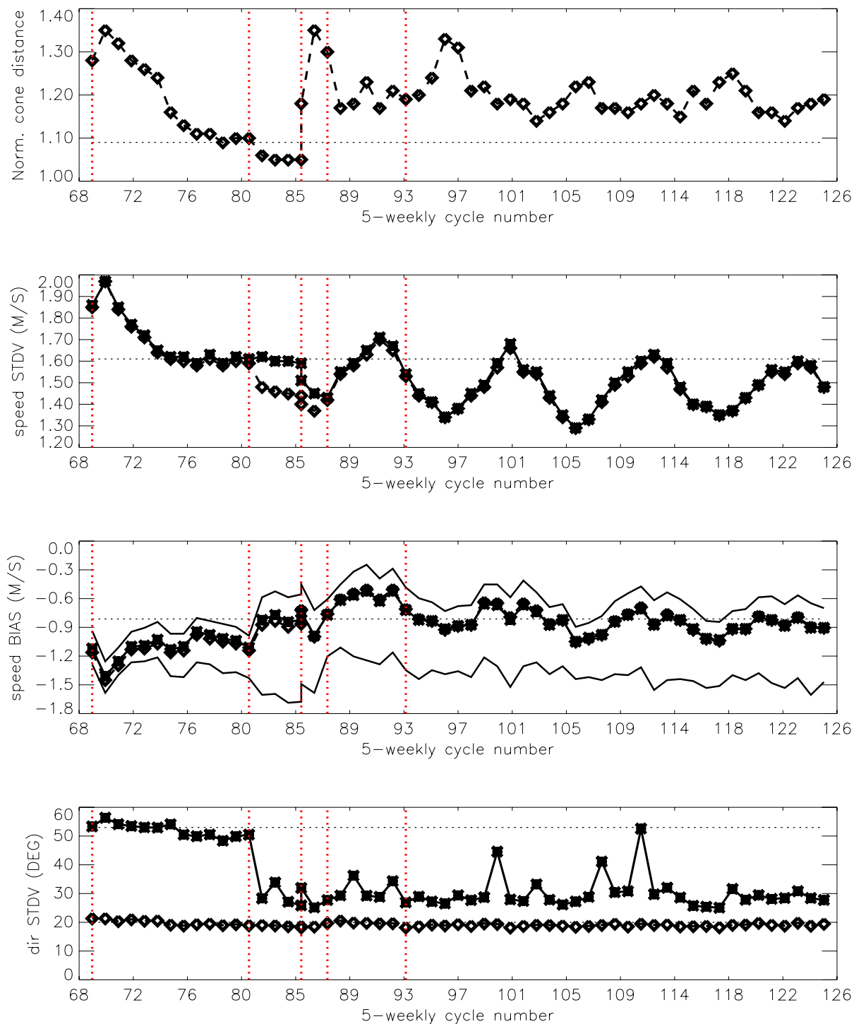
FIGURE 11 Evolution of the performance of the ERS-2 Scatterometer averaged over 5-weekly cycles from 12 December 2001 (cycle 69) to 7 May 2007 (end cycle 125) for the UWI product (solid, star) and de-aliased winds based on CMOD4 (dashed, diamond). Results are based on data that passed the UWI QC flags. For cycle 85 two values are plotted; the first value for the global set, the second one for the regional set. Dotted lines represent values for cycle 59 (5 December 2000 to 17 January 2001), i.e. the last stable cycle of the nominal period. From top to bottom panel are shown the normalized distance to the one (CMOD4 only) the standard deviation of the wind speed compared to FG winds, the corresponding bias (for UWI winds the extreme inter-node averages are shown as well), and the standard deviation of wind direction compared to FG.
