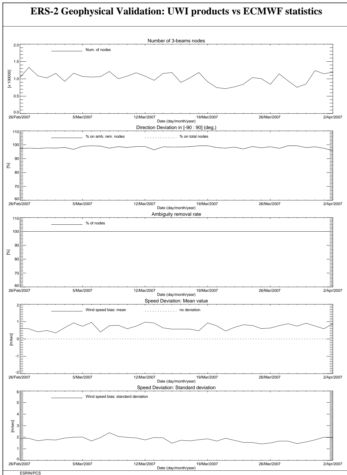
FIGURE 10 ERS-2 Scatterometer: wind products performance for cycle 124.
