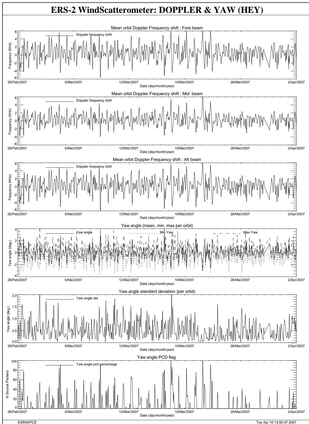
FIGURE 27 Doppler frequency shift and Yaw error angle evolution cycle 124.
