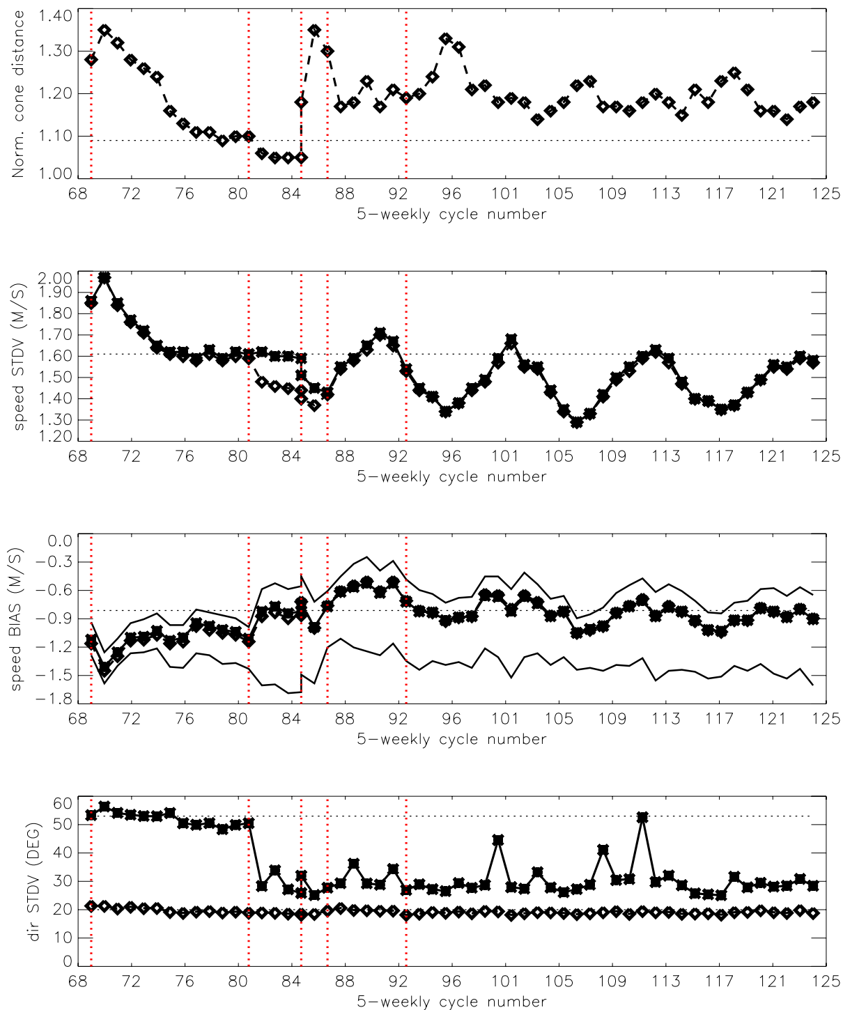
FIGURE 11 Evolution of the performance of the ERS-2 Scatterometer averaged over 5-weekly cycles from 12 December 2001 (cycle 69) to 2 April 2007 (end cycle 124) for the UWI product (solid, star) and de-aliased winds based on CMOD4(dashed, diamond). Results are based on data that passed the UWI QC flags. For cycle 85 two values are plotted; the first value for the global set, the second one for the regional set. Dotted lines represent values for cycle 59 (5 December 2000 to 17 January 2001),i.e. the last stable cycle of the nominal period. From top to bottom panel are shown the normalized distance to the one (CMOD4 only) the standard deviation of the wind speed compared to FG winds, the corresponding bias (for UWI winds the extreme inter-node averages are shown as well),and the standard deviation of wind direction compared to FG.
