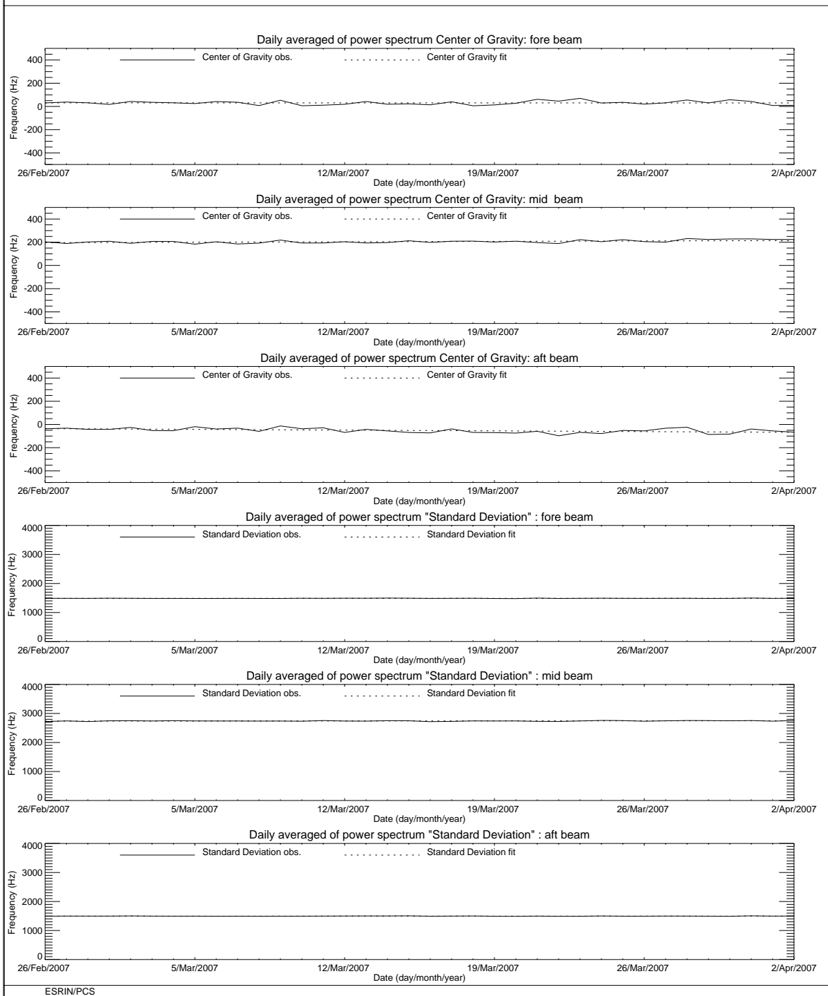
FIGURE 3 ERS-2 Scatterometer: Centre of Gravity and standard deviation of received power spectrum for cycle 124.
