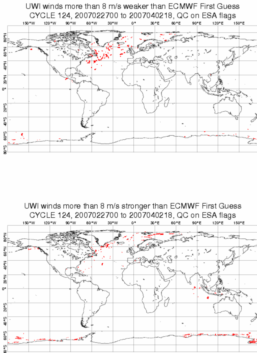
FIGURE 19 Locations of data during cycle 124 for which UWI winds are more than 8 m/s weaker (top panel) respectively stronger (lower panel) than FGAT, and on which QC on UWI flags and the ECMWF land/sea-ice mask was applied.
