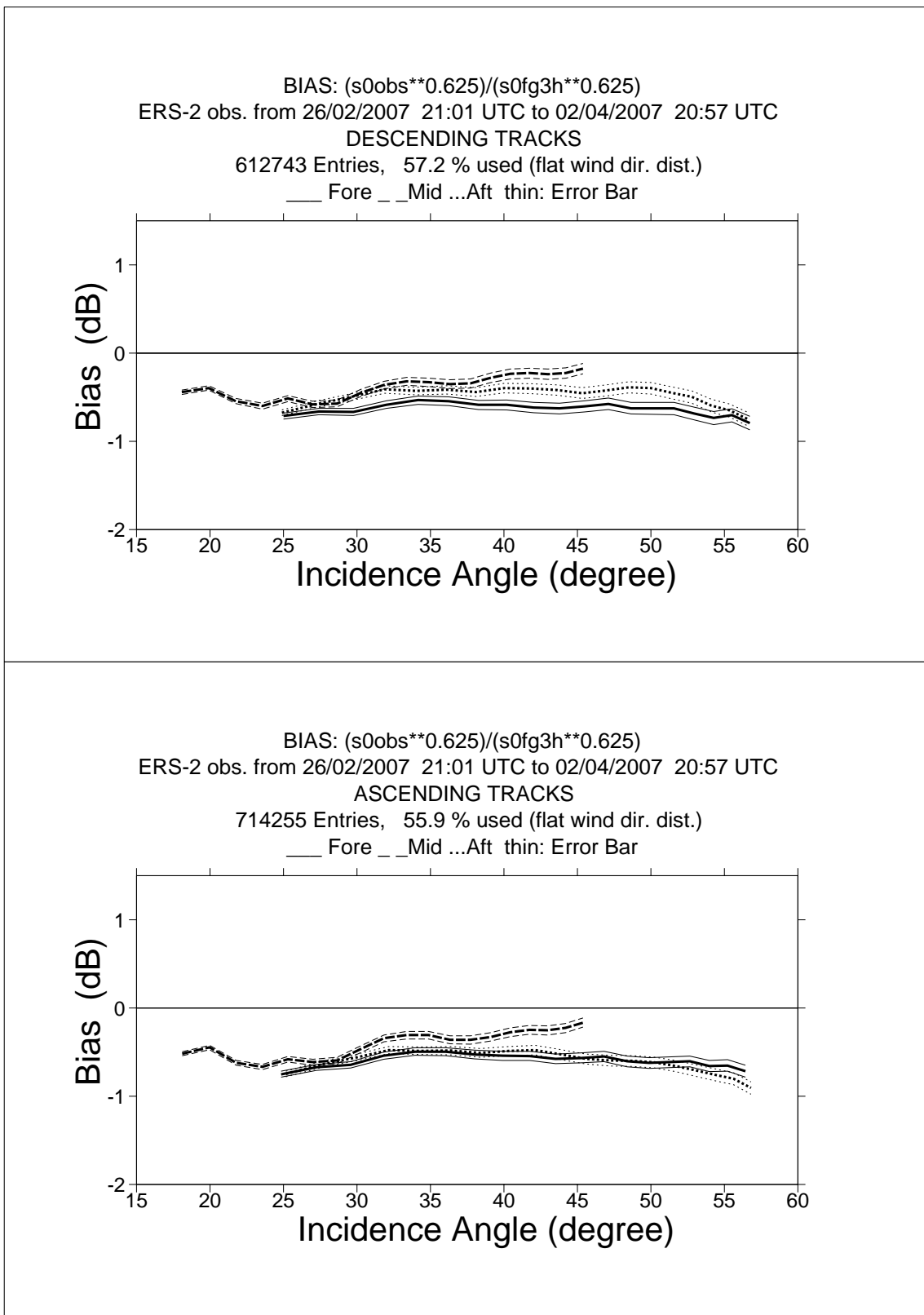
FIGURE 1 ERS-2 Scatterometer Ocean Calibration cycle 124. Ratio of \langle \sigma_0^{0.625} \rangle / \langle CMOD4(\text{First Guess})^{0.625} \rangle converted in dB for the fore beam (solid line), mid beam (dashed line) an aft beam (dotted line), as a function of incidence angle for descending and ascending tracks. The thin lines indicate the error bars on the estimated mean. First-guess winds are based on the in time closest (+3h, +6h, +9h, or +12h) T511 forecast field, and are bilinearly interpolated in space.
