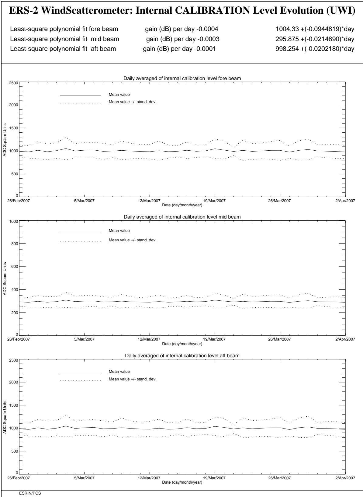
FIGURE 7 ERS-2 Scatterometer: power of internal calibration level cycle 124.
