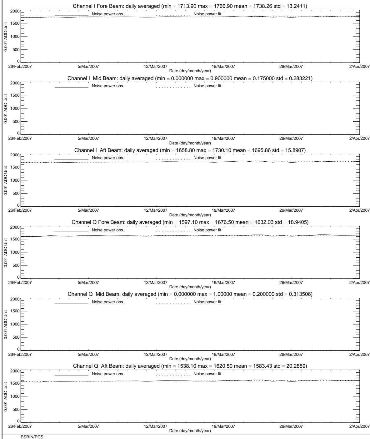
FIGURE 5 ERS-2 Scatterometer: noise power I and Q channel for cycle 124.
