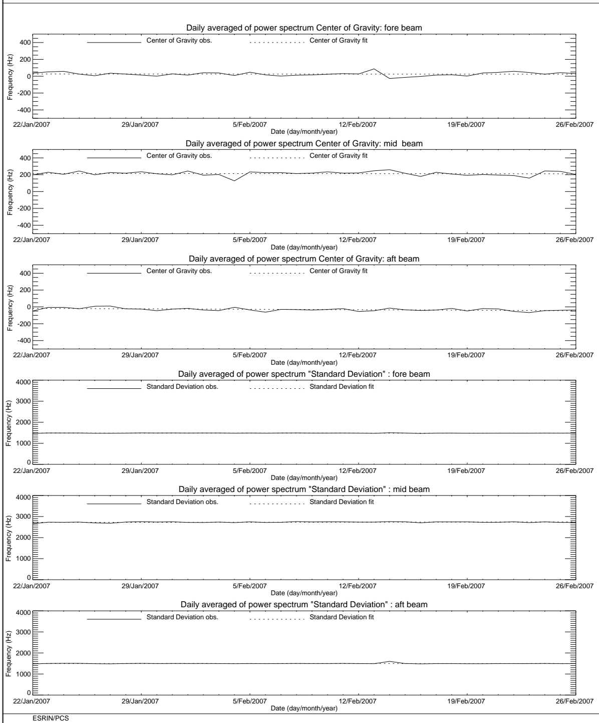
FIGURE 3 ERS-2 Scatterometer: Centre of Gravity and standard deviation of received power spectrum for cycle 123.
