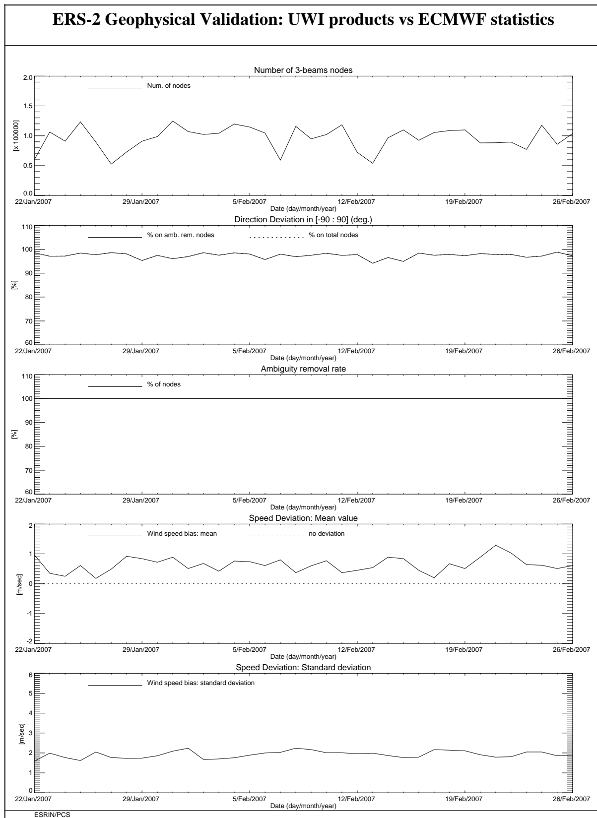
FIGURE 10 ERS-2 Scatterometer: wind products performance for cycle 123.
