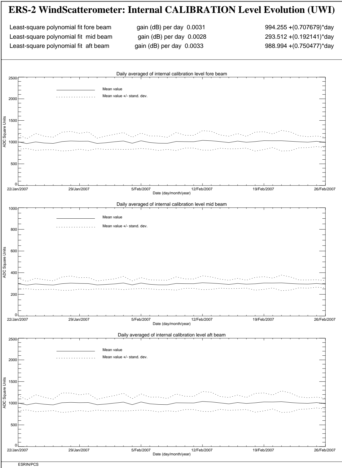
FIGURE 7 ERS-2 Scatterometer: power of internal calibration level cycle 123.
