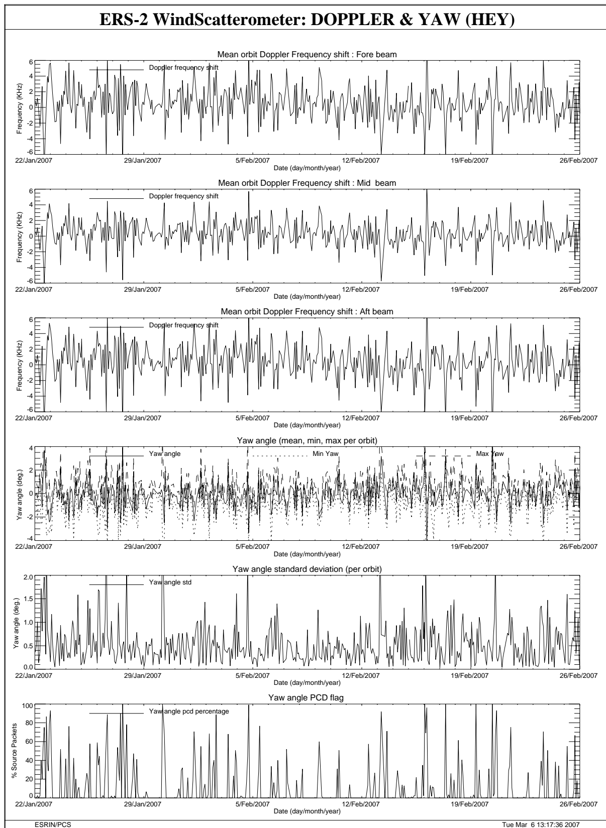
FIGURE 27 Doppler frequency shift and Yaw error angle evolution cycle 123.
