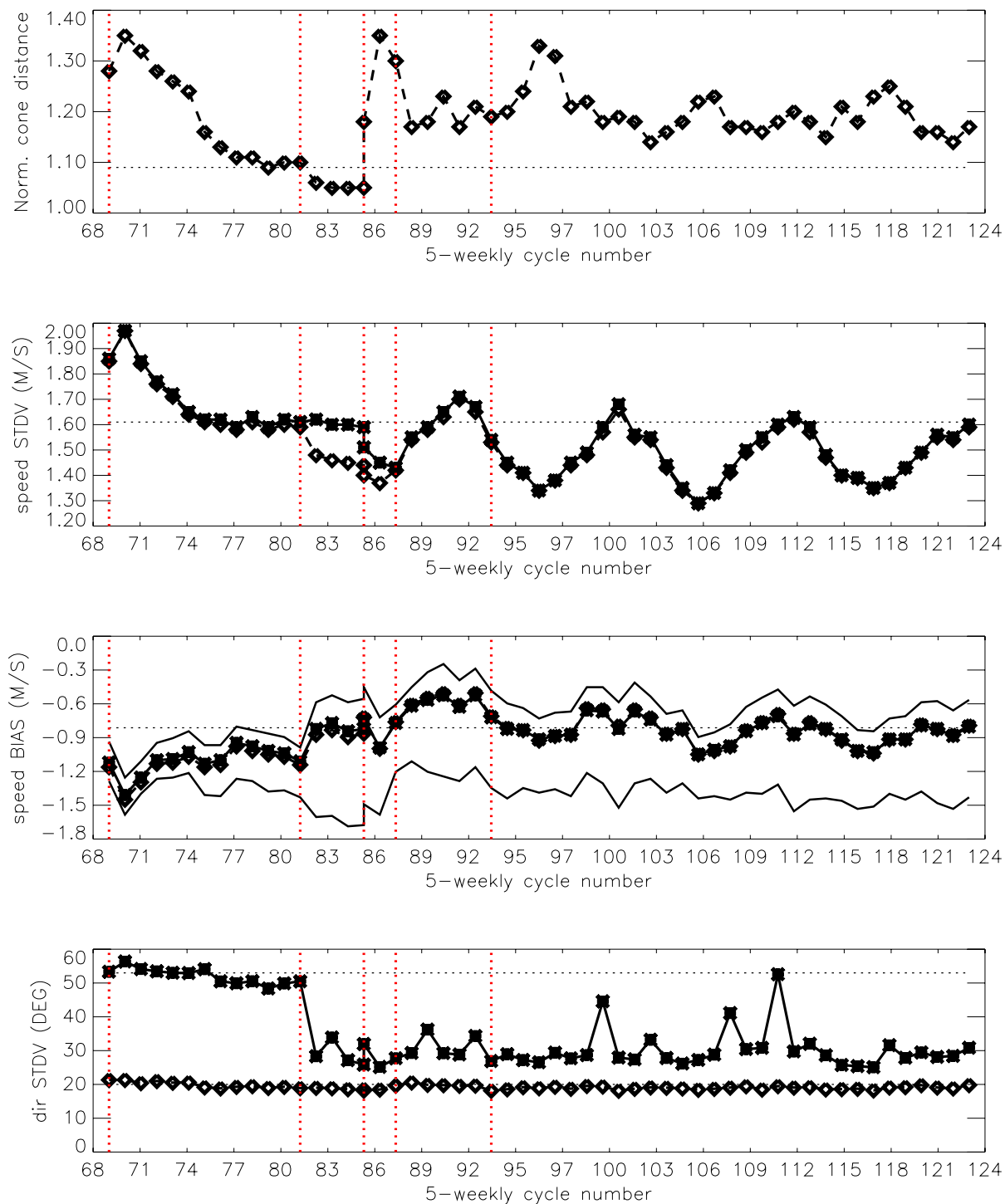
FIGURE 11 Evolution of the performance of the ERS-2 Scatterometer averaged over 5-weekly cycles from 12 December 2001 (cycle 69) to 26 February 2007 (end cycle 123) for the UWI product (solid, star) and de-aliased winds based on CMOD4(dashed, diamond). Results are based on data that passed the UWI QC flags. For cycle 85 two values are plotted; the first value for the global set, the second one for the regional set. Dotted lines represent values for cycle 59 (5 December 2000 to 17 January 2001),i.e. the last stable cycle of the nominal period. From top to bottom panel are shown the normalized distance to the one (CMOD4 only) the standard deviation of the wind speed compared to FG winds, the corresponding bias (for UWI winds the extreme inter-node averages are shown as well),and the standard deviation of wind direction compared to FG.
