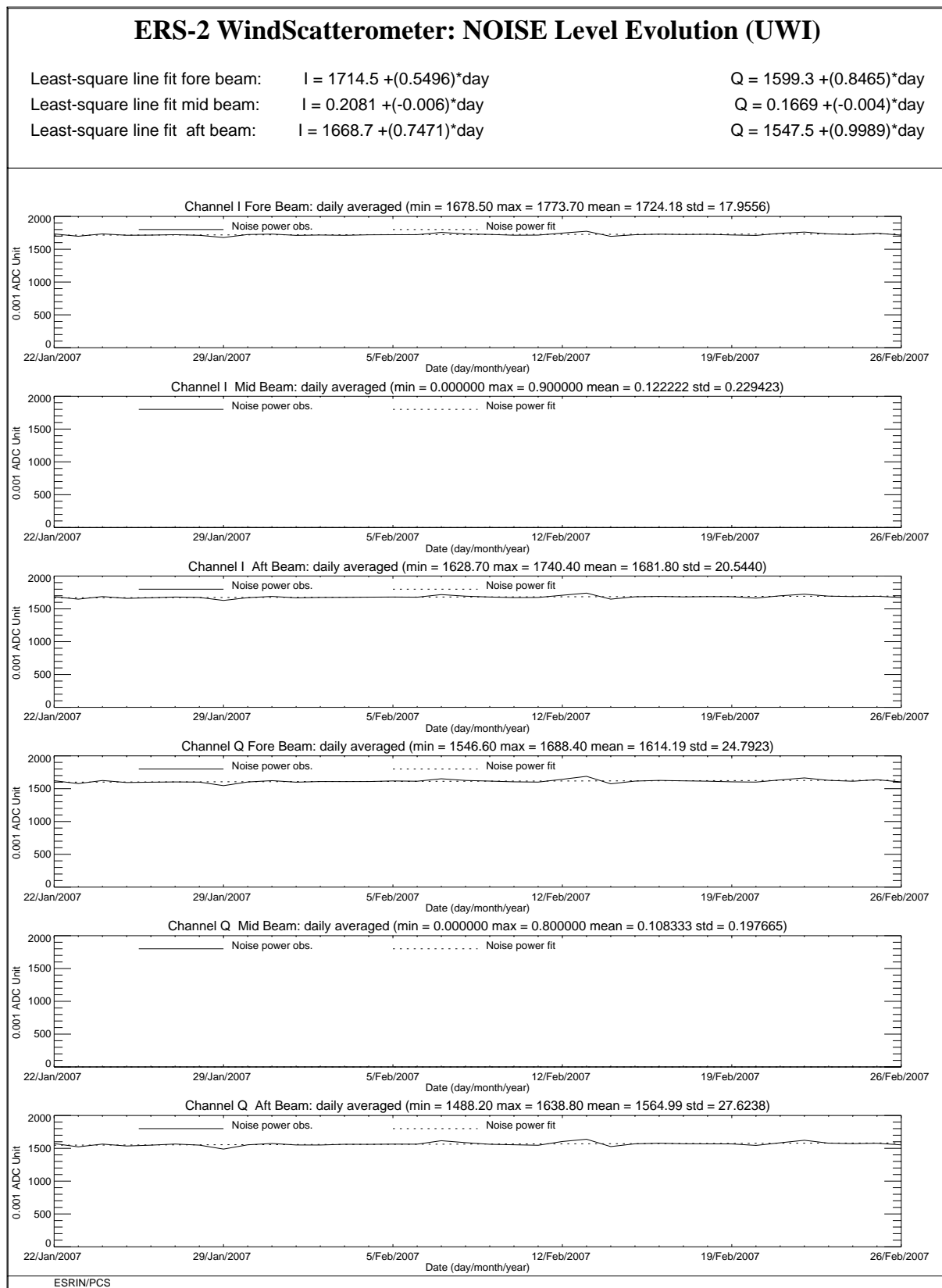
FIGURE 5 ERS-2 Scatterometer: noise power I and Q channel for cycle 123.
