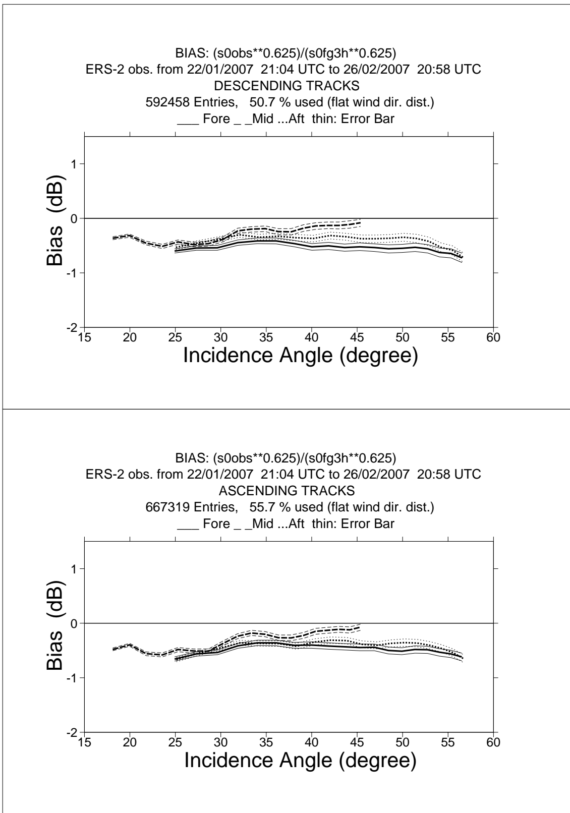
FIGURE 1 ERS-2 Scatterometer Ocean Calibration cycle 123. Ratio of \langle \sigma_0^{0.625} \rangle / \langle CMOD4(First\ Guess)^{0.625} \rangle converted in dB for the fore beam (solid line), mid beam (dashed line) an aft beam (dotted line), as a function of incidence angle for descending and ascending tracks. The thin lines indicate the error bars on the estimated mean. First-guess winds are based on the in time closest (+3h, +6h, +9h, or +12h) T511 forecast field, and are bilinearly interpolated in space.
