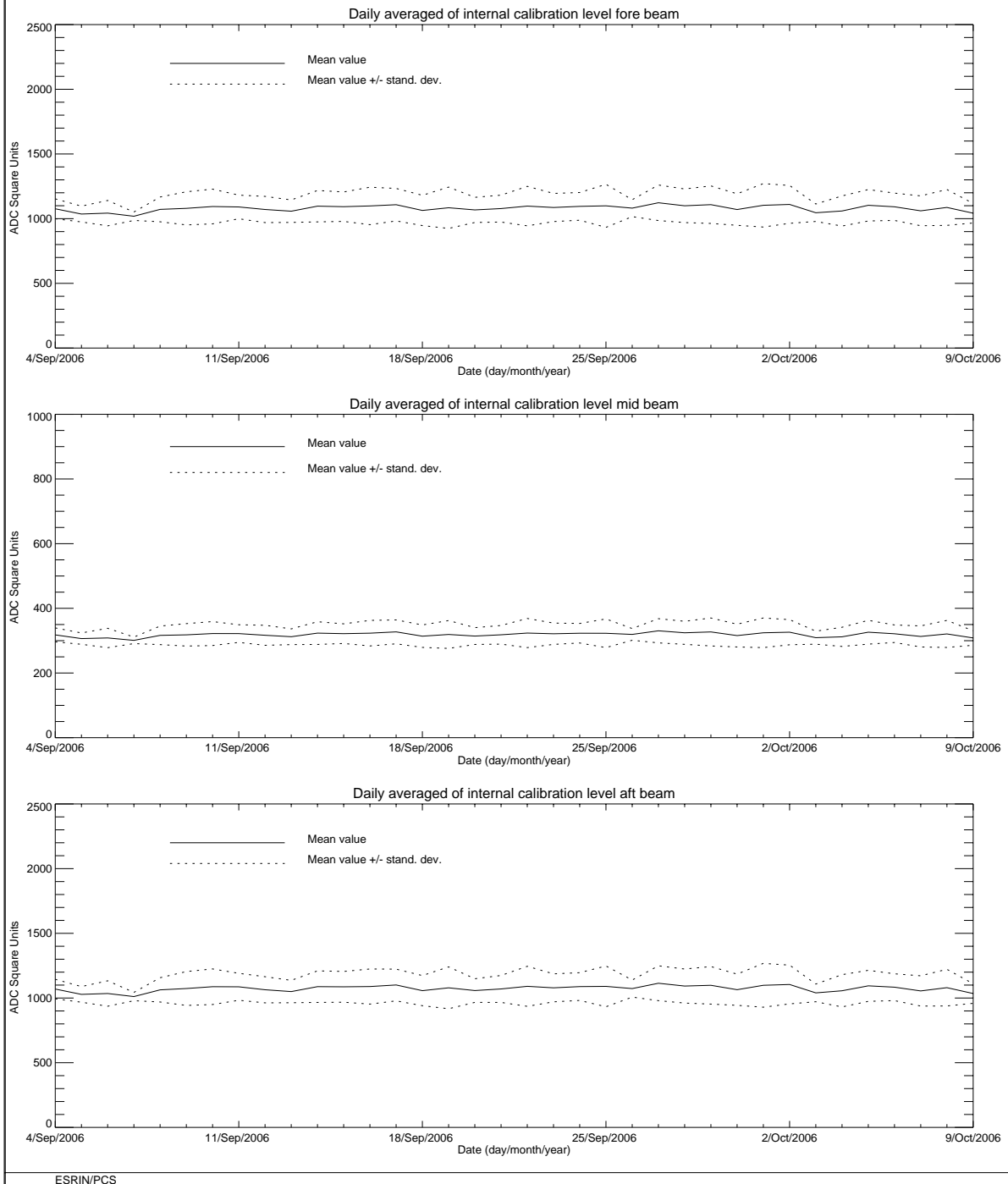
FIGURE 7 ERS-2 Scatterometer: power of internal calibration level cycle 119.
