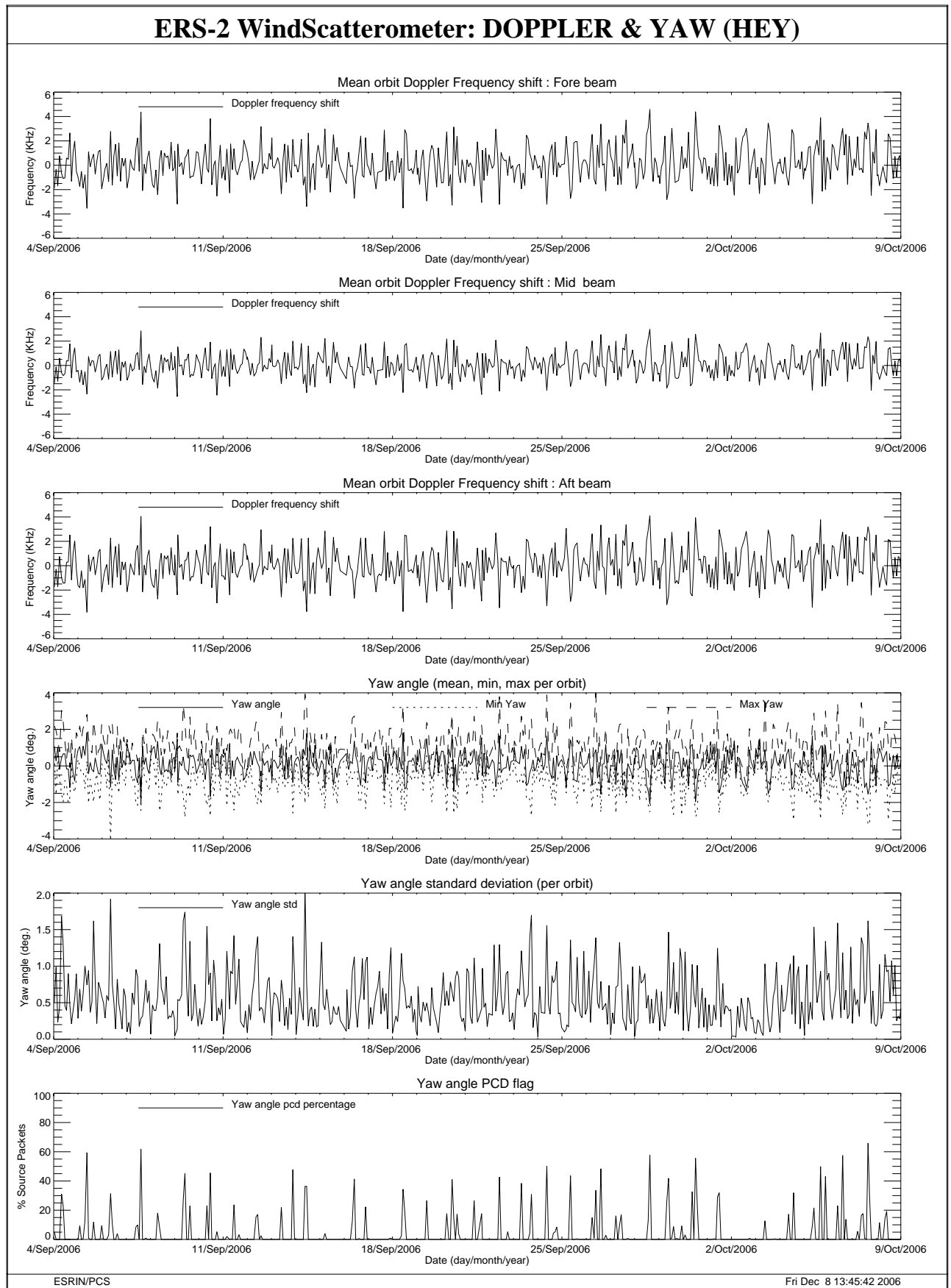
FIGURE 27 Doppler frequency shift and Yaw error angle evolution cycle 119.
