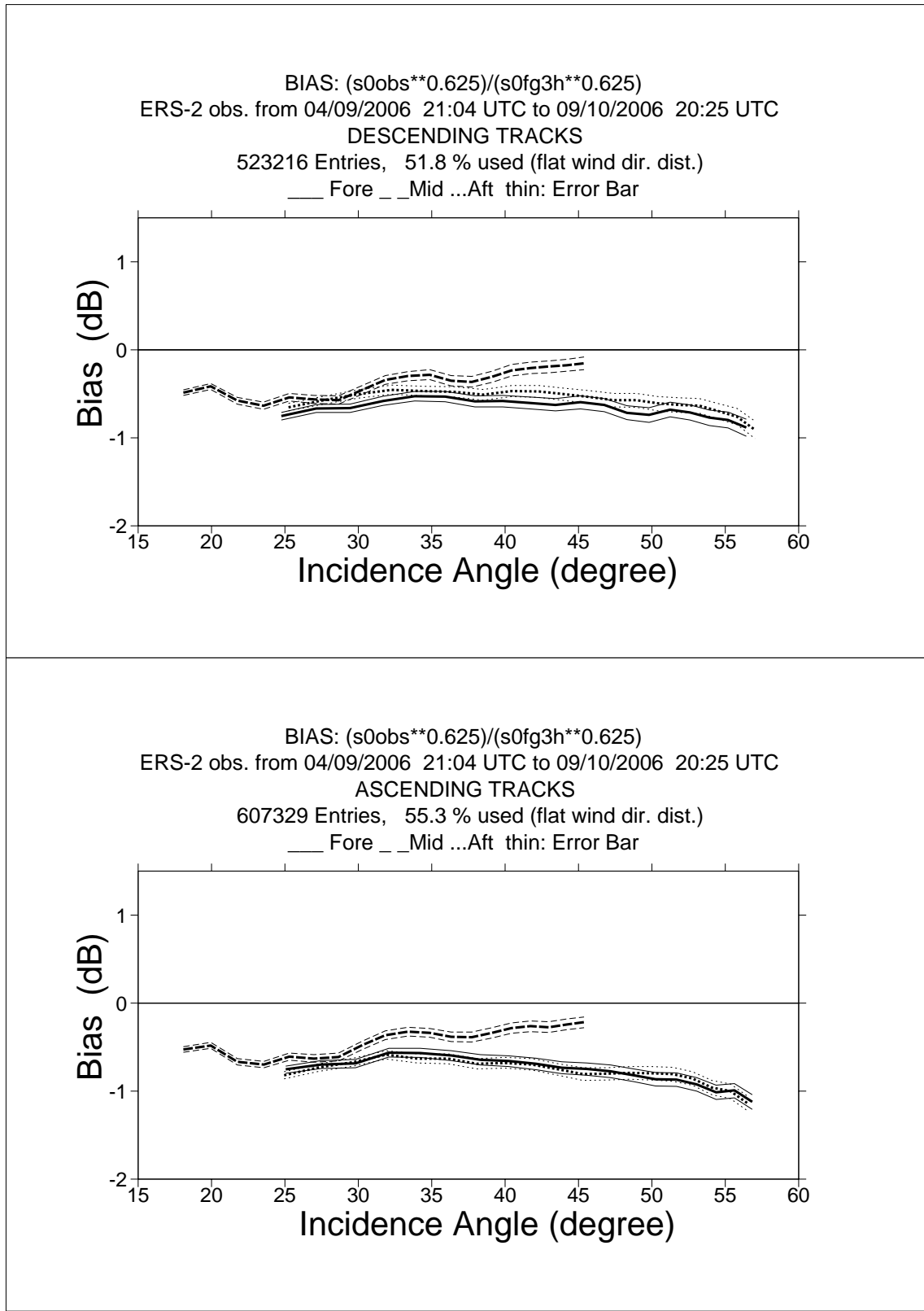
FIGURE 1 ERS-2 Scatterometer Ocean Calibration cycle 119. Ratio of \langle \sigma_0^{0.625} \rangle / \langle C_{MOD4}(\text{First Guess})^{0.625} \rangle converted in dB for the fore beam (solid line), mid beam (dashed line) an aft beam (dotted line), as a function of incidence angle for descending and ascending tracks. The thin lines indicate the error bars on the estimated mean. First-guess winds are based on the in time closest (+3h, +6h, +9h, or +12h) T511 forecast field, and are bilinearly interpolated in space.
