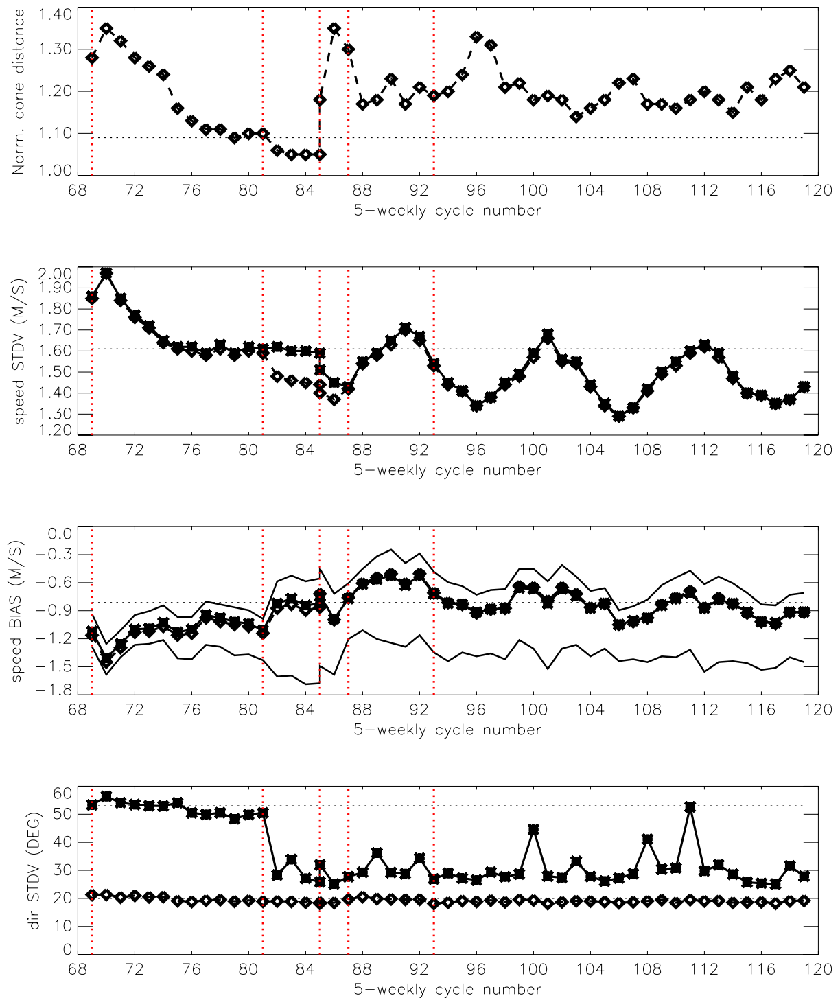
FIGURE 11 Evolution of the performance of the ERS-2 Scatterometer averaged over 5-weekly cycles from 12 December 2001 (cycle 69) to 9 October 2006 (end cycle 119) for the UWI product (solid, star) and de-aliased winds based on CMOD4 (dashed, diamond). Results are based on data that passed the UWI QC flags. For cycle 85 two values are plotted; the first value for the global set, the second one for the regional set. Dotted lines represent values for cycle 59 (5 December 2000 to 17 January 2001), i.e. the last stable cycle of the nominal period. From top to bottom panel are shown the normalized distance to the one (CMOD4 only) the standard deviation of the wind speed compared to FG winds, the corresponding bias (for UWI winds the extreme inter-node averages are shown as well), and the standard deviation of wind direction compared to FG.
