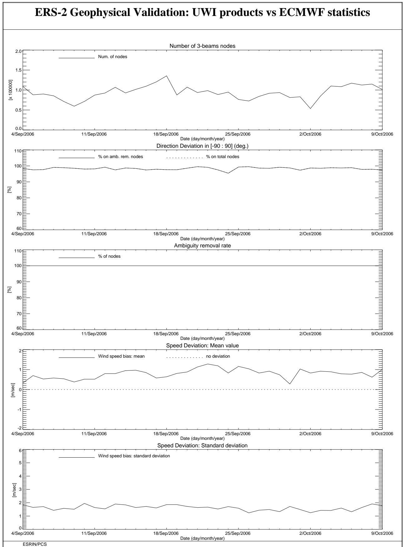
FIGURE 10 ERS-2 Scatterometer: wind products performance for cycle 119.
