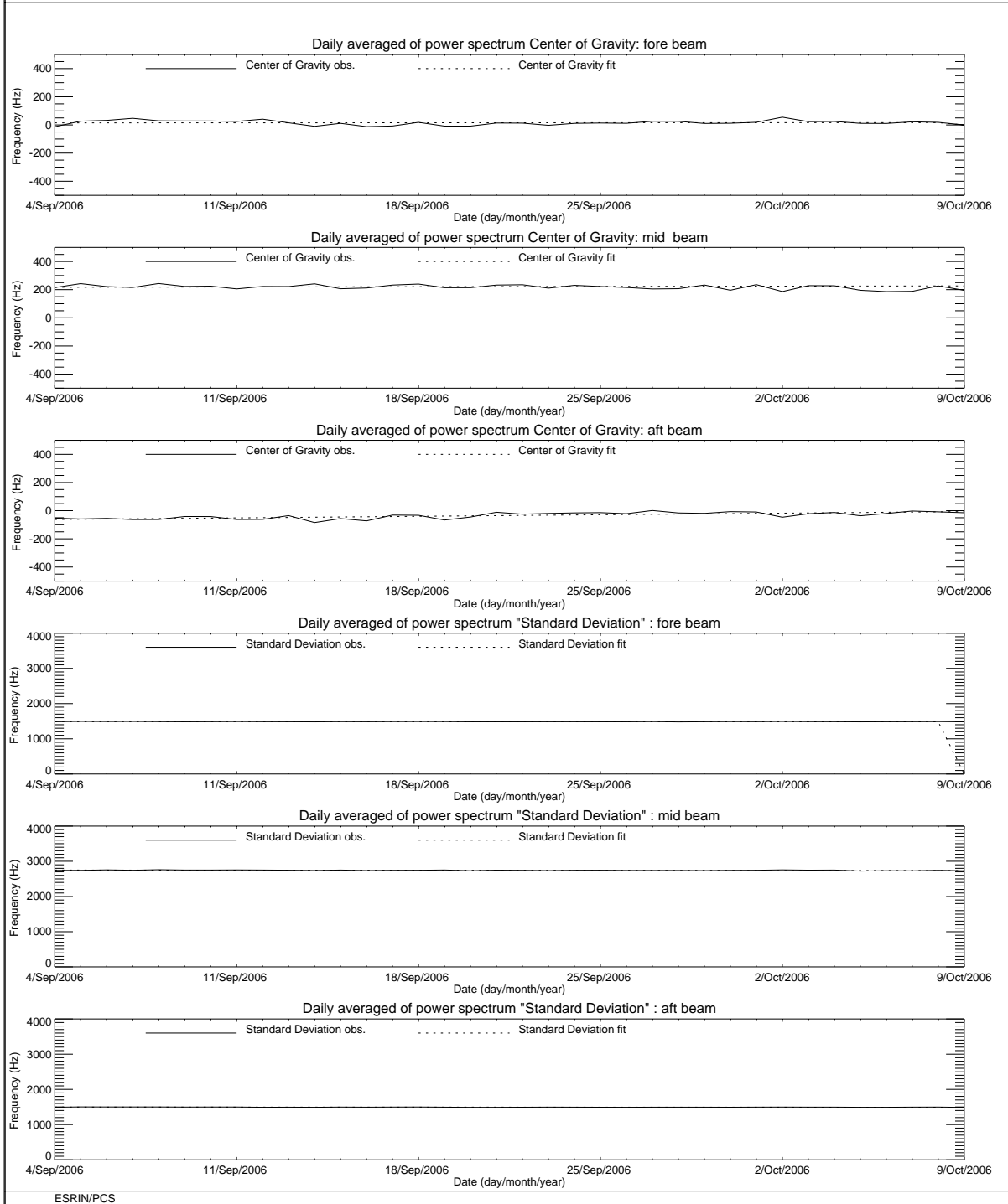
FIGURE 3 ERS-2 Scatterometer: Centre of Gravity and standard deviation of received power spectrum during the cycle 119.
