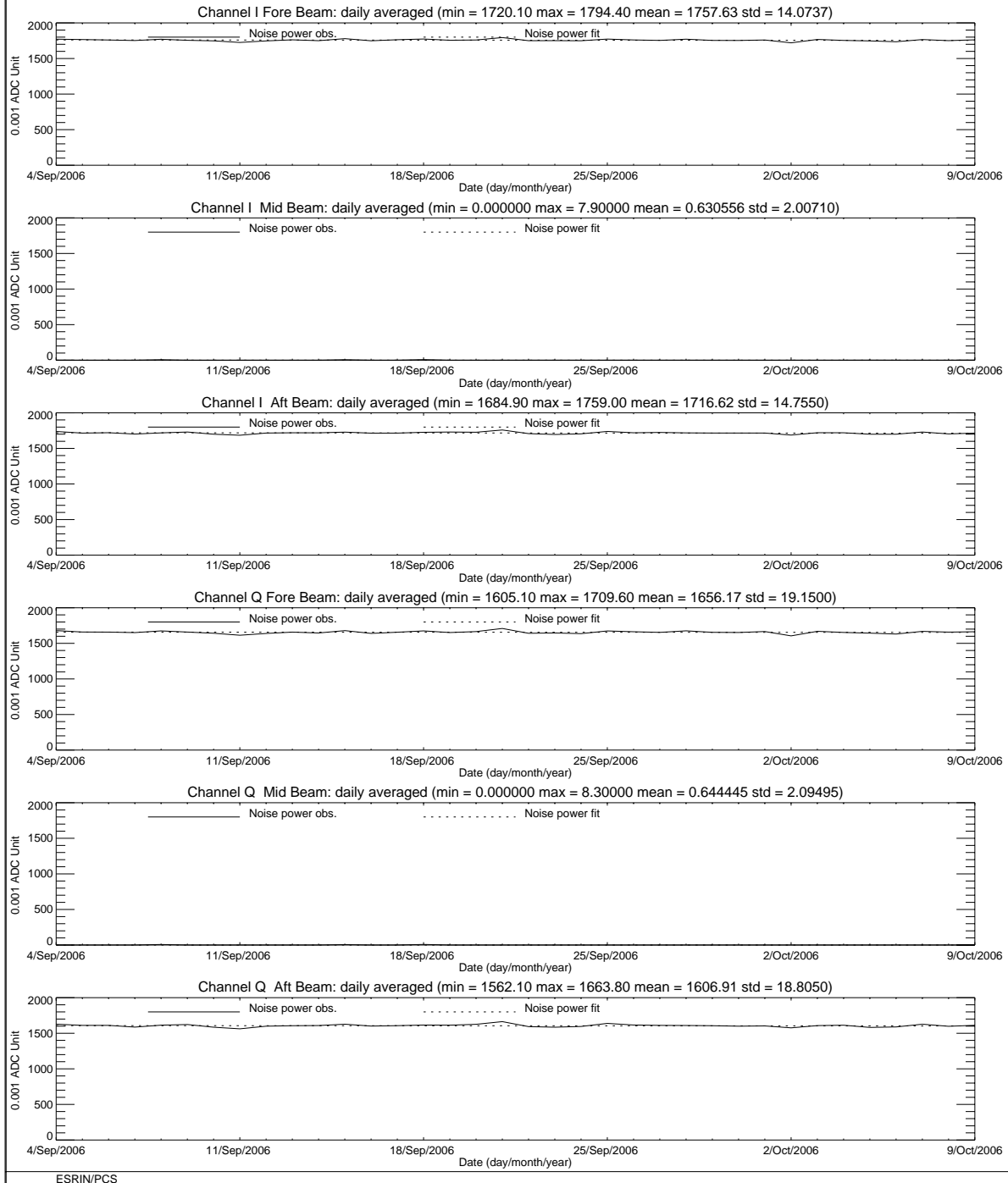
FIGURE 5 ERS-2 Scatterometer: noise power I and Q channel for cycle 119.
