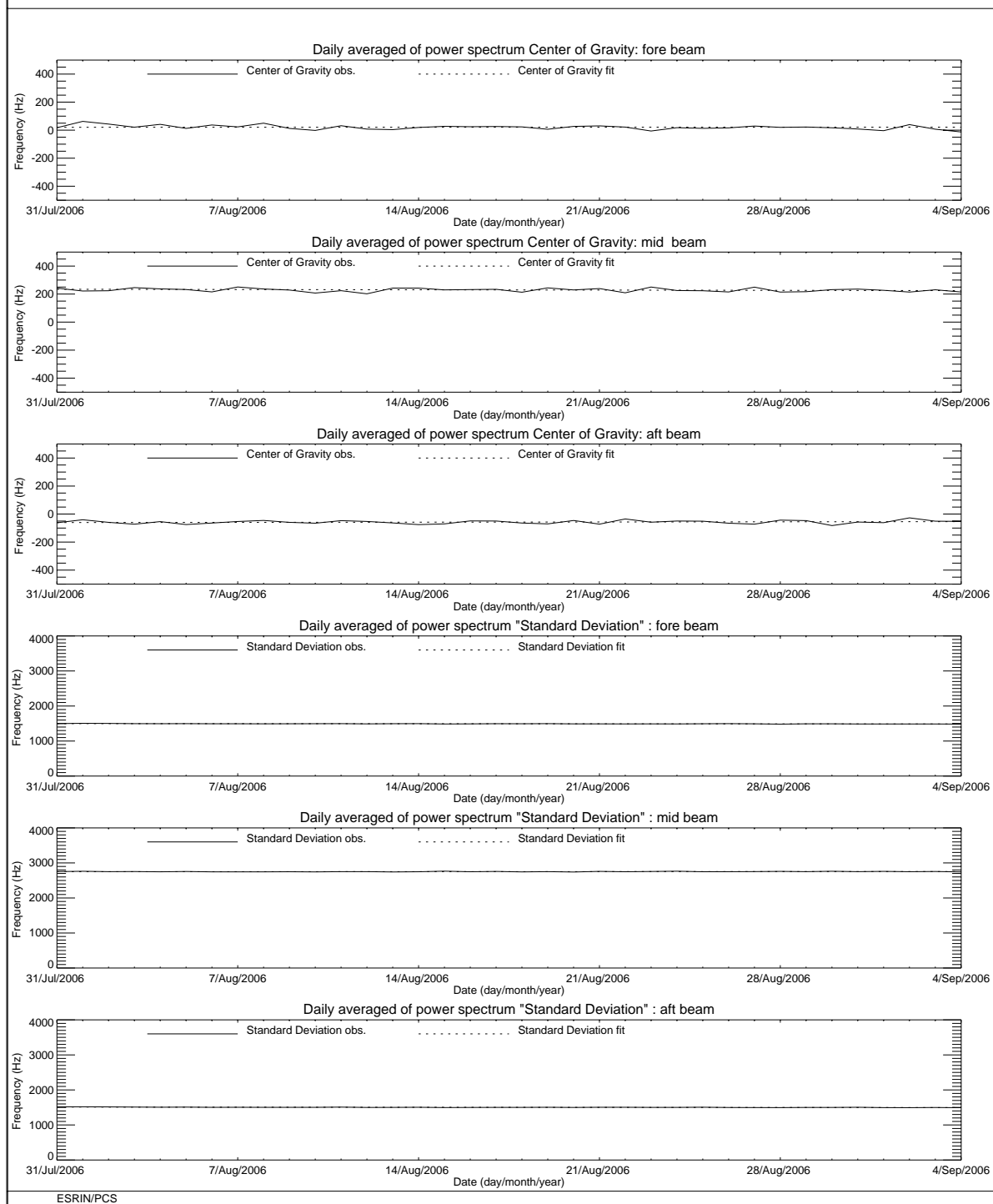
FIGURE 3 ERS-2 Scatterometer: Centre of Gravity and standard deviation of received power spectrum during the cycle 118.
