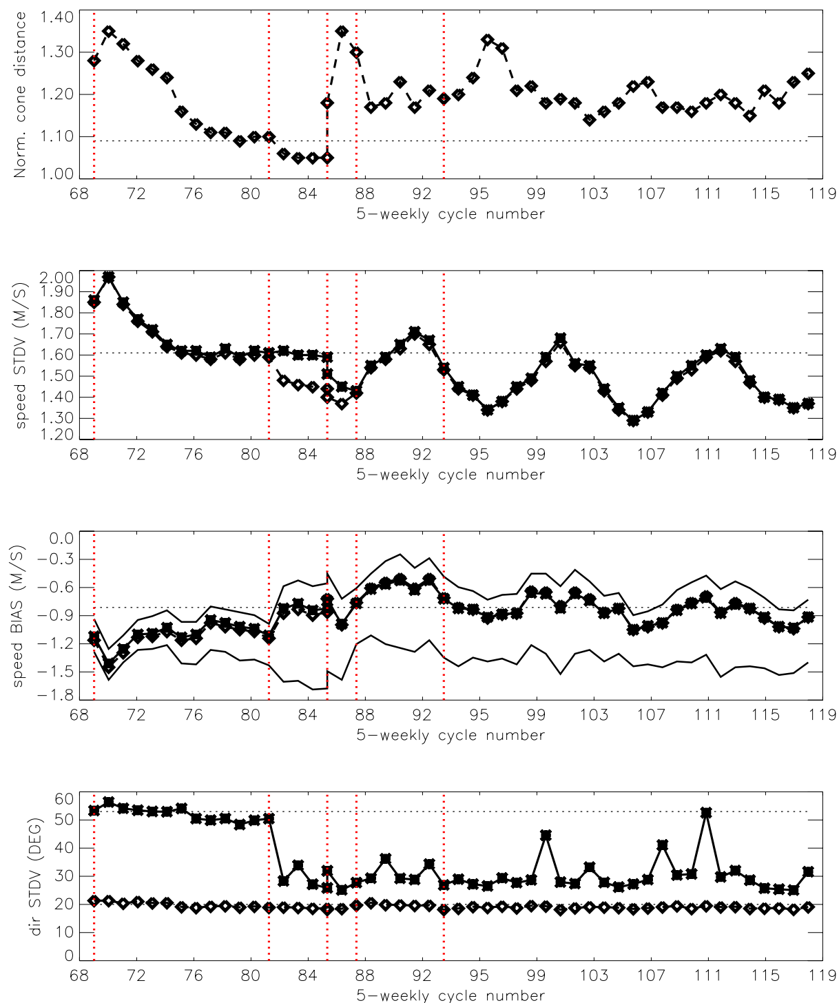
FIGURE 11 Evolution of the performance of the ERS-2 Scatterometer averaged over 5-weekly cycles from 12 December 2001 (cycle 69) to 04 September 2006 (end cycle 118) for the UWI product (solid, star) and de-aliased winds based on CMOD4(dashed, diamond). Results are based on data that passed the UWI QC flags. For cycle 85 two values are plotted; the first value for the global set, the second one for the regional set. Dotted lines represent values for cycle 59 (5 December 2000 to 17 January 2001), i.e. the last stable cycle of the nominal period. From top to bottom panel are shown the normalized distance to the one (CMOD4 only) the standard deviation of the wind speed compared to FG winds, the corresponding bias (for UWI winds the extreme inter-node averages are shown as well), and the standard deviation of wind direction compared to FG.
