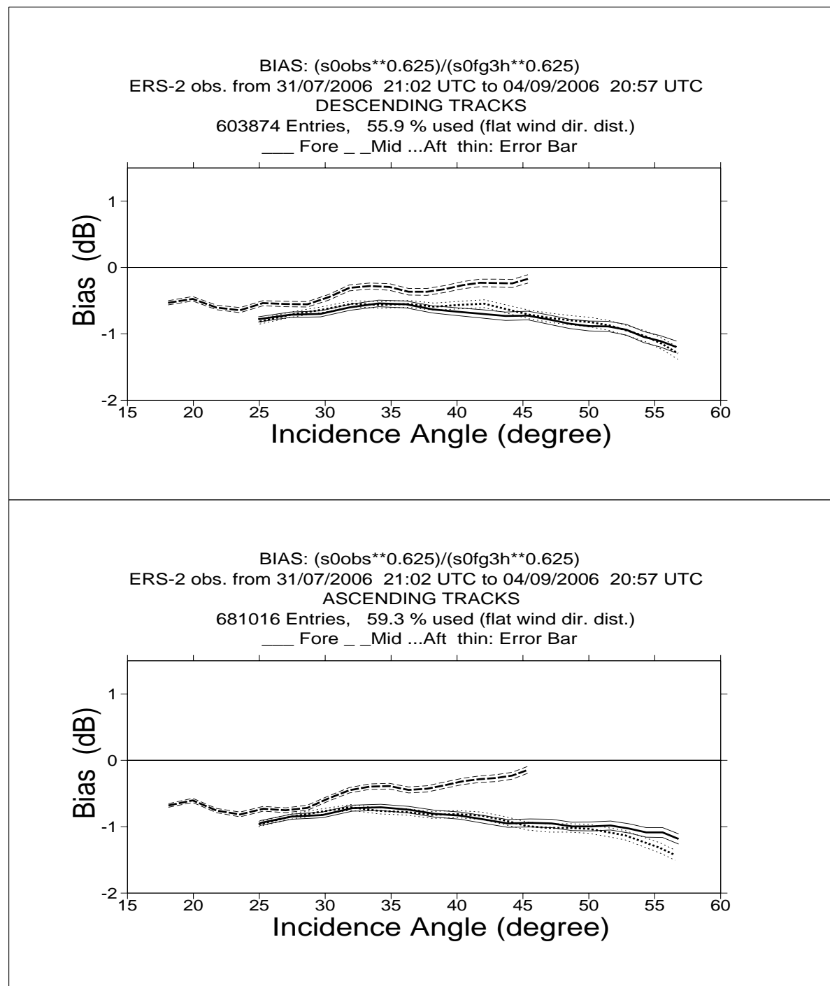
FIGURE 1 ERS-2 Scatterometer Ocean Calibration cycle 118. Ratio of \langle \sigma_0^{0.625} \rangle / \langle CMOD4(First\ Guess)^{0.625} \rangle converted in dB for the fore beam (solid line), mid beam (dashed line) and aft beam (dotted line), as a function of incidence angle for descending and ascending tracks. The thin lines indicate the error bars on the estimated mean. First-guess winds are based on the in time closest (+3h, +6h, +9h, or +12h) T511 forecast field, and are bilinear interpolated in space.
