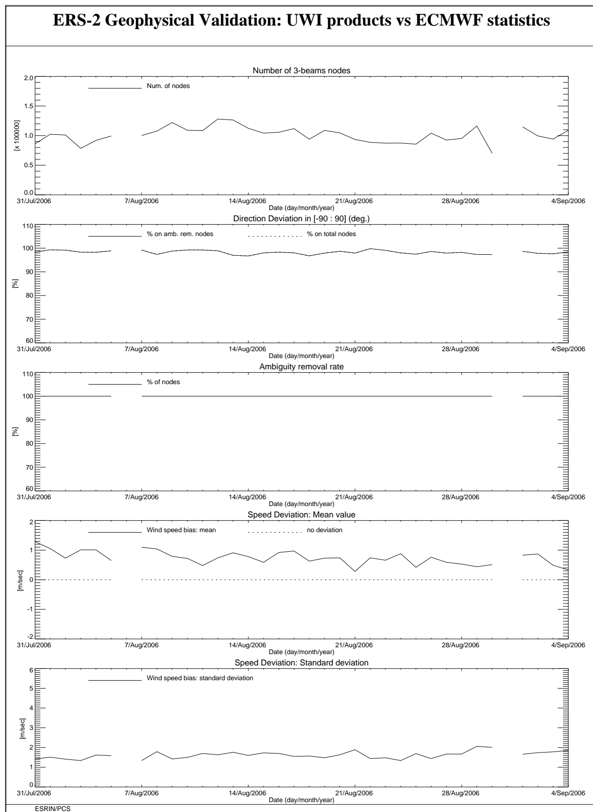
FIGURE 10 ERS-2 Scatterometer: wind products performance for cycle 118.
