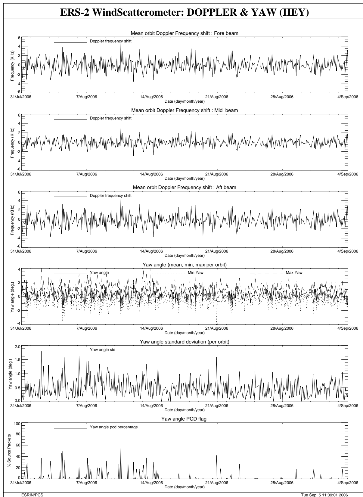
FIGURE 27 Doppler frequency shift and Yaw error angle evolution cycle 118.
