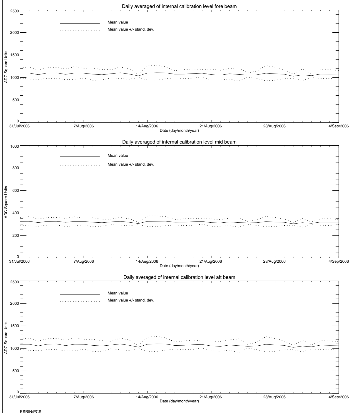
FIGURE 7 ERS-2 Scatterometer: power of internal calibration level cycle 118.
