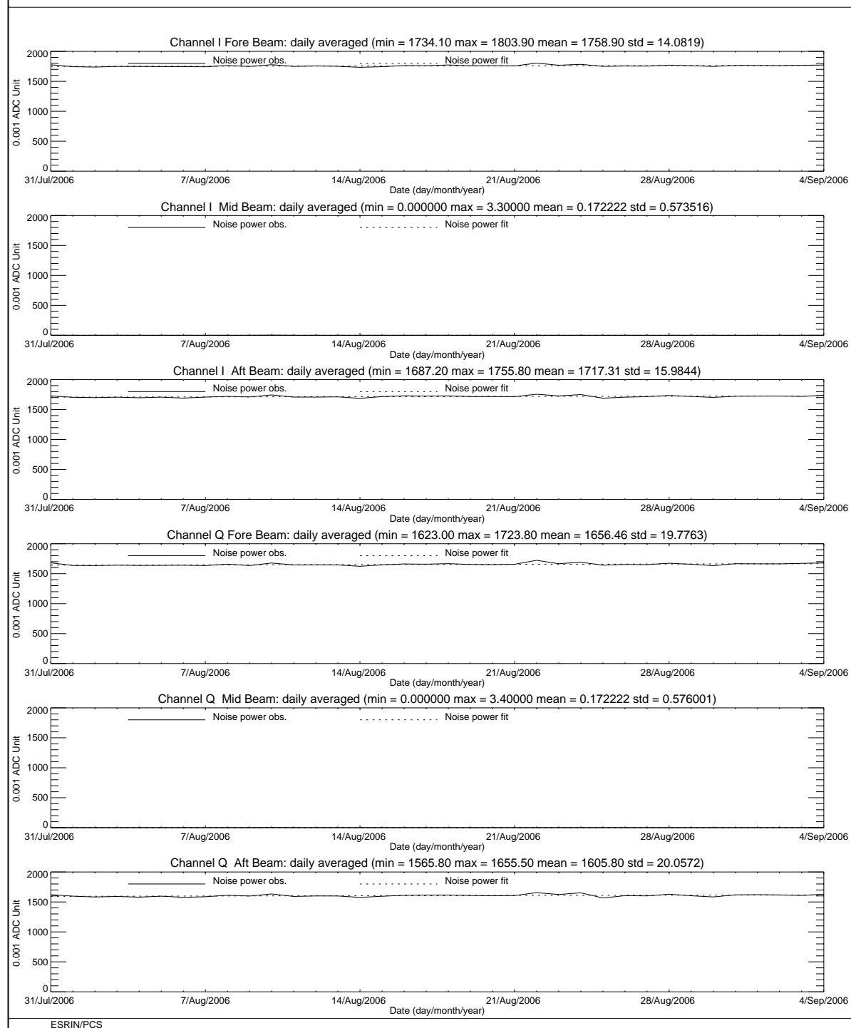
FIGURE 5 ERS-2 Scatterometer: noise power I and Q channel for cycle 118.
