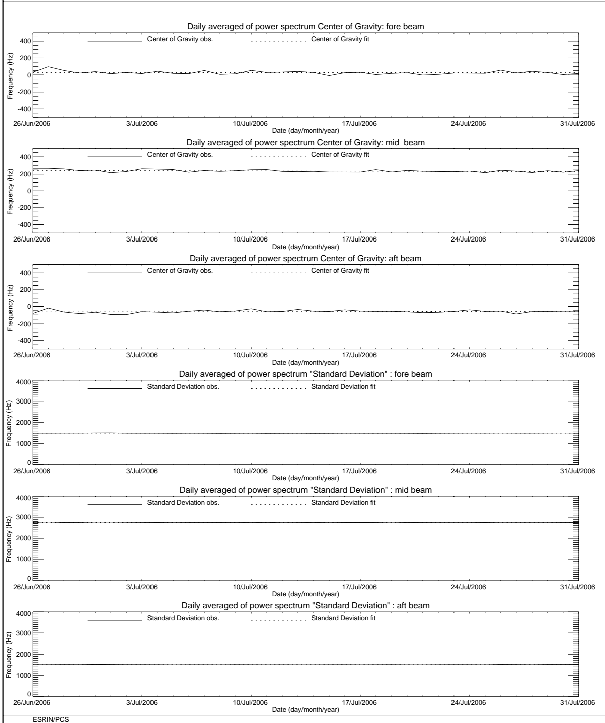
FIGURE 3 ERS-2 Scatterometer: Centre of Gravity and standard deviation of received power spectrum during the cycle 117.
