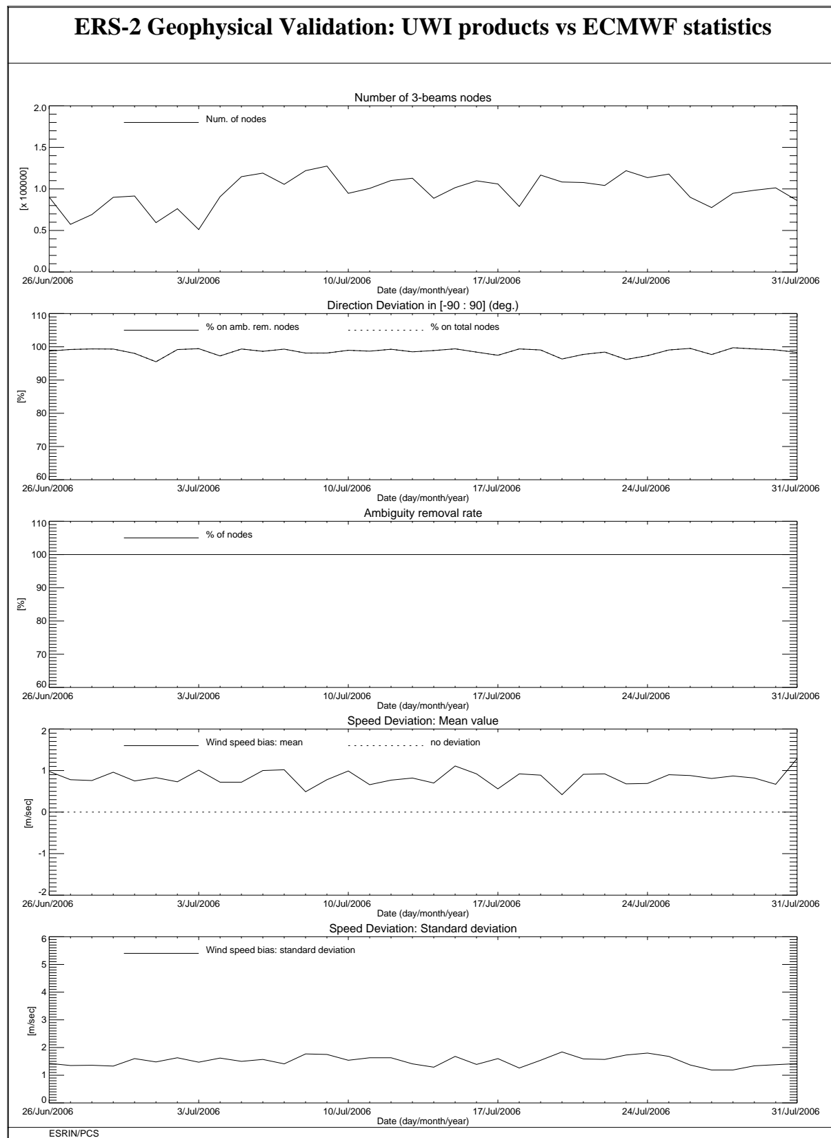
FIGURE 10 ERS-2 Scatterometer: wind products performance for cycle 117.
