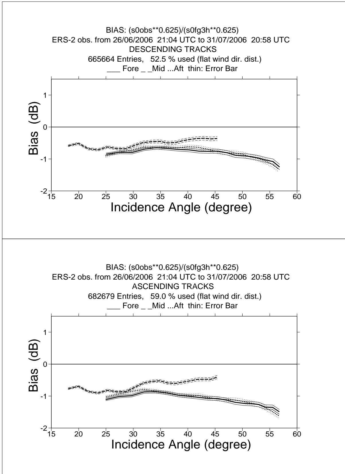
FIGURE 1 ERS-2 Scatterometer Ocean Calibration cycle 117. Ratio of \langle \sigma_0^{0.625} \rangle / \langle \text{CMOD4}(\text{First Guess})^{0.625} \rangle converted in dB for the fore beam (solid line), mid beam (dashed line) an aft beam (dotted line), as a function of incidence angle for descending and ascending tracks. The thin lines indicate the error bars on the estimated mean. First-guess winds are based on the in time closest (+3h, +6h, +9h, or +12h) T511 forecast field, and are bilinear interpolated in space.
