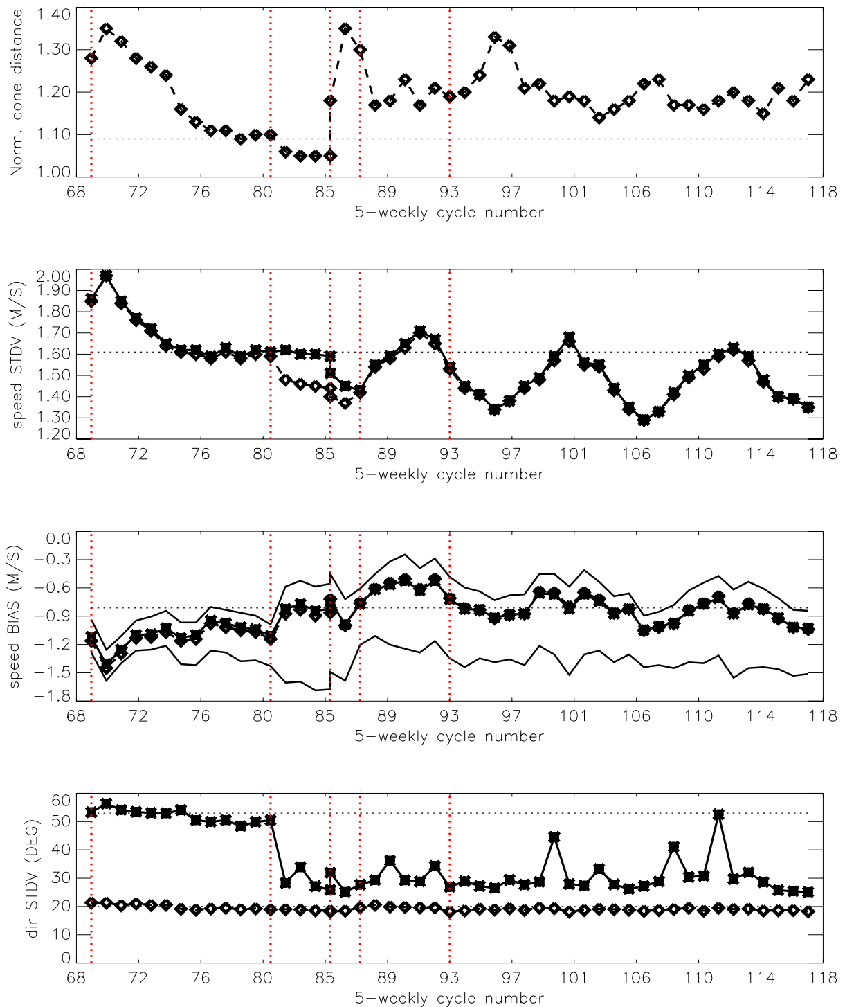
FIGURE 11 Evolution of the performance of the ERS-2 Scatterometer averaged over 5-weekly cycles from 12 December 2001 (cycle 69) to 31 July 2006 (end cycle 117) for the UWI product (solid, star) and de-aliased winds based on CMOD4(dashed, diamond). Results are based on data that passed the UWI QC flags. For cycle 85 two values are plotted; the first value for the global set, the second one for the regional set. Dotted lines represent values for cycle 59 (5 December 2000 to 17 January 2001),i.e. the last stable cycle of the nominal period. From top to bottom panel are shown the normalized distance to the one (CMOD4 only) the standard deviation of the wind speed compared to FG winds, the corresponding bias(for UWI winds the extreme inter-node averages are shown as well),and the standard deviation of wind direction compared to FG.
