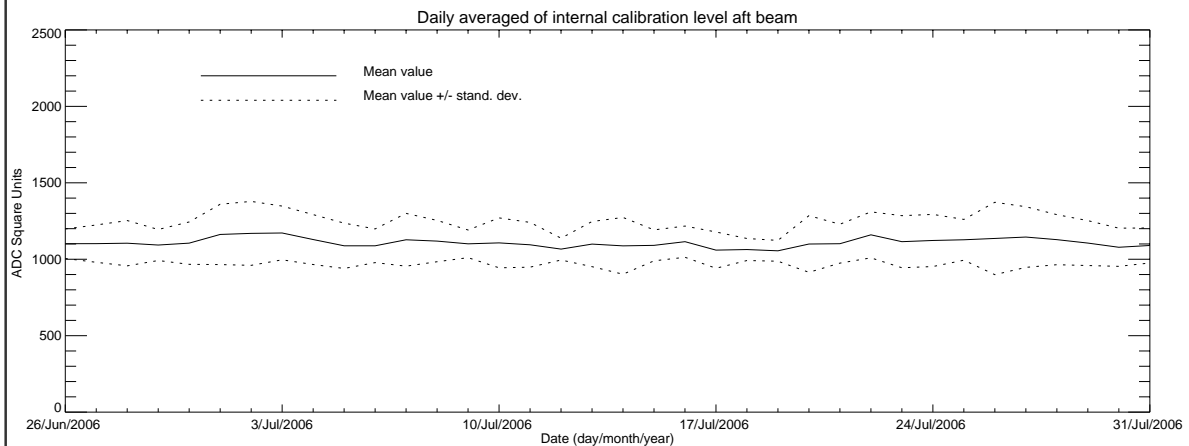
FIGURE 7 ERS-2 Scatterometer: power of internal calibration level cycle 117.
