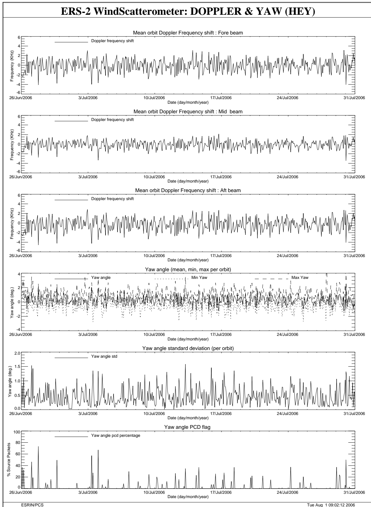
FIGURE 27 Doppler frequency shift and Yaw error angle evolution cycle 117.
