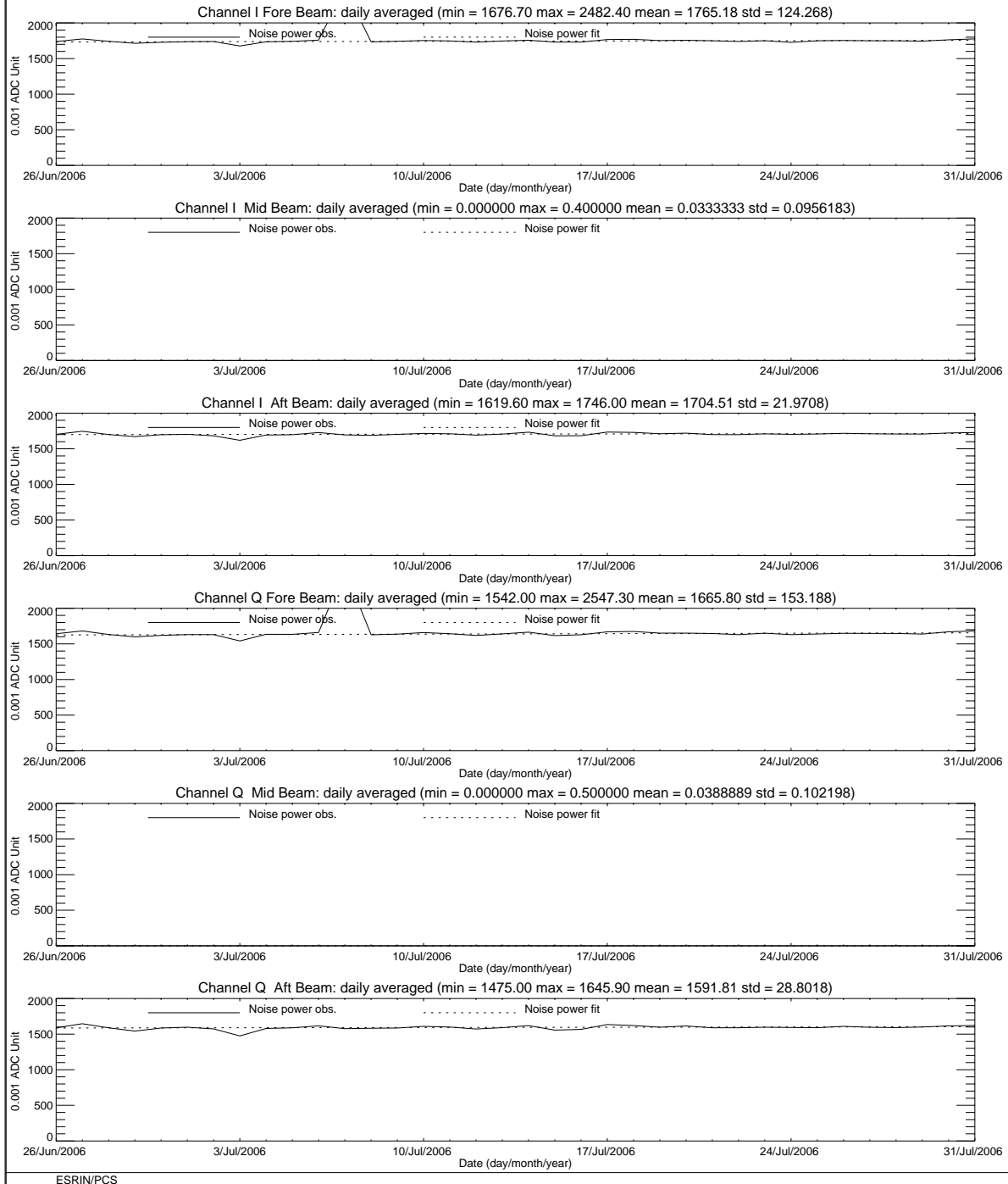
FIGURE 5 ERS-2 Scatterometer: noise power I and Q channel for cycle 117.
