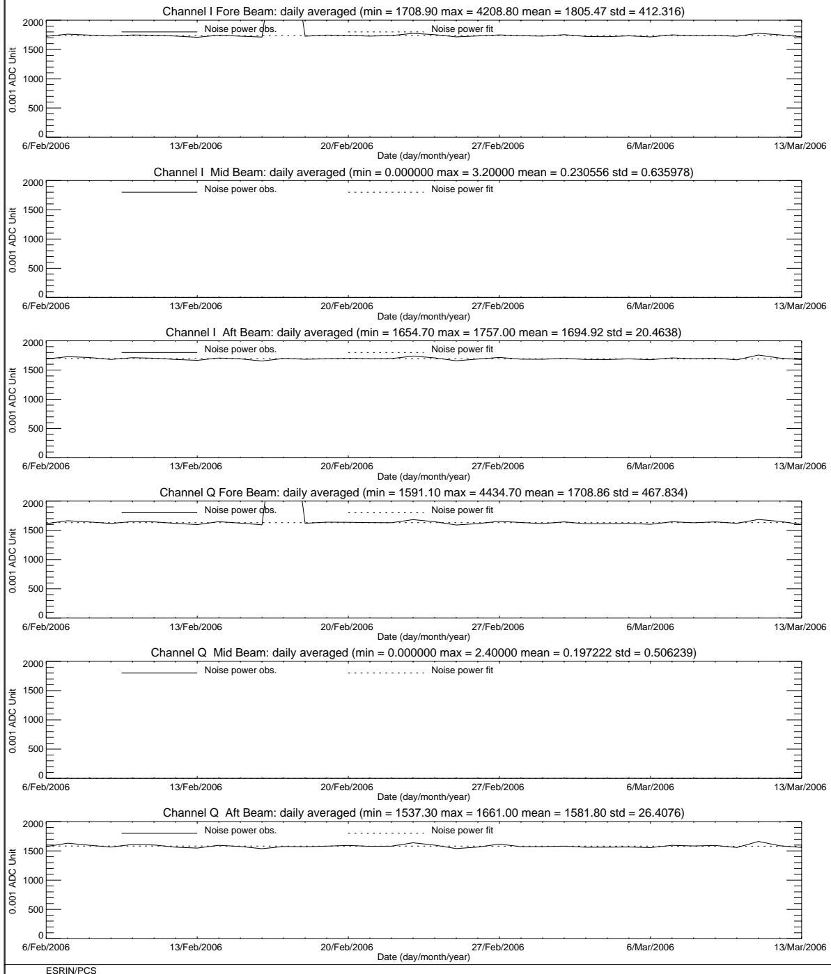
FIGURE 5 ERS-2 Scatterometer: noise power I and Q channel for cycle 113.
