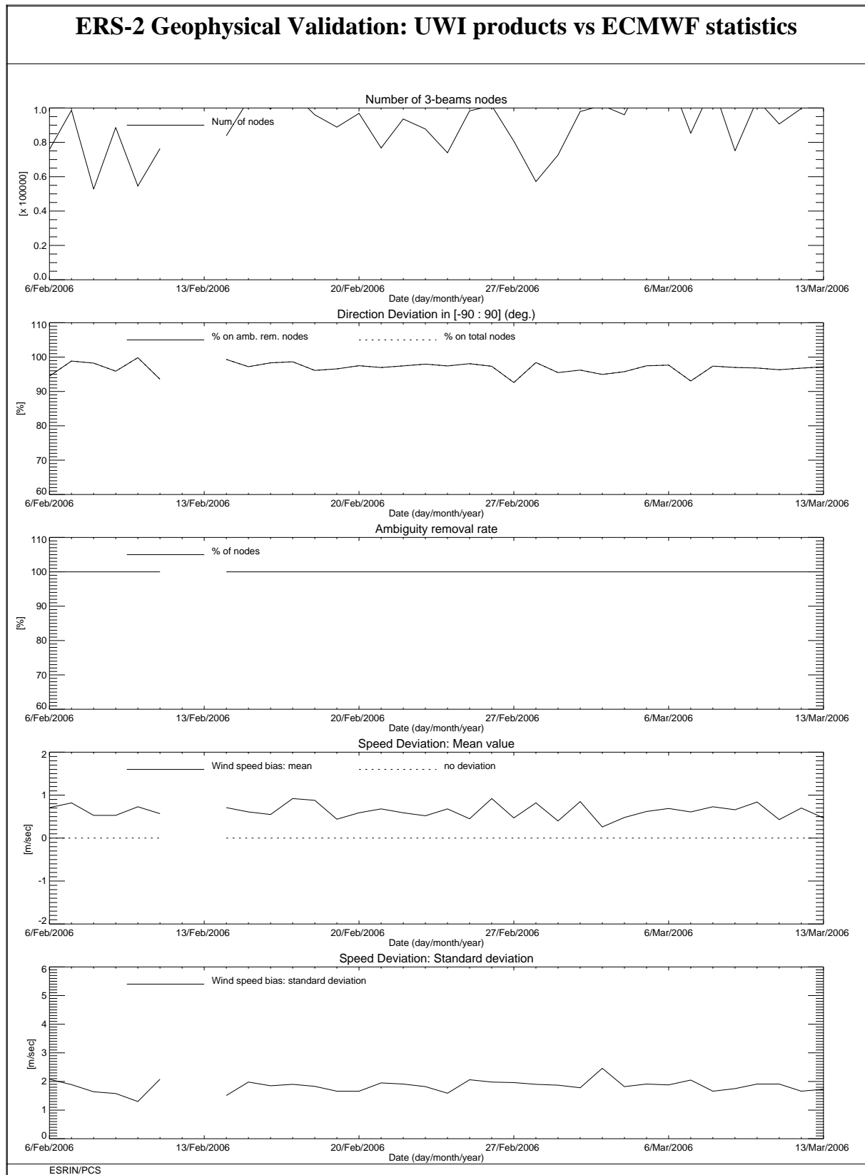
FIGURE 10 ERS-2 Scatterometer: wind products performance for cycle 113.
