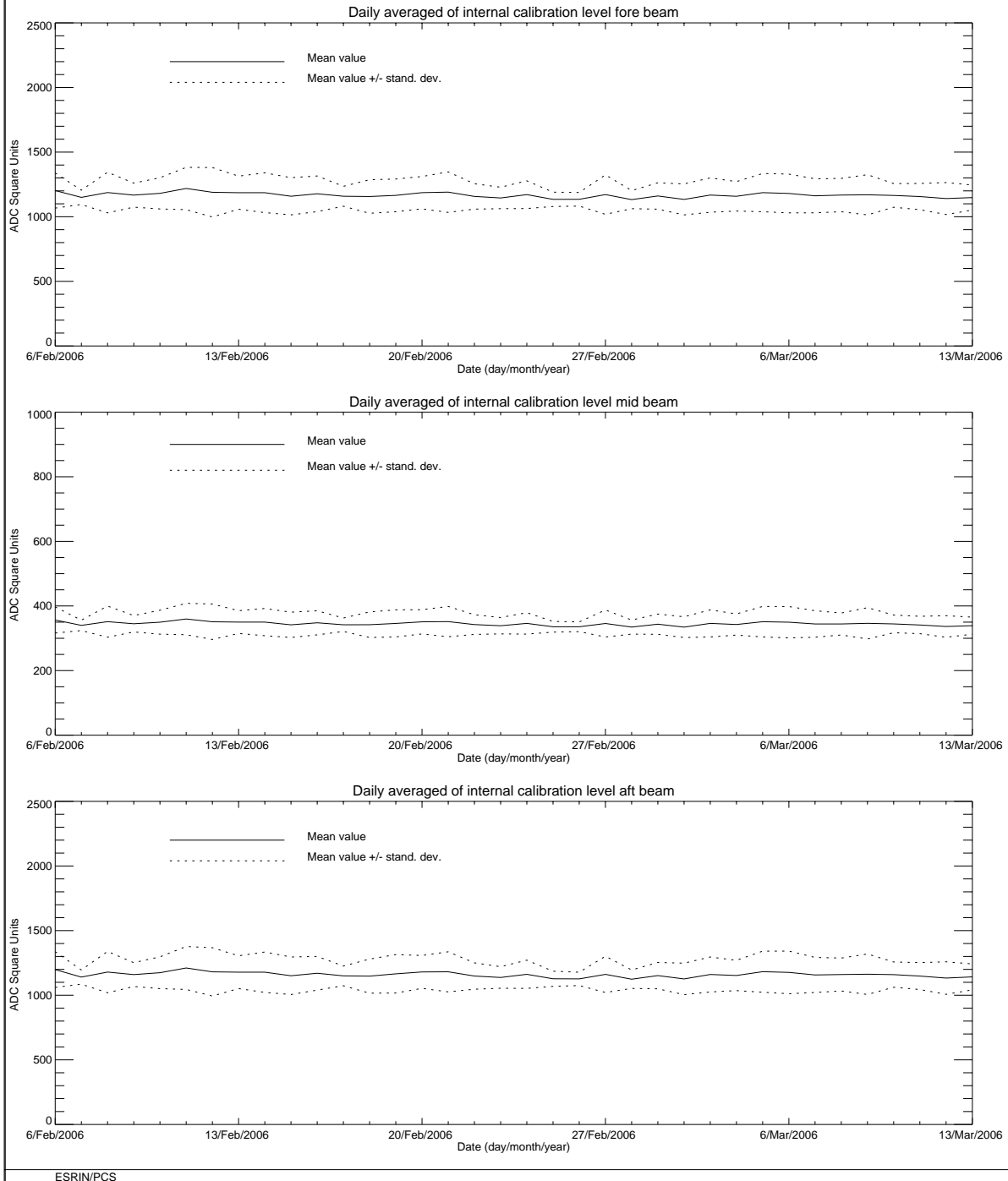
FIGURE 7 ERS-2 Scatterometer: power of internal calibration level cycle 113.
