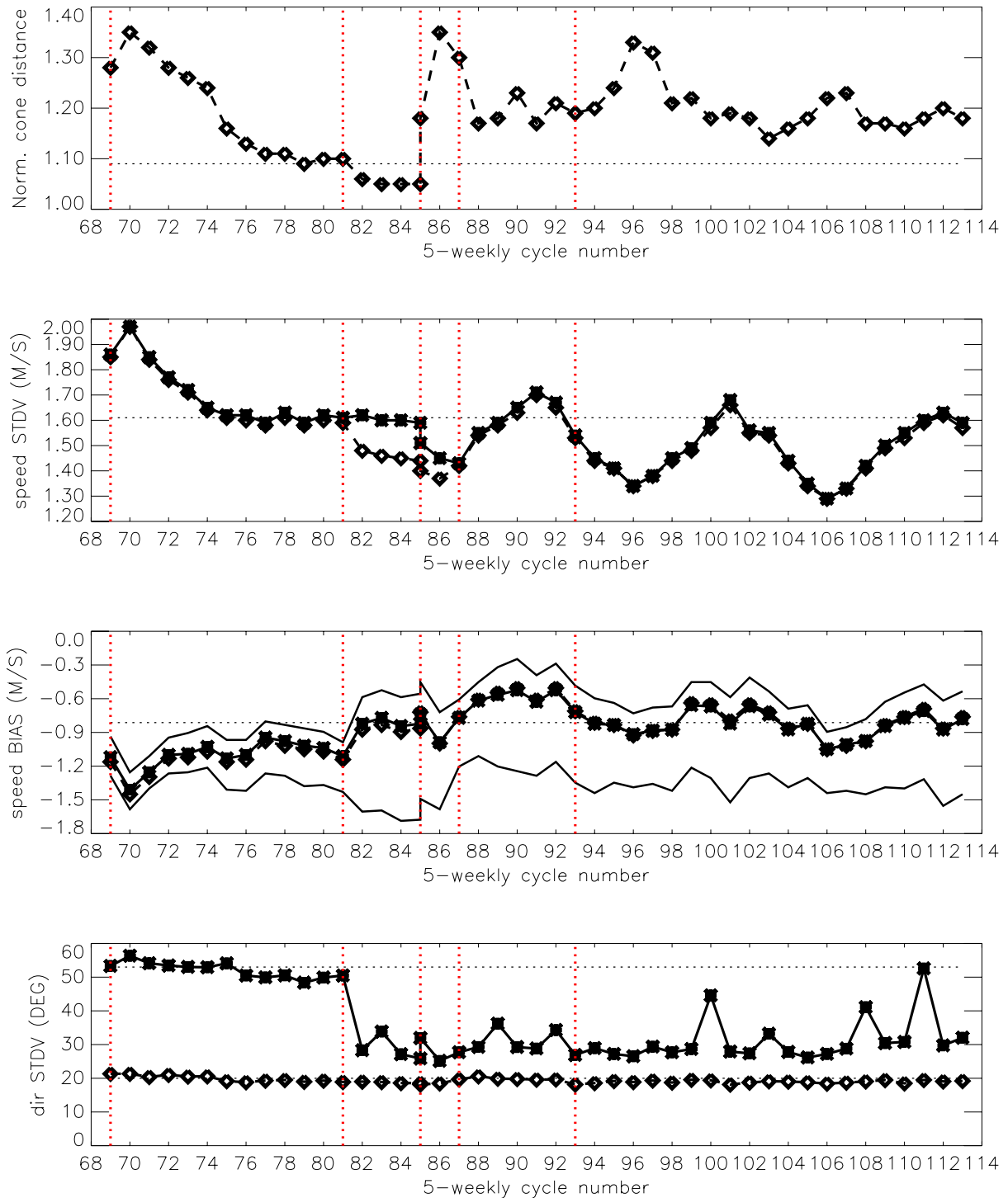
FIGURE 11 Evolution of the performance of the ERS-2 Scatterometer averaged over 5-weekly cycles from 12 December 2001 (cycle 69) to 13 March 2006 (end cycle 113) for the UWI product (solid, star) and de-aliased winds based on CMOD4(dashed, diamond). Results are based on data that passed the UWI QC flags. For cycle 85 two values are plotted; the first value for the global set, the second one for the regional set. Dotted lines represent values for cycle 59 (5 December 2000 to 17 January 2001),i.e. the last stable cycle of the nominal period. From top to bottom panel are shown the normalized distance to the one (CMOD4 only) the standard deviation of the wind speed compared to FG winds, the corresponding bias(for UWI winds the extreme inter-node averages are shown as well),and the standard deviation of wind direction compared to FG.
