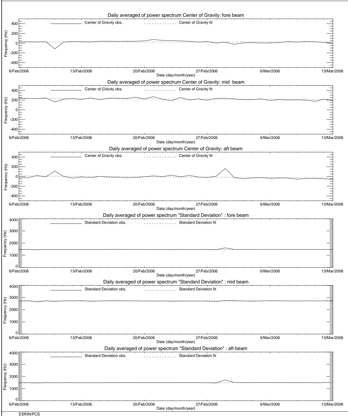
FIGURE 3 ERS-2 Scatterometer: Centre of Gravity and standard deviation of received power spectrum during the cycle 113.
