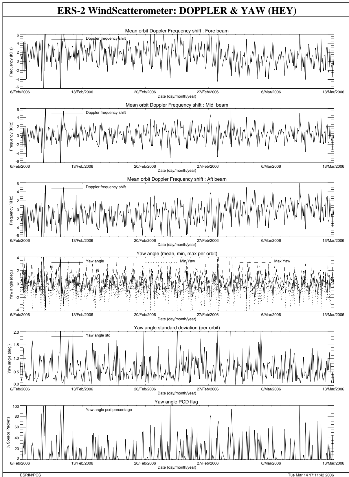
FIGURE 27 Doppler frequency shift and Yaw error angle evolution cycle 113.
