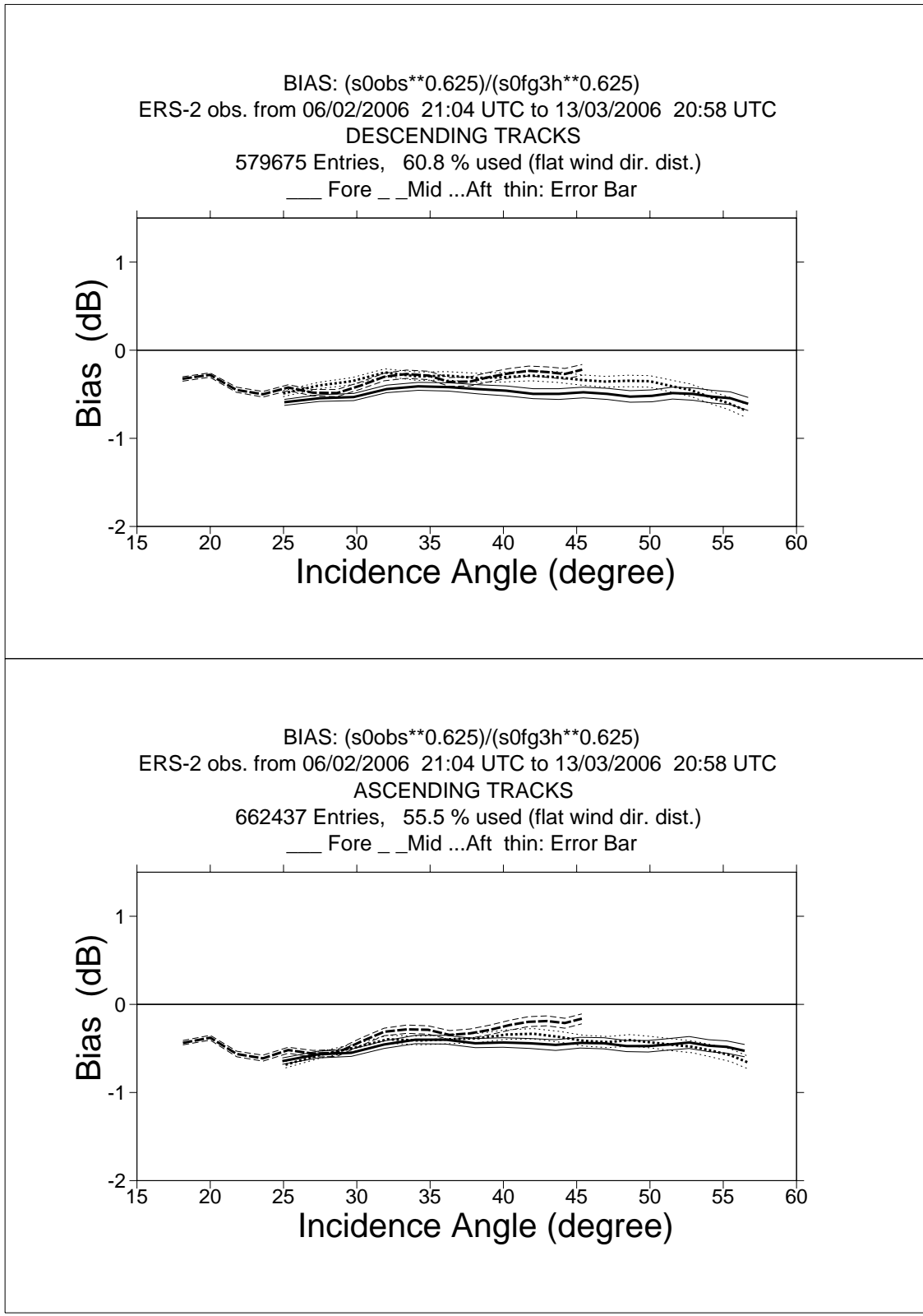
FIGURE 1 ERS-2 Scatterometer Ocean Calibration cycle 113. Ratio of \langle \sigma_0^{0.625} \rangle / \langle \text{CMOD4}(\text{First Guess})^{0.625} \rangle converted in dB for the fore beam (solid line), mid beam (dashed line) and aft beam (dotted line), as a function of incidence angle for descending and ascending tracks. The thin lines indicate the error bars on the estimated mean. First-guess winds are based on the in time closest (+3h, +6h, +9h, or +12h) T511 forecast field, and are bilinearly interpolated in space.
