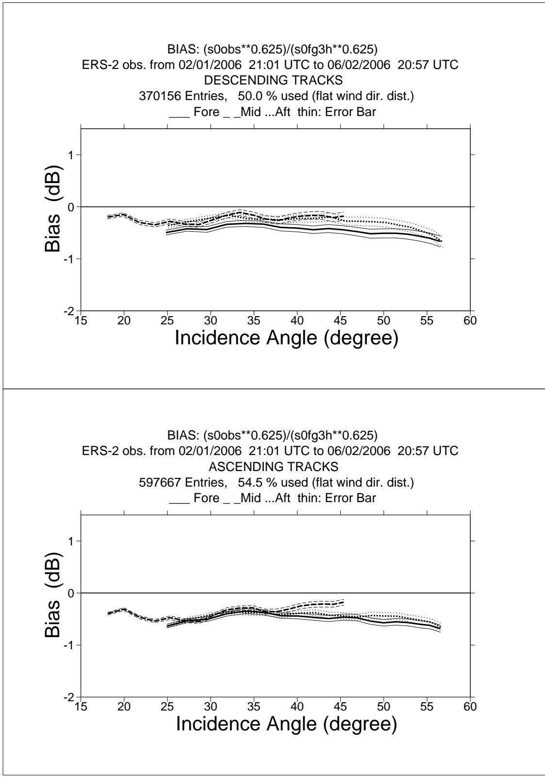
FIGURE 1 ERS-2 Scatterometer Ocean Calibration cycle 112. Ratio of \langle \sigma_0^{0.625} \rangle / \langle C_{MOD4}(\text{First Guess})^{0.625} \rangle converted in dB for the fore beam (solid line), mid beam (dashed line) an aft beam (dotted line), as a function of incidence angle for descending and ascending tracks. The thin lines indicate the error bars on the estimated mean. First-guess winds are based on the in time closest (+3h, +6h, +9h, or +12h) T511 forecast field, and are bilinearly interpolated in space.
