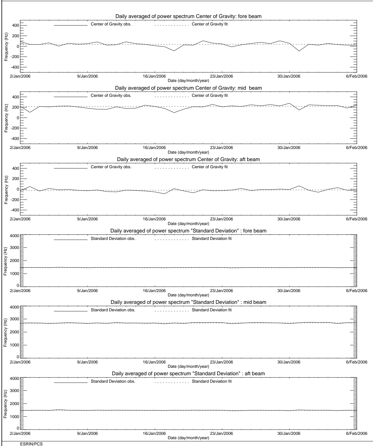
FIGURE 3 ERS-2 Scatterometer: Centre of Gravity and standard deviation of received power spectrum during the cycle 112.
