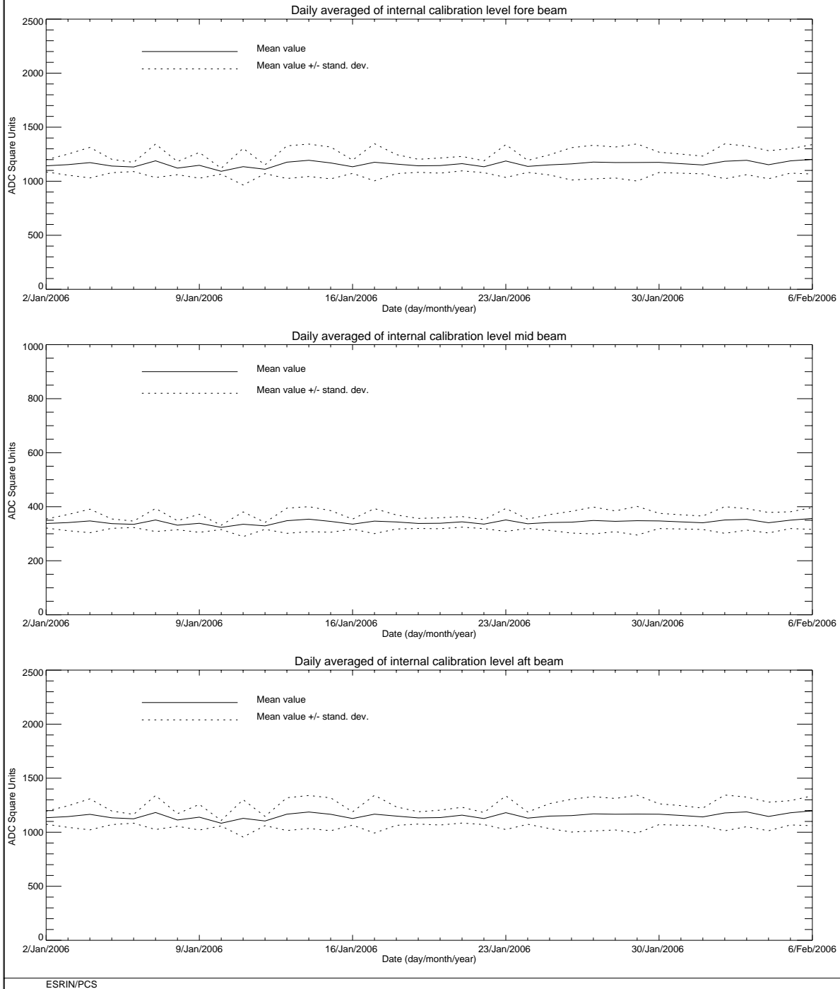
FIGURE 7 ERS-2 Scatterometer: power of internal calibration level cycle 112.
