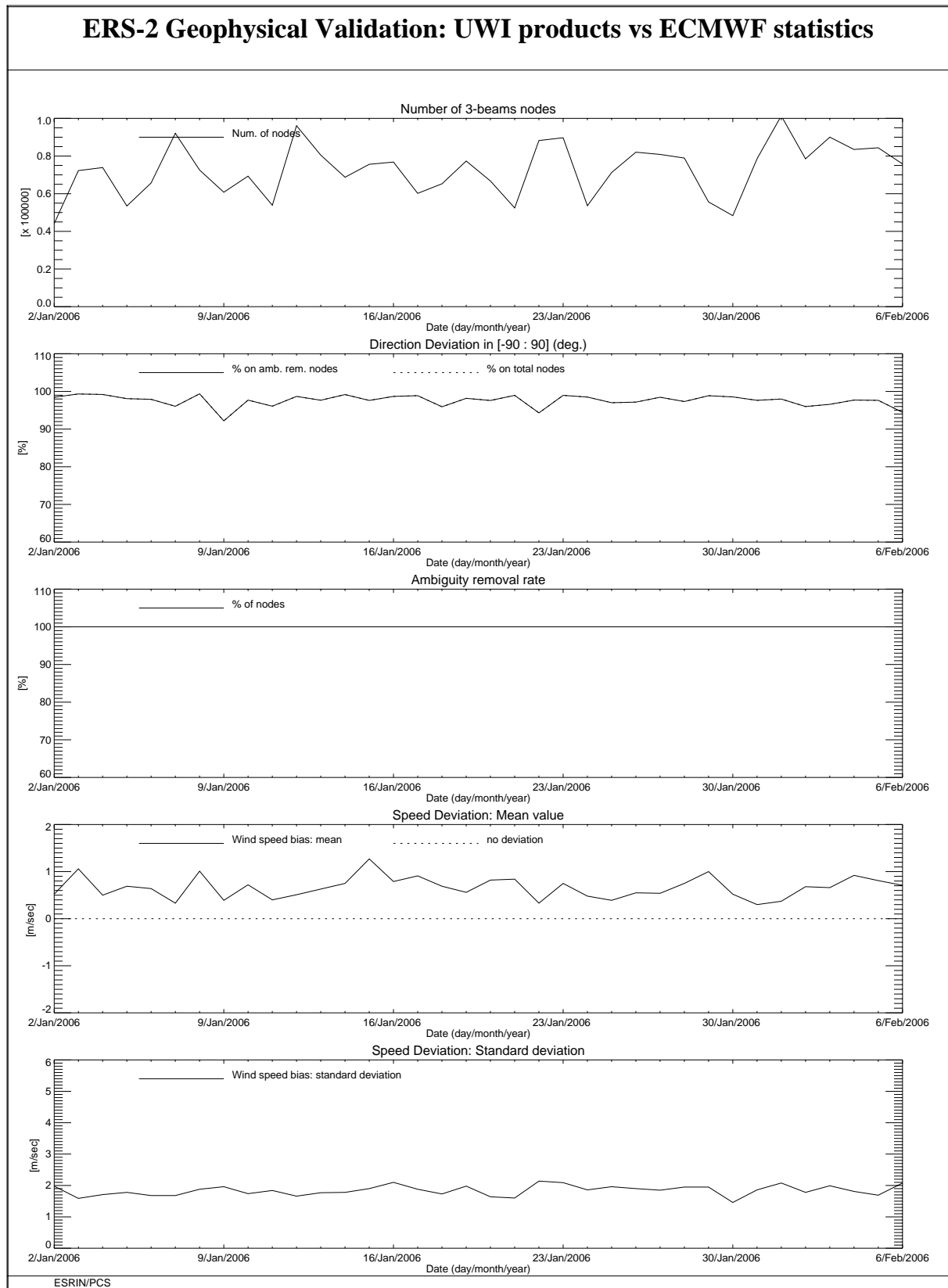
FIGURE 10 ERS-2 Scatterometer: wind products performance for cycle 112.
