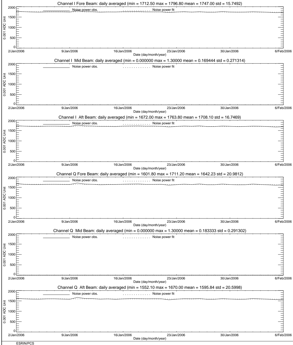
FIGURE 5 ERS-2 Scatterometer: noise power I and Q channel for cycle 112.
