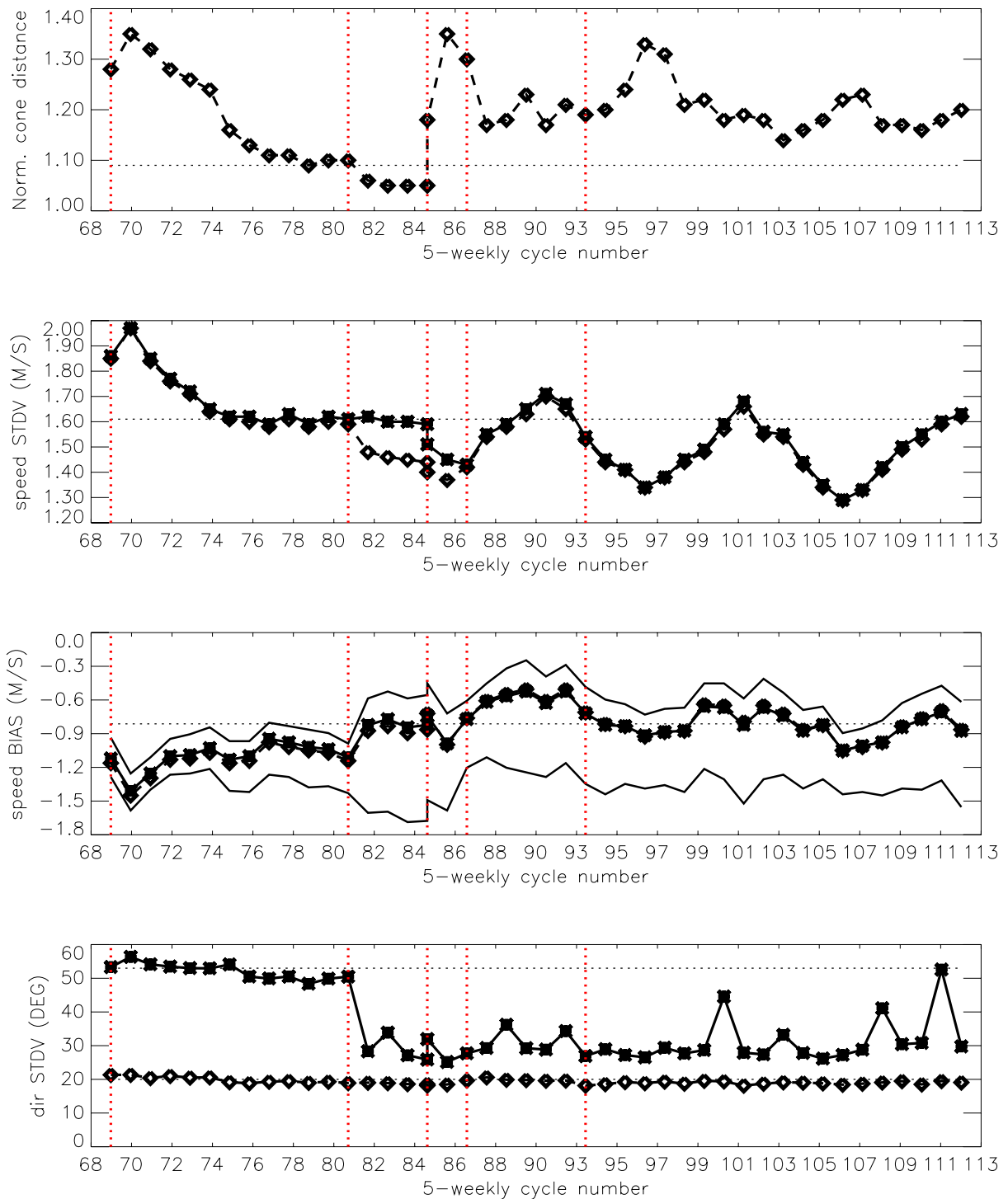
FIGURE 11 Evolution of the performance of the ERS-2 Scatterometer averaged over 5-weekly cycles from 12 December 2001 (cycle 69) to 6 February 2006 (end cycle 112) for the UWI product (solid, star) and de-aliased winds based on CMOD4(dashed, diamond). Results are based on data that passed the UWI QC flags. For cycle 85 two values are plotted; the first value for the global set, the second one for the regional set. Dotted lines represent values for cycle 59 (5 December 2000 to 17 January 2001),i.e. the last stable cycle of the nominal period. From top to bottom panel are shown the normalized distance to the one (CMOD4 only) the standard deviation of the wind speed compared to FG winds, the corresponding bias(for UWI winds the extreme inter-node averages are shown as well),and the standard deviation of wind direction compared to FG.
