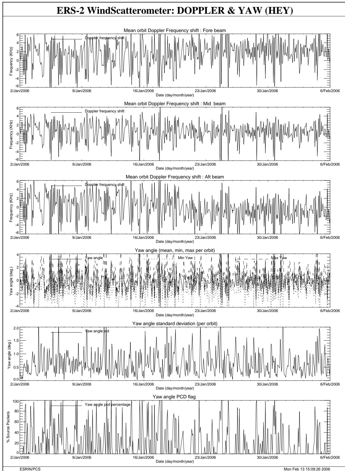
FIGURE 27 Doppler frequency shift and Yaw error angle evolution cycle 112.
