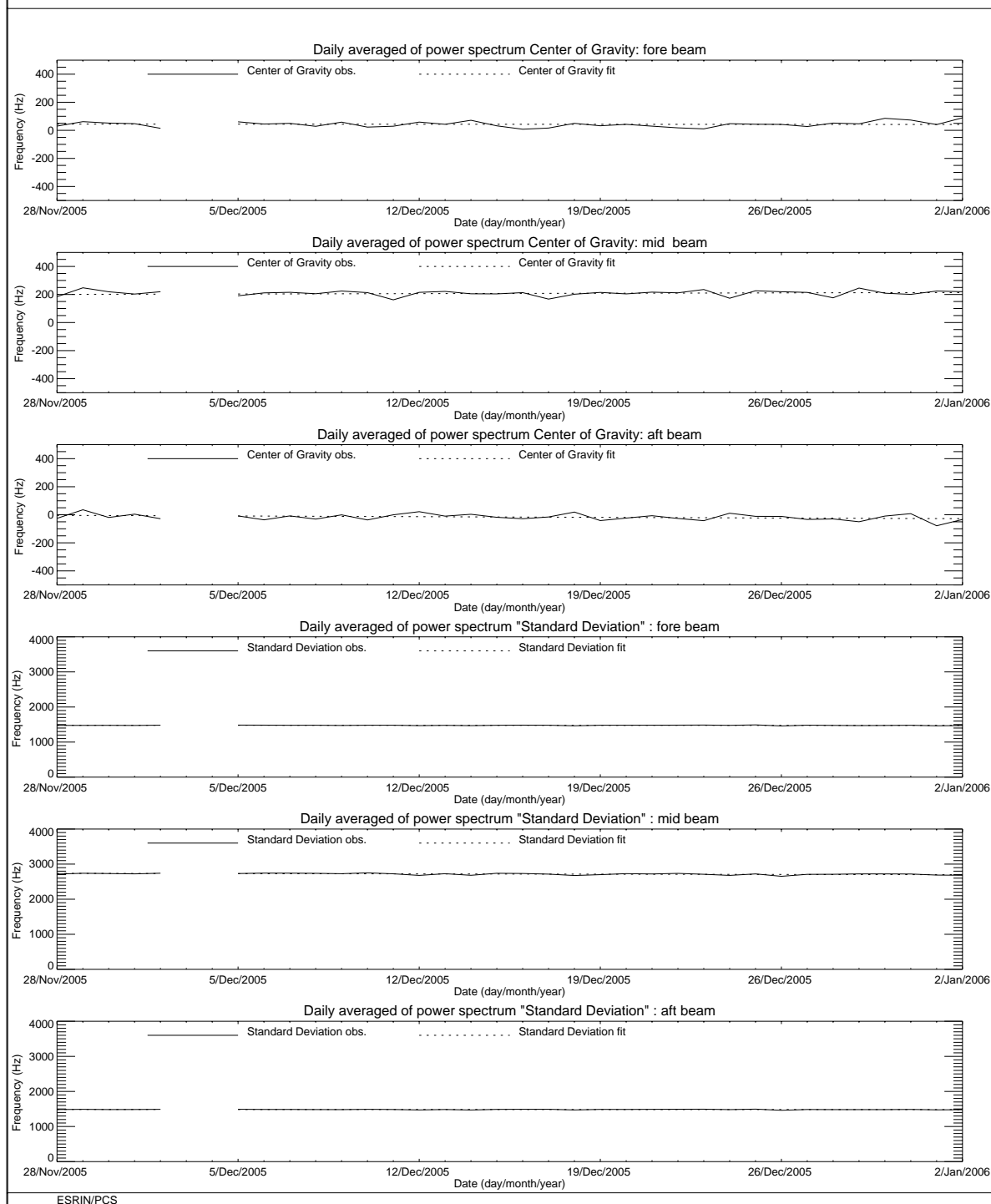
FIGURE 3 ERS-2 Scatterometer: Centre of Gravity and standard deviation of received power spectrum during the cycle 111.
