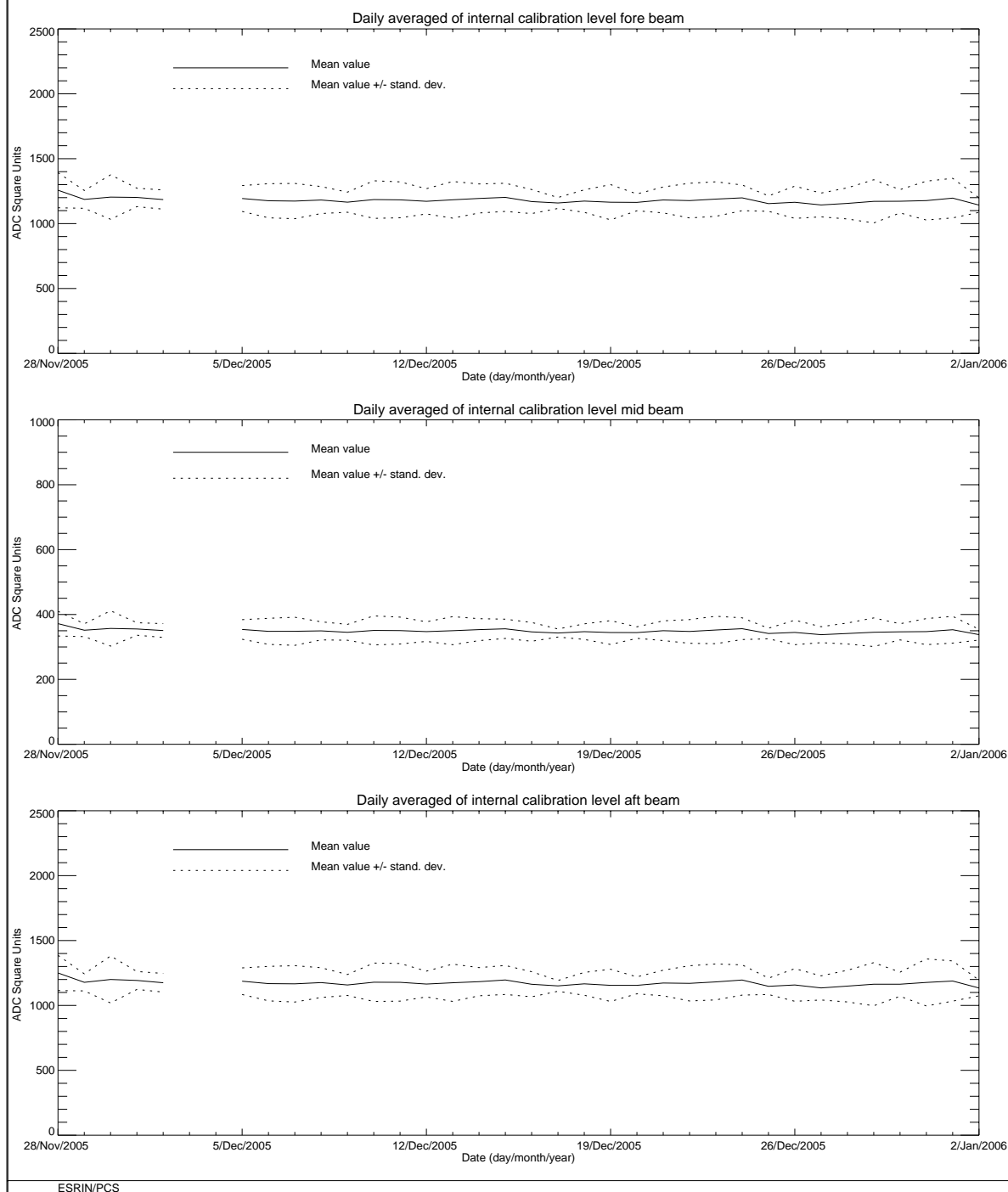
FIGURE 7 ERS-2 Scatterometer: power of internal calibration level cycle 111.
