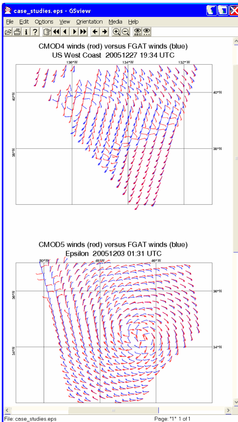
FIGURE 20 Comparison between UWI (red) and ECMWF FG (blue) winds for a case on 27 December 2005 off the US West Coast (top panel) and de-aliased CMOD 5 winds versus ECMWF FG for cyclone Epsilon on 3 December 2005, in the North Atlantic (lower panel)
