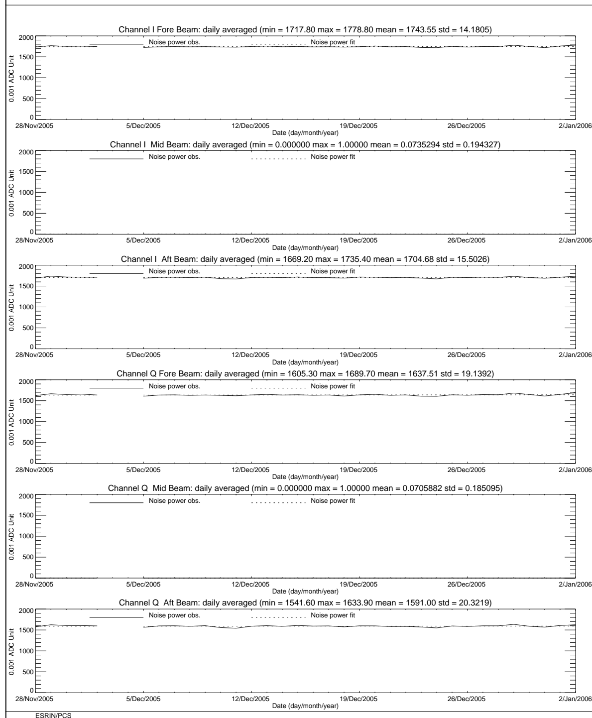
FIGURE 5 ERS-2 Scatterometer: noise power I and Q channel for cycle 111.
