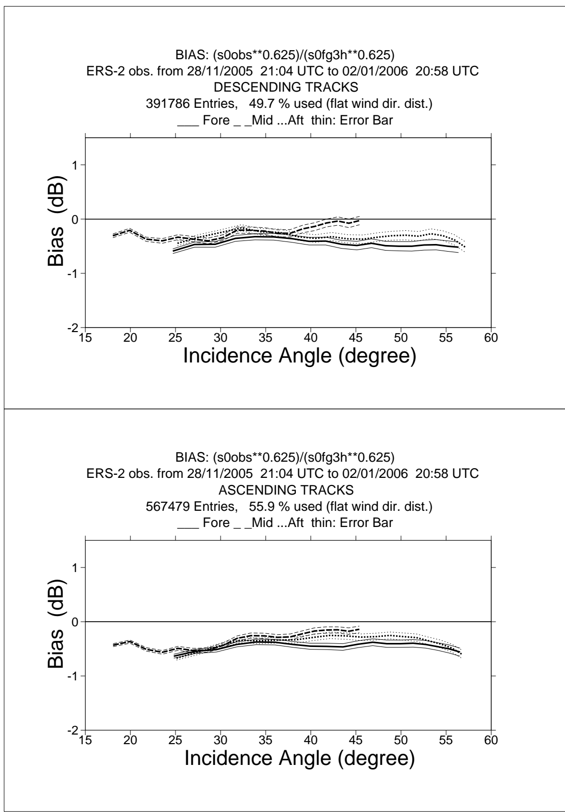
FIGURE 1 ERS-2 Scatterometer Ocean Calibration cycle 111. Ratio of \langle \sigma_0^{0.625} \rangle / \langle \text{CMOD4}(\text{First Guess})^{0.625} \rangle converted in dB for the fore beam (solid line), mid beam (dashed line) and aft beam (dotted line), as a function of incidence angle for descending and ascending tracks. The thin lines indicate the error bars on the estimated mean. First-guess winds are based on the in time closest (+3h, +6h, +9h, or +12h) T511 forecast field, and are bilinearly interpolated in space.
