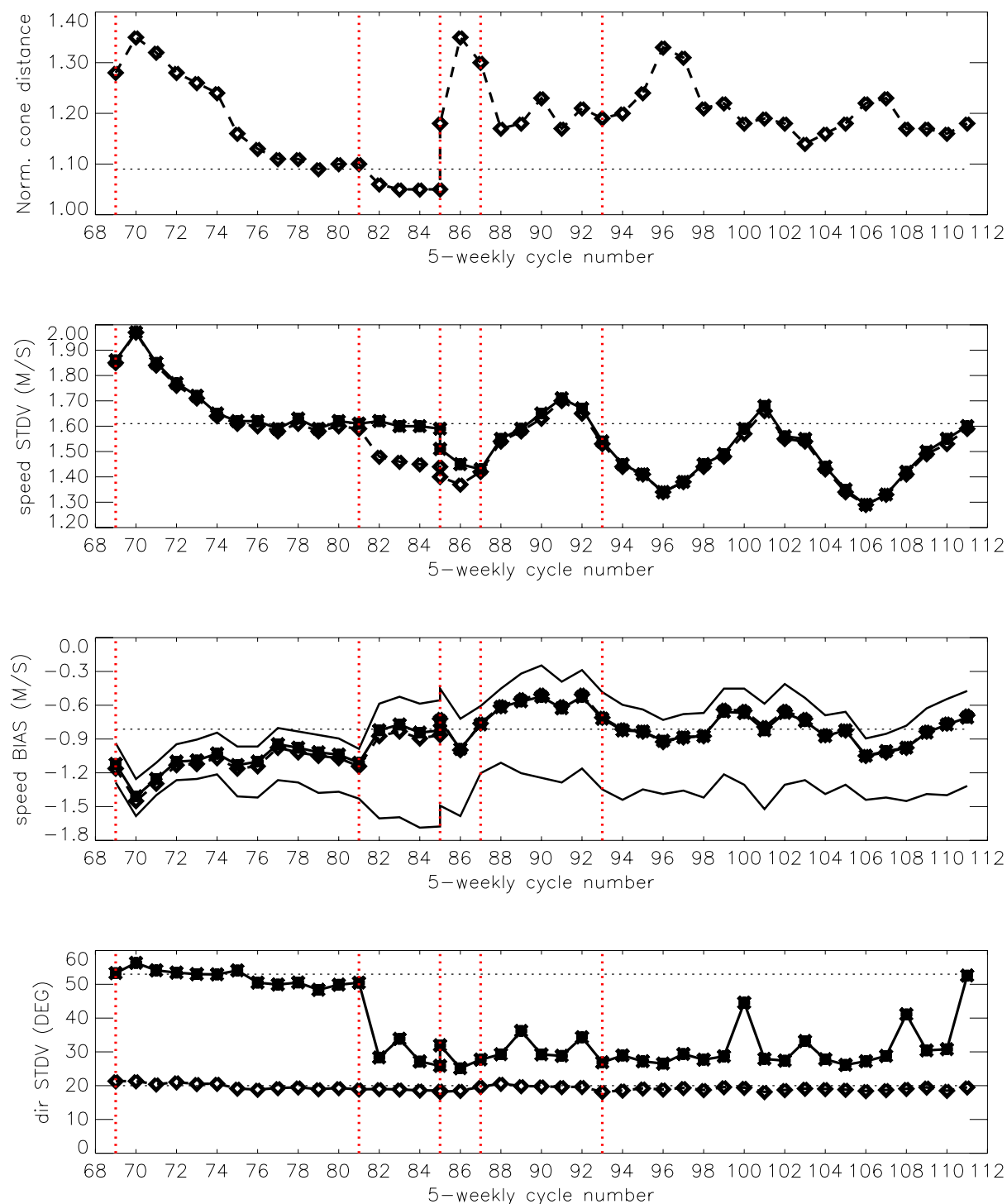
FIGURE 11 Evolution of the performance of the ERS-2 Scatterometer averaged over 5-weekly cycles from 12 December 2001 (cycle 69) to 2 January 2006 (end cycle 111) for the UWI product (solid, star) and de-aliased winds based on CMOD4(dashed, diamond). Results are based on data that passed the UWI QC flags. For cycle 85 two values are plotted; the first value for the global set, the second one for the regional set. Dotted lines represent values for cycle 59 (5 December 2000 to 17 January 2001), i.e. the last stable cycle of the nominal period. From top to bottom panel are shown the normalized distance to the one (CMOD4 only) the standard deviation of the wind speed compared to FG winds, the corresponding bias (for UWI winds the extreme inter-node averages are shown as well), and the standard deviation of wind direction compared to FG.
