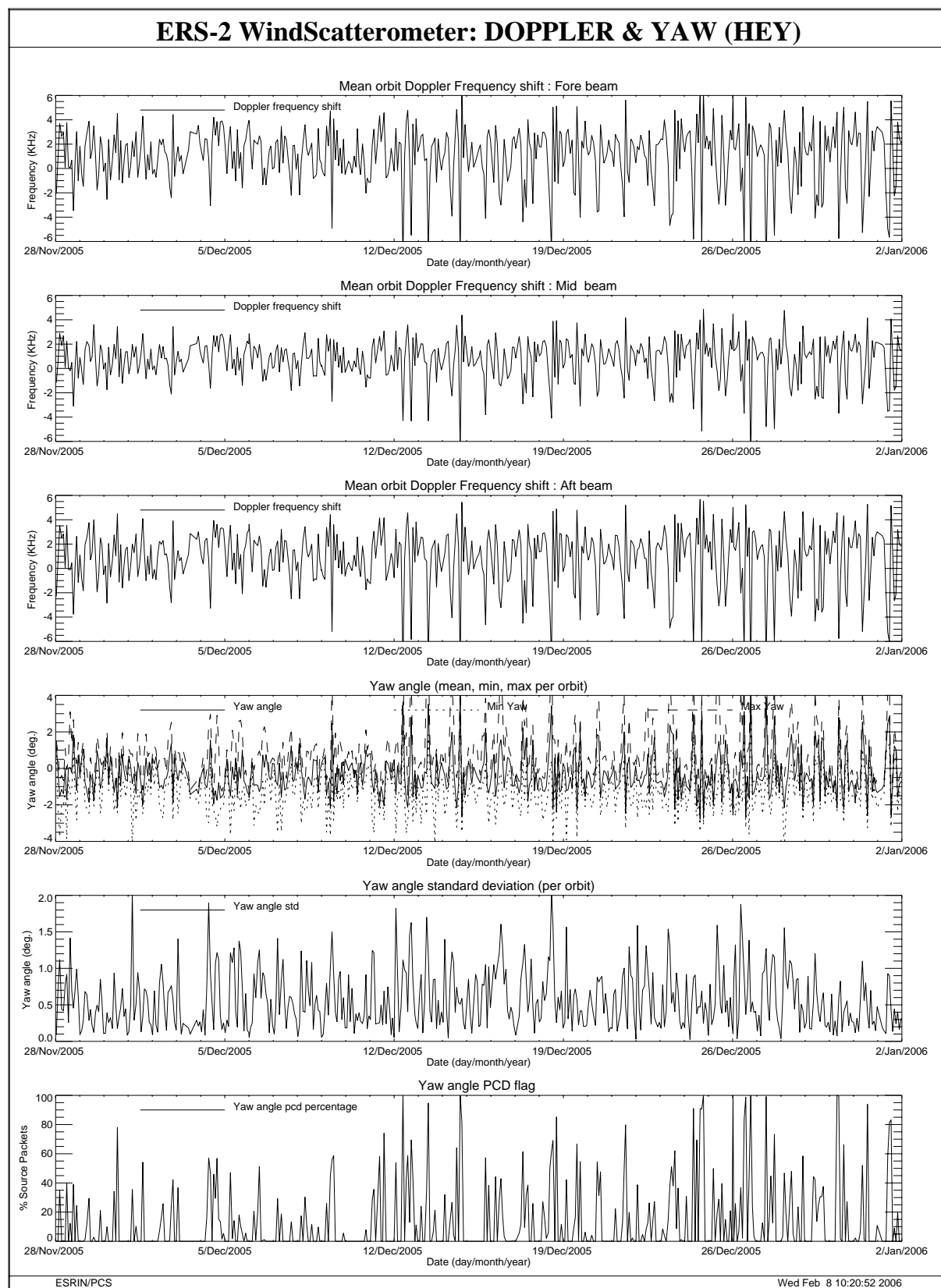
FIGURE 27 Doppler frequency shift and Yaw error angle evolution cycle 111.
