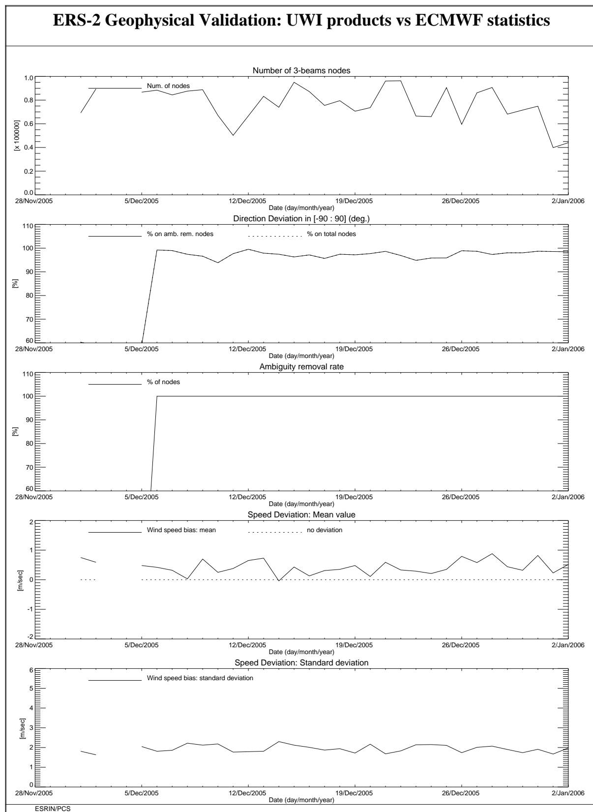
FIGURE 10 ERS-2 Scatterometer: wind products performance for cycle 111.
