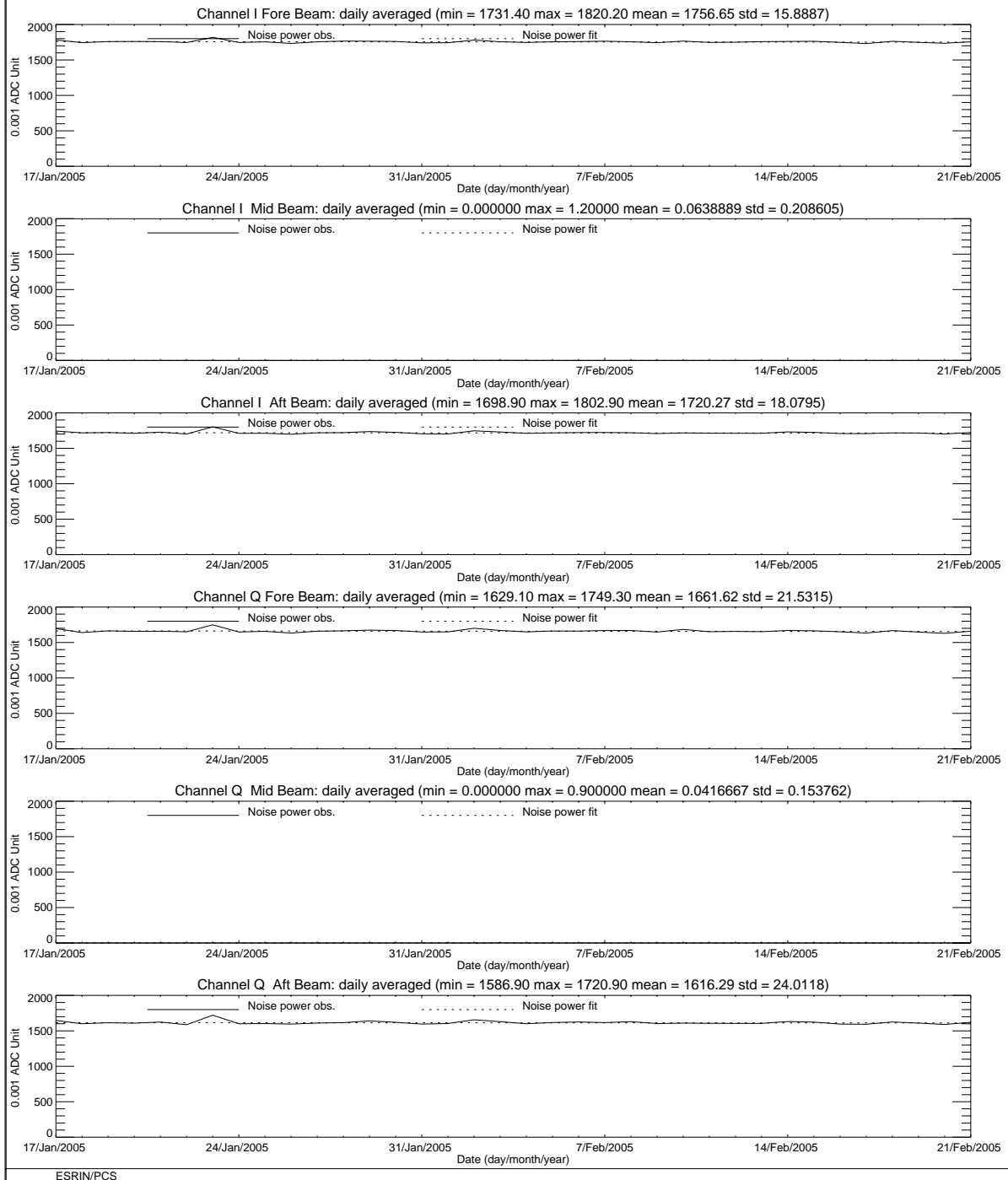
FIGURE 5 ERS-2 Scatterometer: noise power I and Q channel for cycle 102.
