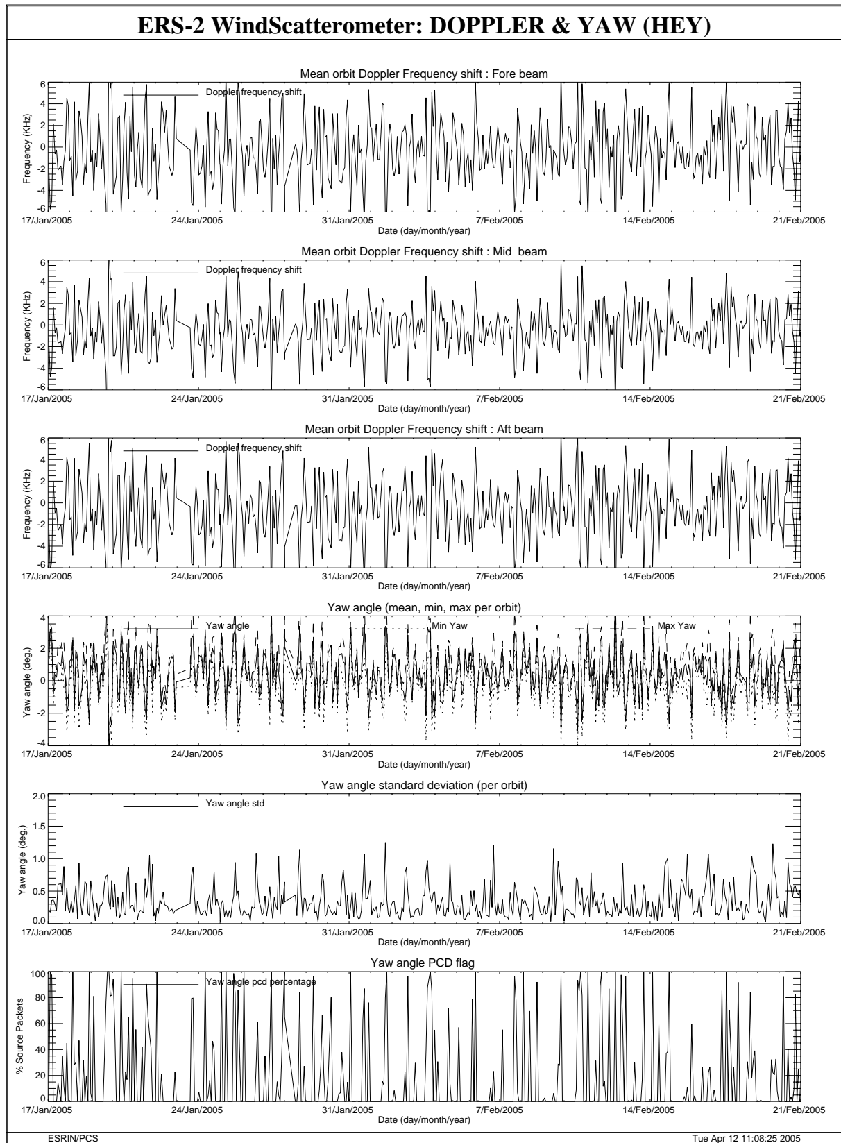
FIGURE 27 Doppler frequency shift and Yaw error angle evolution cycle 102.
