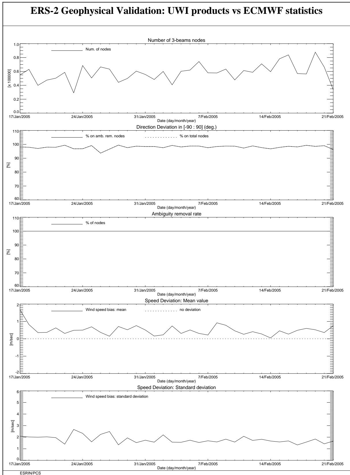
FIGURE 10 ERS-2 Scatterometer: wind products performance for cycle 102.
