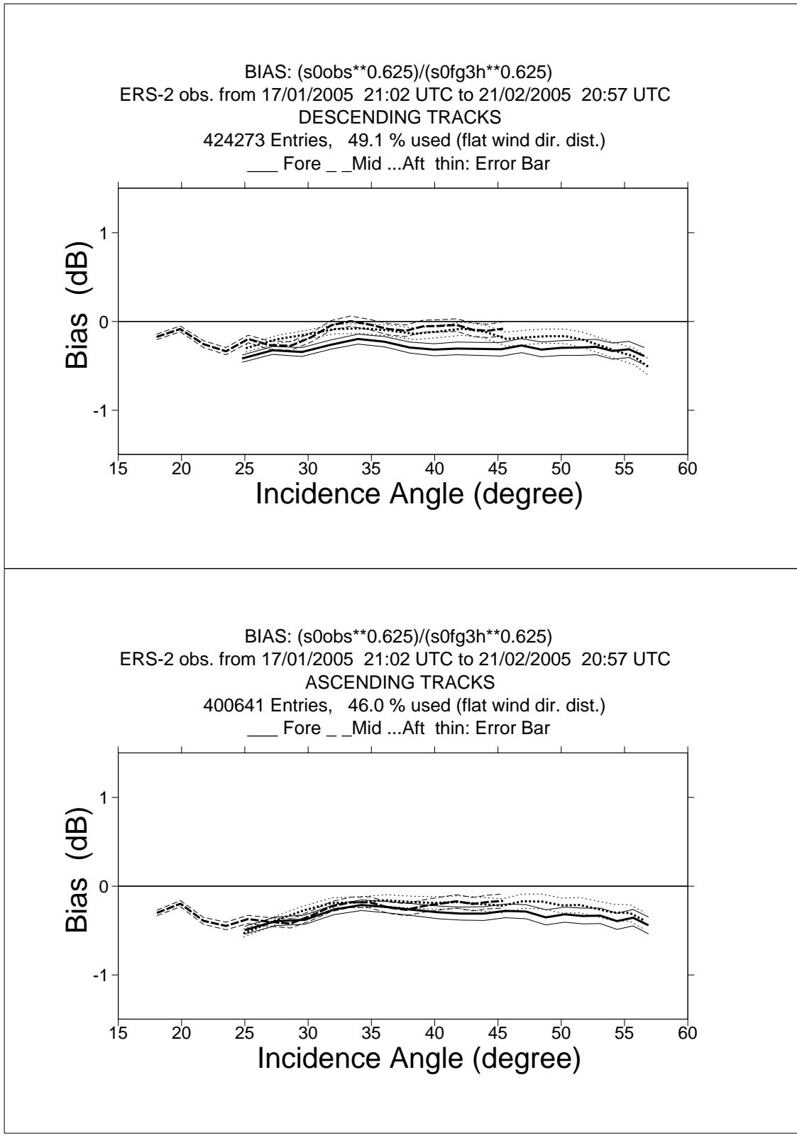
FIGURE 1 ERS-2 Scatterometer Ocean Calibration cycle 102. Ratio of \langle \sigma_0^{0.625} \rangle / \langle \text{CMOD4}(\text{First Guess})^{0.625} \rangle converted in dB for the fore beam (solid line), mid beam (dashed line) and aft beam (dotted line), as a function of incidence angle for descending and ascending tracks. The thin lines indicate the error bars on the estimated mean. First-guess winds are based on the in time closest (+3h, +6h, +9h, or +12h) T511 forecast field, and are bilinearly interpolated in space.
