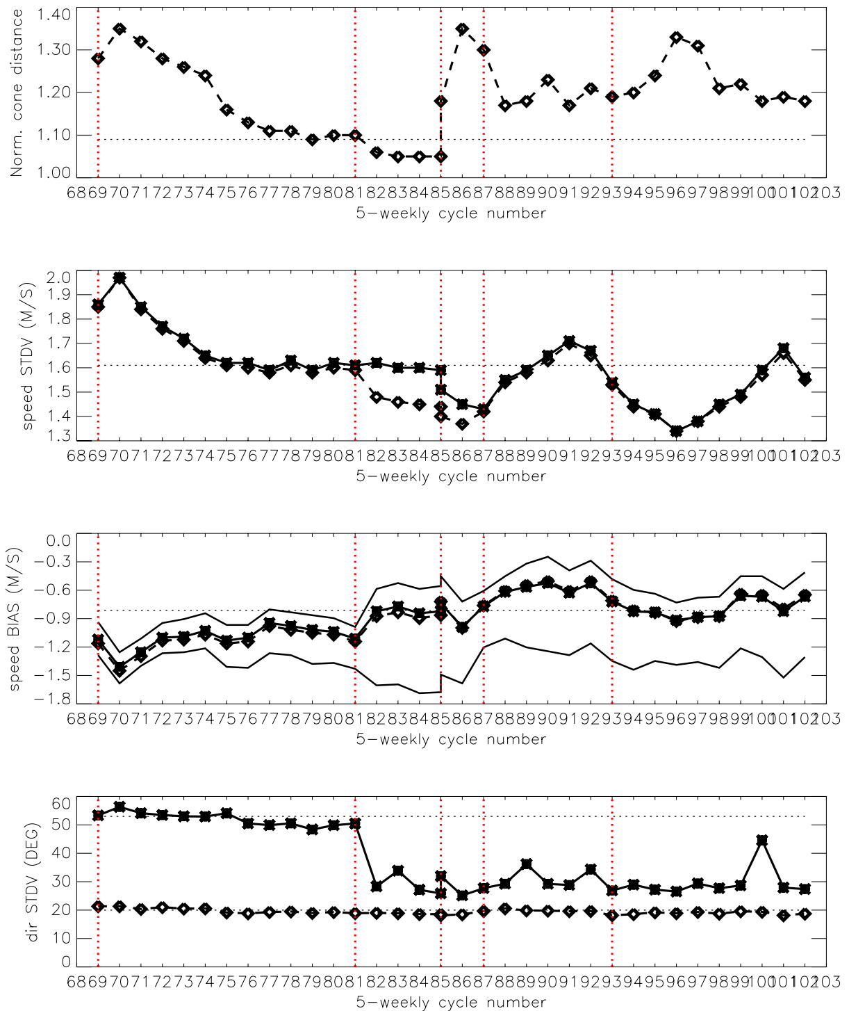
FIGURE 11 Evolution of the performance of the ERS-2 Scatterometer averaged over 5-weekly cycles from 12 December 2001 (cycle 69) to 21 February 2005 (end cycle 102) for the UWI product (solid, star) and de-aliased winds based on CMOD4(dashed, diamond). Results are based on data that passed the UWI QC flags. For cycle 85 two values are plotted; the first value for the global set, the second one for the regional set. Dotted lines represent values for cycle 59 (5 December 2000 to 17 January 2001),i.e. the last stable cycle of the nominal period. From top to bottom panel are shown the normalized distance to the one (CMOD4 only) the standard deviation of the wind speed compared to FG winds, the corresponding bias(for UWI winds the extreme inter-node averages are shown as well),and the standard deviation of wind direction compared to FG.
