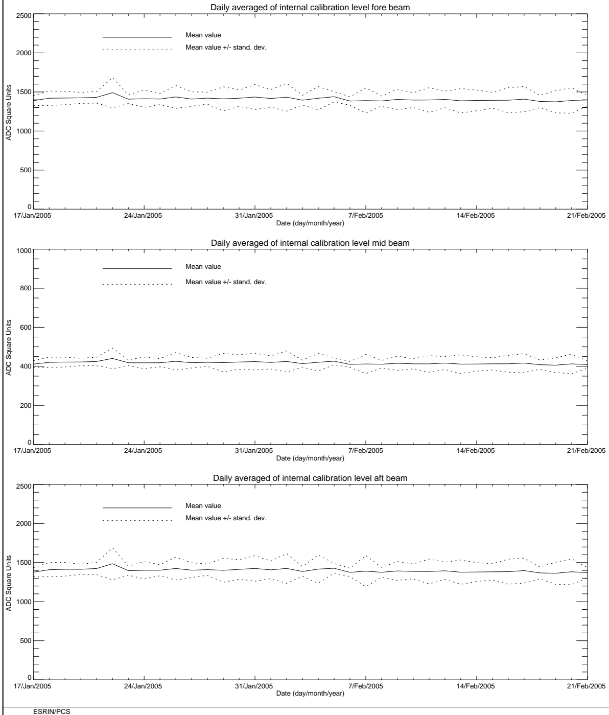
FIGURE 7 ERS-2 Scatterometer: power of internal calibration level cycle 102.
