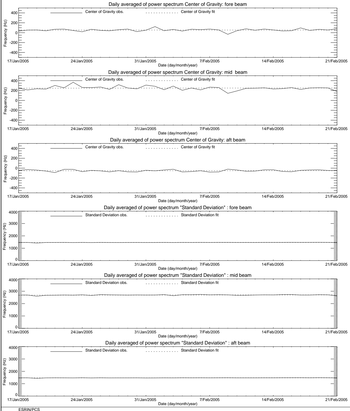
FIGURE 3 ERS-2 Scatterometer: Centre of Gravity and standard deviation of received power spectrum during the cycle 102.
