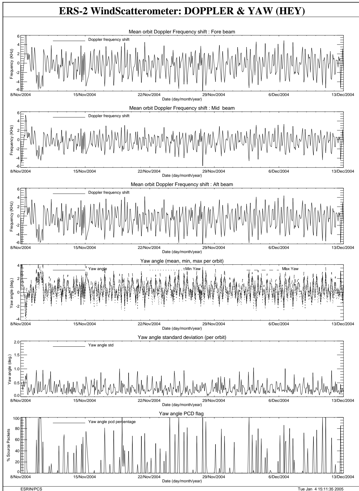
FIGURE 27 Doppler frequency shift and Yaw error angle evolution cycle 100.
