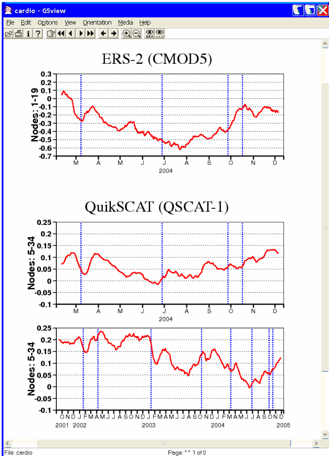
FIGURE 25 Bias relative to FG winds of the wind speed of ERS-2 winds (based on bias-corrected CMOD4 before 9 March 2004, and on CMOD5 afterwards) for nodes 1-19 (top panel) respectively of 50-km QuikSCAT (based on the QSCAT-1 model function) for nodes 5-34 (i.e., inner-beam zone; middle and lower panels) versus ECMWF first guess for the period of cycle 92 to 100. Curves represent centered 15-day running means for the top and middle panel, and a 30-day running mean for the lower panel. Vertical dashed blue lines mark ECMWF model changes
