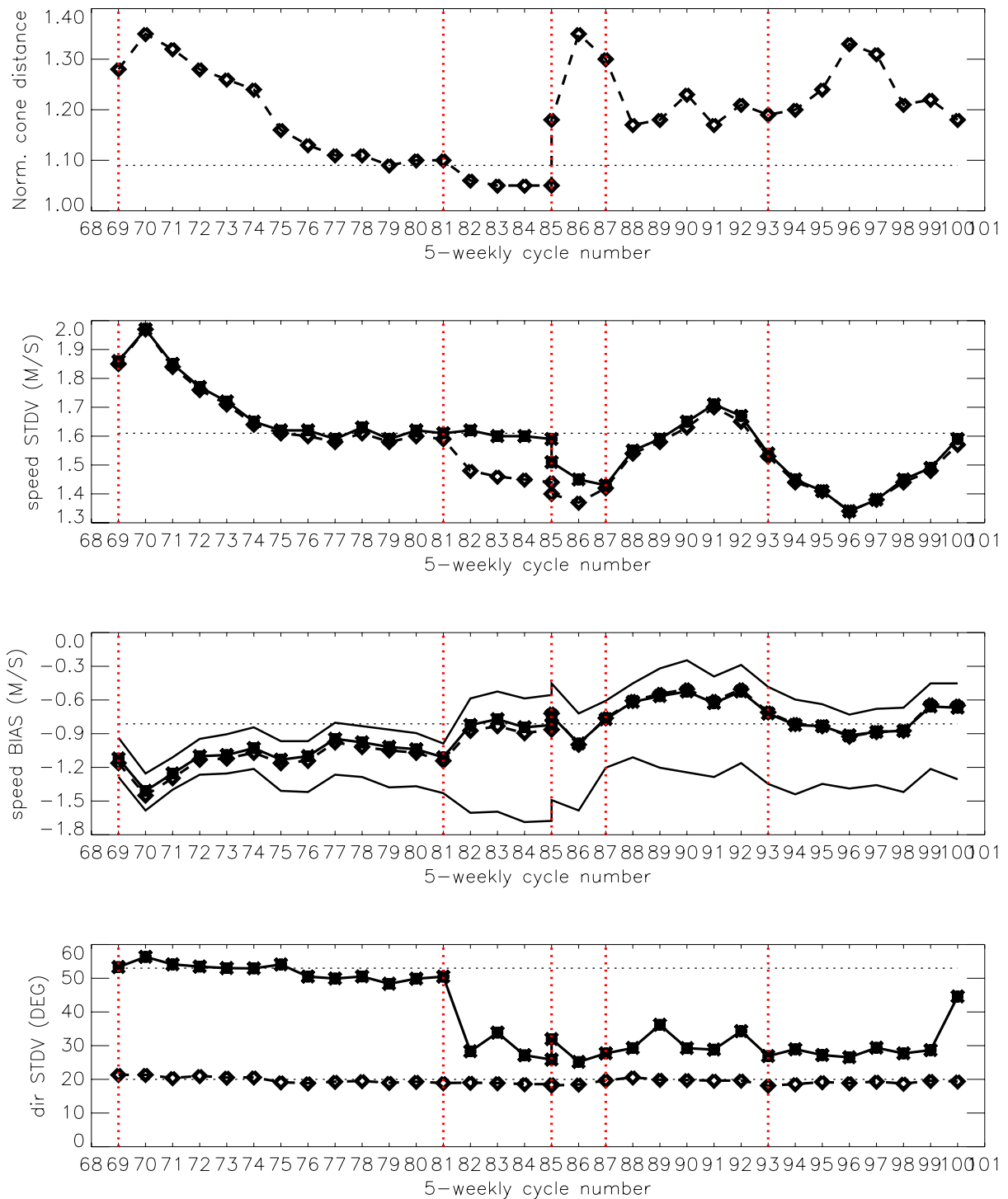
FIGURE 11 Evolution of the performance of the ERS-2 Scatterometer averaged over 5-weekly cycles from 12 December 2001 (cycle 69) to 13 December 2004 (end cycle 100) for the UWI product (solid, star) and de-aliased winds based on CMOD4(dashed, diamond). Results are based on data that passed the UWI QC flags. For cycle 85 two values are plotted; the first value for the global set, the second one for the regional set. Dotted lines represent values for cycle 59 (5 December 2000 to 17 January 2001),i.e. the last stable cycle of the nominal period. rom top to bottom panel are shown the normalized distance to the one (CMOD4 only) the standard deviation of the wind speed compared to FG inds, the corresponding bias(for UWI winds the extreme inter-node averages are shown as well),and the standard deviation of wind direction compared to FG.
