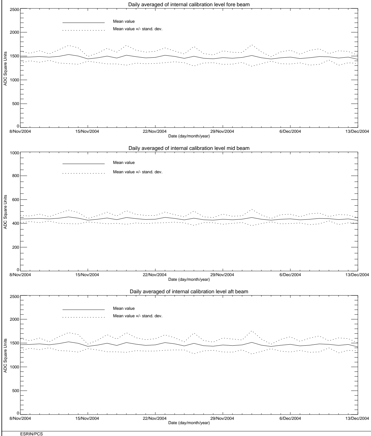
FIGURE 7 ERS-2 Scatterometer: power of internal calibration level cycle 100.
