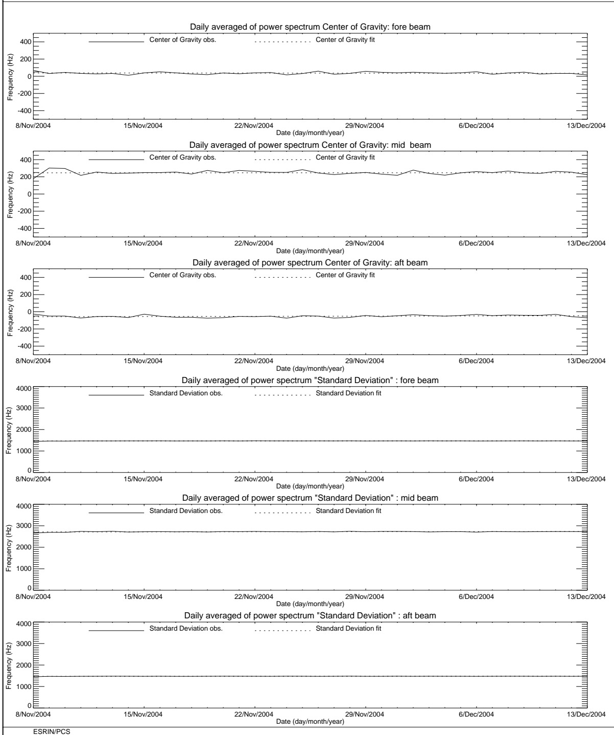
FIGURE 3 ERS-2 Scatterometer: Centre of Gravity and standard deviation of received power spectrum during the cycle 100.
