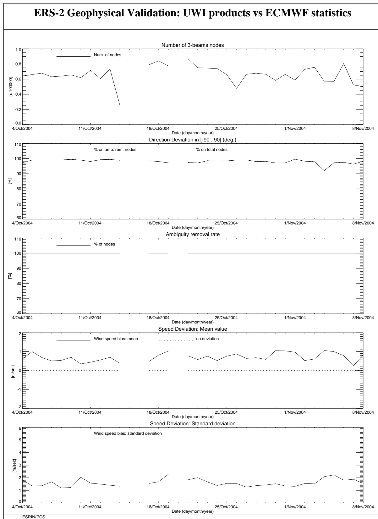
FIGURE 10 ERS-2 Scatterometer: wind products performance for cycle 99.
