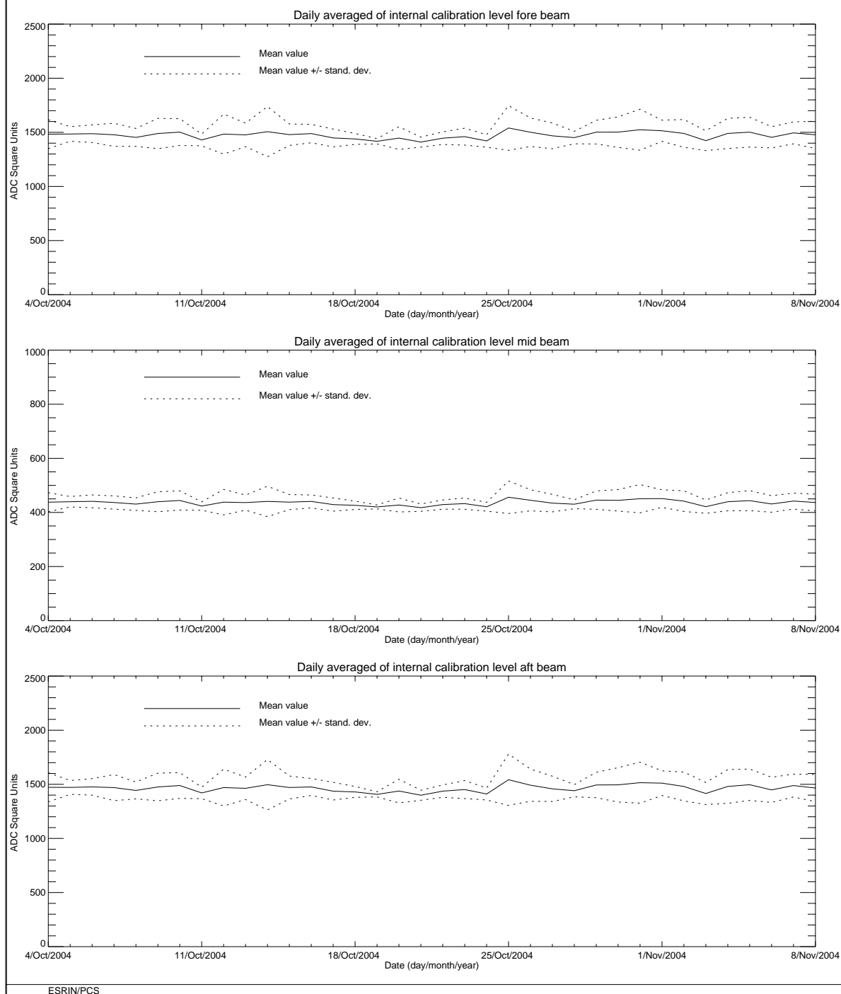
FIGURE 7 ERS-2 Scatterometer: power of internal calibration level cycle 99.
