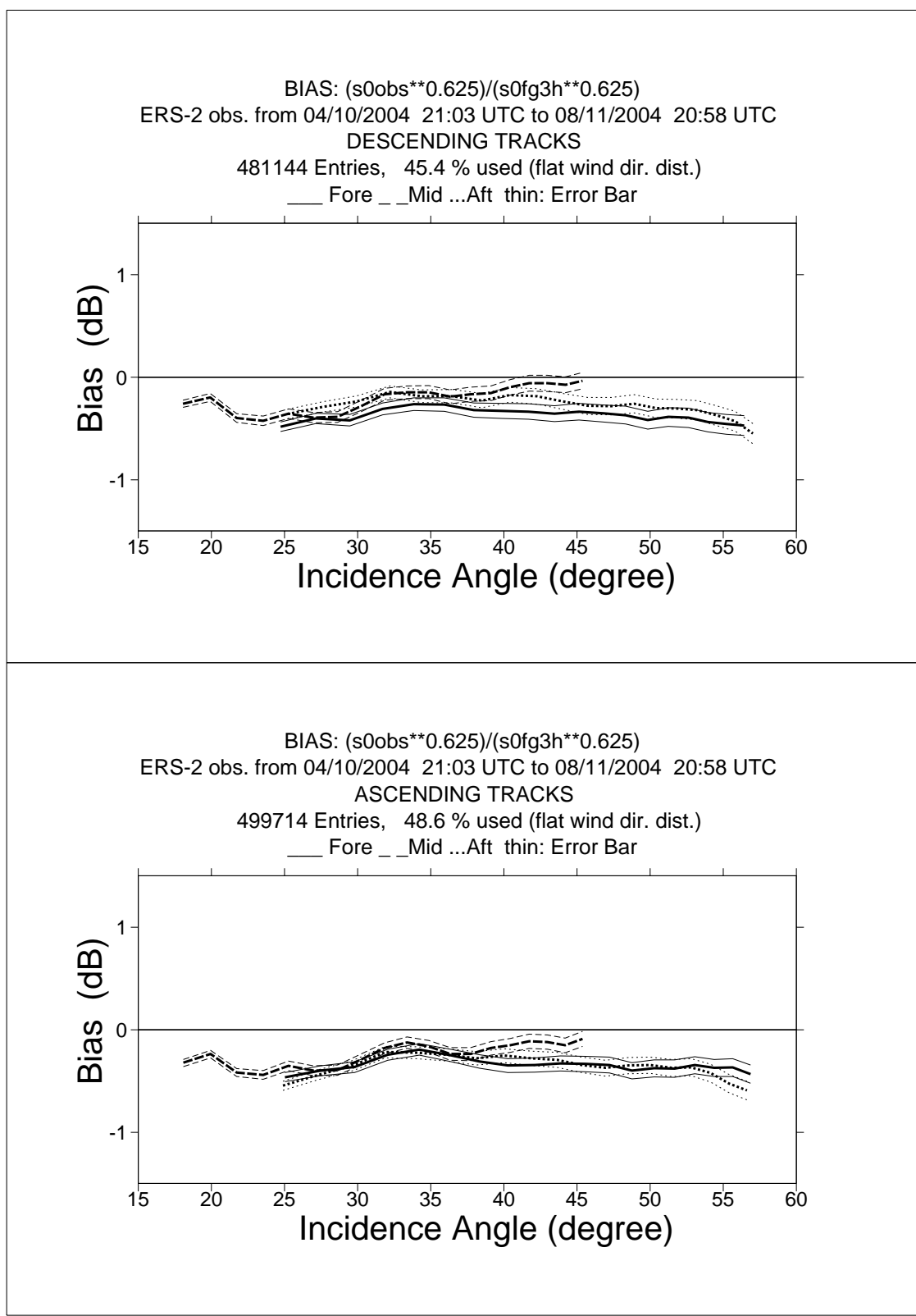
FIGURE 1 ERS-2 Scatterometer Ocean Calibration cycle 99. Ratio of \langle \sigma_0^{0.625} \rangle / \langle \text{CMOD4}(\text{First Guess})^{0.625} \rangle converted in dB for the fore beam (solid line), mid beam (dashed line) and aft beam (dotted line), as a function of incidence angle for descending and ascending tracks. The thin lines indicate the error bars on the estimated mean. First-guess winds are based on the in time closest (+3h, +6h, +9h, or +12h) T511 forecast field, and are bilinearly interpolated in space.
