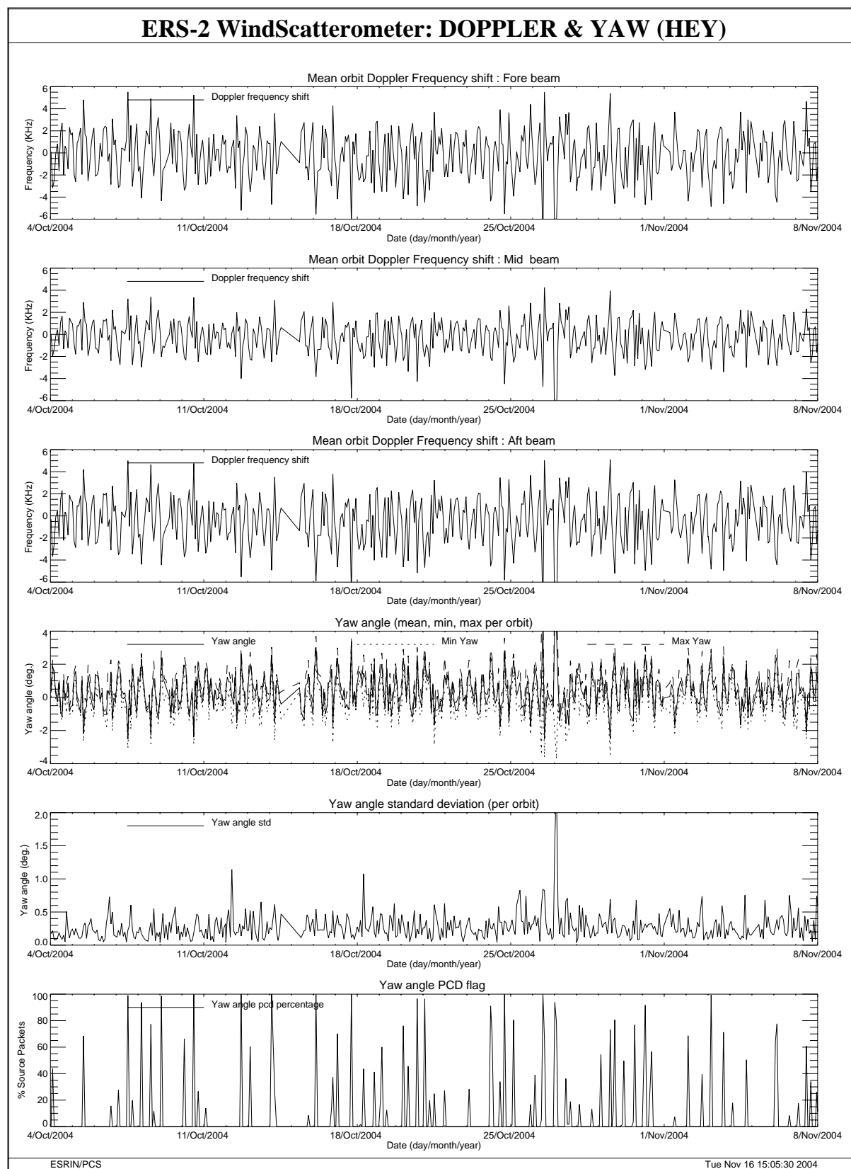
FIGURE 27 Doppler frequency shift and Yaw error angle evolution cycle 99.
