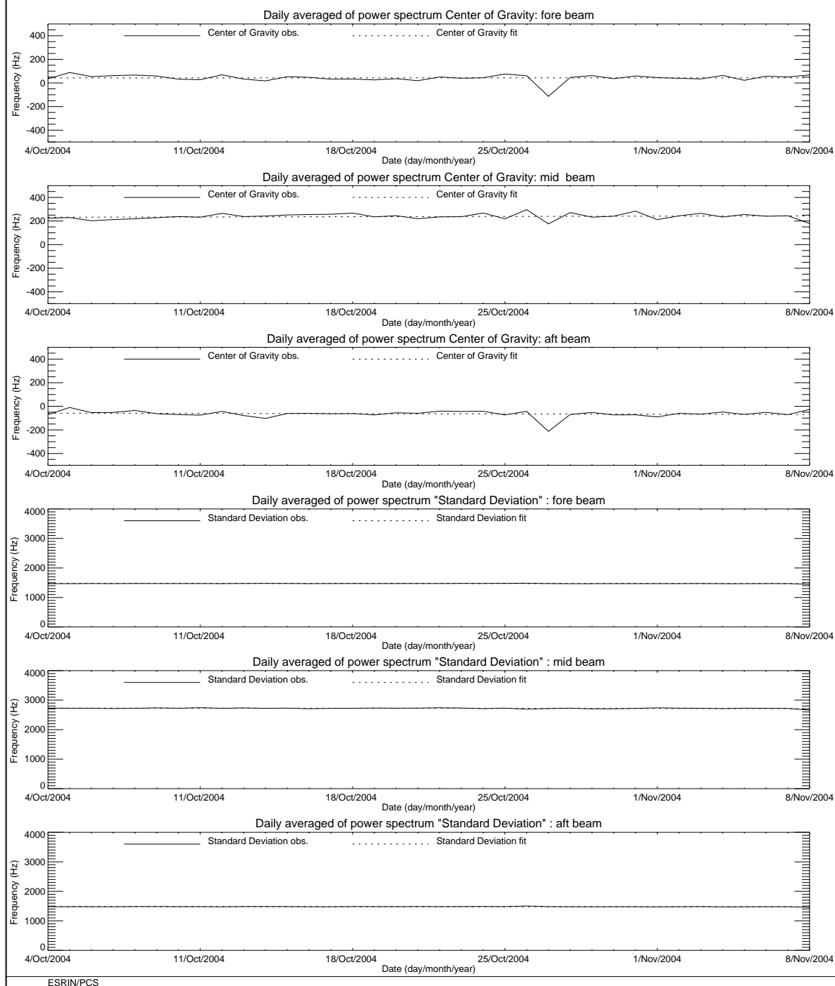
FIGURE 3 ERS-2 Scatterometer: Centre of Gravity and standard deviation of received power spectrum during the cycle 99.
