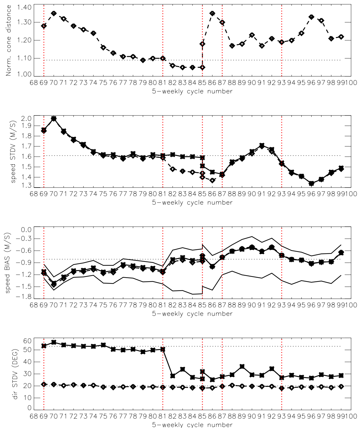
FIGURE 11 Evolution of the performance of the ERS-2 Scatterometer averaged over 5-weekly cycles from 12 December 2001 (cycle 69) to 8 November 2004 (end cycle 99) for the UWI product (solid, star) and de-aliased winds based on CMOD4(dashed, diamond). Results are based on data that passed the UWI QC flags. For cycle 85 two values are plotted; the first value for the global set, the second one for the regional set. Dotted lines represent values for cycle 59(5 December 2000 to 17 January 2001),i.e. the last stable cycle of the nominal period. rom top to bottom panel are shown the normalized distance to the one (CMOD4 only) the standard deviation of the wind speed compared to FG inds, the corresponding bias(for UWI winds the extreme inter-node averages are shown as well),and the standard deviation of wind direction compared to FG.
