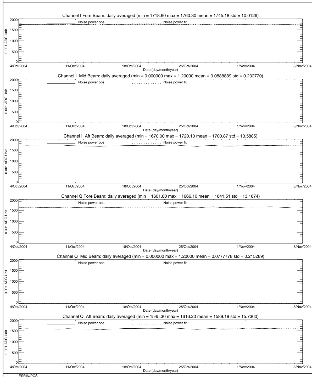
FIGURE 5 ERS-2 Scatterometer: noise power I and Q channel for cycle 99.
