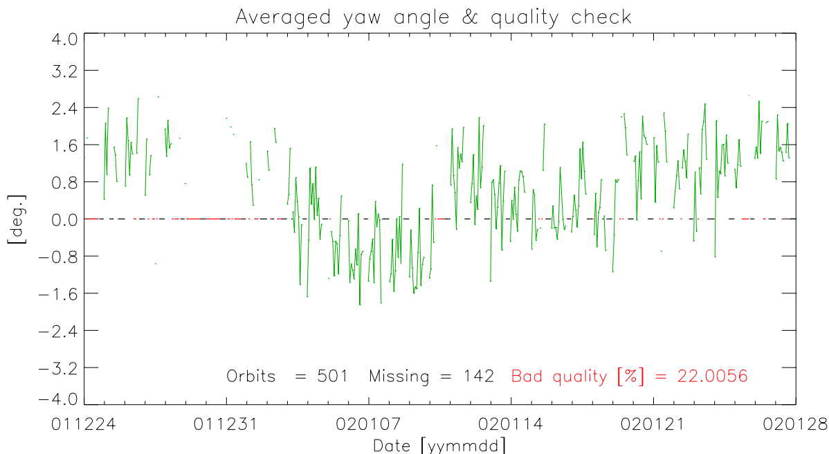
FIGURE 29. Averaged yaw error angle for cycle 70
