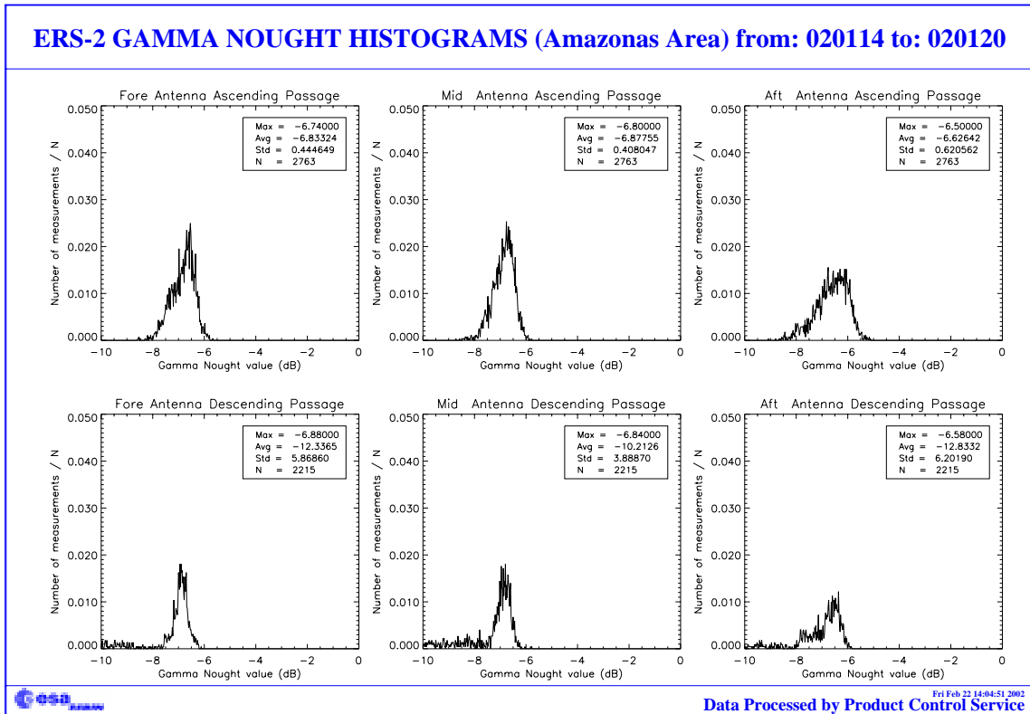
FIGURE 13. Gamma-nought histograms over Brazilian rain forest: fourth week of the cycle 70.
