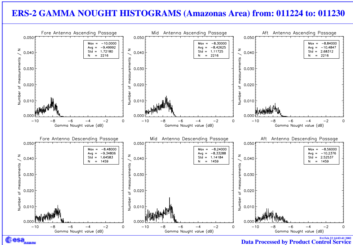
FIGURE 10. Gamma-nought histograms over Brazilian Rain forest: first week of the cycle 70.
