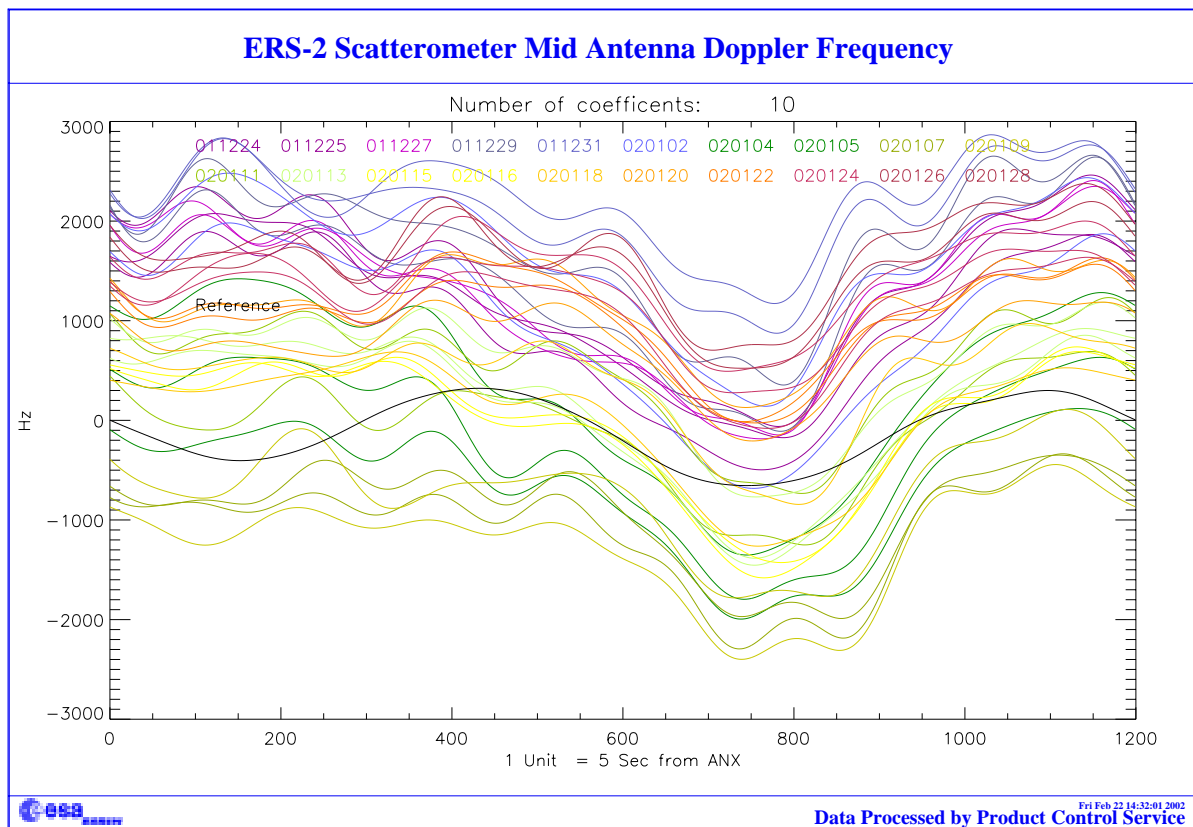
FIGURE 21. Low pass filtered evolution of the Mid beam CoG as function of ascending node time (1 unit 5 s.) cycle 70.
