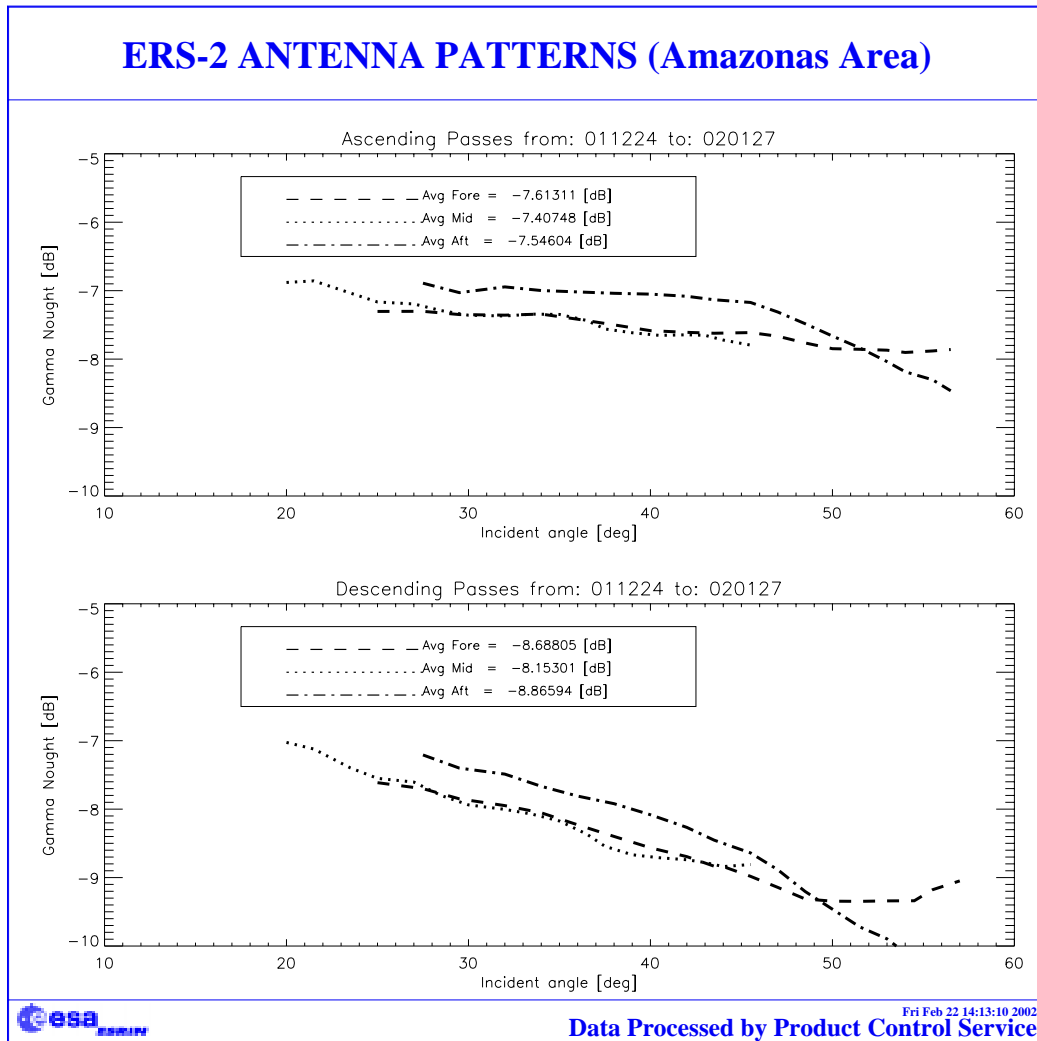
FIGURE 5. ERS-2 Scatterometer antenna patterns as function of the incidence angle: cycle 70.
