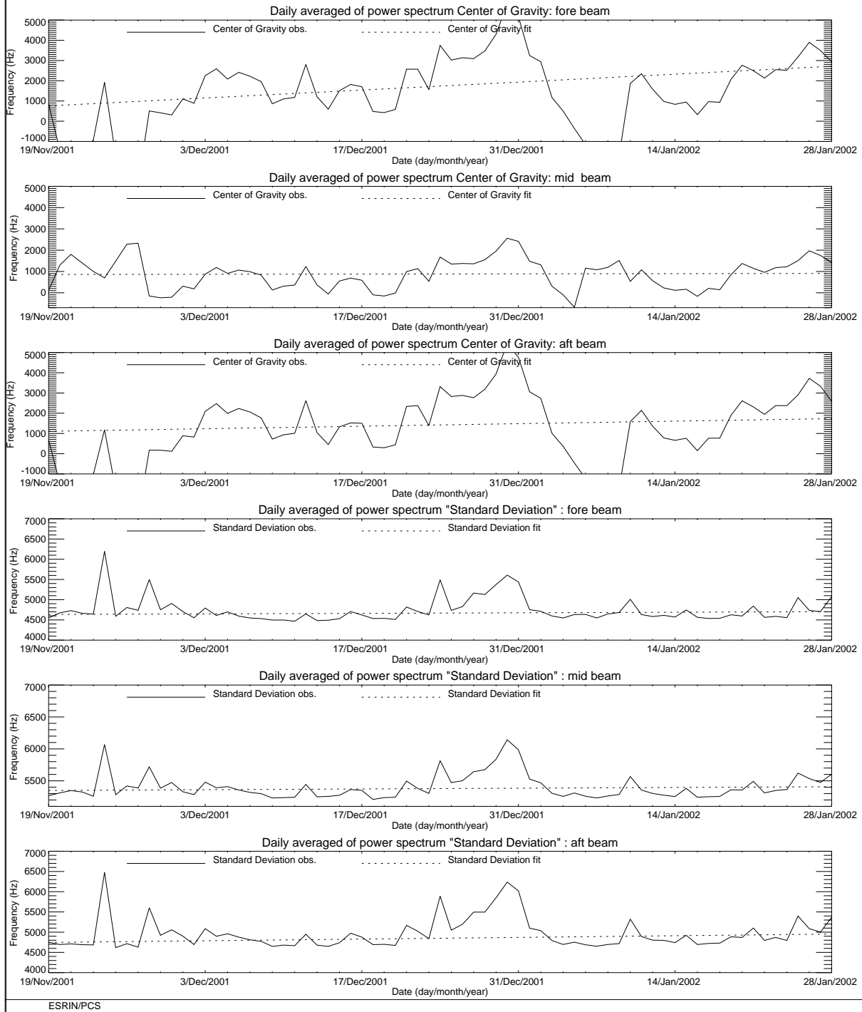
FIGURE 20. ERS-2 Scatterometer: Centre of Gravity and standard deviation of received power spectrum during the cycle 70.
