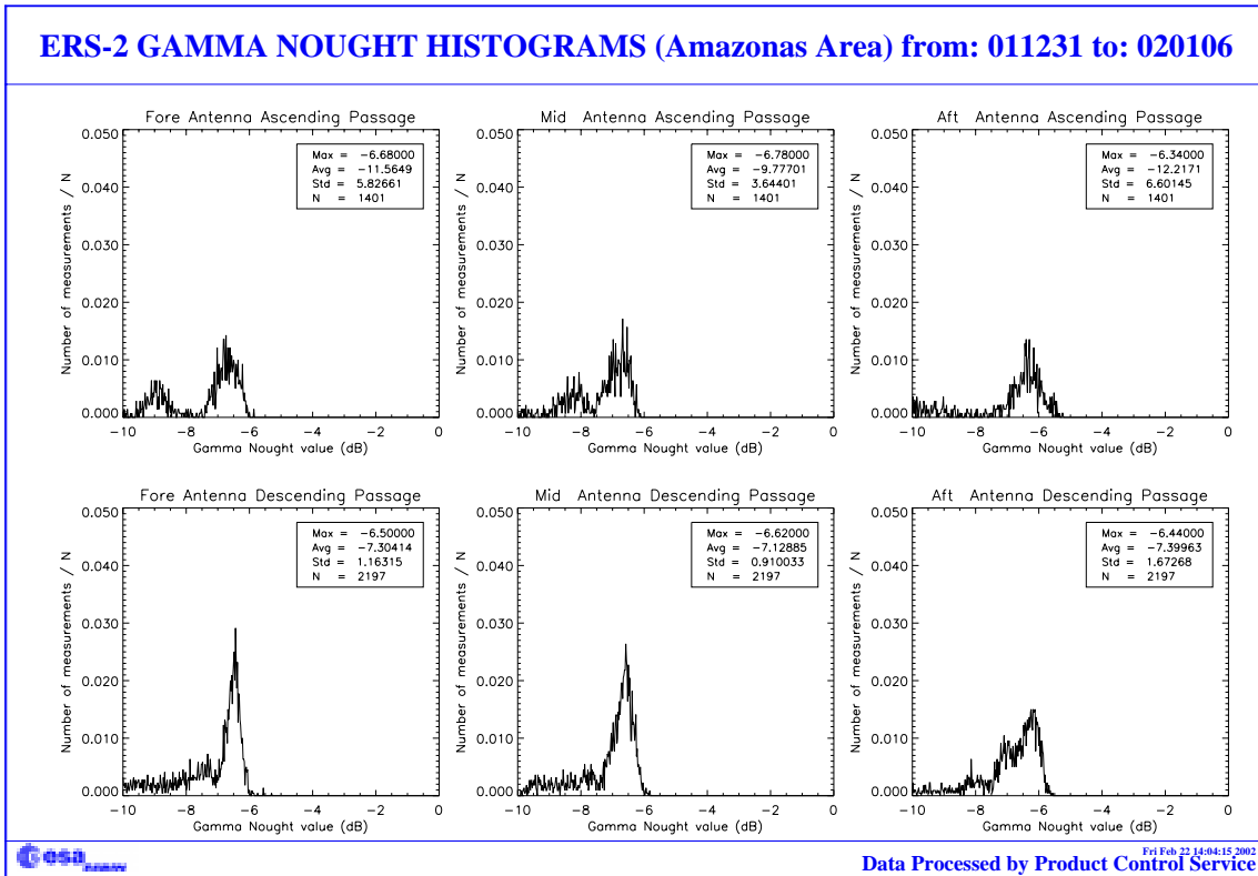
FIGURE 11. Gamma-nought histograms over Brazilian Rain forest: second week of the cycle 70.
