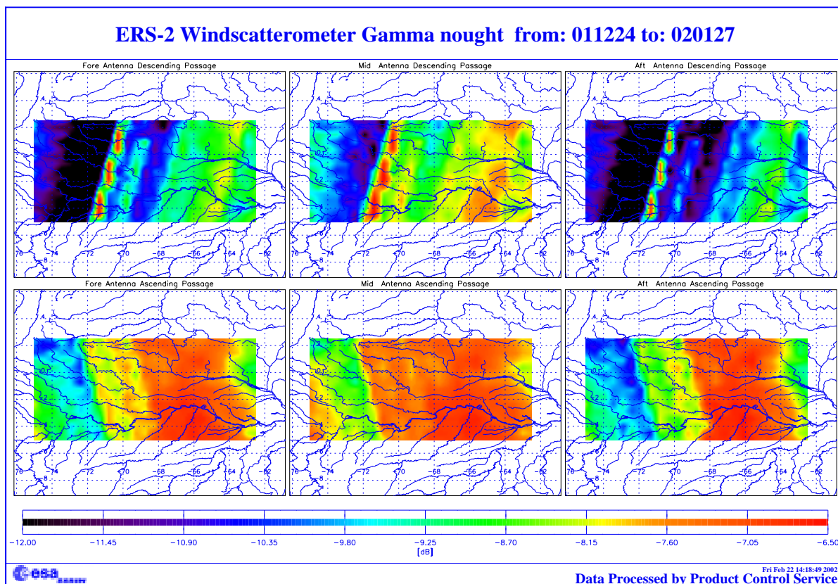
FIGURE 15. ERS-2 Scatterometer: gamma nought over the Brazilian rain forest cycle 70.
