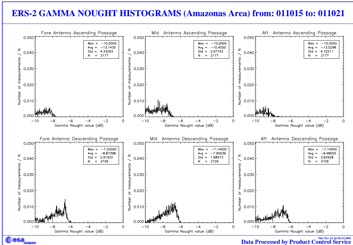
FIGURE 10. Gamma-nought histograms over Brazilian Rain forest: first week of the cycle 68.
