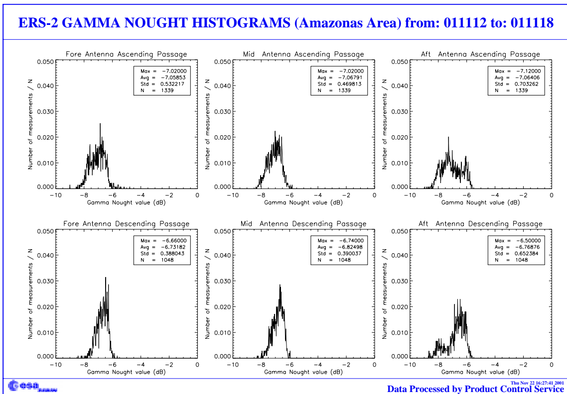
FIGURE 14. Gamma-nought histograms over Brazilian rain forest: fifth week of the cycle 68
