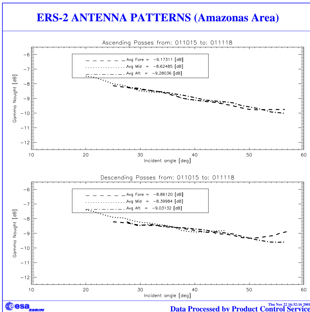
FIGURE 5. ERS-2 Scatterometer antenna patterns as function of the incidence angle: cycle 68.
