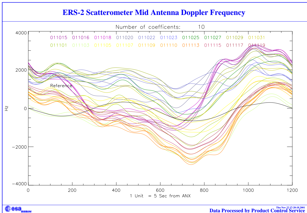
FIGURE 21. Low pass filtered evolution of the Mid beam CoG as function of ascending node time (1 unit 5 s.) cycle 68.
