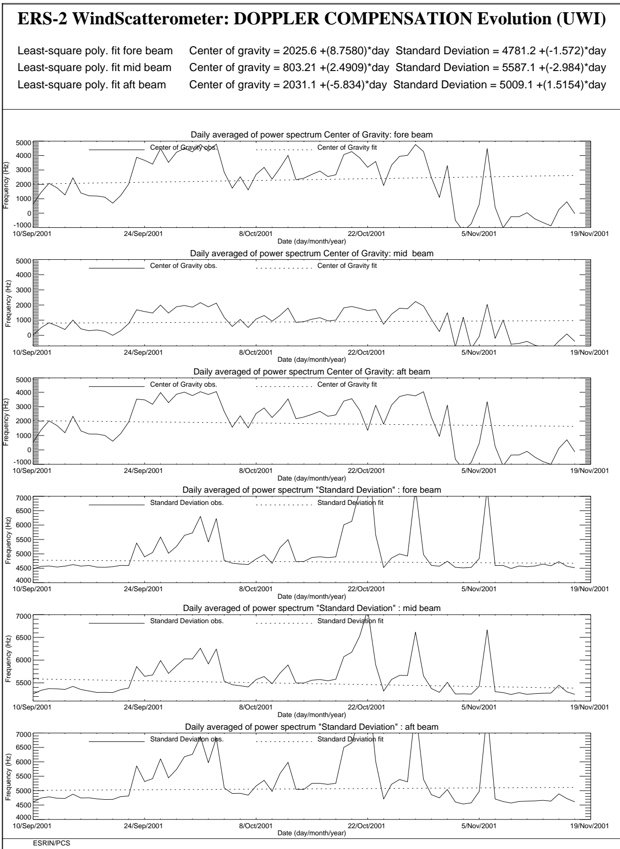
FIGURE 20. ERS-2 Scatterometer: Centre of Gravity and standard deviation of received power spectrum during the cycle 68.
