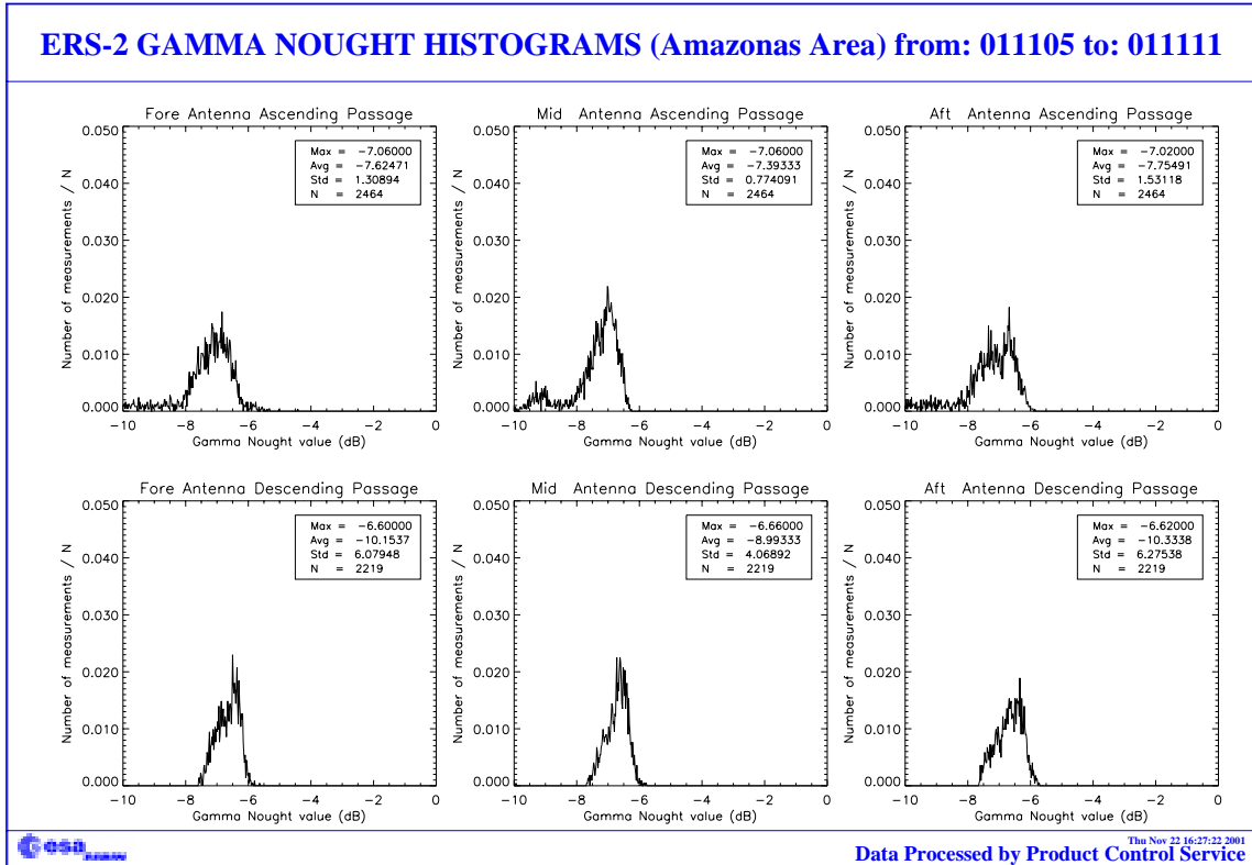
FIGURE 13. Gamma-nought histograms over Brazilian rain forest: fourth week of the cycle 68.
