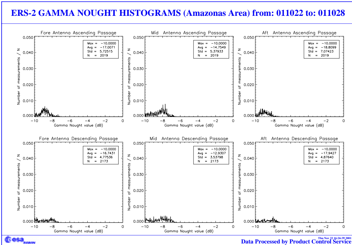
FIGURE 11. Gamma-nought histograms over Brazilian Rain forest: second week of the cycle 68.
