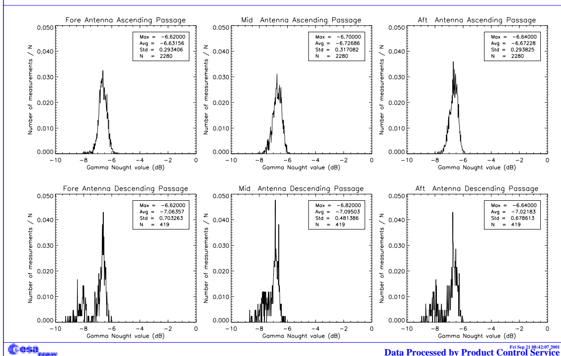
FIGURE 12. Gamma-nought histograms over Brazilian rain forest: third week of the cycle 66.
