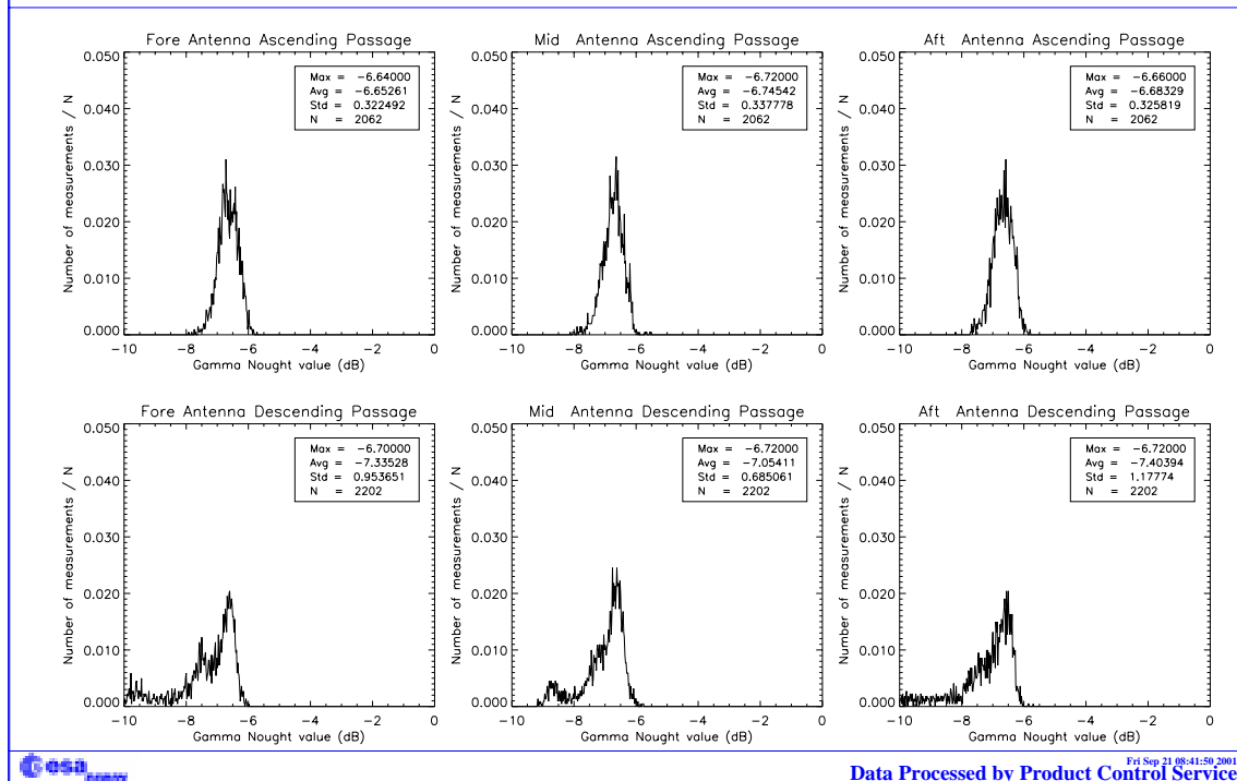
FIGURE 11. Gamma-nought histograms over Brazilian Rain forest: second week of the cycle 66.
