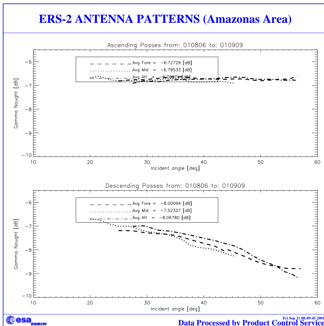
FIGURE 5. ERS-2 Scatterometer antenna patterns as function of the incidence angle: cycle 66.
