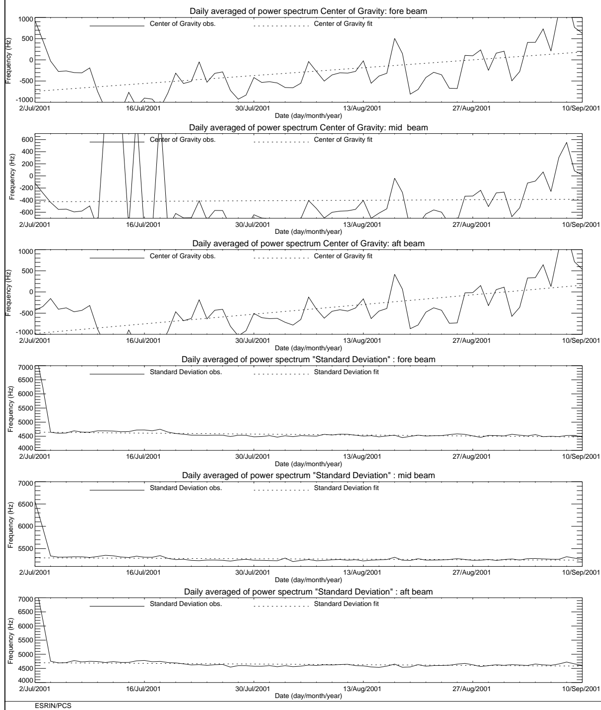
FIGURE 20. ERS-2 Scatterometer: Centre of Gravity and standard deviation of received power spectrum during the cycle 64 and cycle 66.
