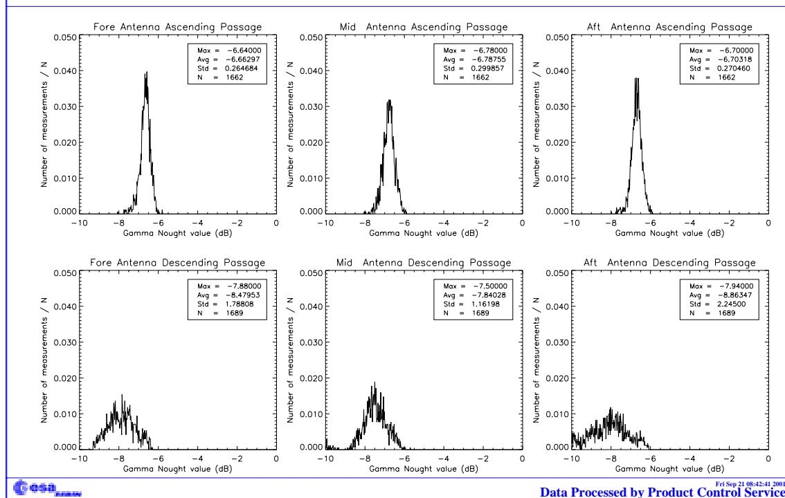
FIGURE 14. Gamma-nought histograms over Brazilian rain forest: fifth week of the cycle 66
