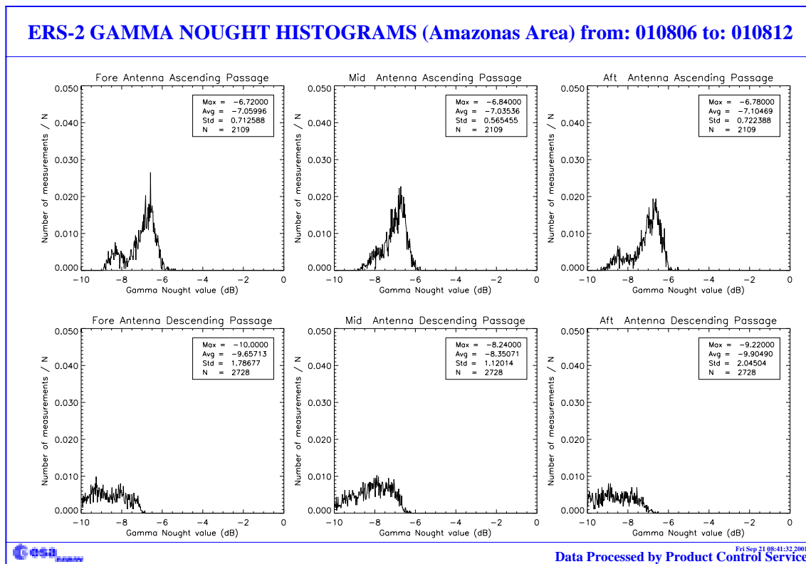
FIGURE 10. Gamma-nought histograms over Brazilian Rain forest: first week of the cycle 66.
