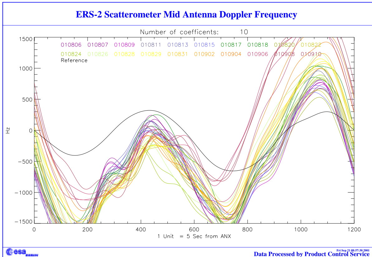
FIGURE 21. Low pass filtered evolution of the Mid beam CoG as function of ascending node time (1 unit 5 s.) cycle 66.
