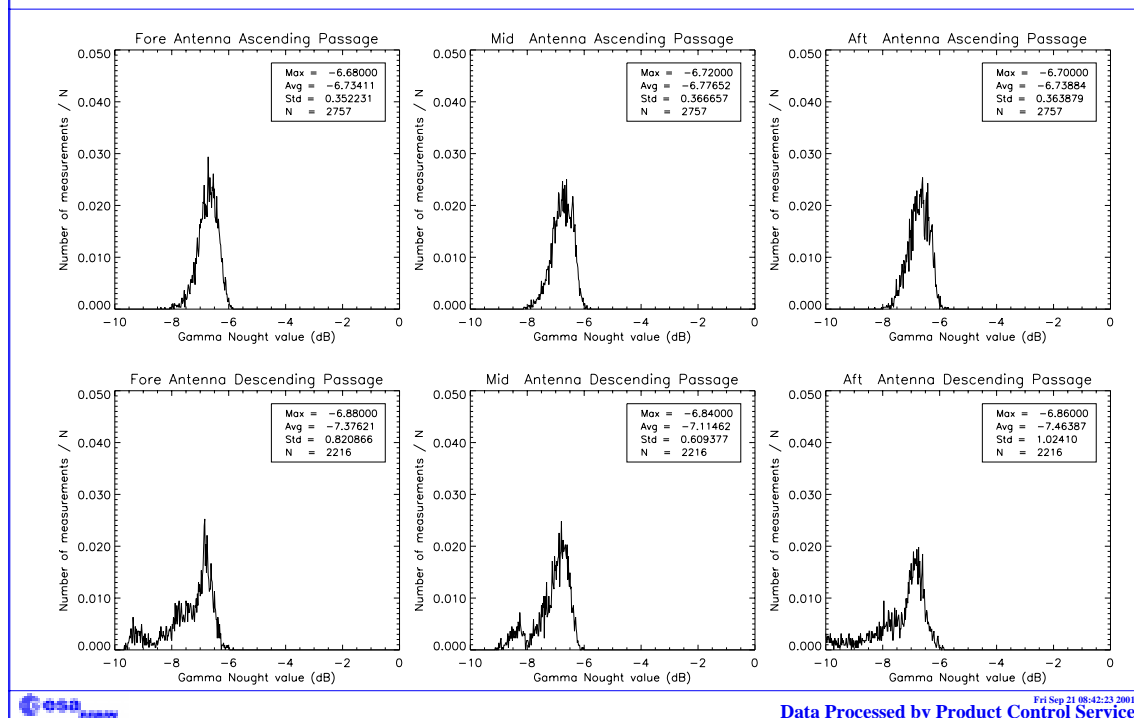
FIGURE 13. Gamma-nought histograms over Brazilian rain forest: fourth week of the cycle 66.
