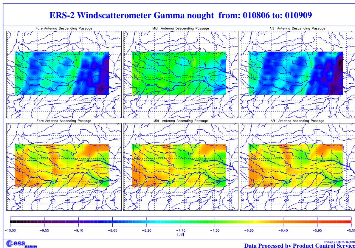
FIGURE 15. ERS-2 Scatterometer: gamma nought over the Brazilian rain forest cycle 66.
