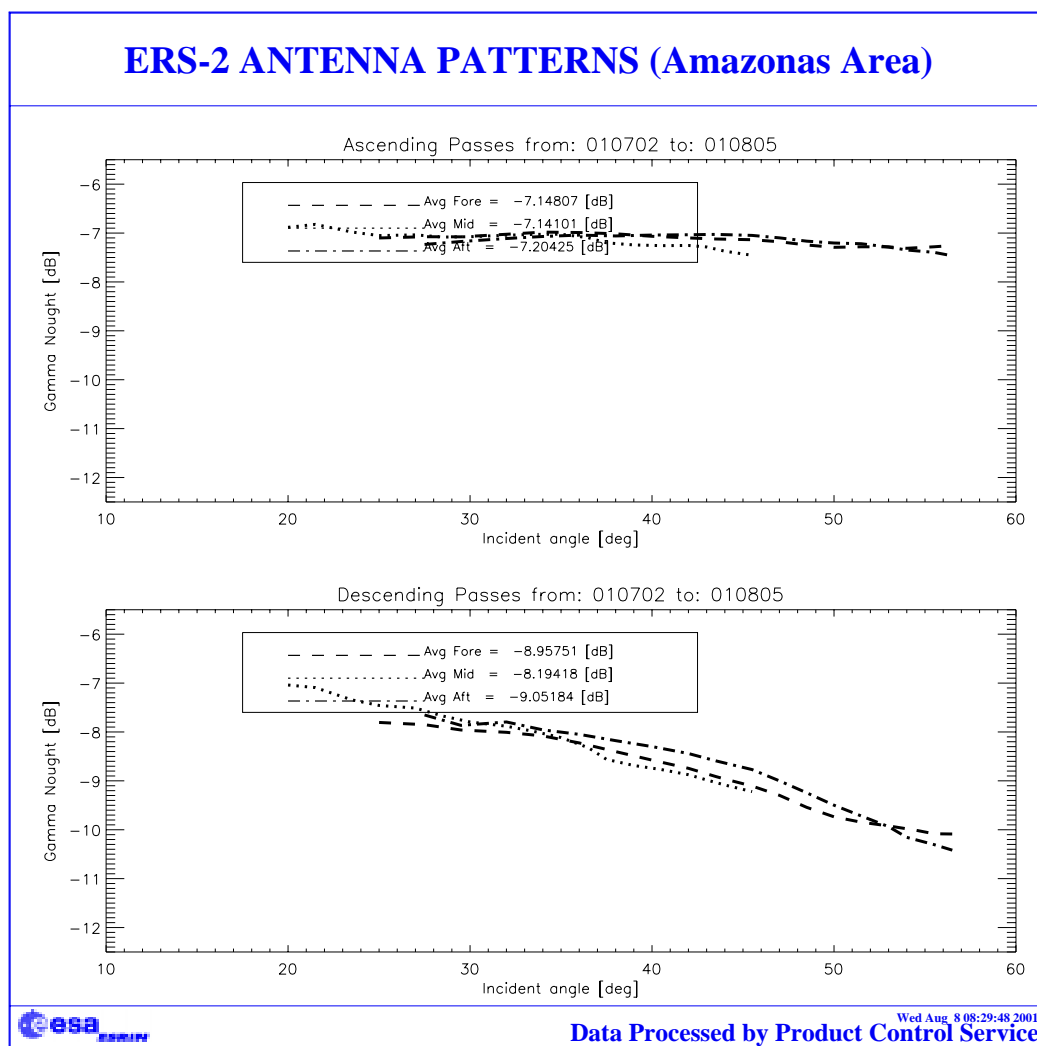
FIGURE 5. ERS-2 Scatterometer antenna patterns as function of the incidence angle: cycle 65.
