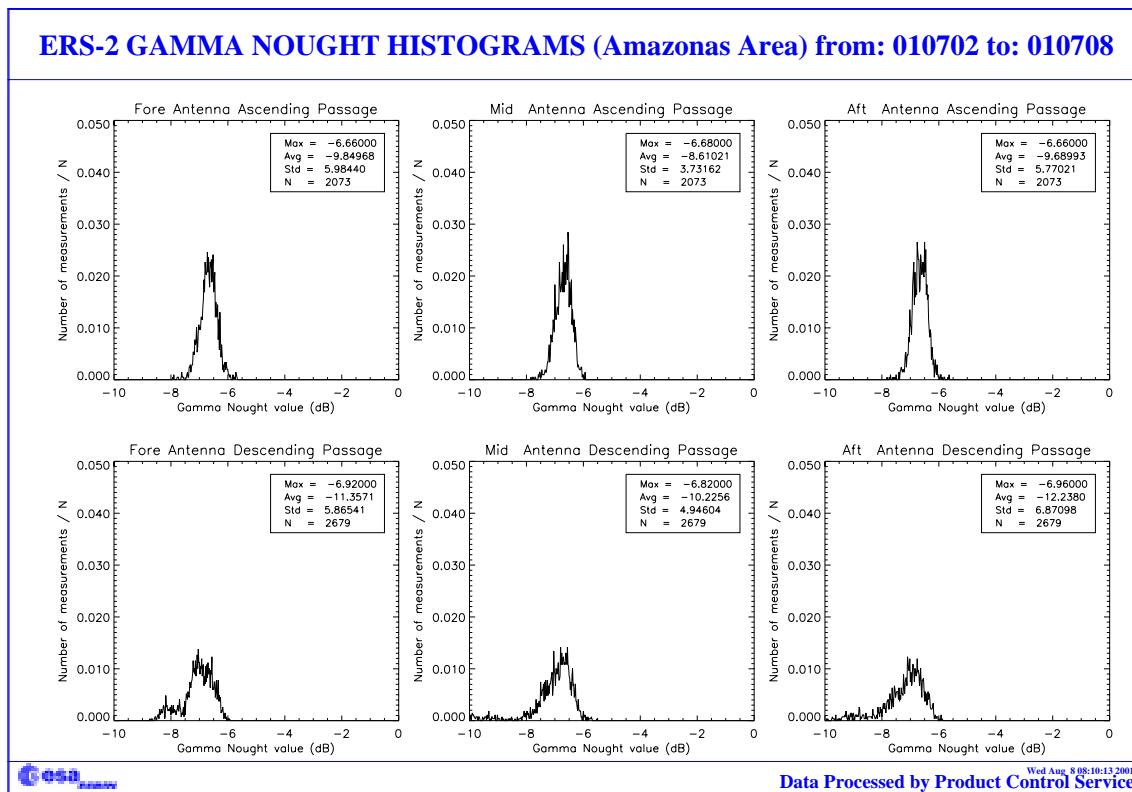
FIGURE 10. Gamma-nought histograms over Brazilian Rain forest: first week of the cycle 65.
