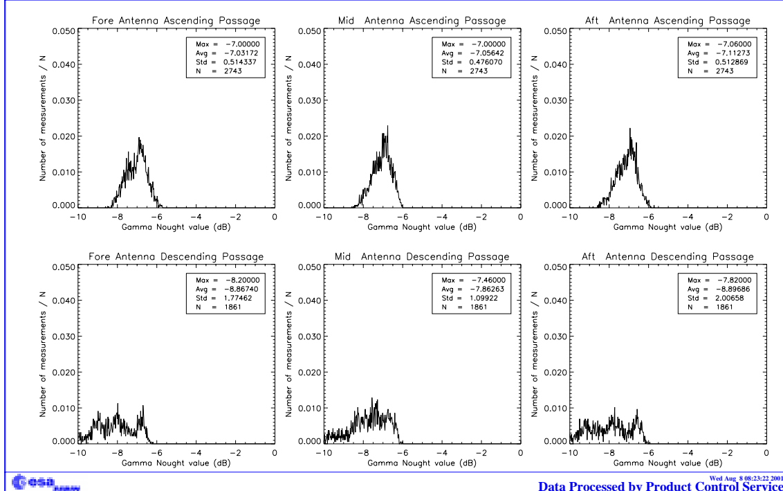
FIGURE 13. Gamma-nought histograms over Brazilian rain forest: fourth week of the cycle 65.
