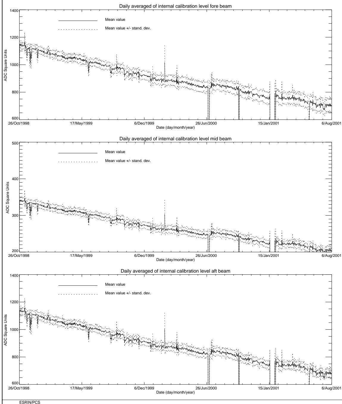
FIGURE 26. ERS-2 Scatterometer: power of internal calibration level since 26 th October 1998 when the transmitted power was increased by 2.0 dB.
