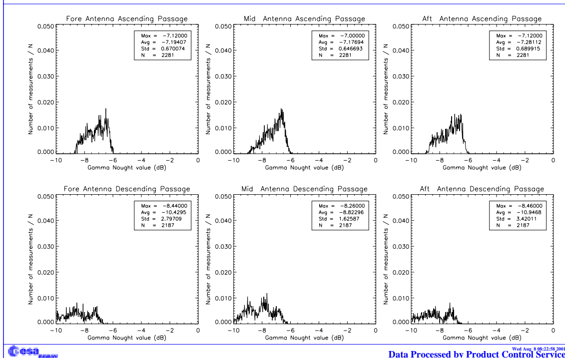
FIGURE 12. Gamma-nought histograms over Brazilian rain forest: third week of the cycle 65.
