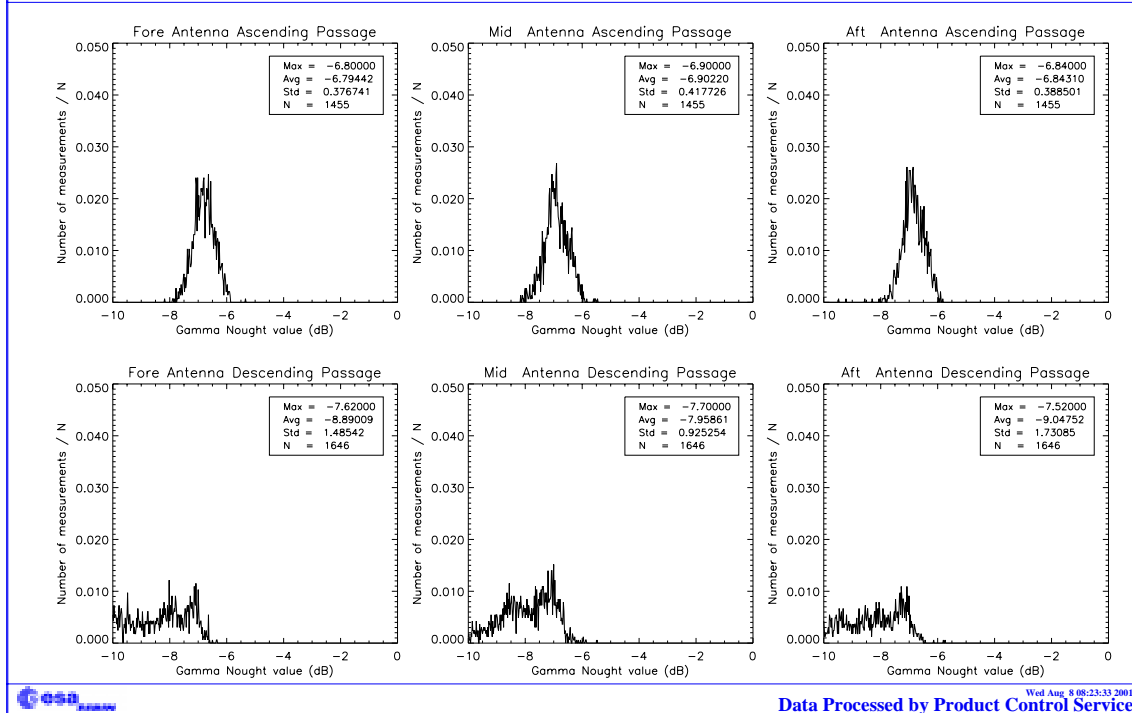
FIGURE 14. Gamma-nought histograms over Brazilian rain forest: fifth week of the cycle 65
