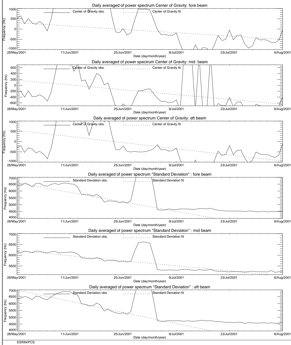
FIGURE 20. ERS-2 Scatterometer: Centre of Gravity and standard deviation of received power spectrum during the cycle 64 and cycle 65.
