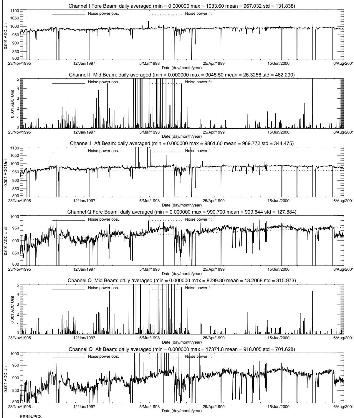
FIGURE 22. ERS-2 Scatterometer: noise power I and Q channel since the beginning of the mission.
