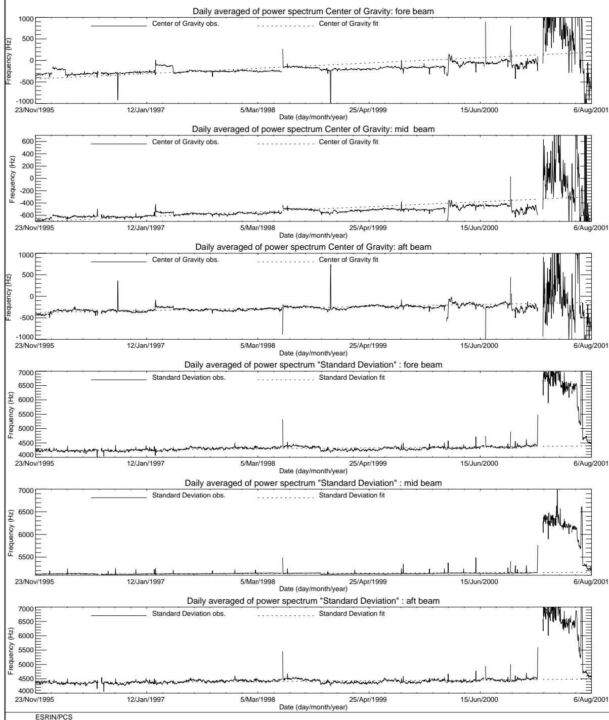
FIGURE 19. ERS-2 Scatterometer: Centre of Gravity and standard deviation of received power spectrum since the beginning of the mission.
