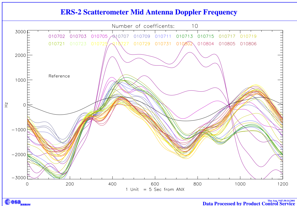
FIGURE 21. Low pass filtered evolution of the Mid beam CoG as function of ascending node time (1 unit 5 s.) Cycle 65.
