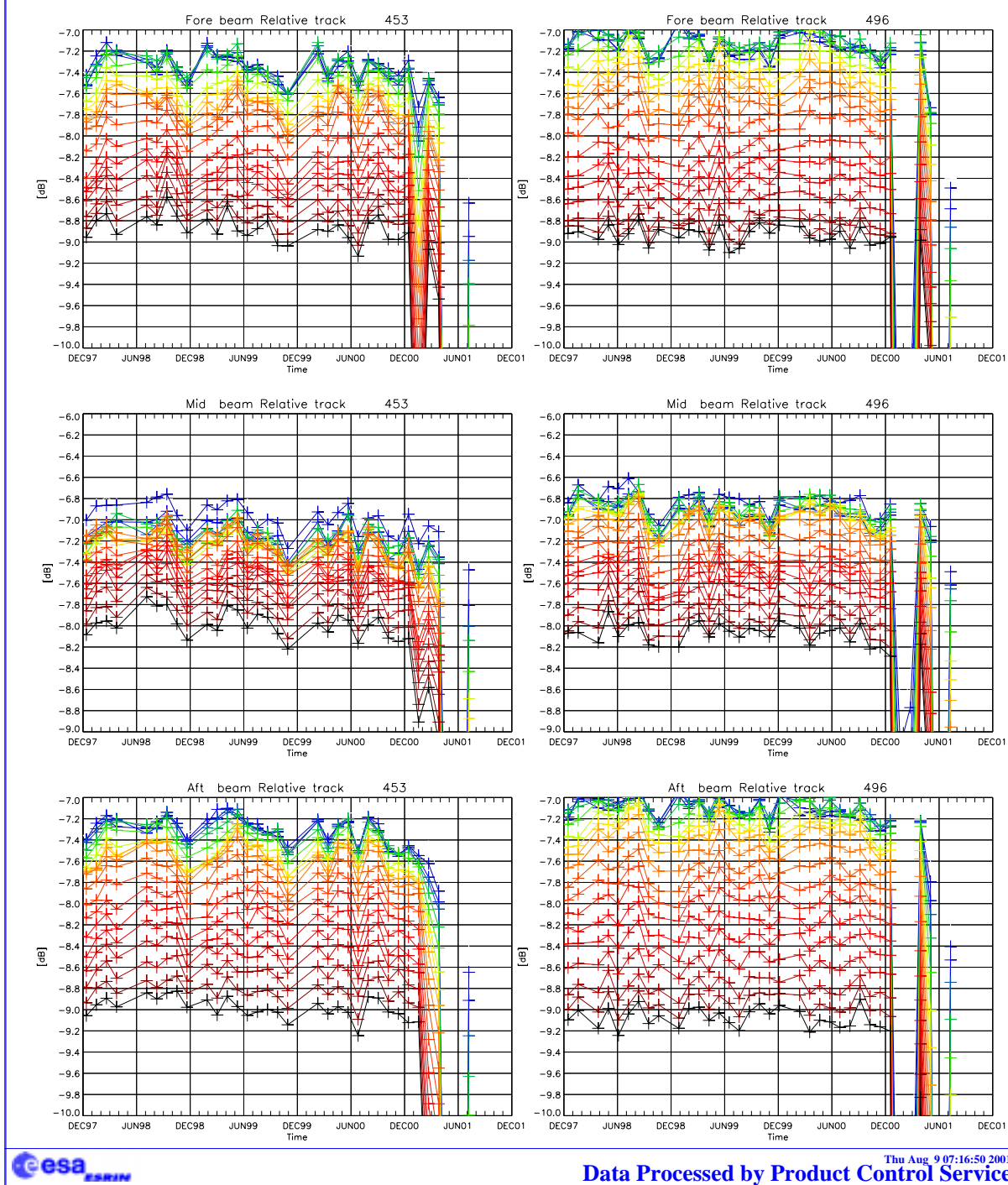
FIGURE 17. Sigma nought over the test area: descending passes relative tracks 453 (left panels) and 496 (right panels); all nodes across the swath (since December 1997).
