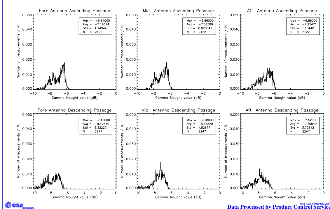
FIGURE 11. Gamma-nought histograms over Brazilian Rain forest: second week of the cycle 65.
