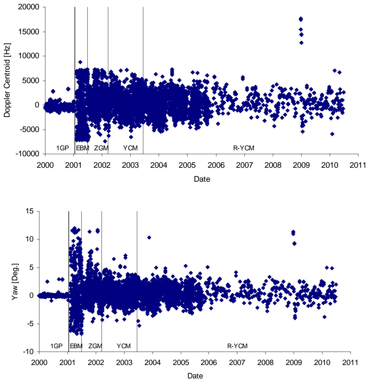
Figure 3.1. ERS-2 SAR Doppler Centroid (top) and Yaw (bottom) Evolution since January 2000
