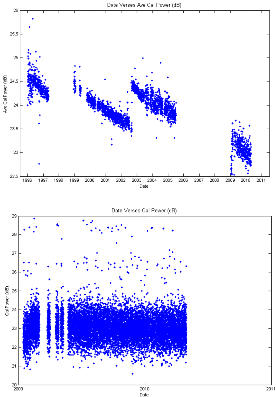
Figure 3.2 ERS-2 Wave Mode Calibration Pulse Power
