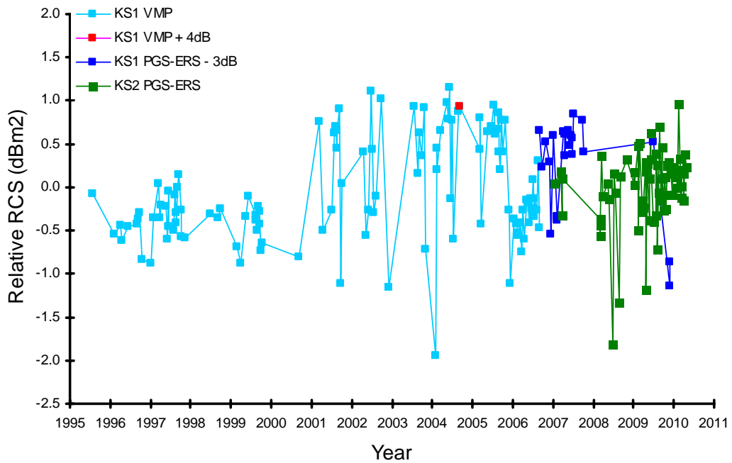
Figure 5.3. ERS-2 Kiruna ground station stability.
