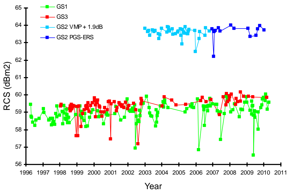
Figure 5.4. ERS-2 Neustrelitz ground station stability.
