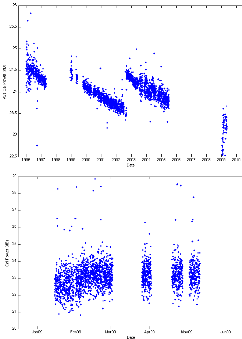
Figure 3.2 ERS-2 Wave Mode Calibration Pulse Power
