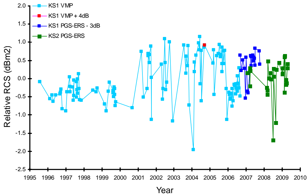
Figure 5.3. ERS-2 Kiruna ground station stability.
