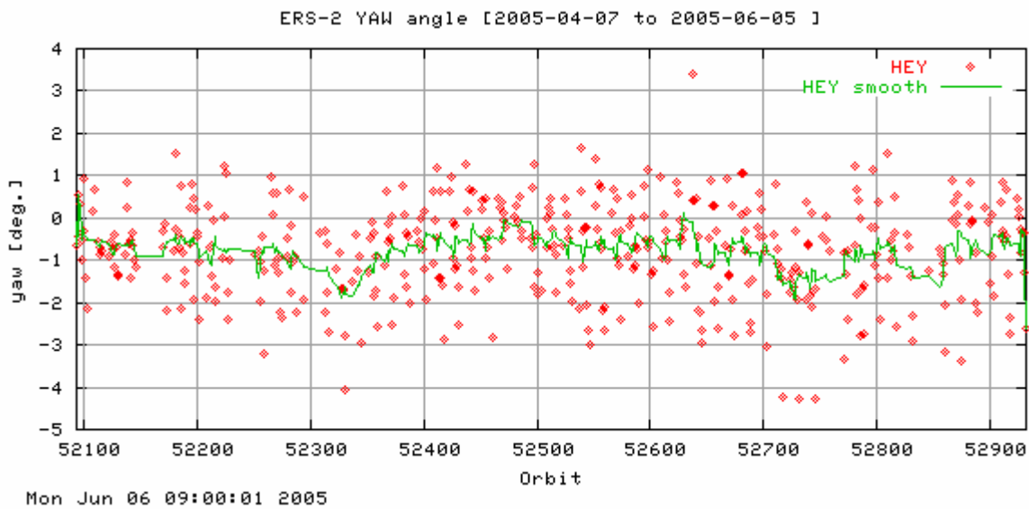
Figure 17: Mean yaw angle/orbit derived from HEY data since 03-Feb-2004
