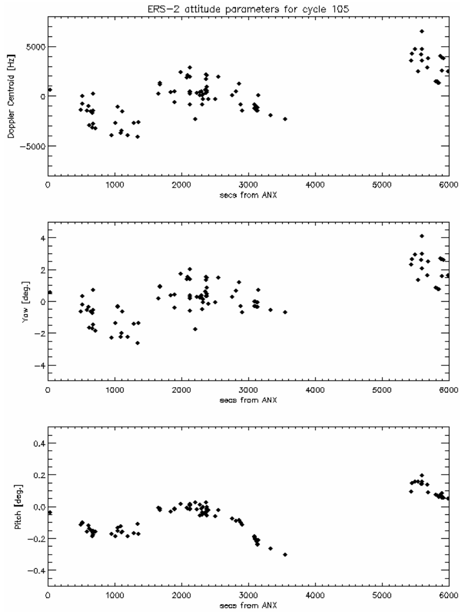
Figure 18: SAR Doppler and yaw evolution wrt elapsed seconds since the ANX
