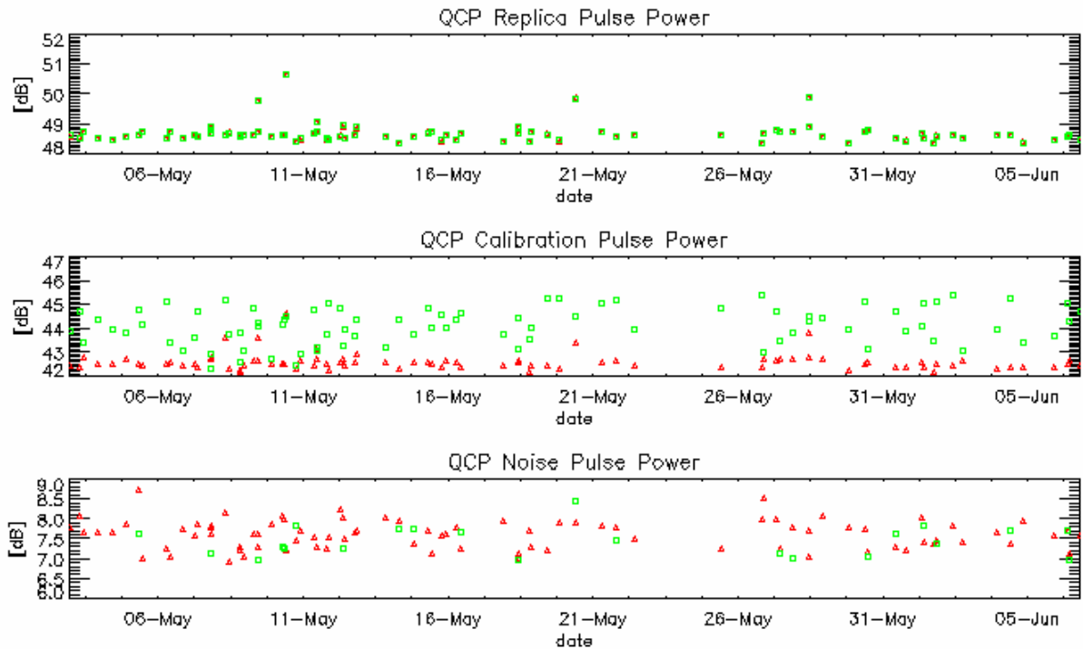
Figure 11: Evolution of Replica, calibration and noise pulses from QCP files for the current cycle
