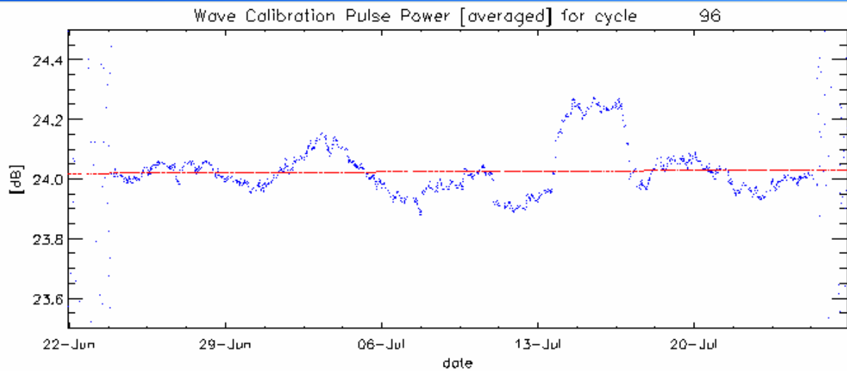
Figure 13: Evolution of Mean Calibration Pulse Power since for the current cycle
