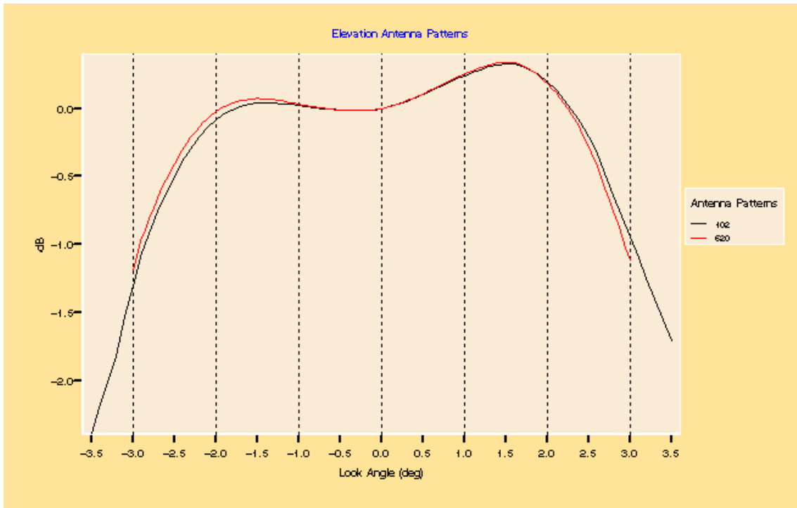
Figure 3: Antenna pattern combination (red curve) plus reference pattern (black curve) for descending passes
