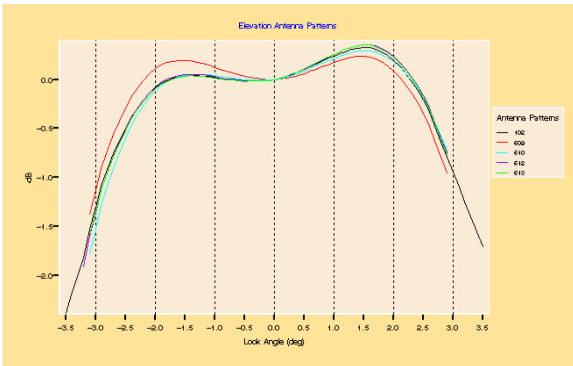
Figure 2: Antenna patterns derived from the selected ascending passes plus reference pattern (in black)
