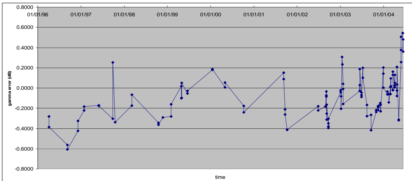
Figure 7: Gamma error up to cycle 95
