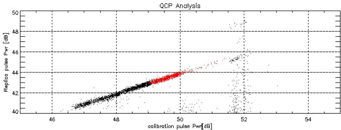
Figure 11: Joint evolution of Replica and calibration pulses. Black dots represent all the data since. Red ones are the data since the last gain increase.
