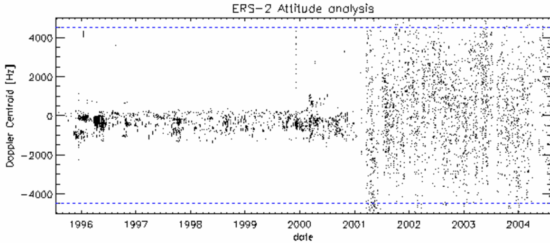
Figure 15: Evolution of Doppler Centroid Frequency since the beginning of the mission
