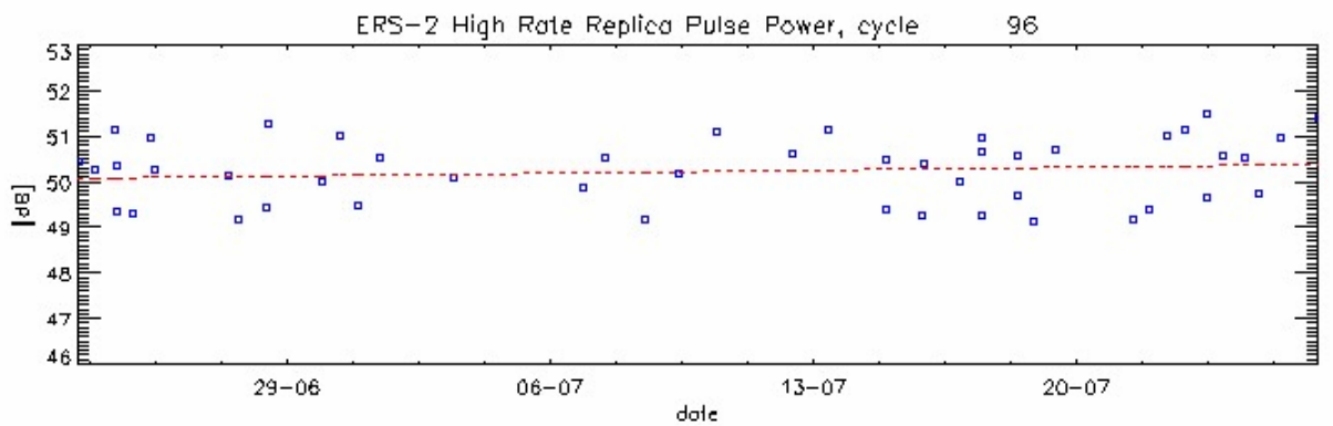
Figure 9: Evolution of replica pulse power since gain increase
