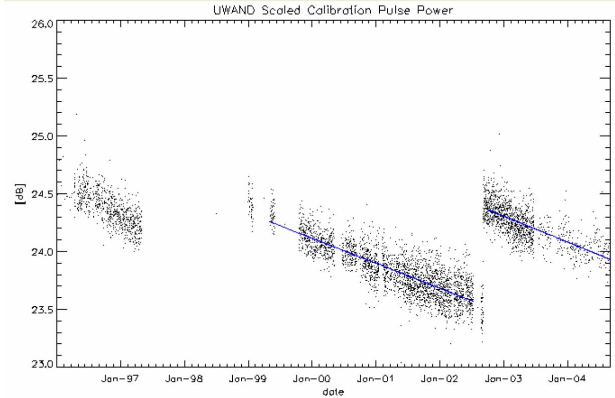
Figure 12: Evolution of Mean Calibration Pulse
