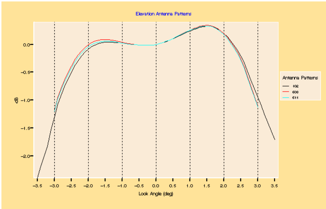
Figure 1: Antenna patterns derived from the selected descending pass plus reference pattern (in black)
