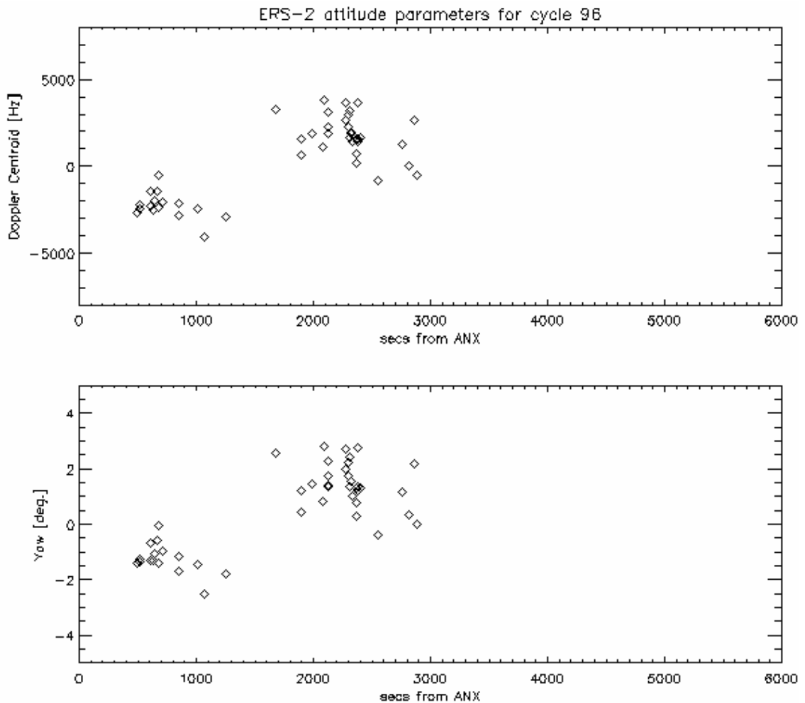
Figure 17: SAR HR Doppler Centroid evolution in time for versus seconds from ANX
