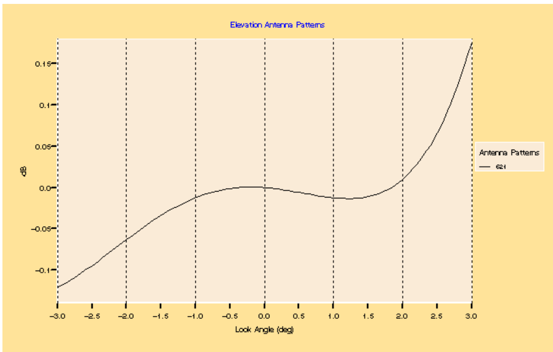
Figure 4: Difference between the reference pattern and the patterns combination for descending passes
