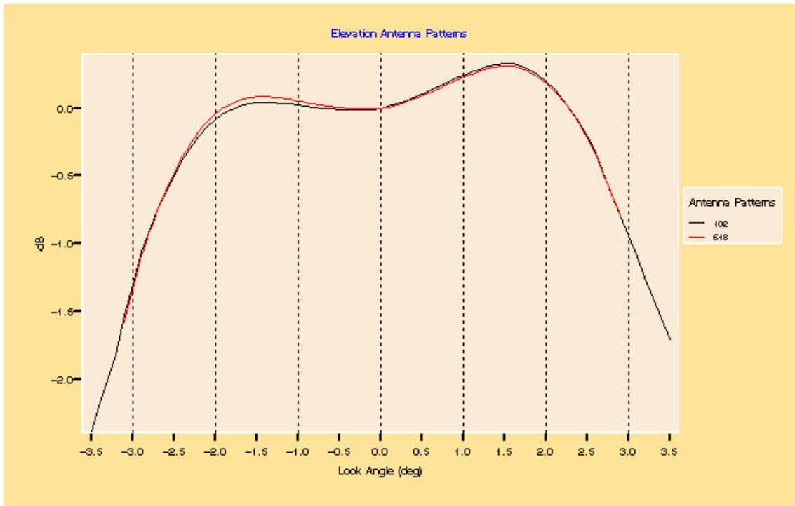
Figure 5: Antenna patterns combination (red curve) plus reference pattern (black curve) for ascending passes
