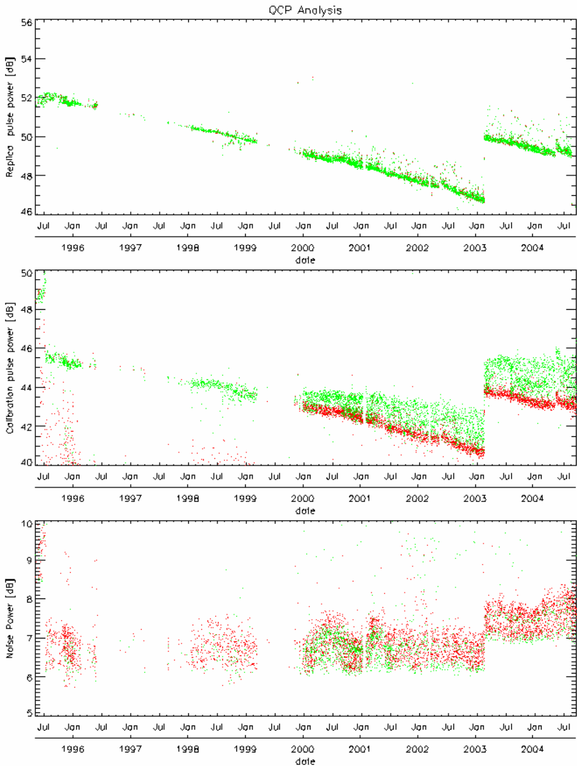
Figure 10: Evolution of Replica, calibration and noise pulses from QCP files. Red points are for the measures at the beginning of the product, while green are the ones at the end.
