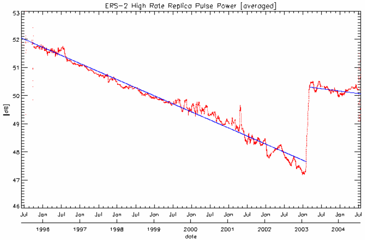
Figure 8: Evolution of Replica pulse power for High Rate products
