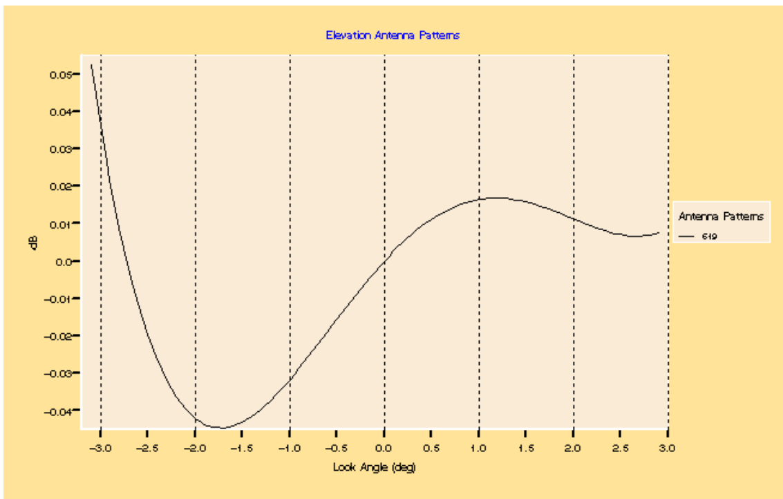
Figure 6: Difference between the reference pattern and the pattern combination for ascending passes
