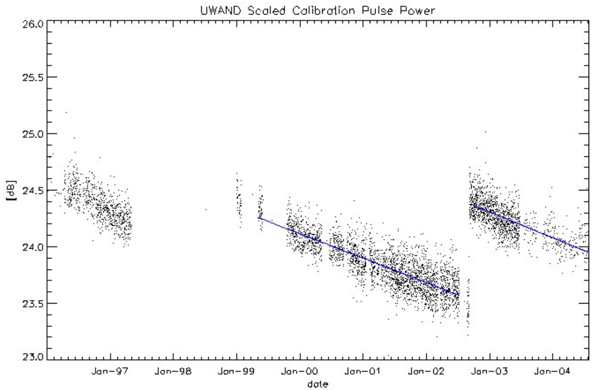
Figure 10: Evolution of Mean Calibration Pulse
