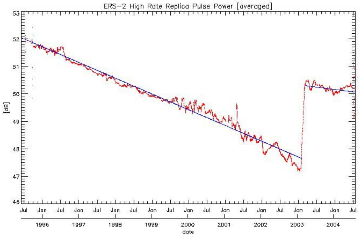
Figure 6: Evolution of Replica pulse power for High Rate products
