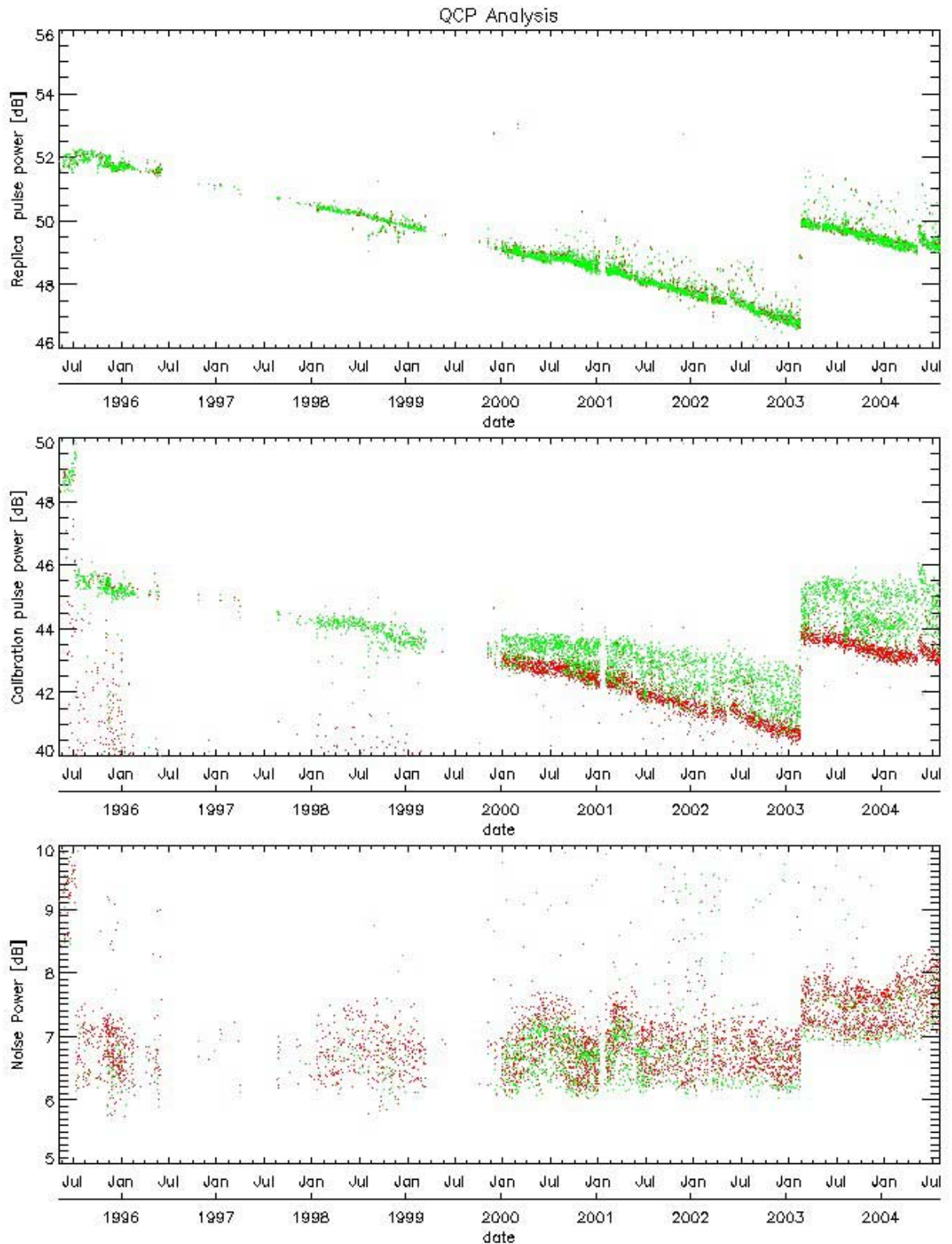
Figure 8: Evolution of Replica, calibration and noise pulses from QCP files. Red points are for the measures at the beginning of the product, while green are the ones at the end.
