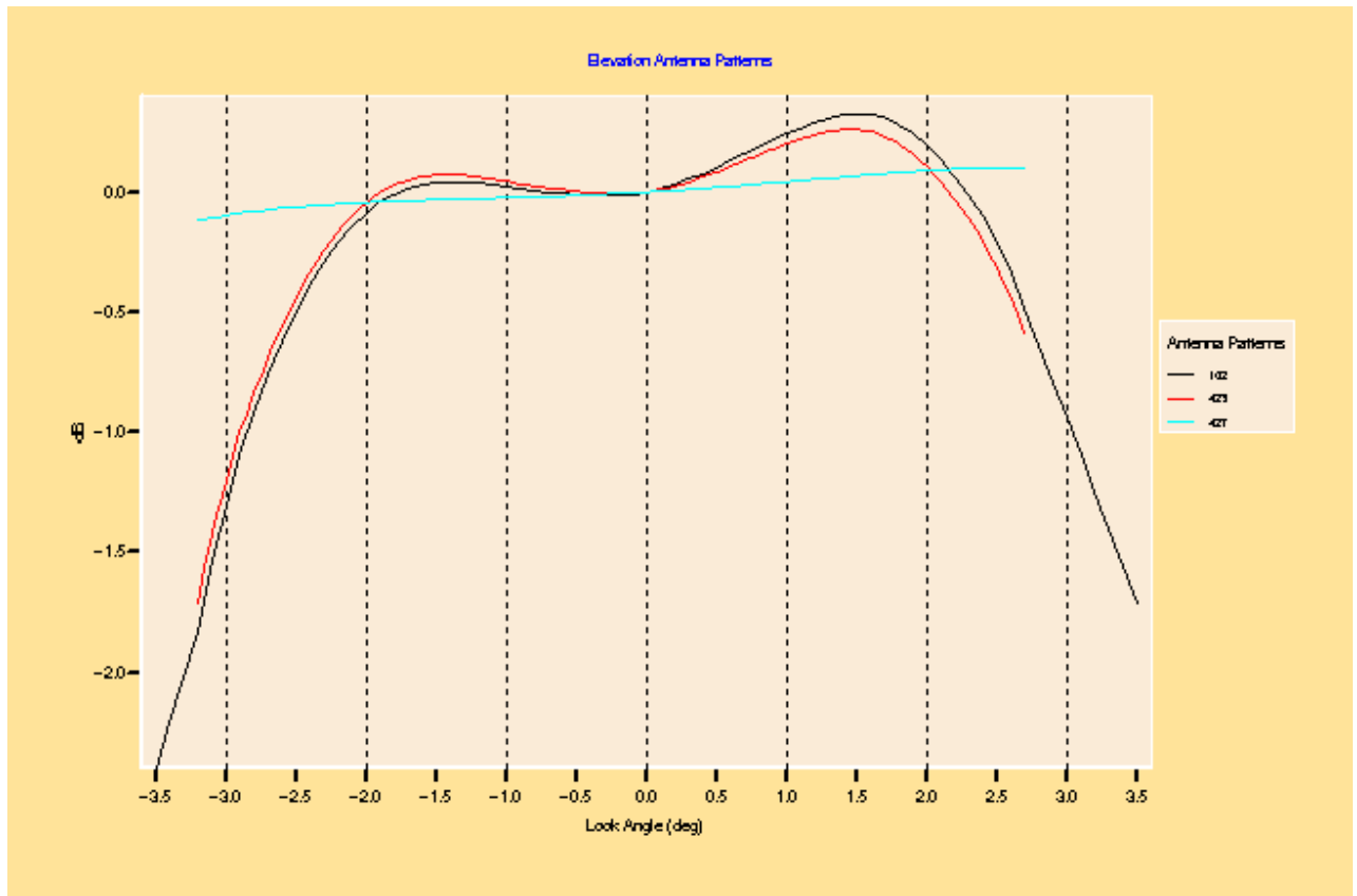
Figure 4: Antenna pattern combination (red curve) plus reference pattern (black curve) plus difference (blue curve) for ascending passes
