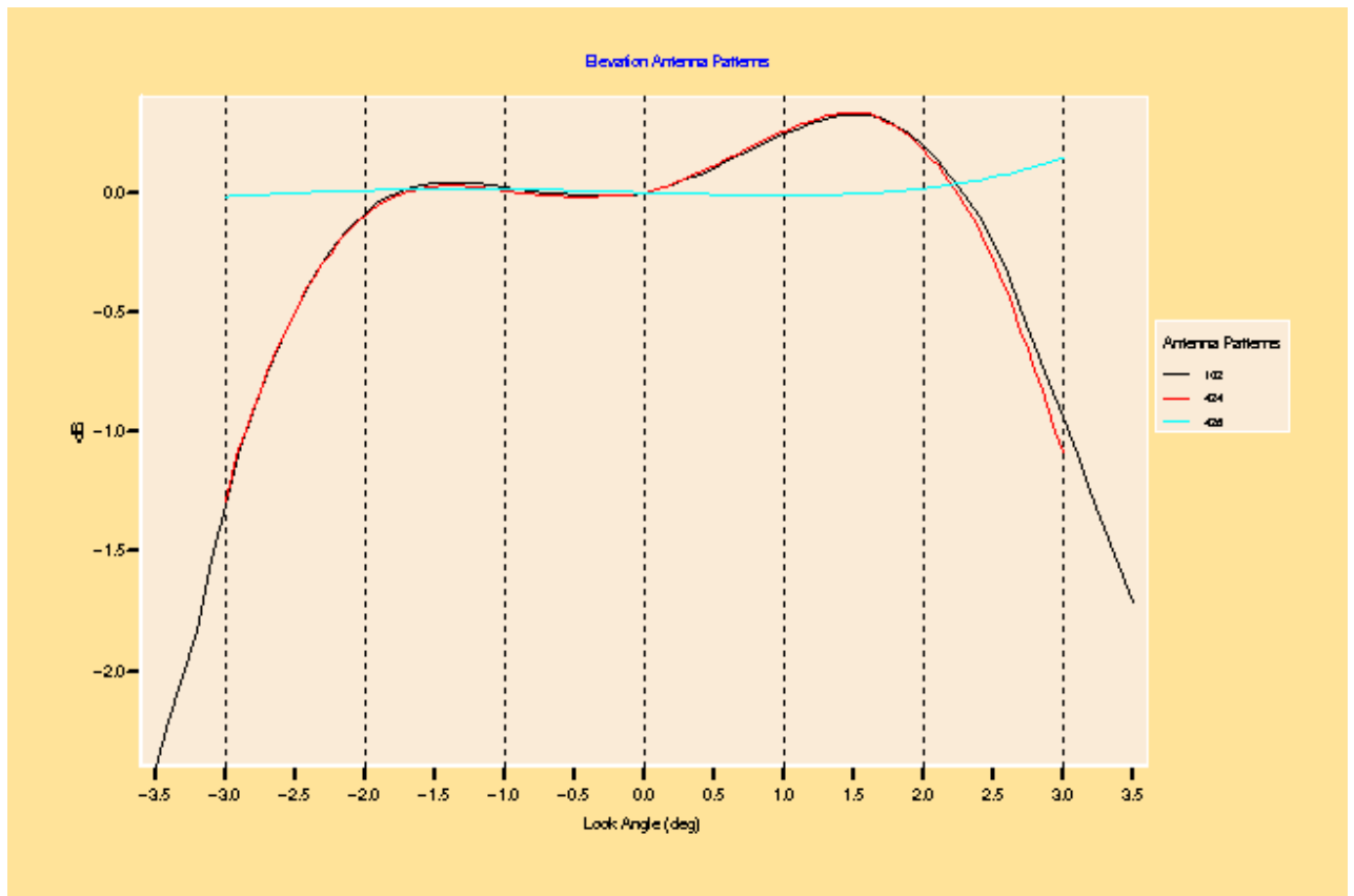
Figure 3: Antenna pattern combination (red curve) plus reference pattern (black curve) plus difference (blue curve) for descending passes
