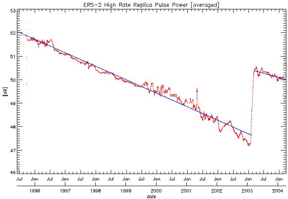
Figure 6: Evolution of Replica pulse power for High Rate products
