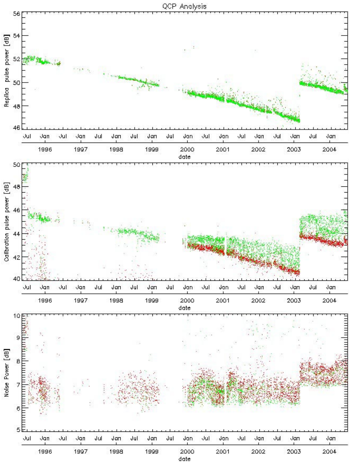
Figure 8: Evolution of Replica, calibration and noise pulses from QCP files. Red points are for the measures at the beginning of the product, while green are the ones at the end.
