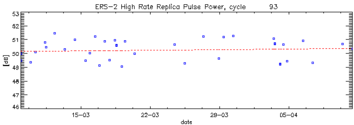
Figure 7: Evolution of replica pulse power since gain increase
