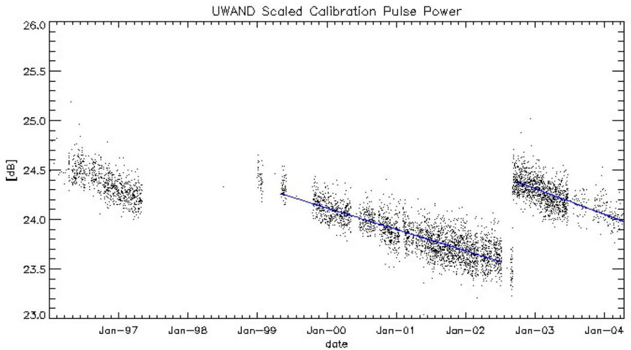
Figure 10: Evolution of Mean Calibration Pulse
