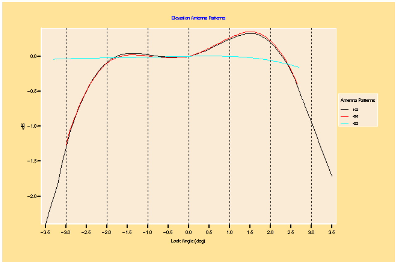
Figure 3: Antenna pattern combination (black curve) plus reference pattern (red curve) plus difference (blue curve) for all passes
