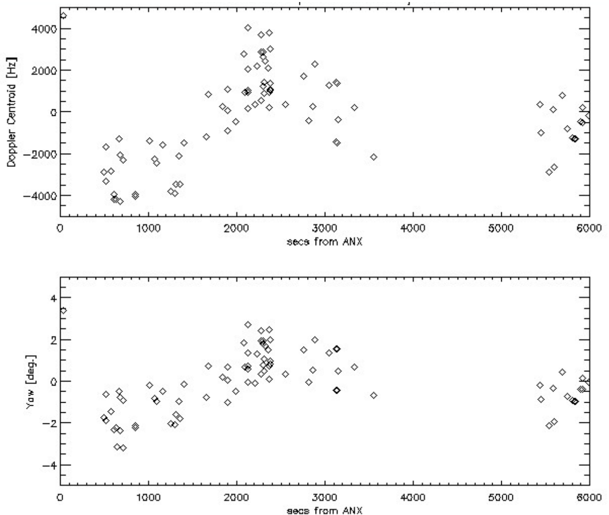
Figure 14: SAR HR Doppler Centroid evolution in time for versus seconds from ANX
