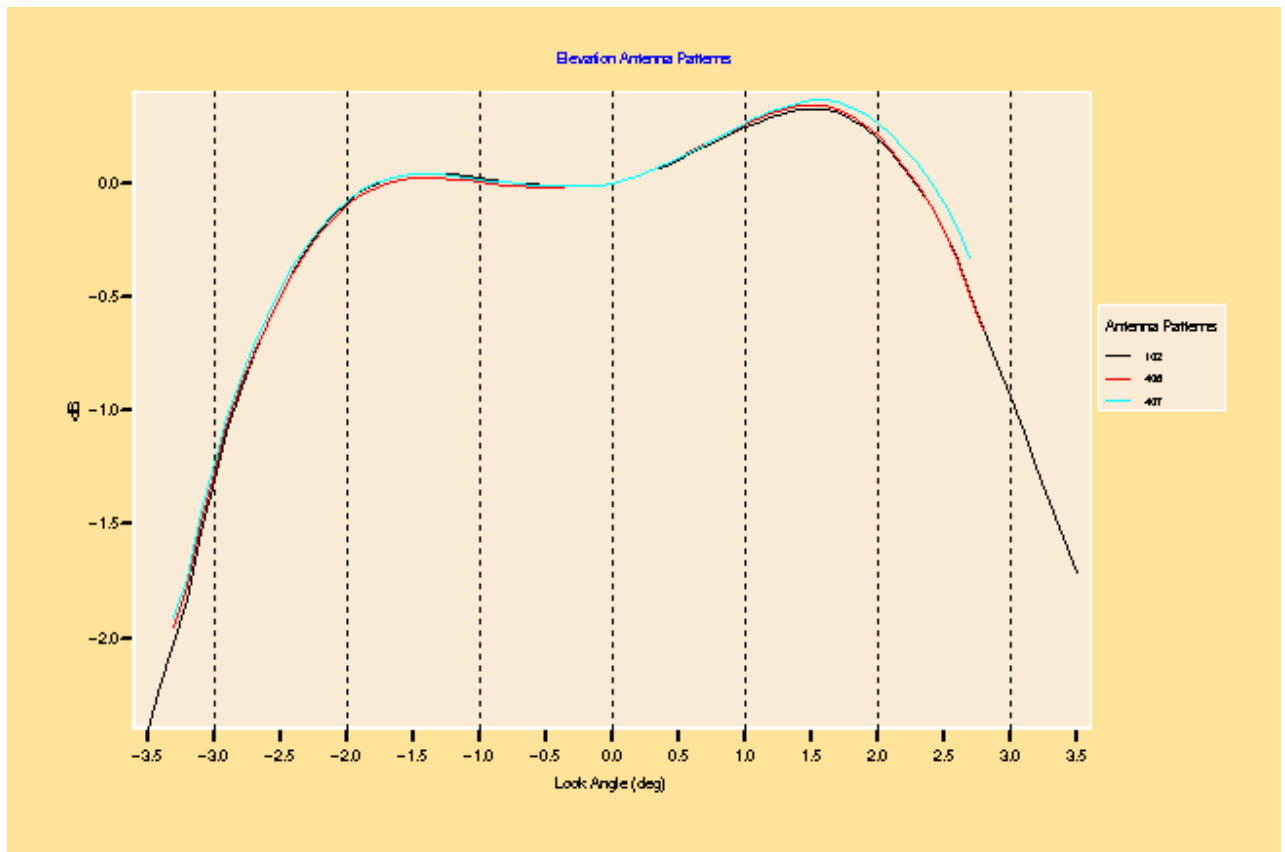
Figure 2: Antenna patterns derived from the selected ascending passes
