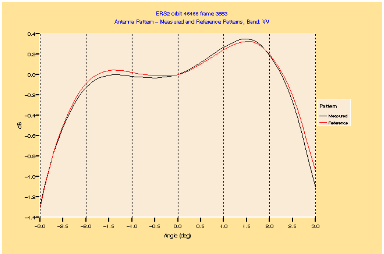
Figure 1: : Antenna patterns derived from the selected descending pass
