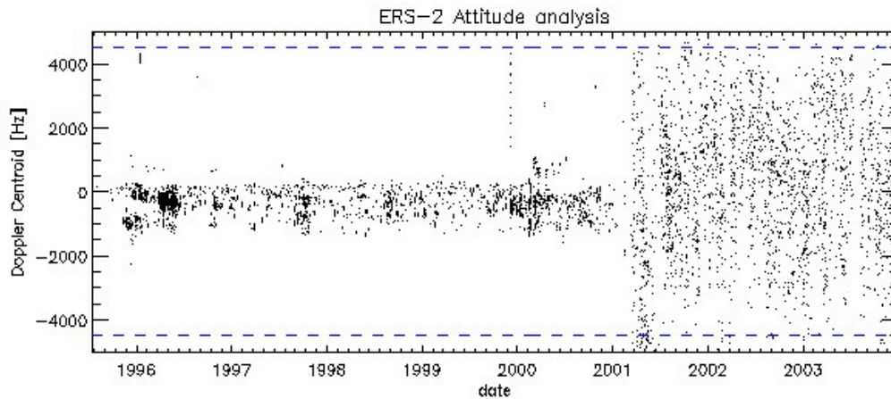
Figure 12: Evolution of Doppler Centroid Frequency since the beginning of the mission
