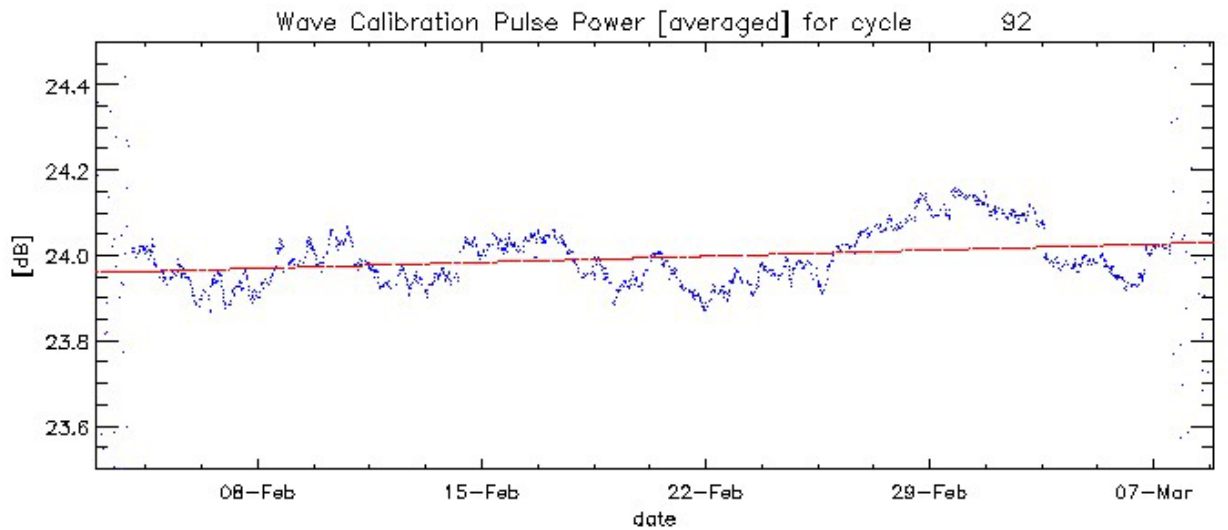
Figure 10: Evolution of Mean Calibration Pulse Power since for the current cycle
