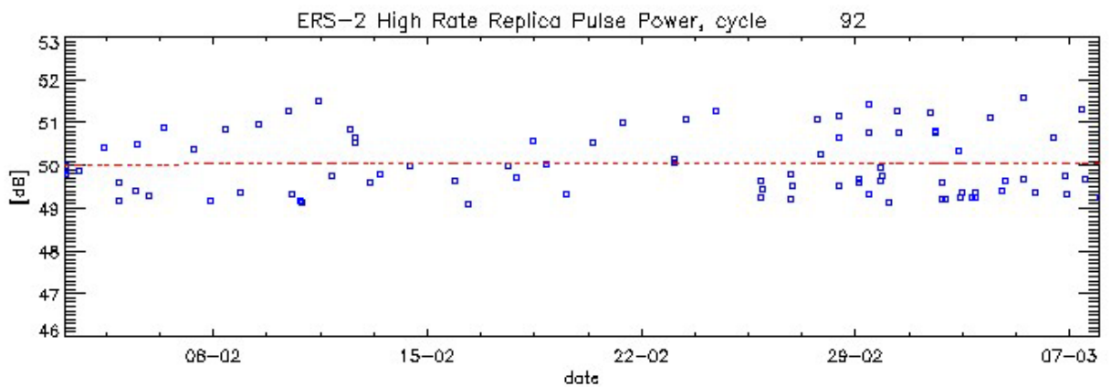
Figure 6: Evolution of replica pulse power since gain increase
