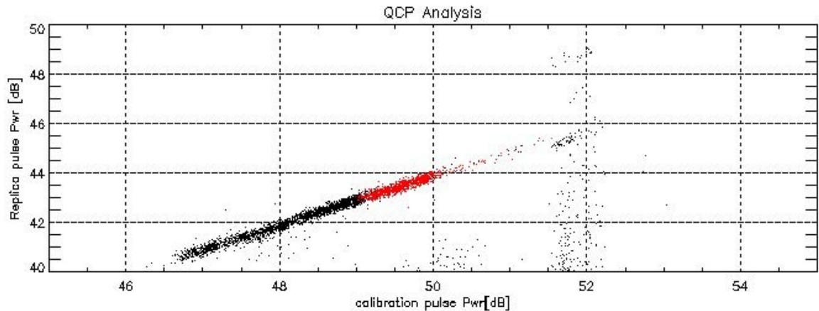
Figure 8: Joint evolution of Replica and calibration pulses. Black dots represent all the data since. Red ones are the data since the last gain increase.
