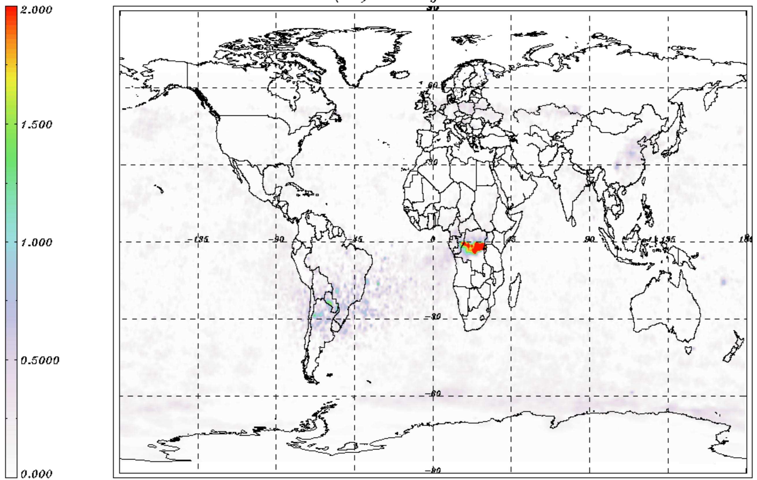
S02 UV7 VCD (DU) monthly mean - November 2011
