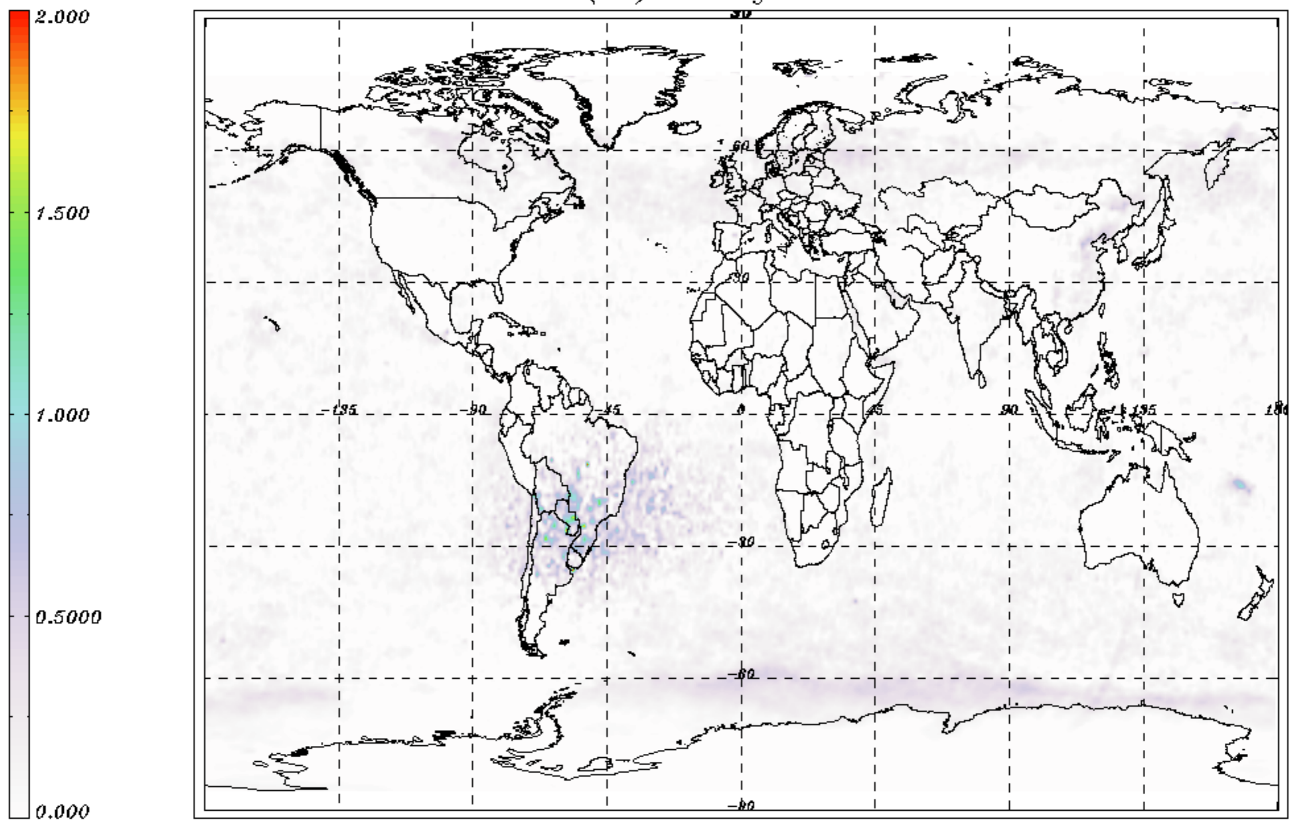
S02 UV7 VCD (DU) monthly mean - October 2011
