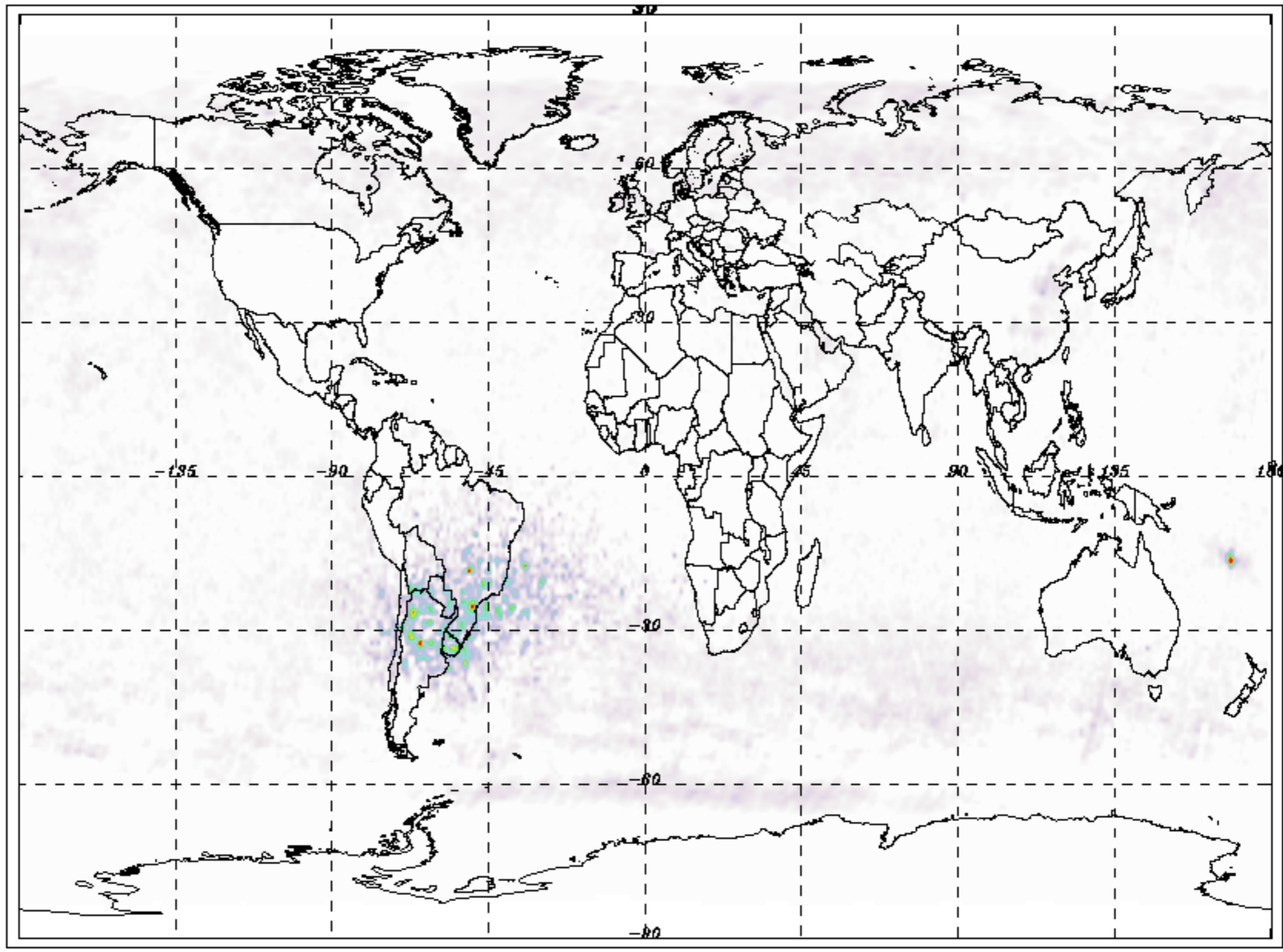
SO2 UV7 VCD (DU) monthly mean - September 2011
