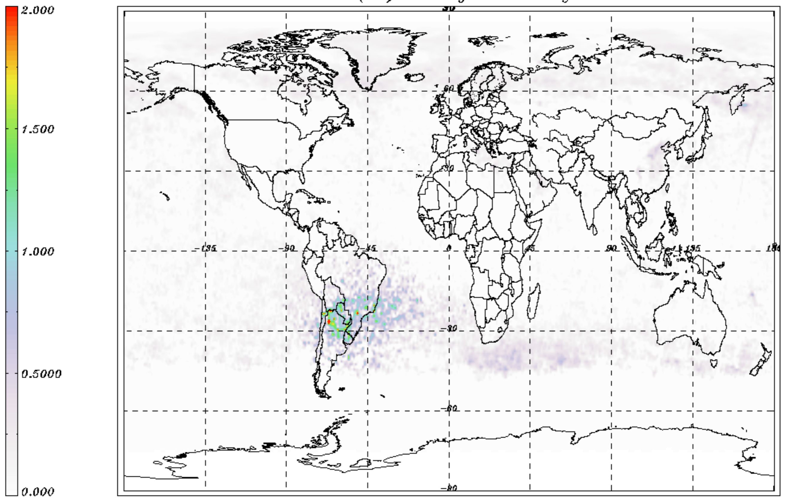
S02 UV7 VCD (DU) monthly mean - August 2011
