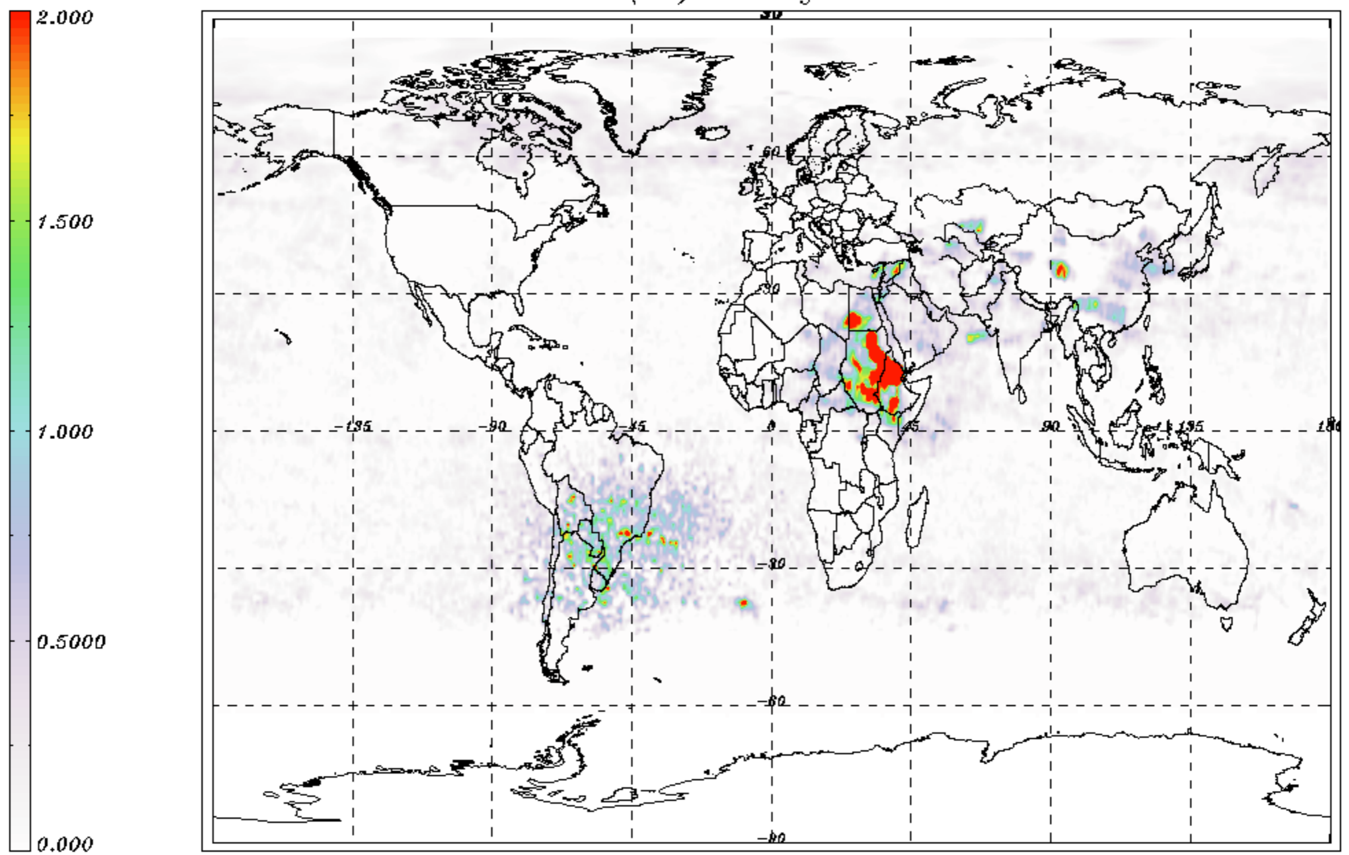
S02 UV7 VCD (DU) monthly mean - June 2011
