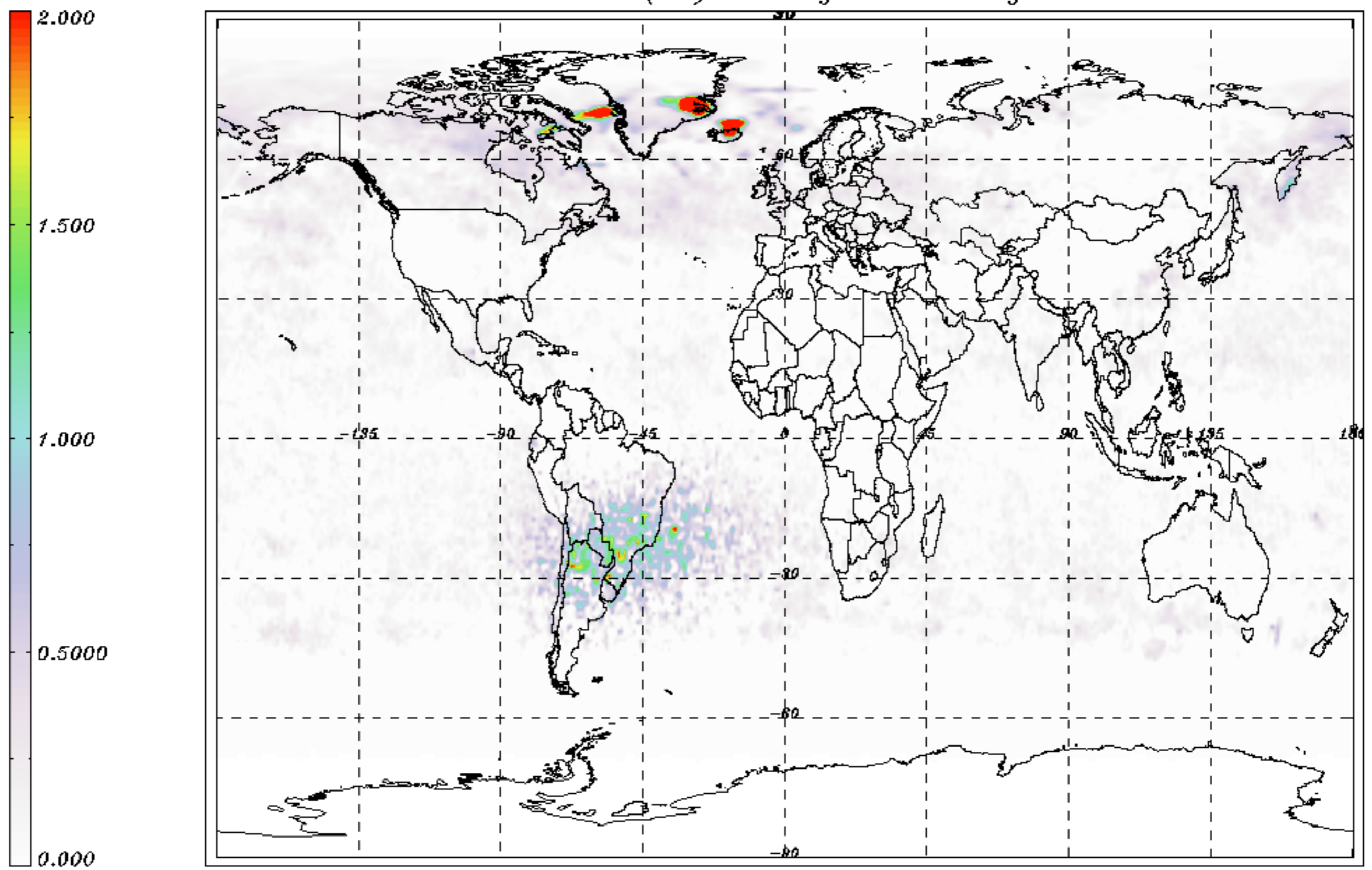
S02 UV7 VCD (DU) monthly mean - May 2011
