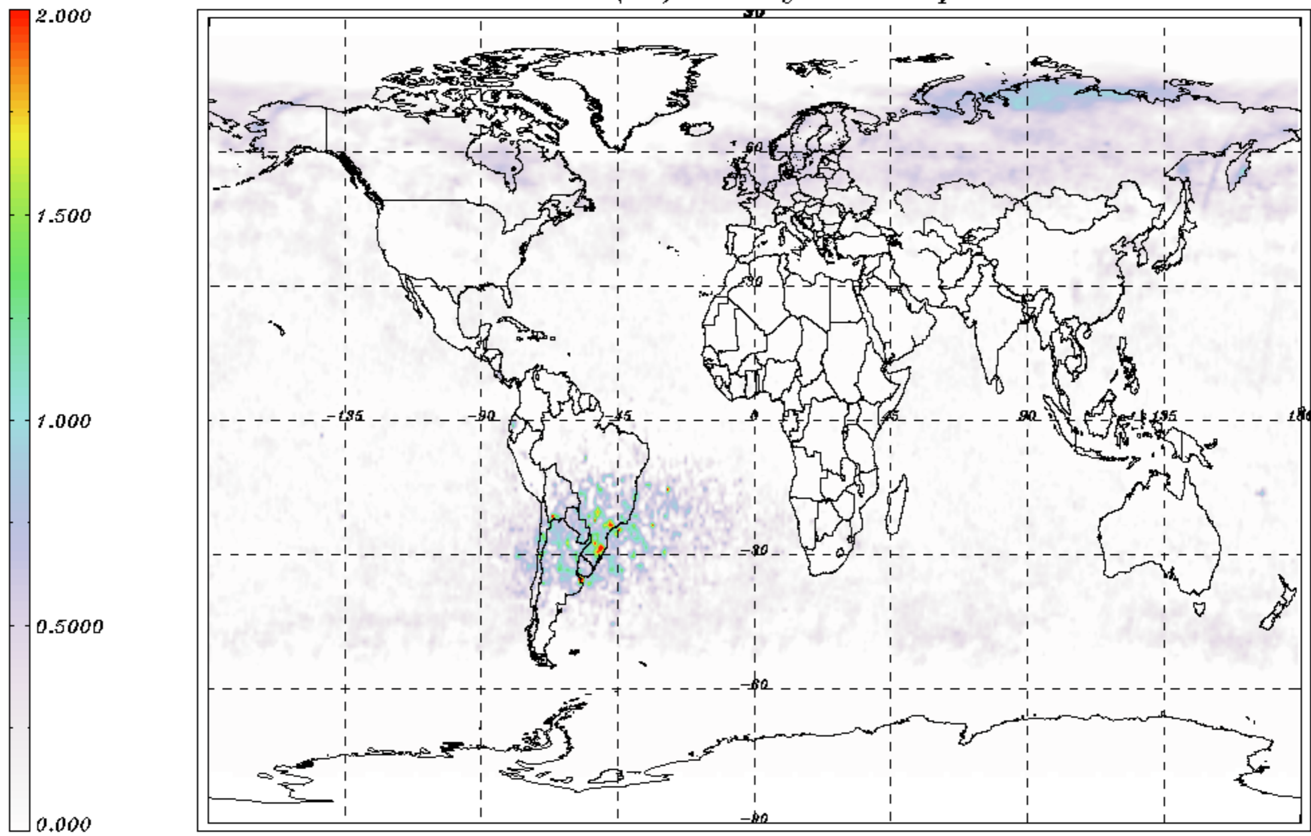
S02 UV7 VCD (DU) monthly mean - April 2011
