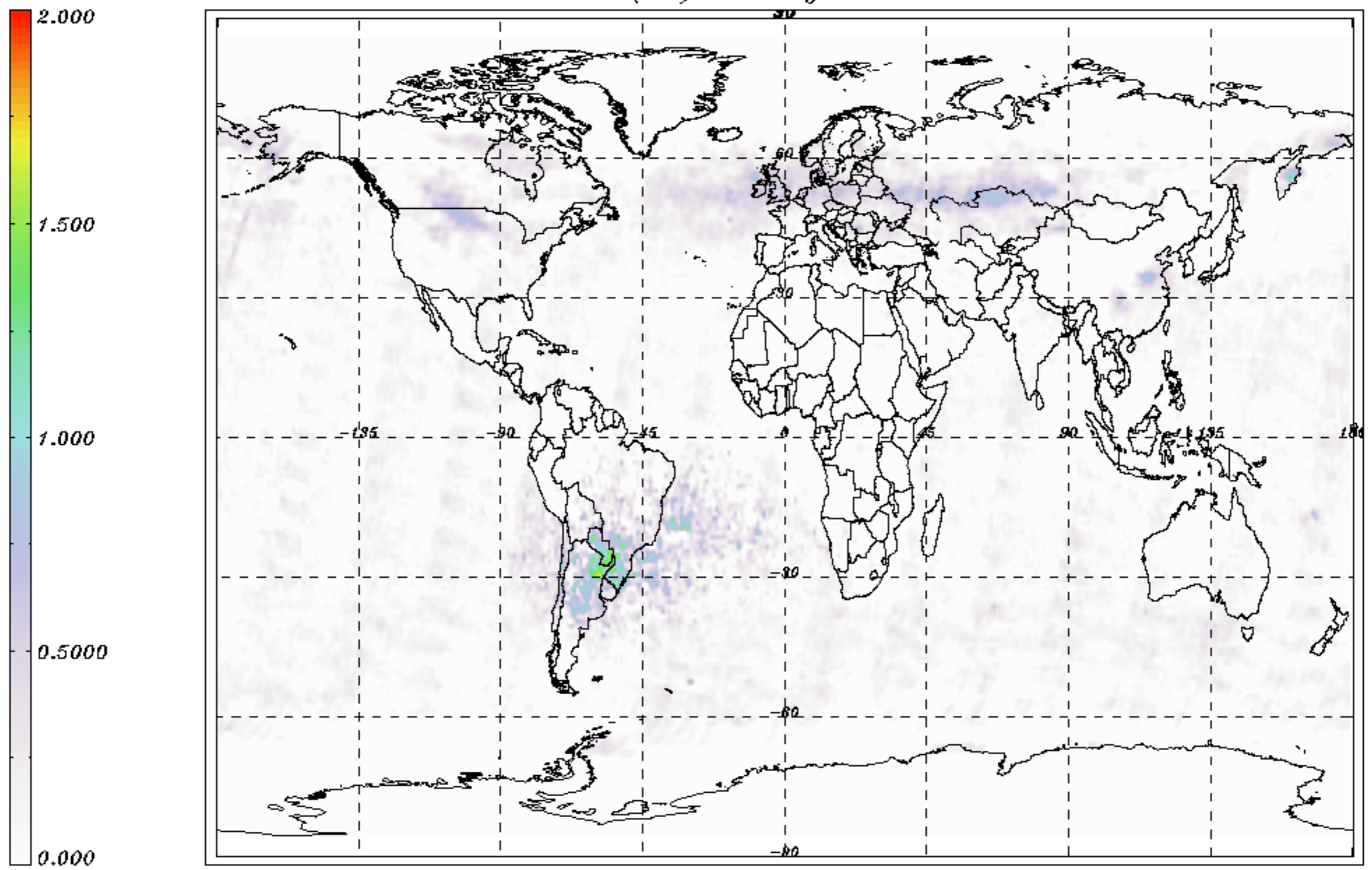
S02 UV7 VCD (DU) monthly mean - March 2011
