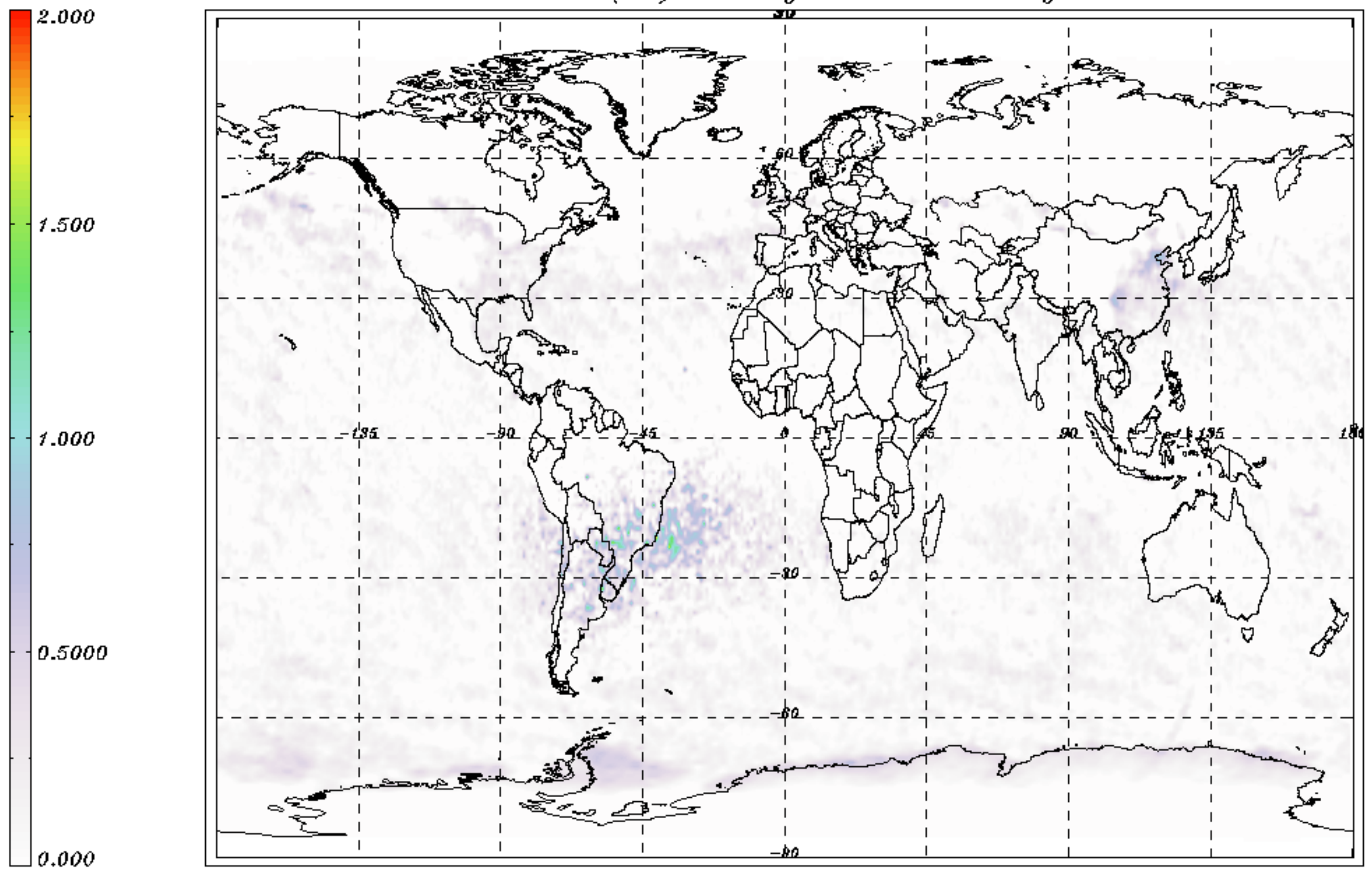
SO2 UV7 VCD (DU) monthly mean - February 2011
