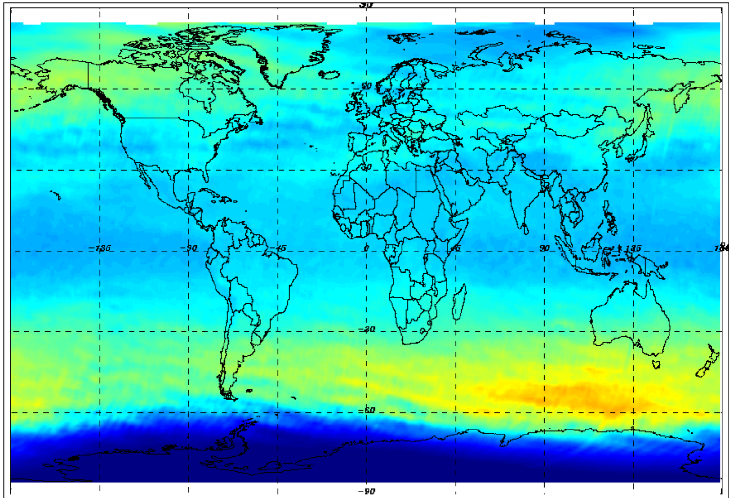
03 VCD (DU) monthly mean - October 2011
