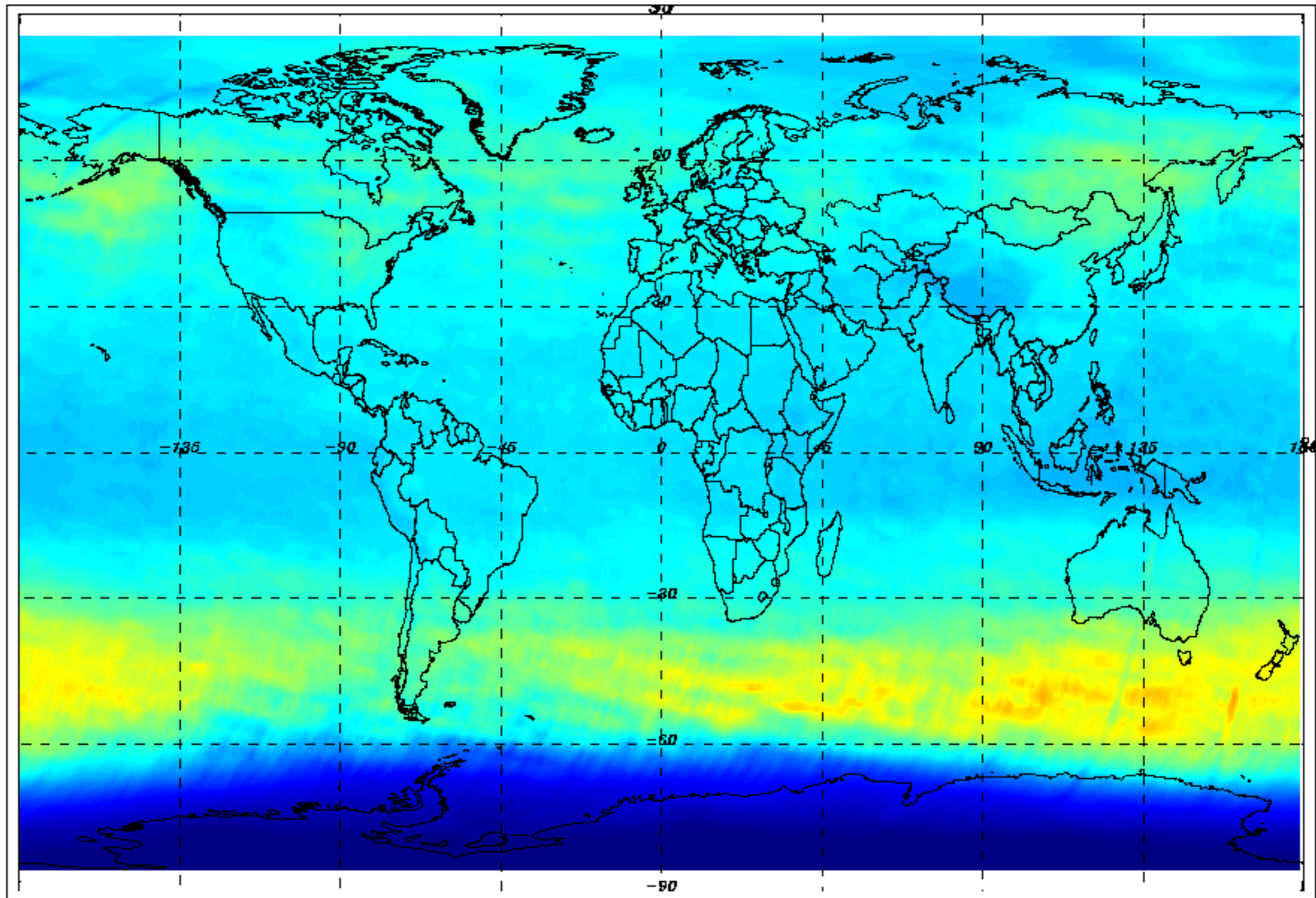
03 VCD (DU) monthly mean - September 2011
