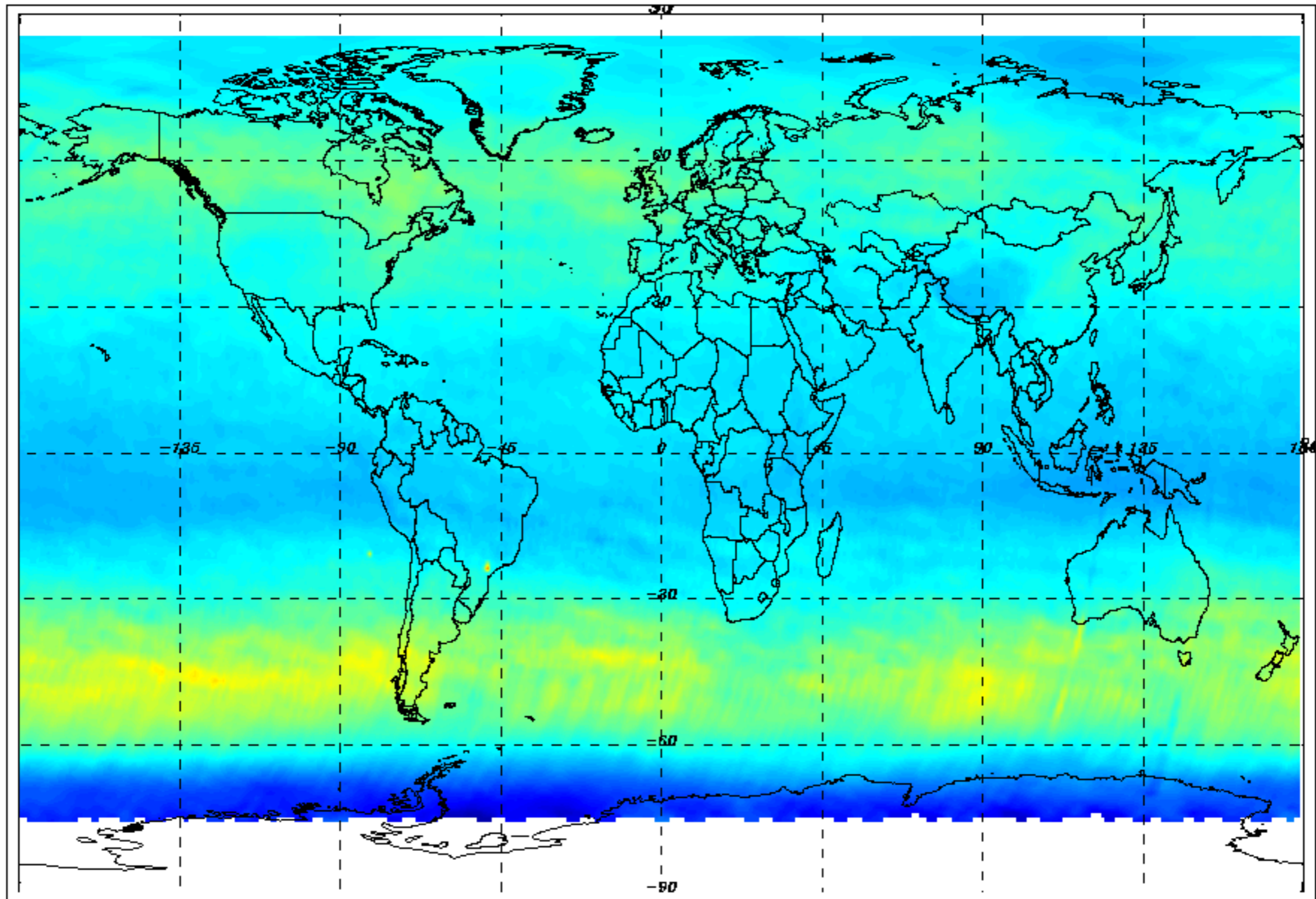
03 VCD (DU) monthly mean - August 2011
