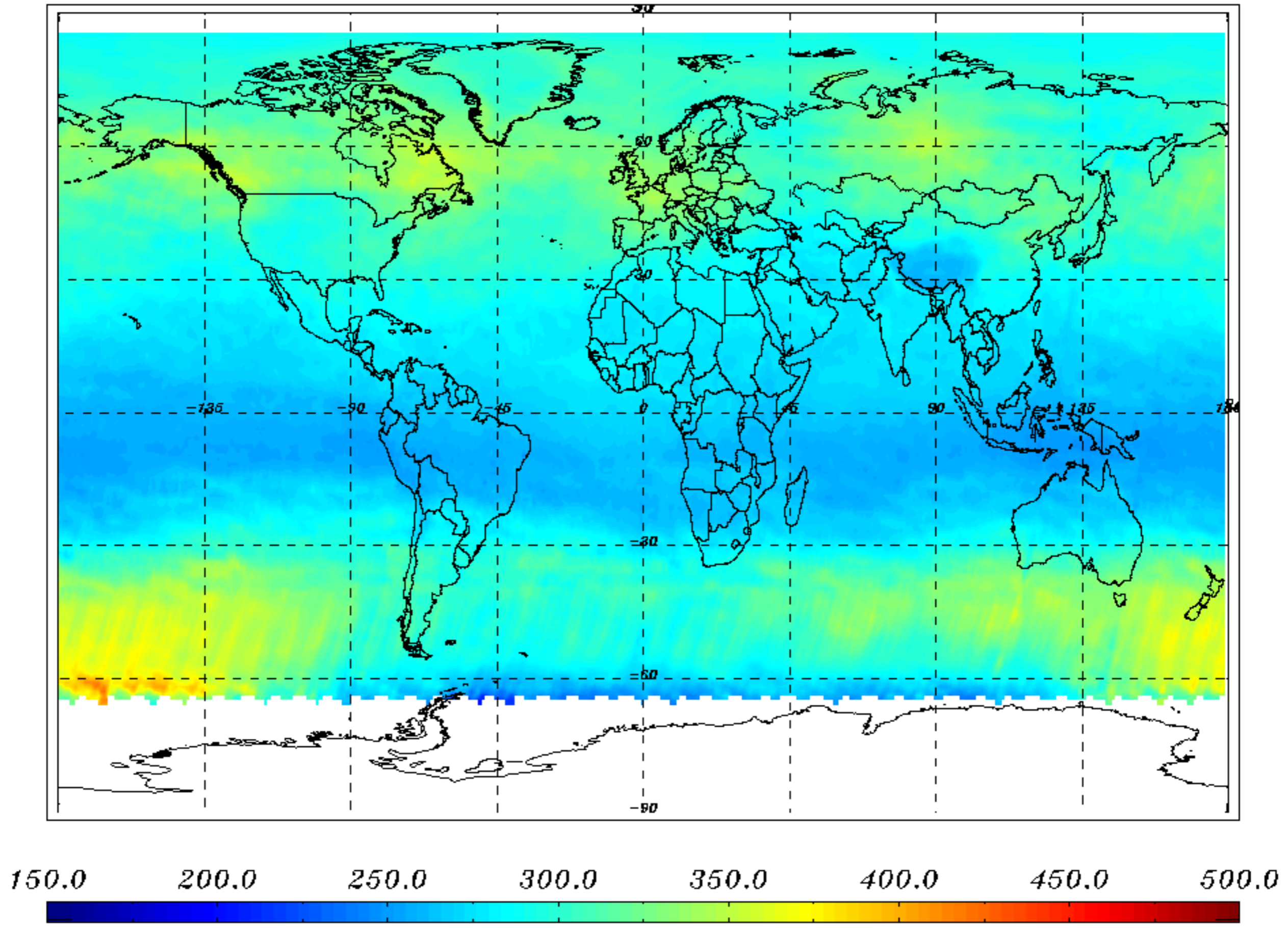
03 VCD (DU) monthly mean - July 2011
